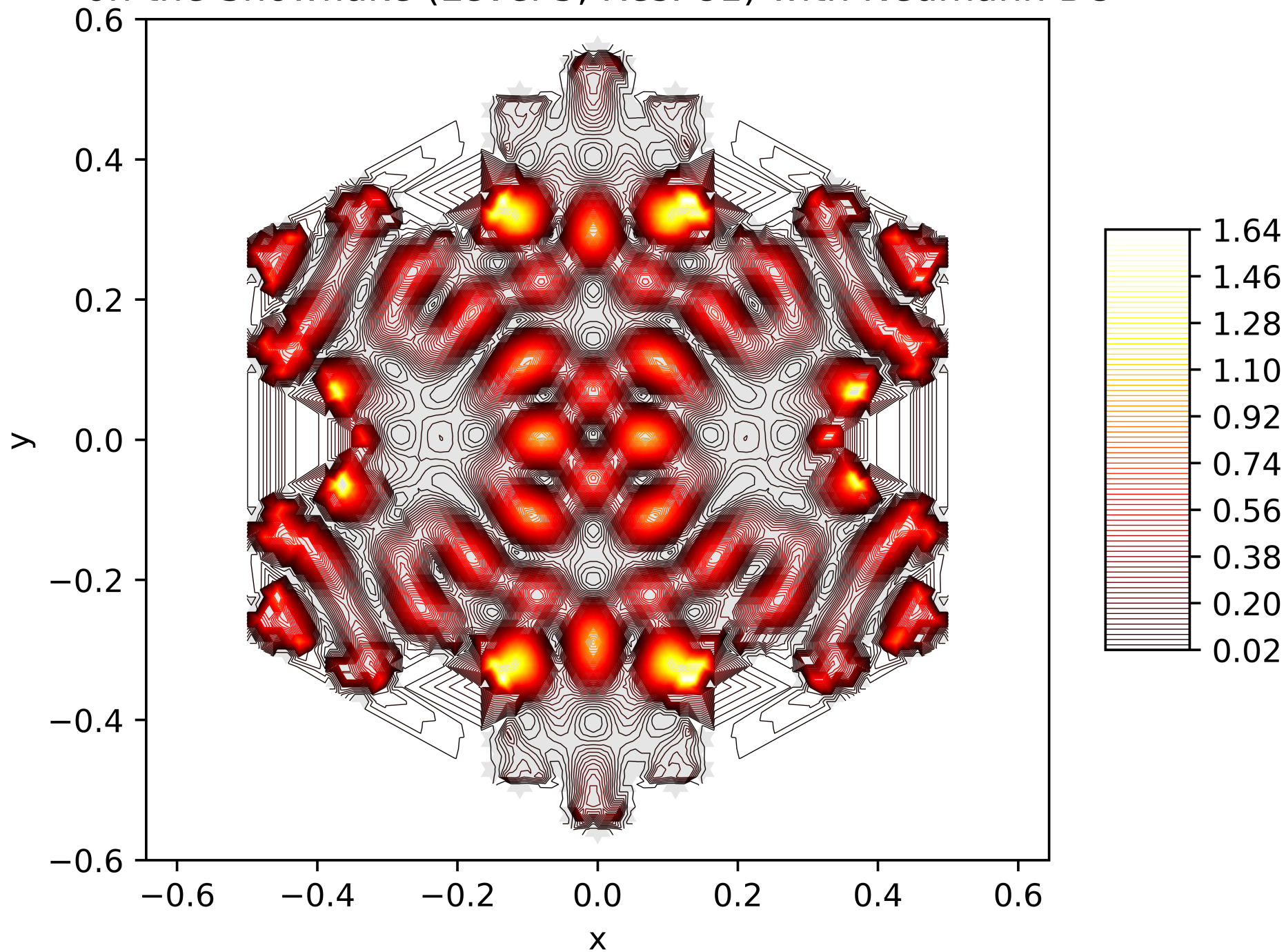
Contour Lines of the Energy Function of the 80. Eigenfunction on the Snowflake (Level 5, Res. 81) with Neumann BC
