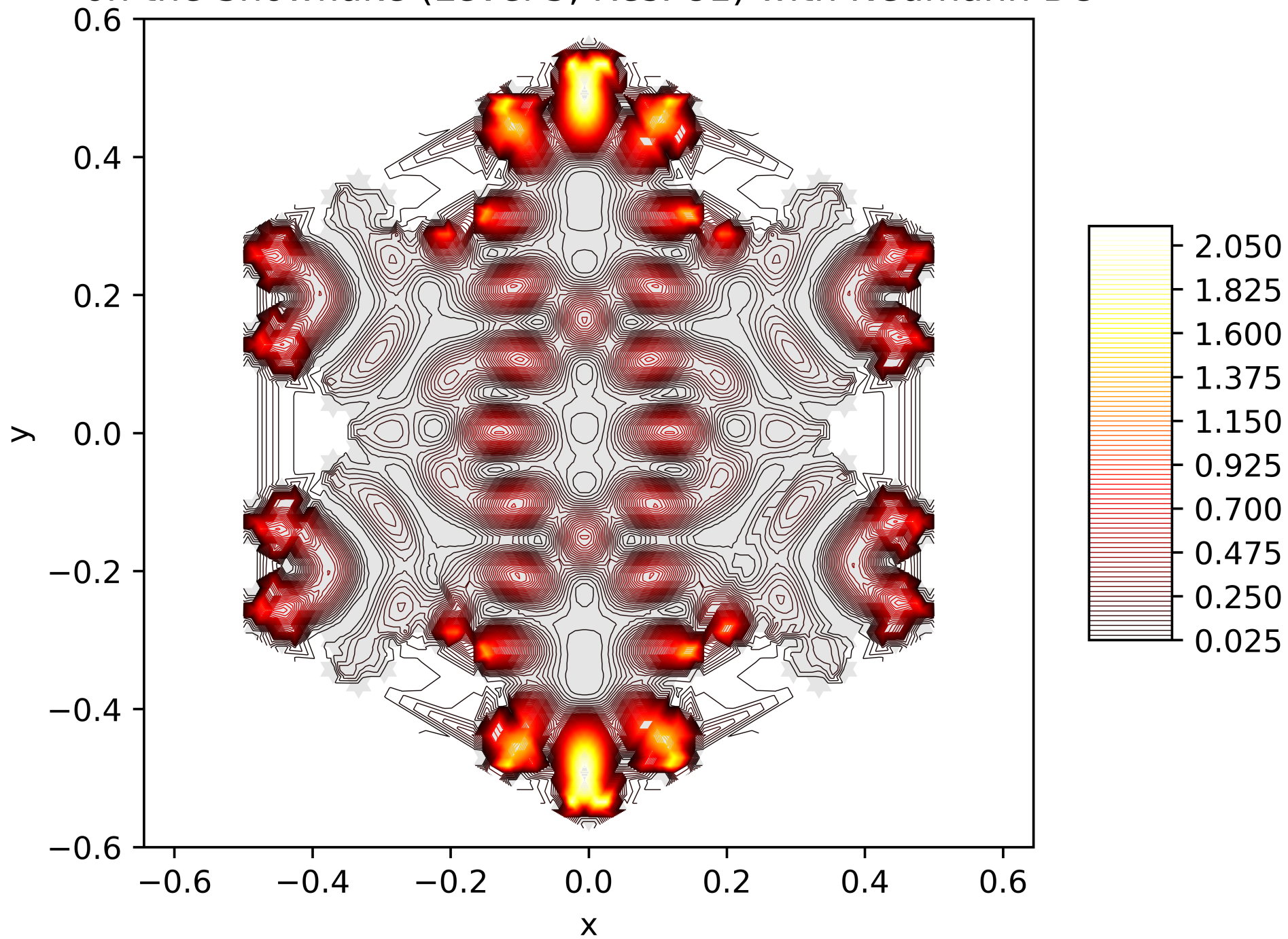
Contour Lines of the Energy Function of the 77. Eigenfunction on the Snowflake (Level 5, Res. 81) with Neumann BC
