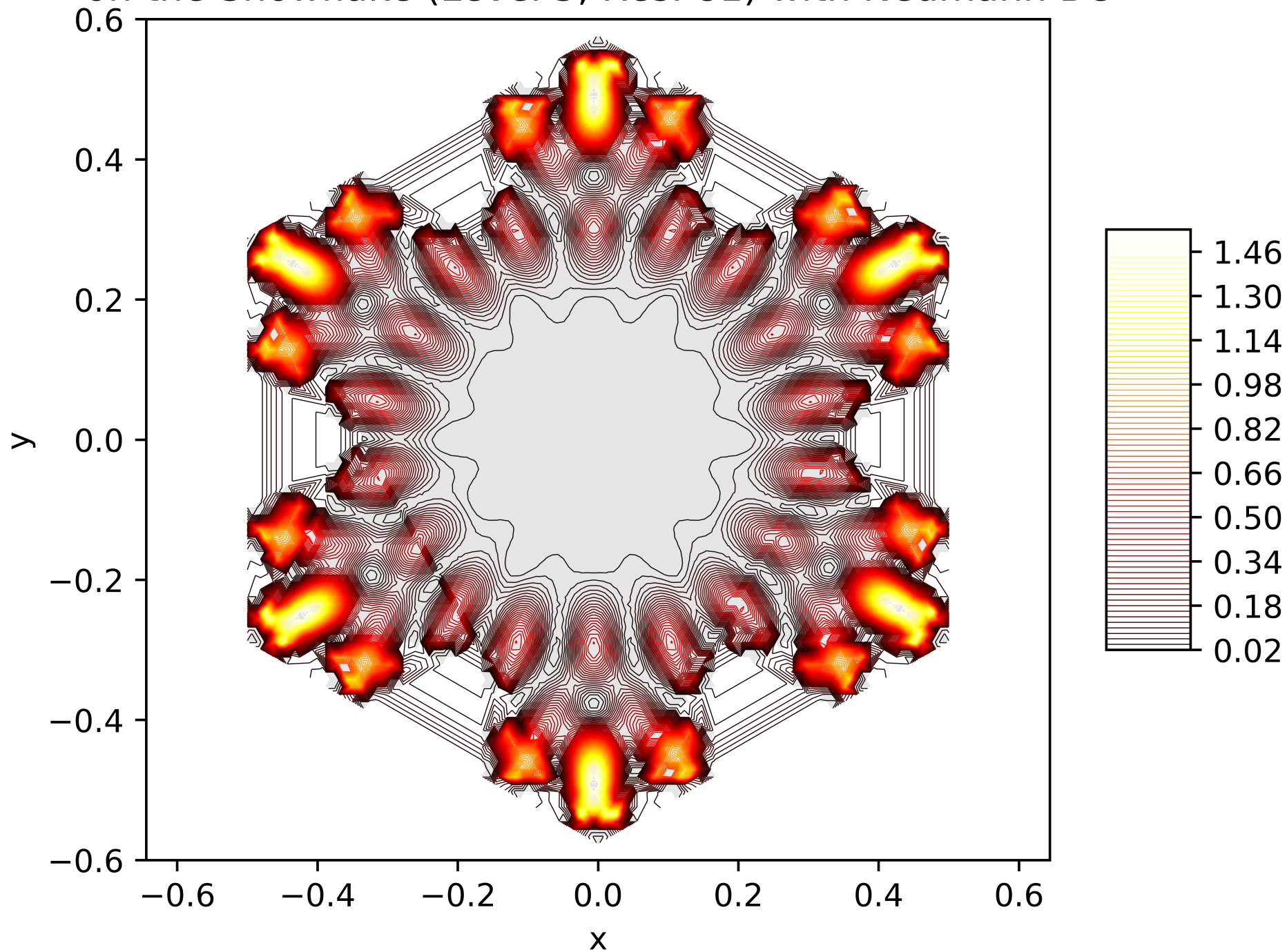
Contour Lines of the Energy Function of the 74. Eigenfunction on the Snowflake (Level 5, Res. 81) with Neumann BC
