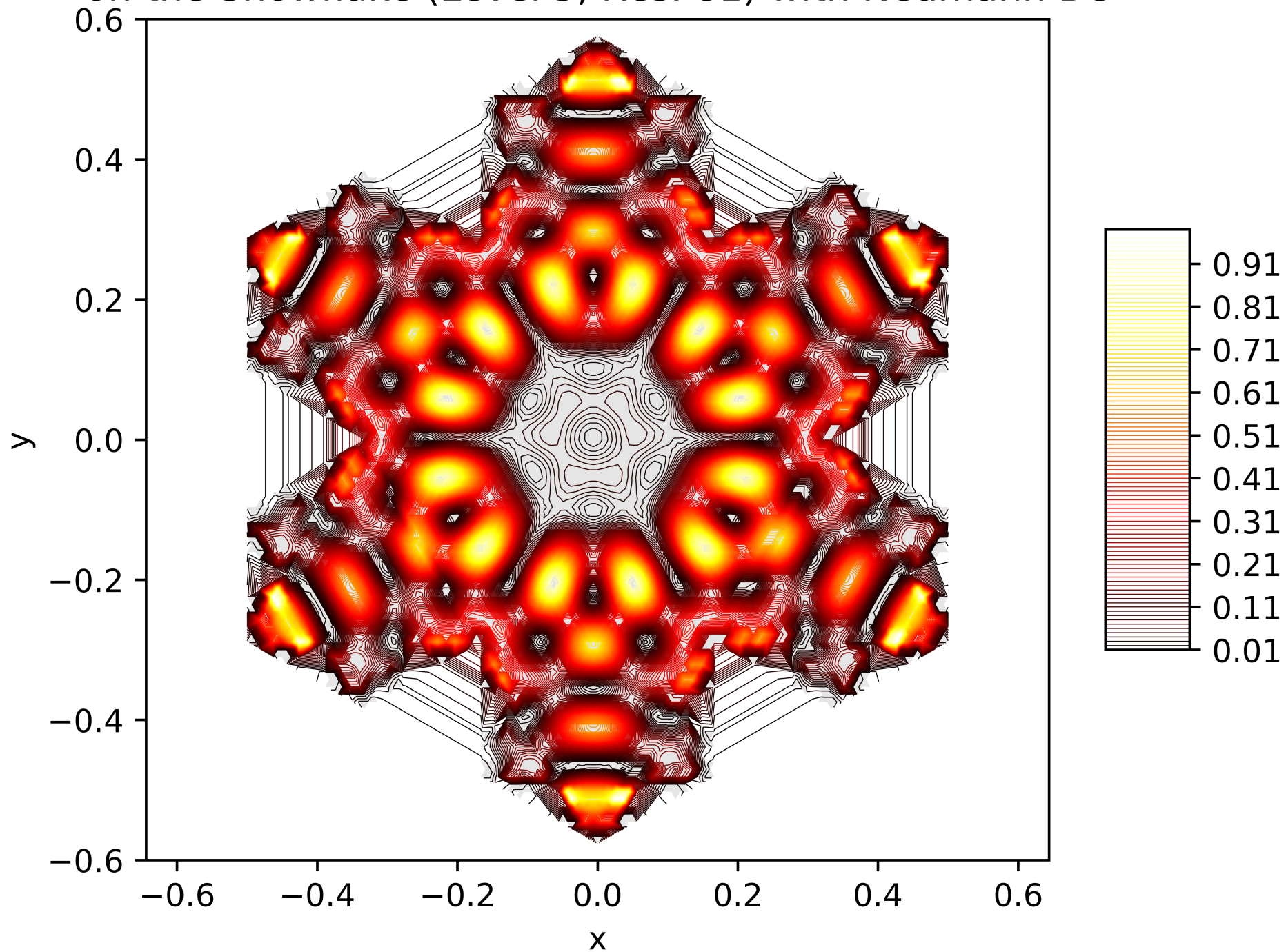
Contour Lines of the Energy Function of the 71. Eigenfunction on the Snowflake (Level 5, Res. 81) with Neumann BC
