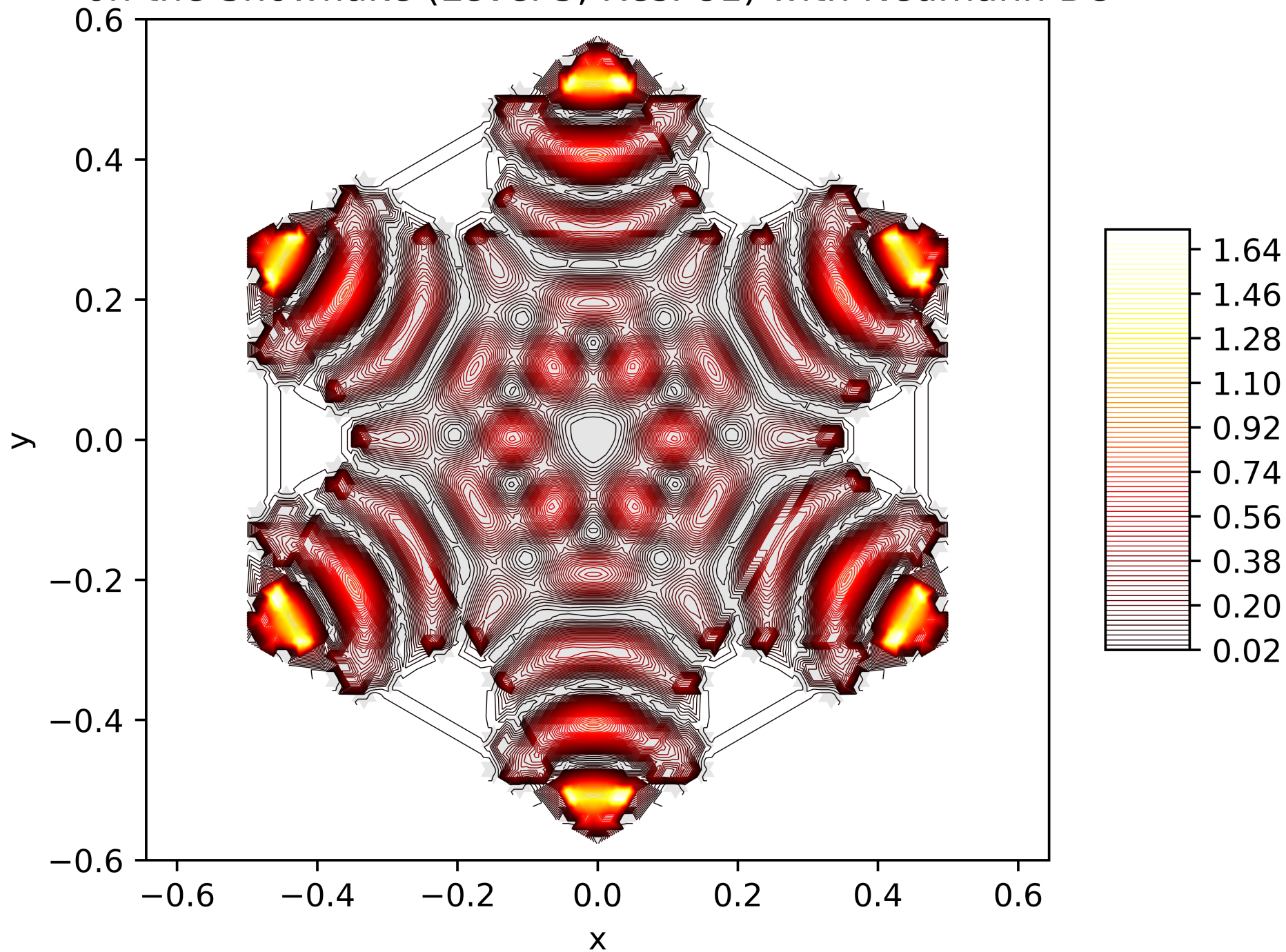
Contour Lines of the Energy Function of the 70. Eigenfunction on the Snowflake (Level 5, Res. 81) with Neumann BC
