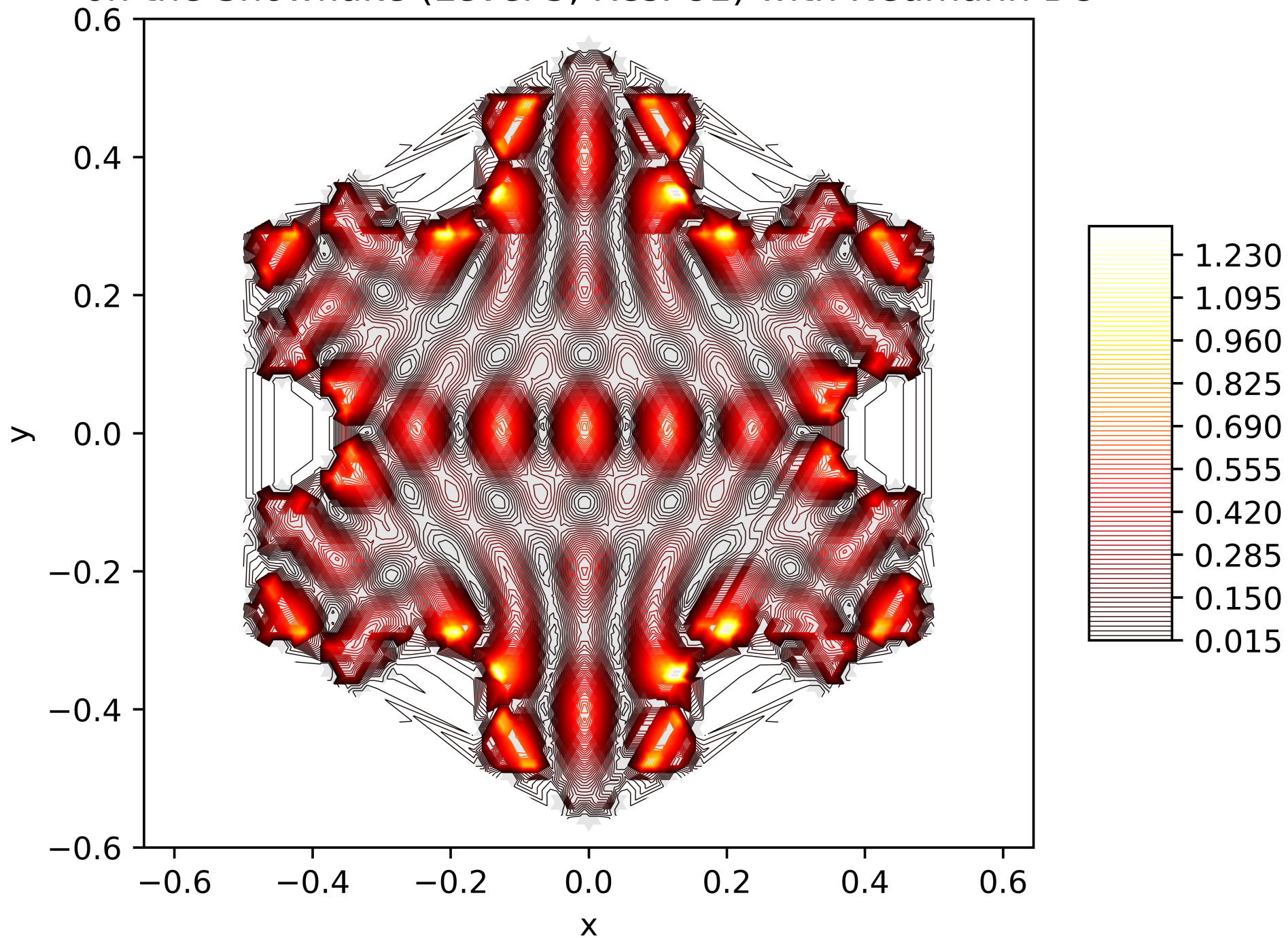
Contour Lines of the Energy Function of the 63. Eigenfunction on the Snowflake (Level 5, Res. 81) with Neumann BC
