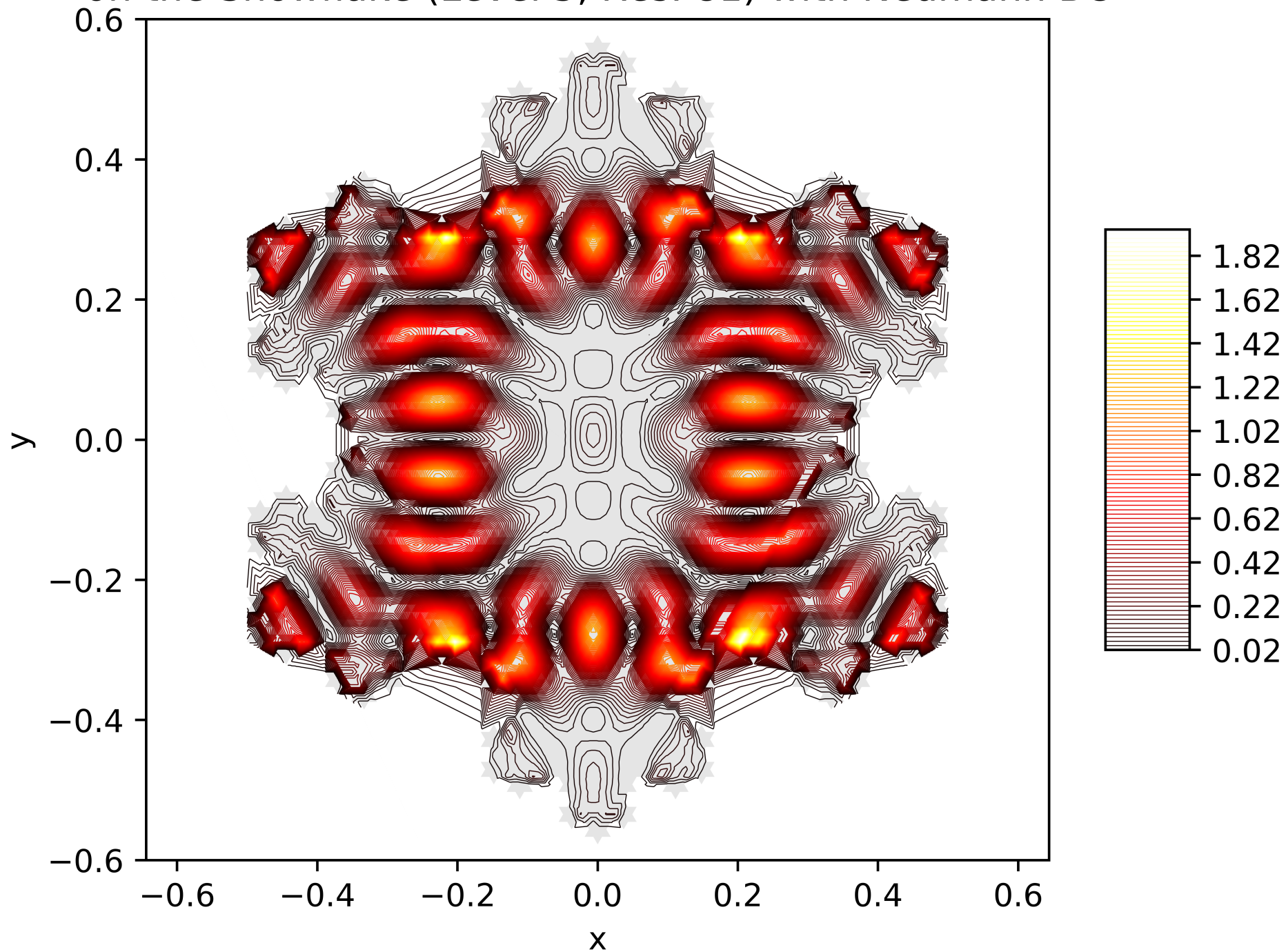
Contour Lines of the Energy Function of the 76. Eigenfunction on the Snowflake (Level 5, Res. 81) with Neumann BC
