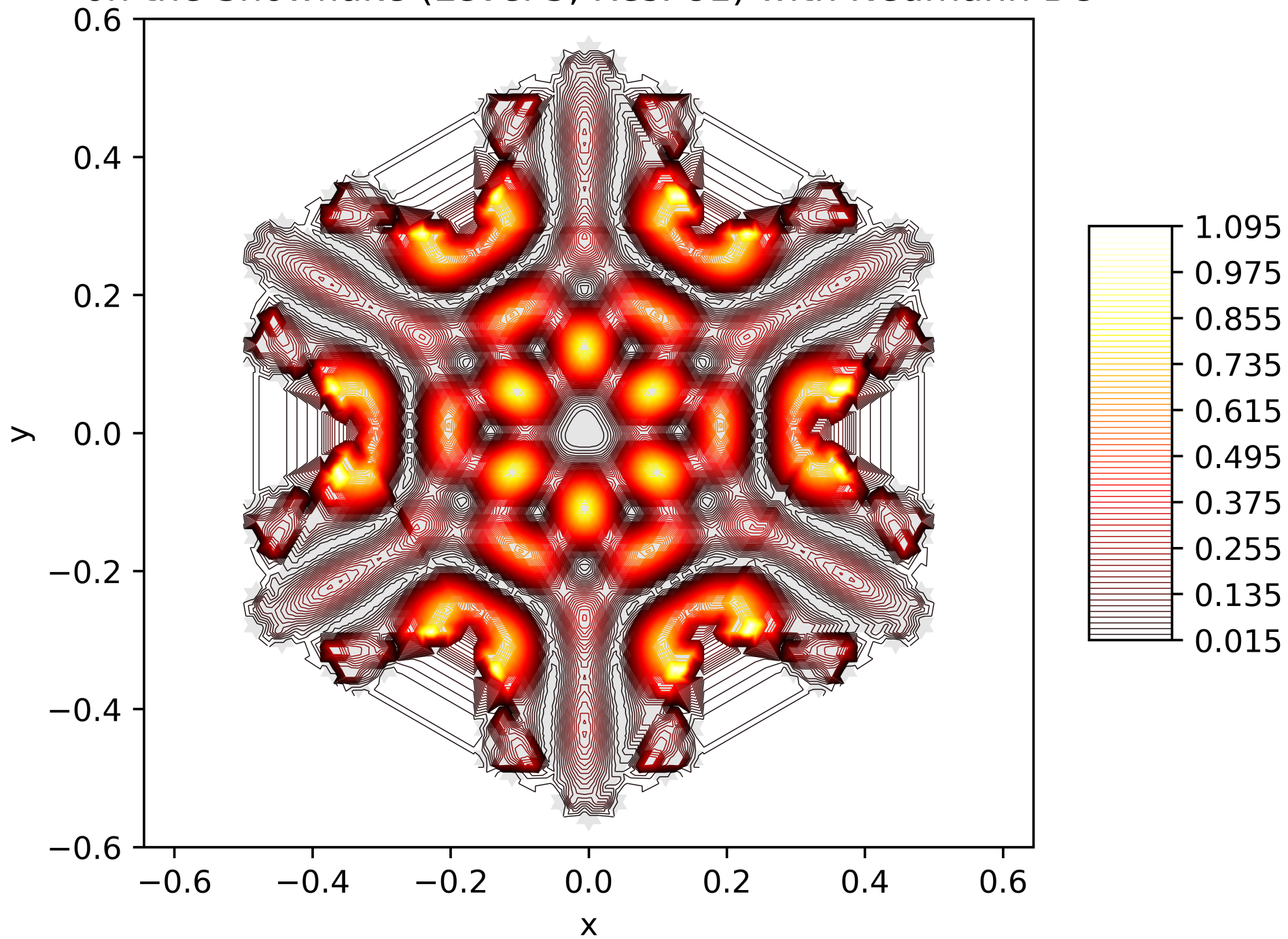
Contour Lines of the Energy Function of the 66. Eigenfunction on the Snowflake (Level 5, Res. 81) with Neumann BC
