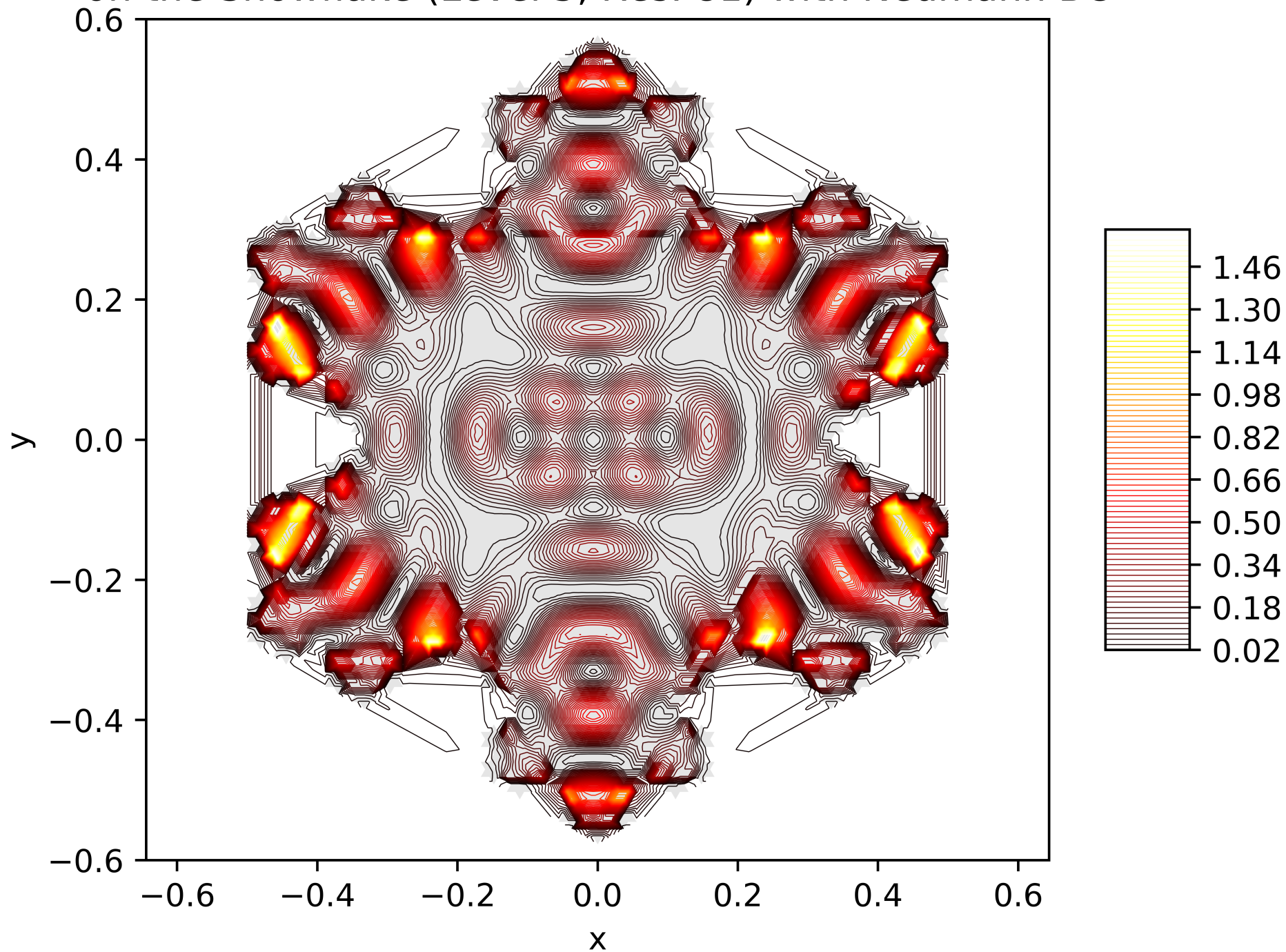
Contour Lines of the Energy Function of the 65. Eigenfunction on the Snowflake (Level 5, Res. 81) with Neumann BC
