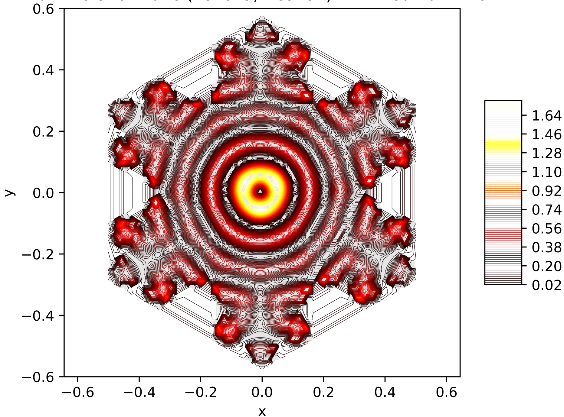
Contour Lines of the Energy Function of the 79. Eigenfunction on the Snowflake (Level 5, Res. 81) with Neumann BC
