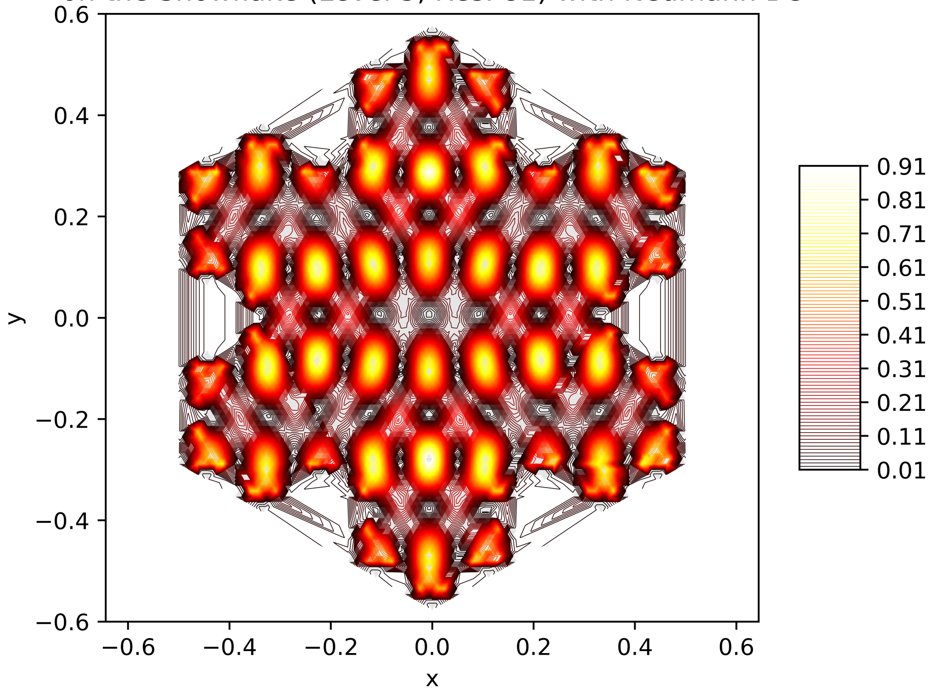
Contour Lines of the Energy Function of the 73. Eigenfunction on the Snowflake (Level 5, Res. 81) with Neumann BC
