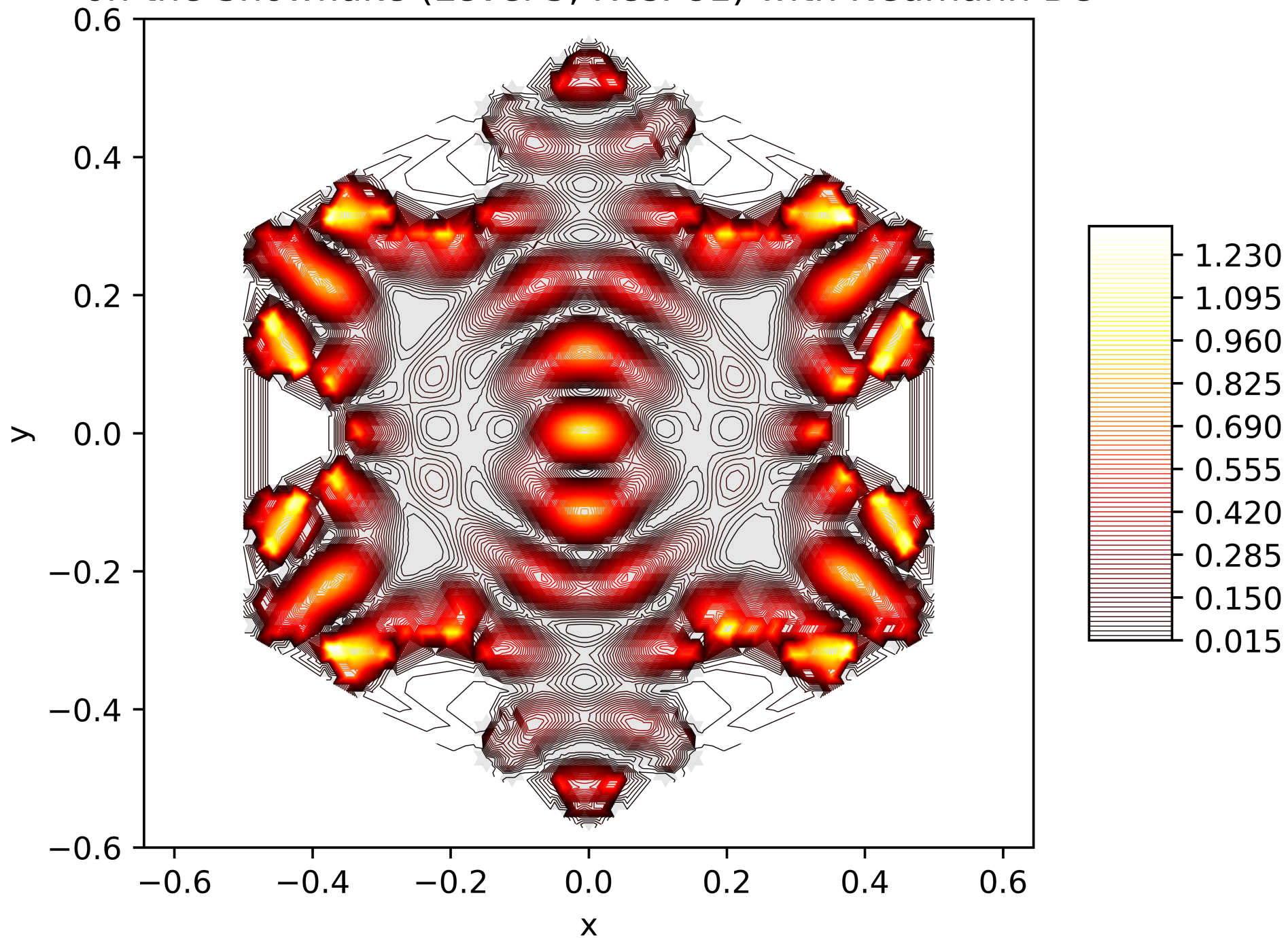
Contour Lines of the Energy Function of the 67. Eigenfunction on the Snowflake (Level 5, Res. 81) with Neumann BC
