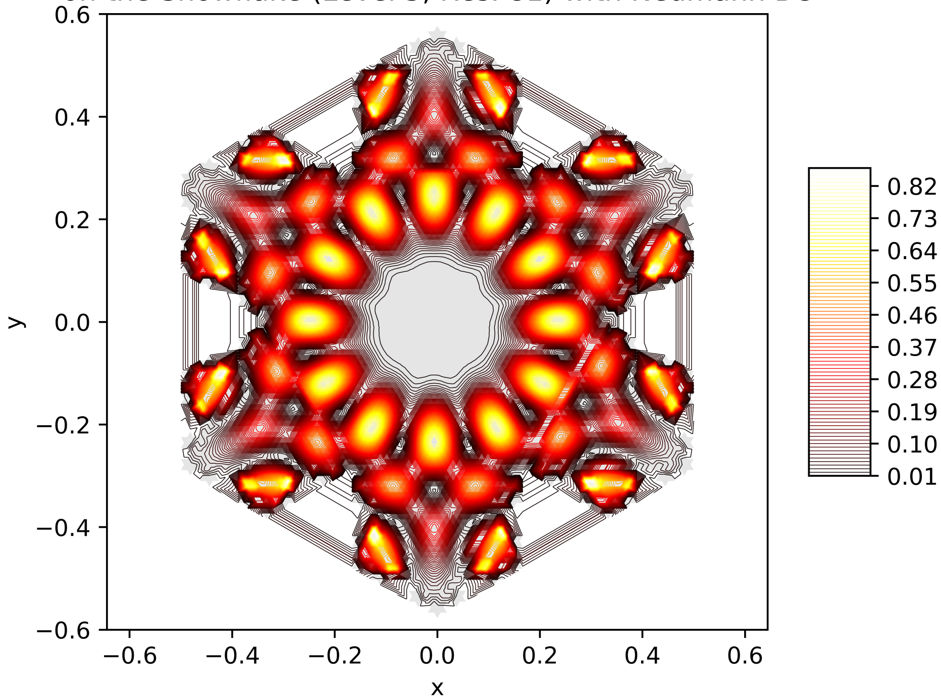
Contour Lines of the Energy Function of the 61. Eigenfunction on the Snowflake (Level 5, Res. 81) with Neumann BC
