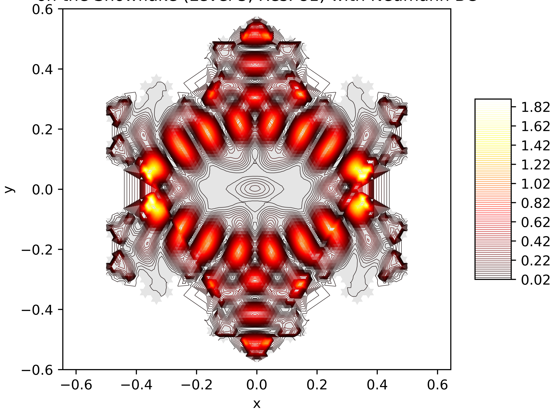
Contour Lines of the Energy Function of the 75. Eigenfunction on the Snowflake (Level 5, Res. 81) with Neumann BC
