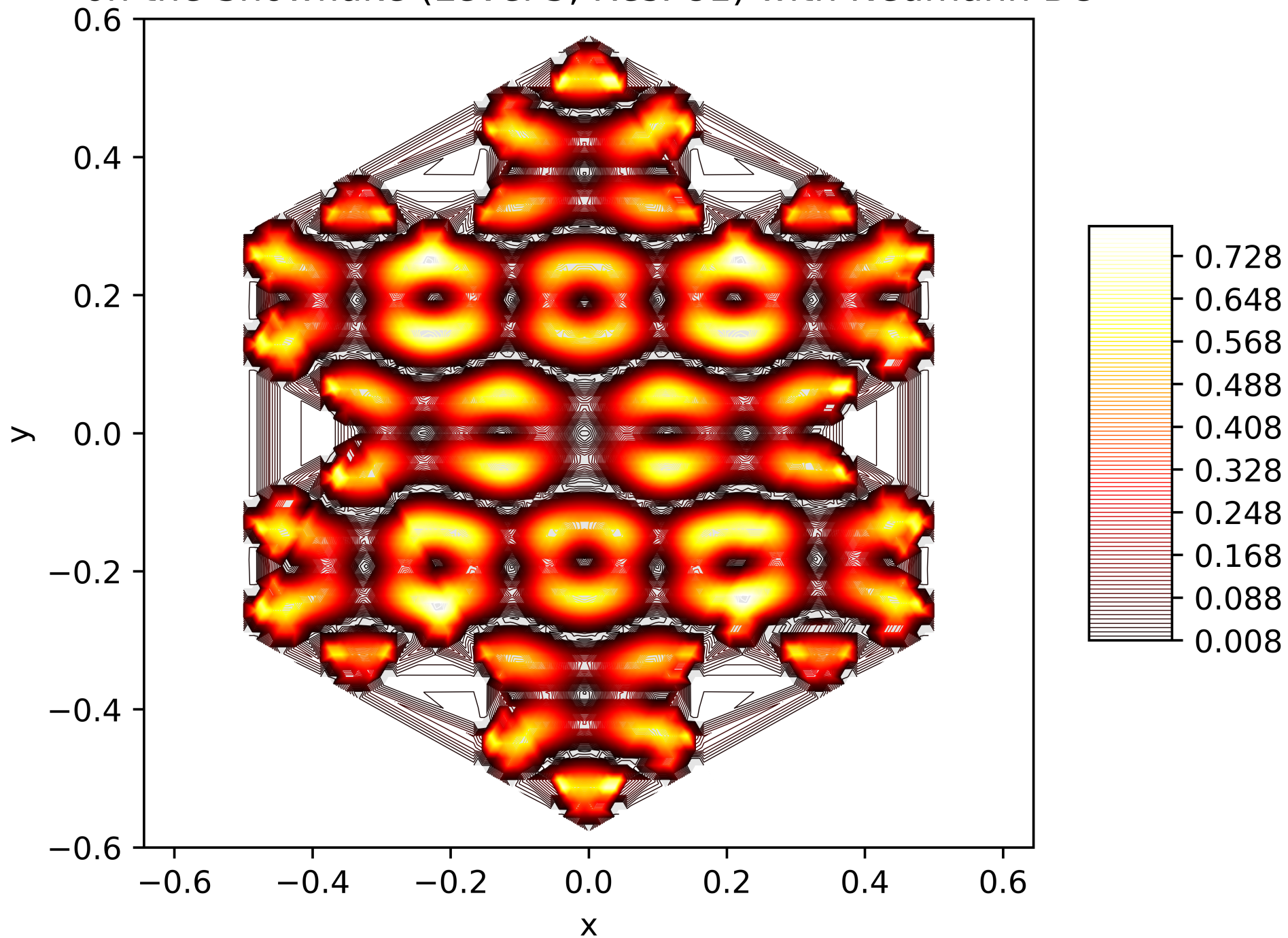
Contour Lines of the Energy Function of the 72. Eigenfunction on the Snowflake (Level 5, Res. 81) with Neumann BC
