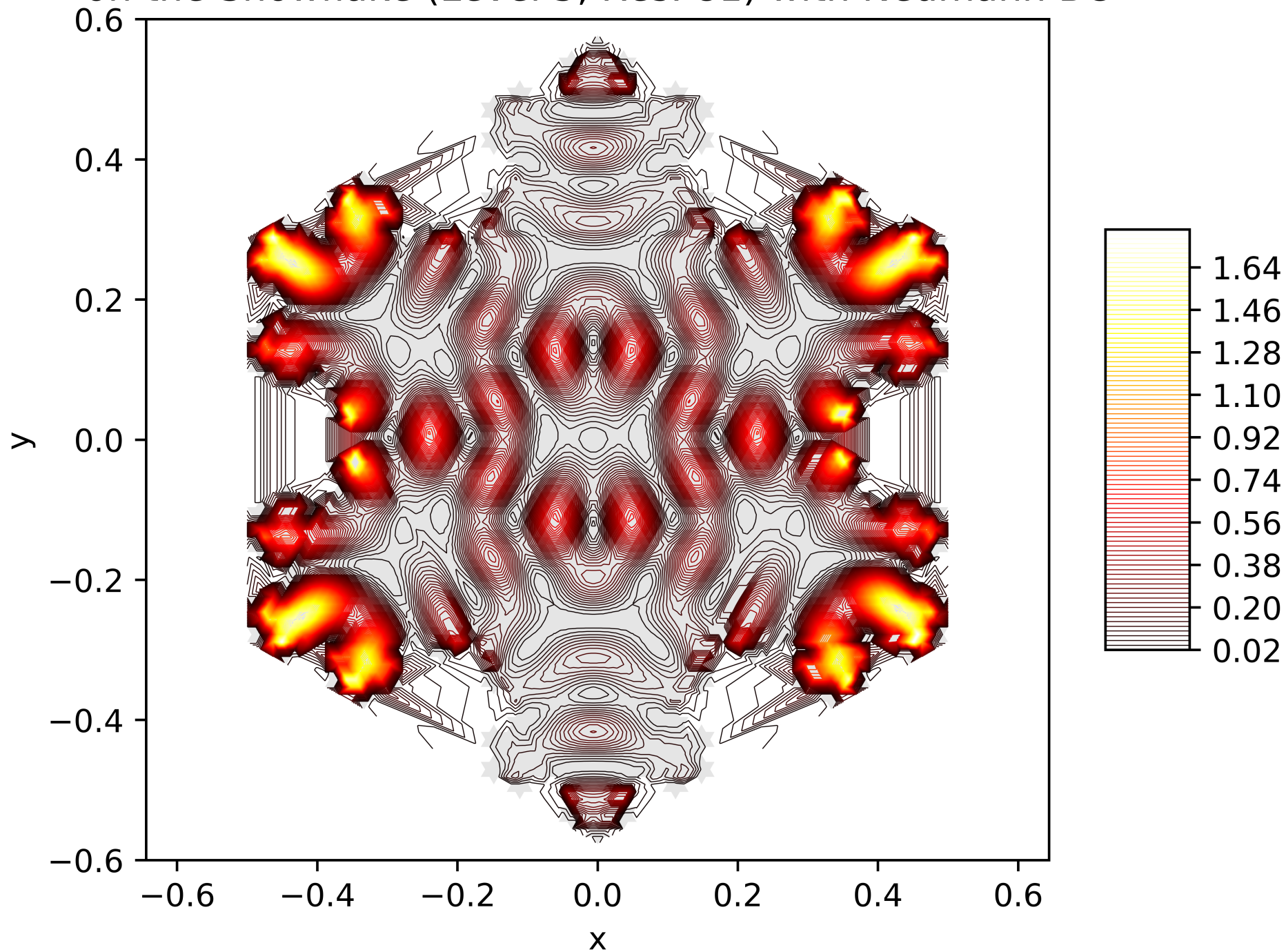
Contour Lines of the Energy Function of the 78. Eigenfunction on the Snowflake (Level 5, Res. 81) with Neumann BC
