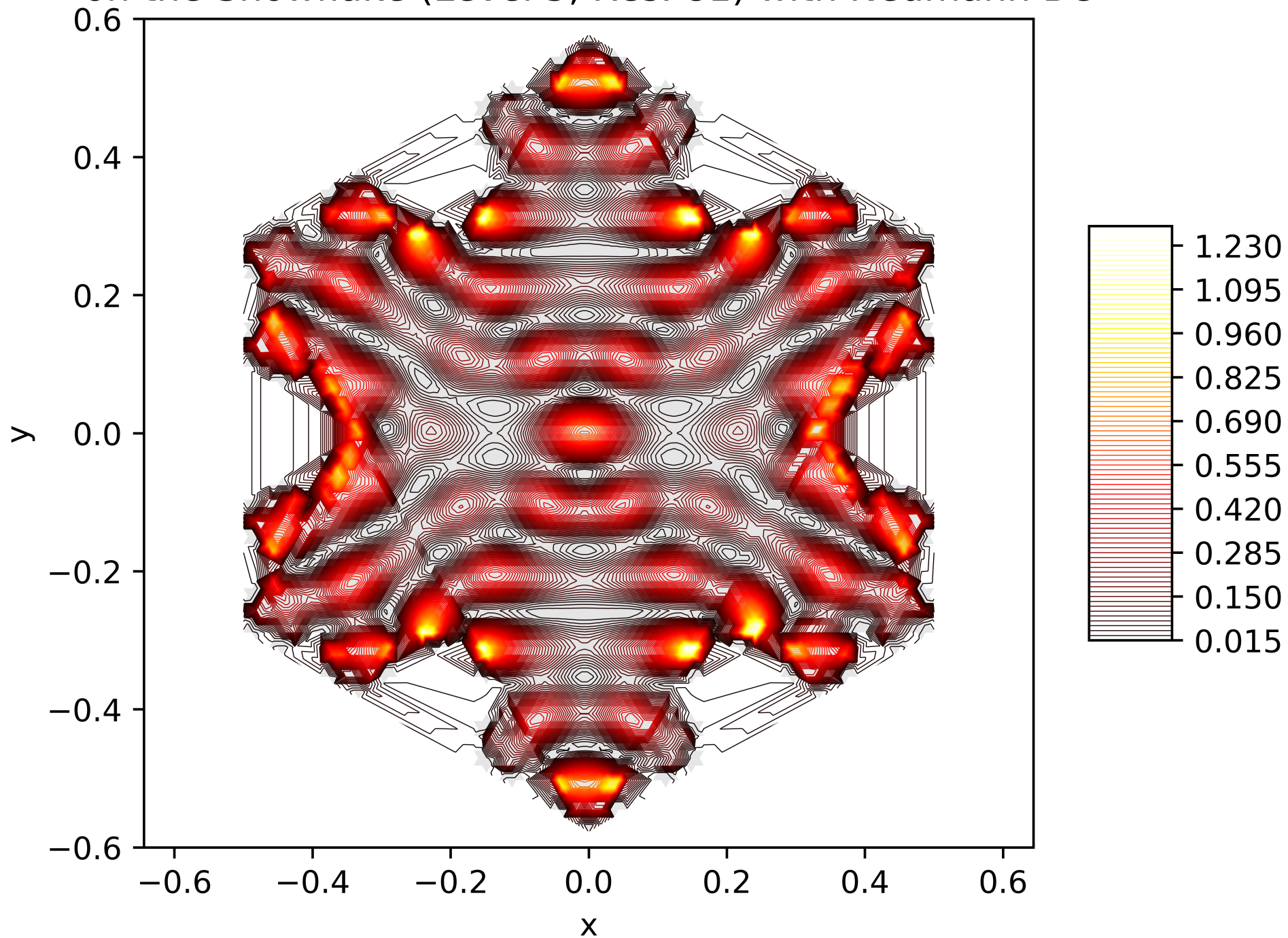
Contour Lines of the Energy Function of the 62. Eigenfunction on the Snowflake (Level 5, Res. 81) with Neumann BC
