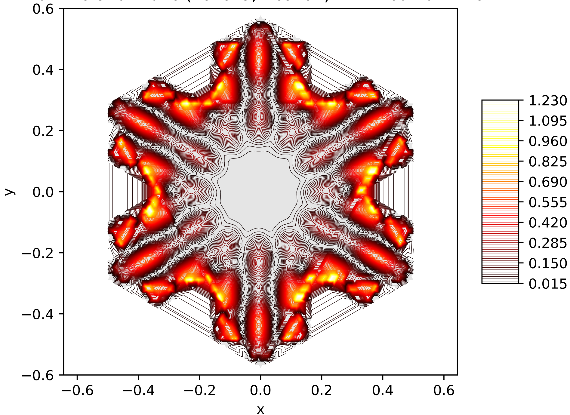
Contour Lines of the Energy Function of the 69. Eigenfunction on the Snowflake (Level 5, Res. 81) with Neumann BC
