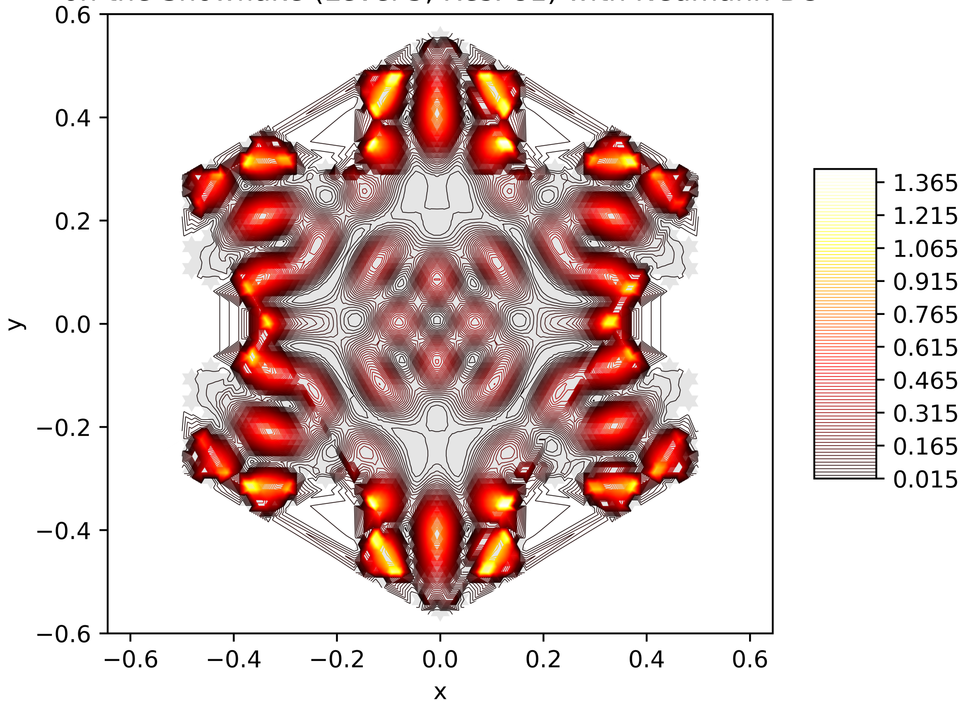
Contour Lines of the Energy Function of the 64. Eigenfunction on the Snowflake (Level 5, Res. 81) with Neumann BC
