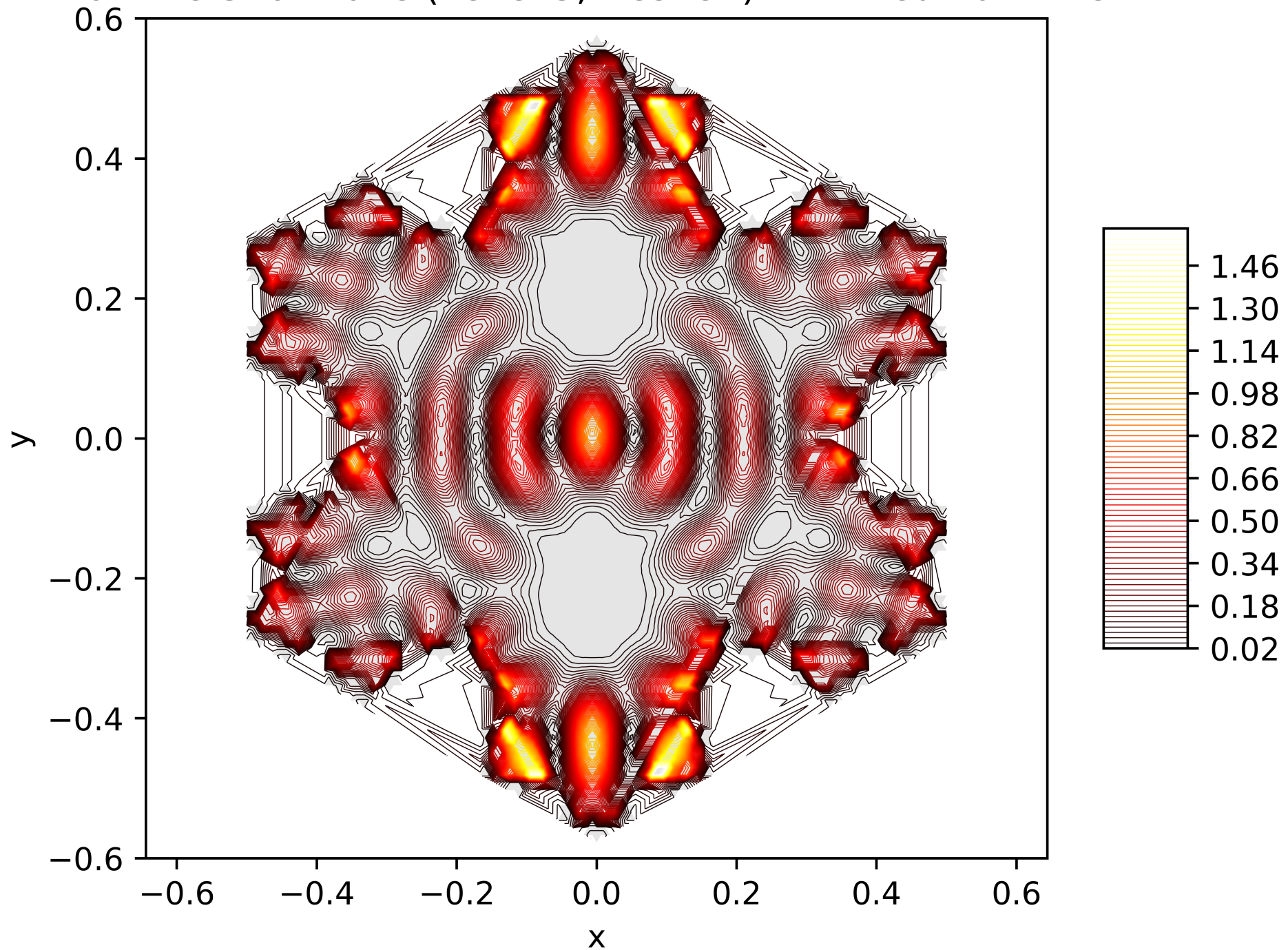
Contour Lines of the Energy Function of the 68. Eigenfunction on the Snowflake (Level 5, Res. 81) with Neumann BC
