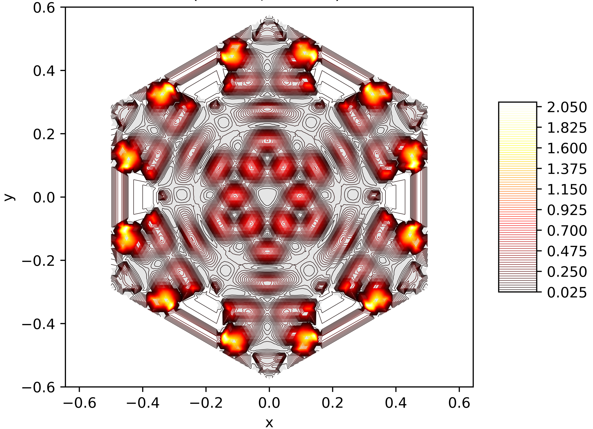
Contour Lines of the Energy Function of the 87. Eigenfunction on the Snowflake (Level 5, Res. 81) with Neumann BC
