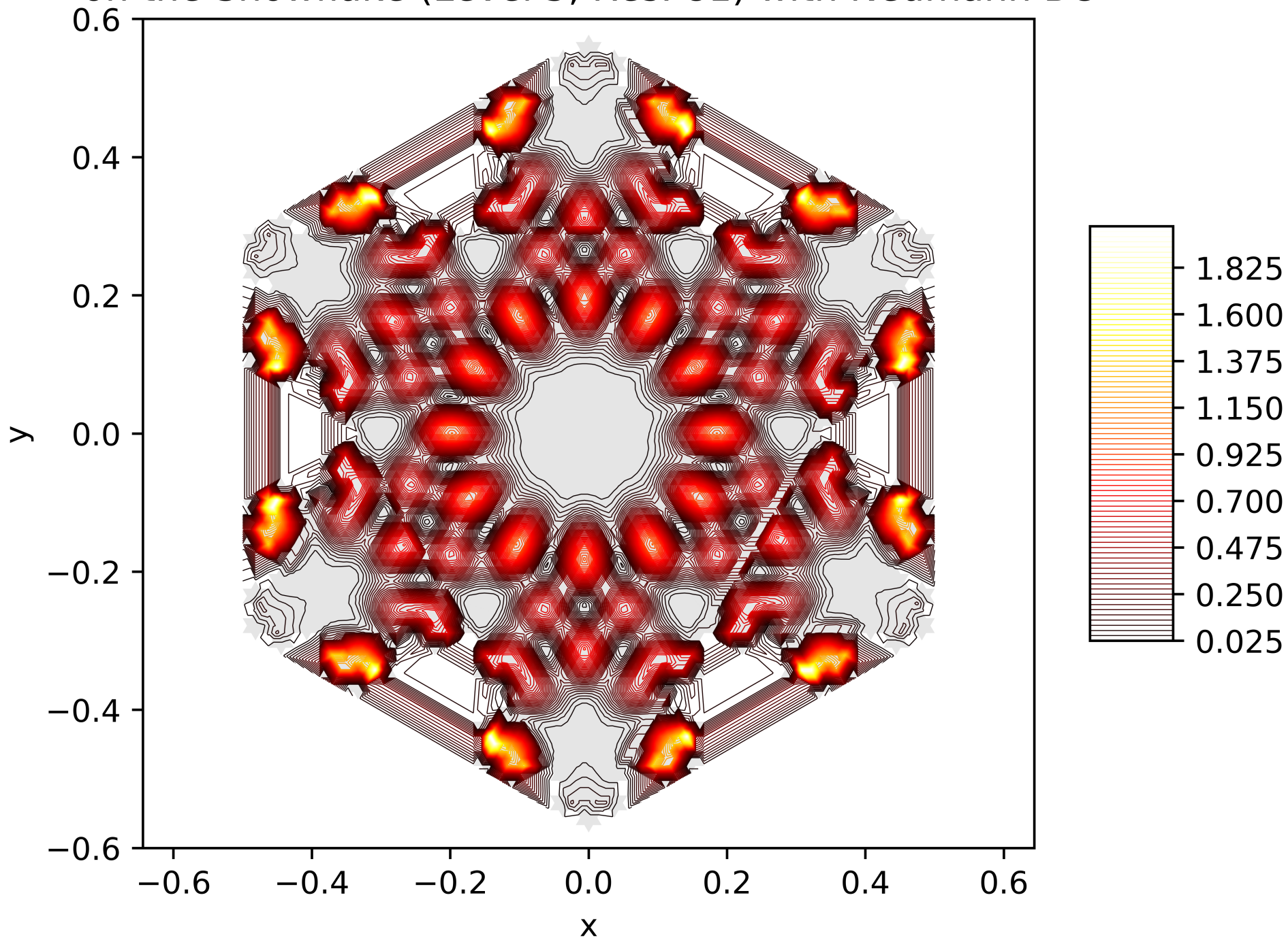
Contour Lines of the Energy Function of the 96. Eigenfunction on the Snowflake (Level 5, Res. 81) with Neumann BC
