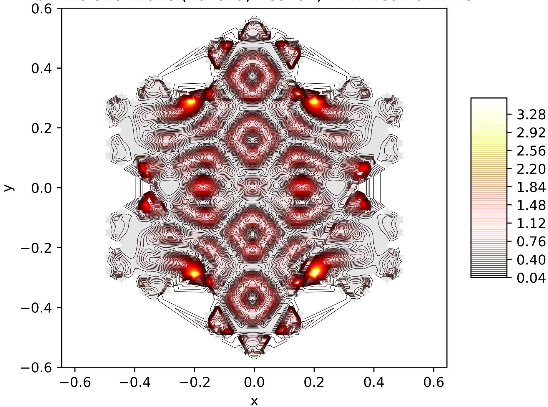
Contour Lines of the Energy Function of the 91. Eigenfunction on the Snowflake (Level 5, Res. 81) with Neumann BC
