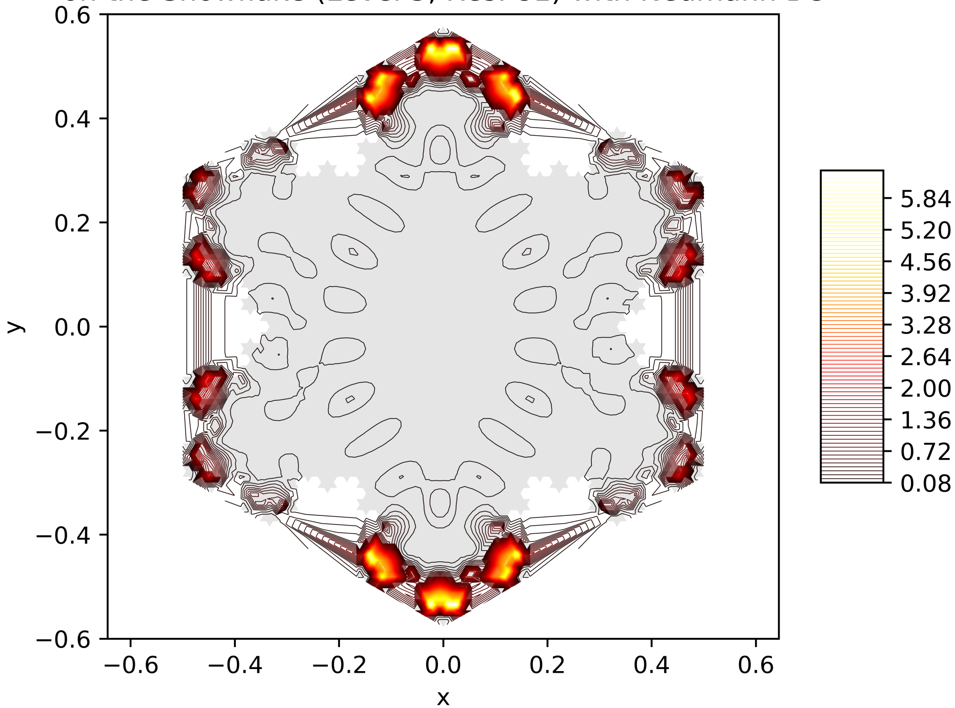
Contour Lines of the Energy Function of the 99. Eigenfunction on the Snowflake (Level 5, Res. 81) with Neumann BC
