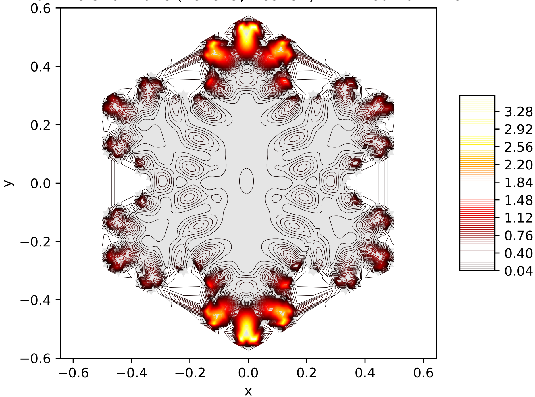
Contour Lines of the Energy Function of the 82. Eigenfunction on the Snowflake (Level 5, Res. 81) with Neumann BC
