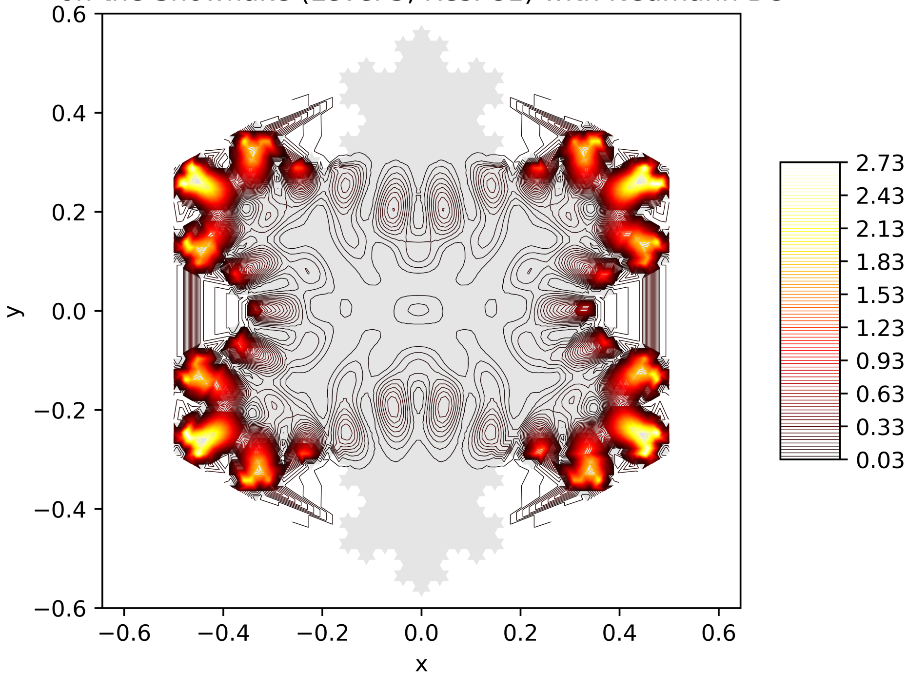
Contour Lines of the Energy Function of the 83. Eigenfunction on the Snowflake (Level 5, Res. 81) with Neumann BC
