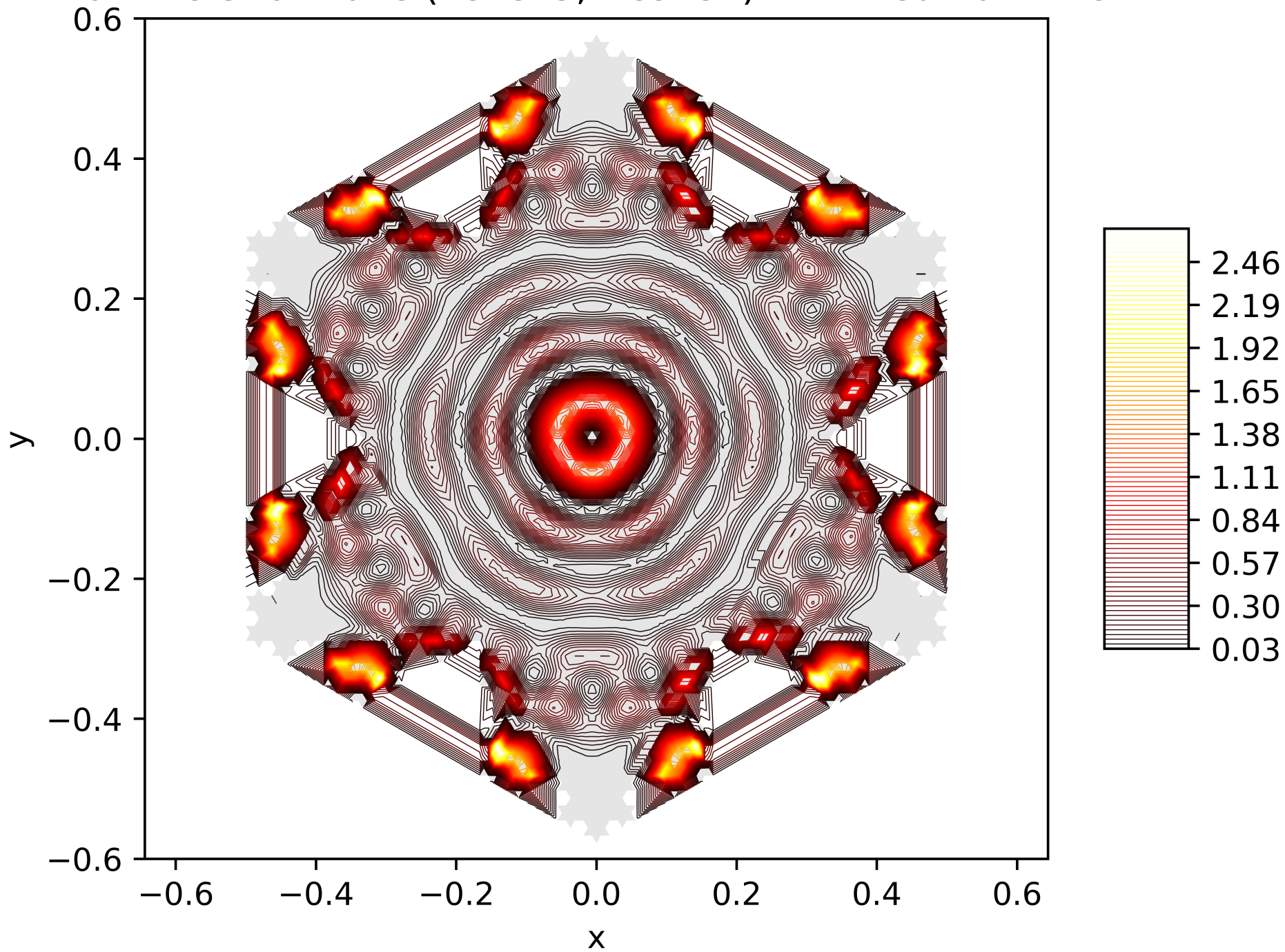
Contour Lines of the Energy Function of the 95. Eigenfunction on the Snowflake (Level 5, Res. 81) with Neumann BC
