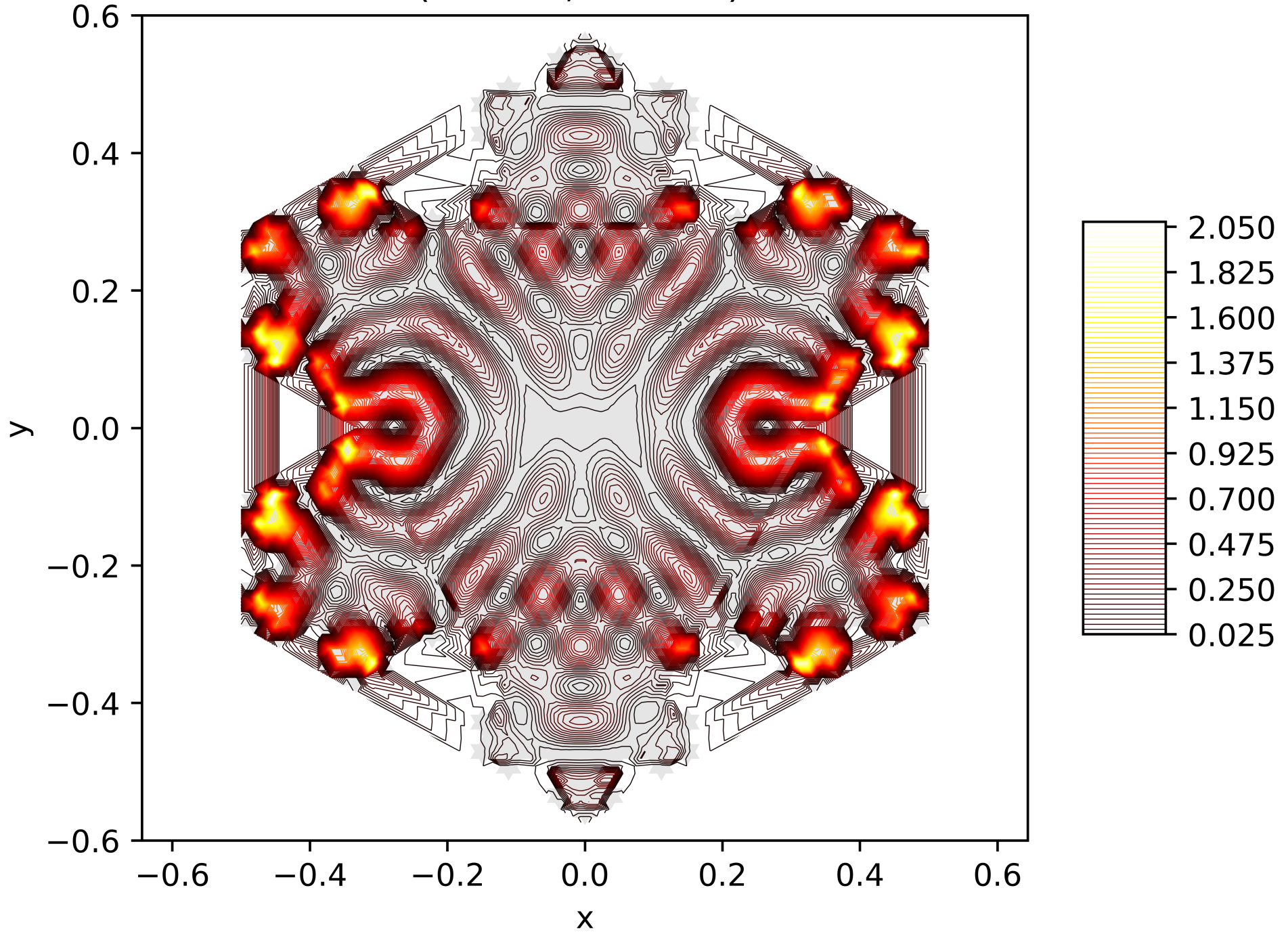
Contour Lines of the Energy Function of the 89. Eigenfunction on the Snowflake (Level 5, Res. 81) with Neumann BC
