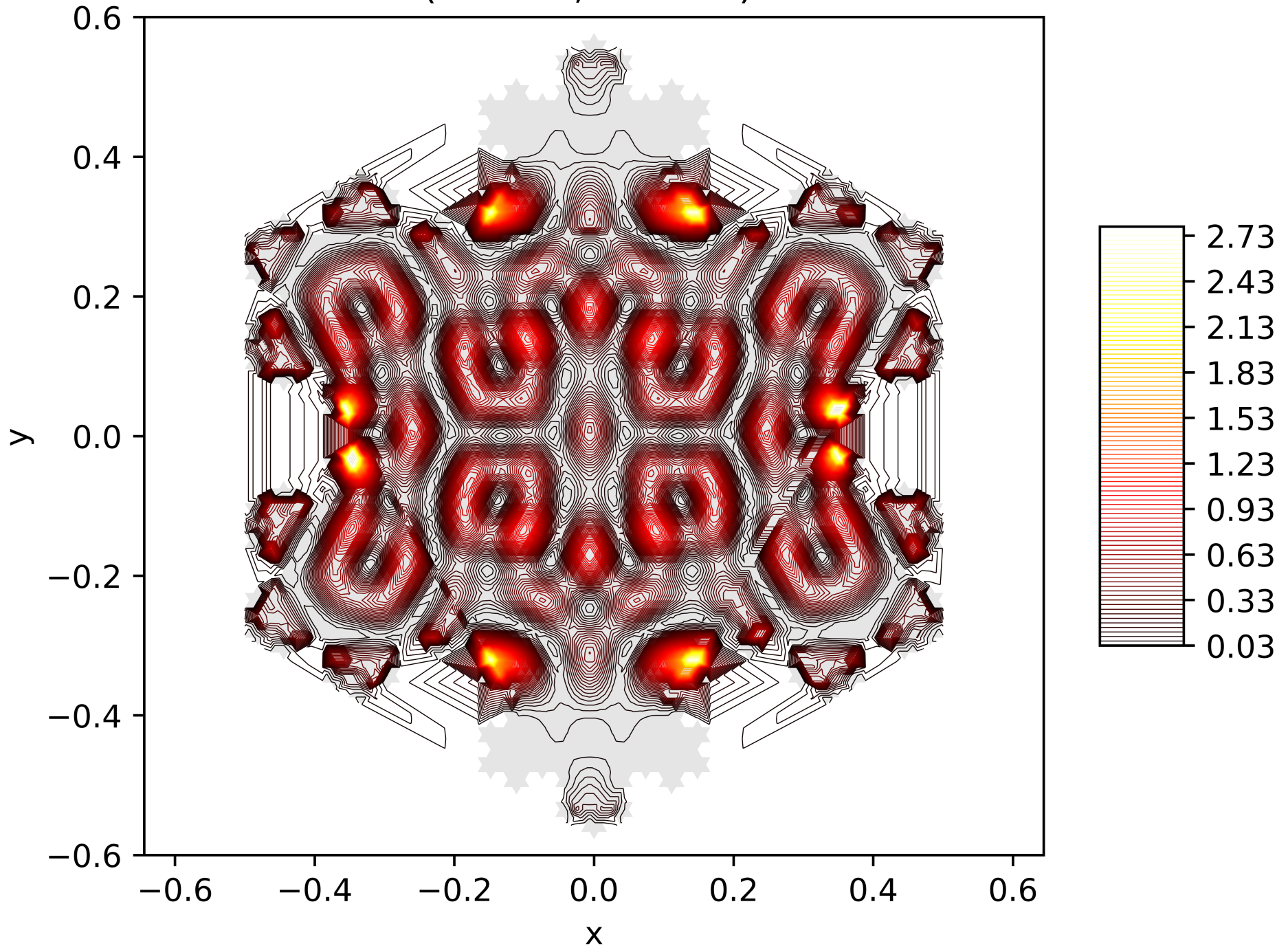
Contour Lines of the Energy Function of the 92. Eigenfunction on the Snowflake (Level 5, Res. 81) with Neumann BC
