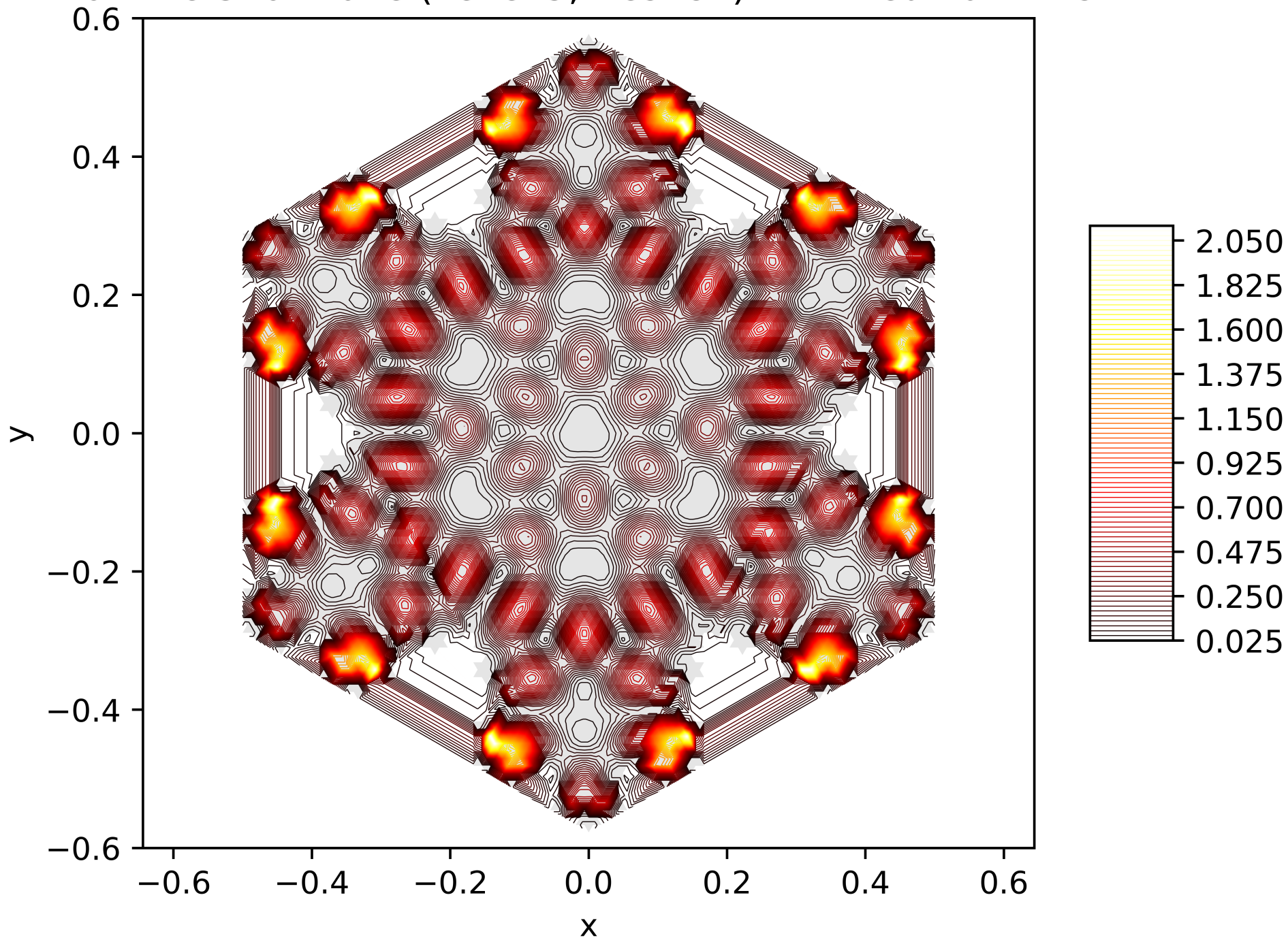
Contour Lines of the Energy Function of the 90. Eigenfunction on the Snowflake (Level 5, Res. 81) with Neumann BC
