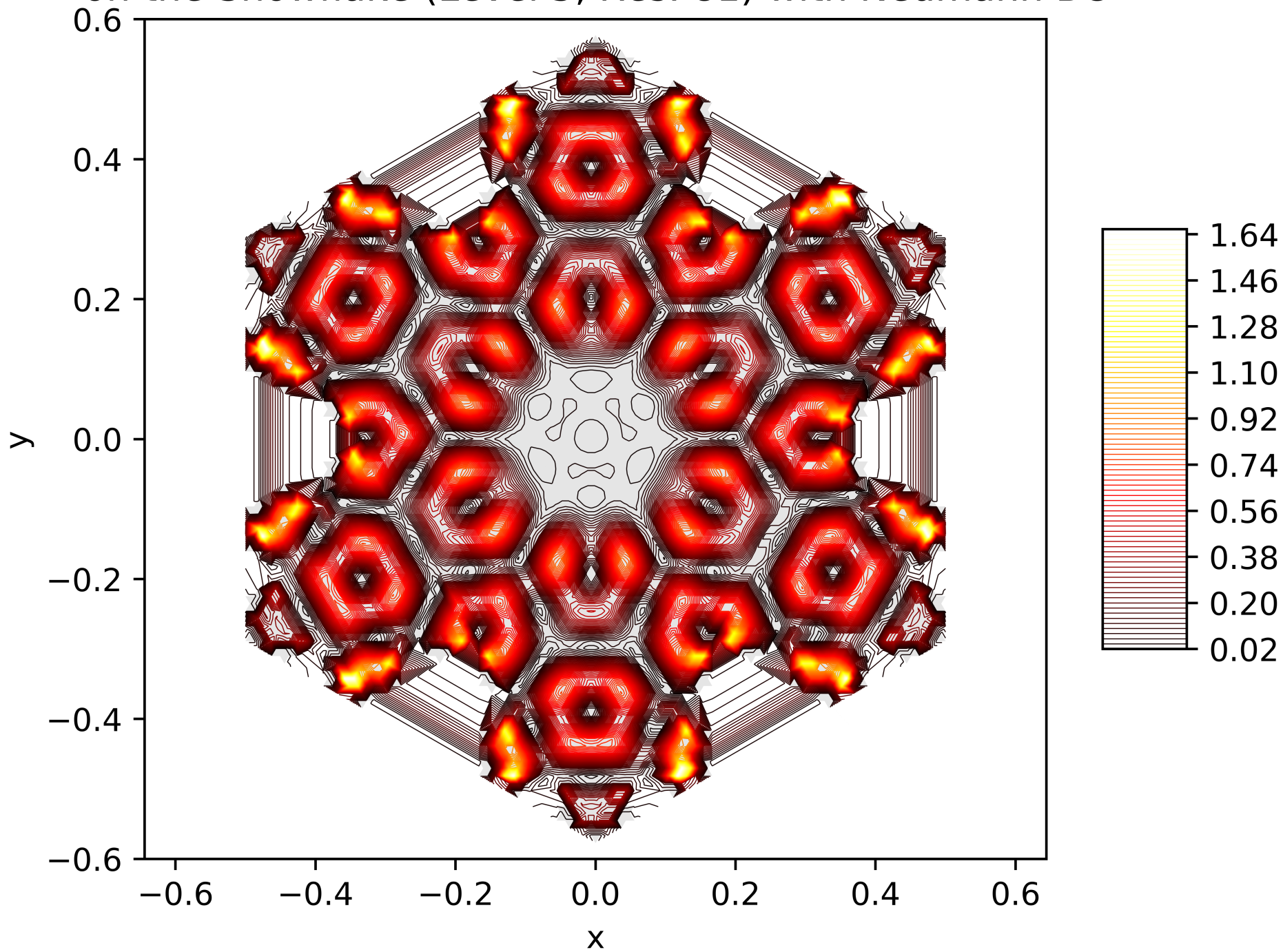
Contour Lines of the Energy Function of the 97. Eigenfunction on the Snowflake (Level 5, Res. 81) with Neumann BC
