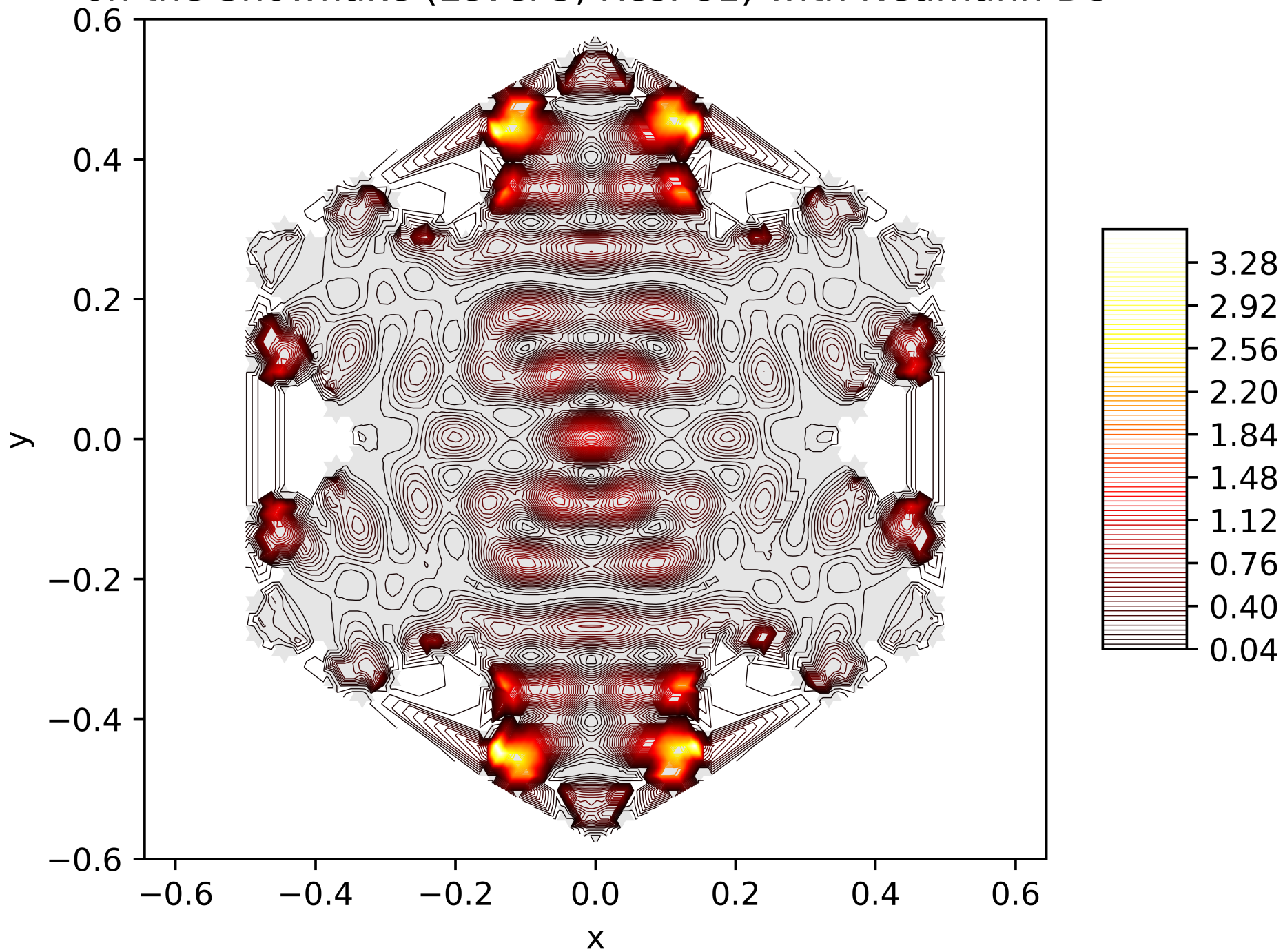
Contour Lines of the Energy Function of the 85. Eigenfunction on the Snowflake (Level 5, Res. 81) with Neumann BC
