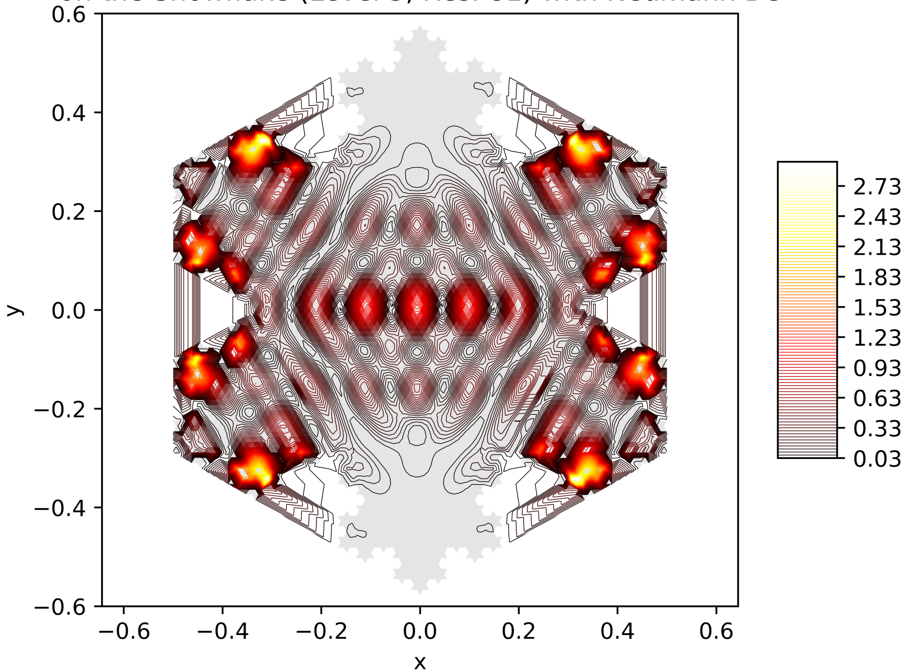
Contour Lines of the Energy Function of the 86. Eigenfunction on the Snowflake (Level 5, Res. 81) with Neumann BC
