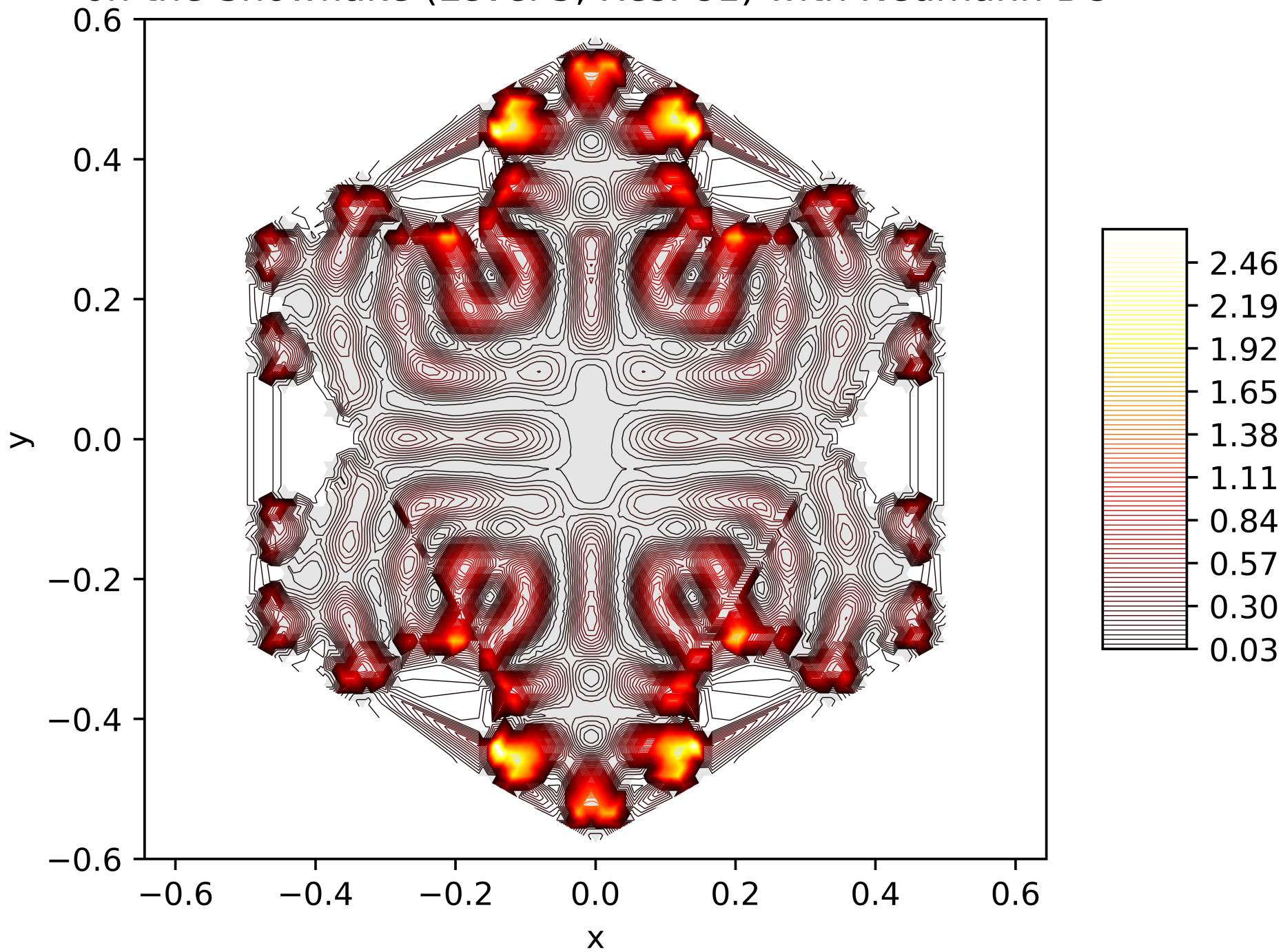
Contour Lines of the Energy Function of the 88. Eigenfunction on the Snowflake (Level 5, Res. 81) with Neumann BC
