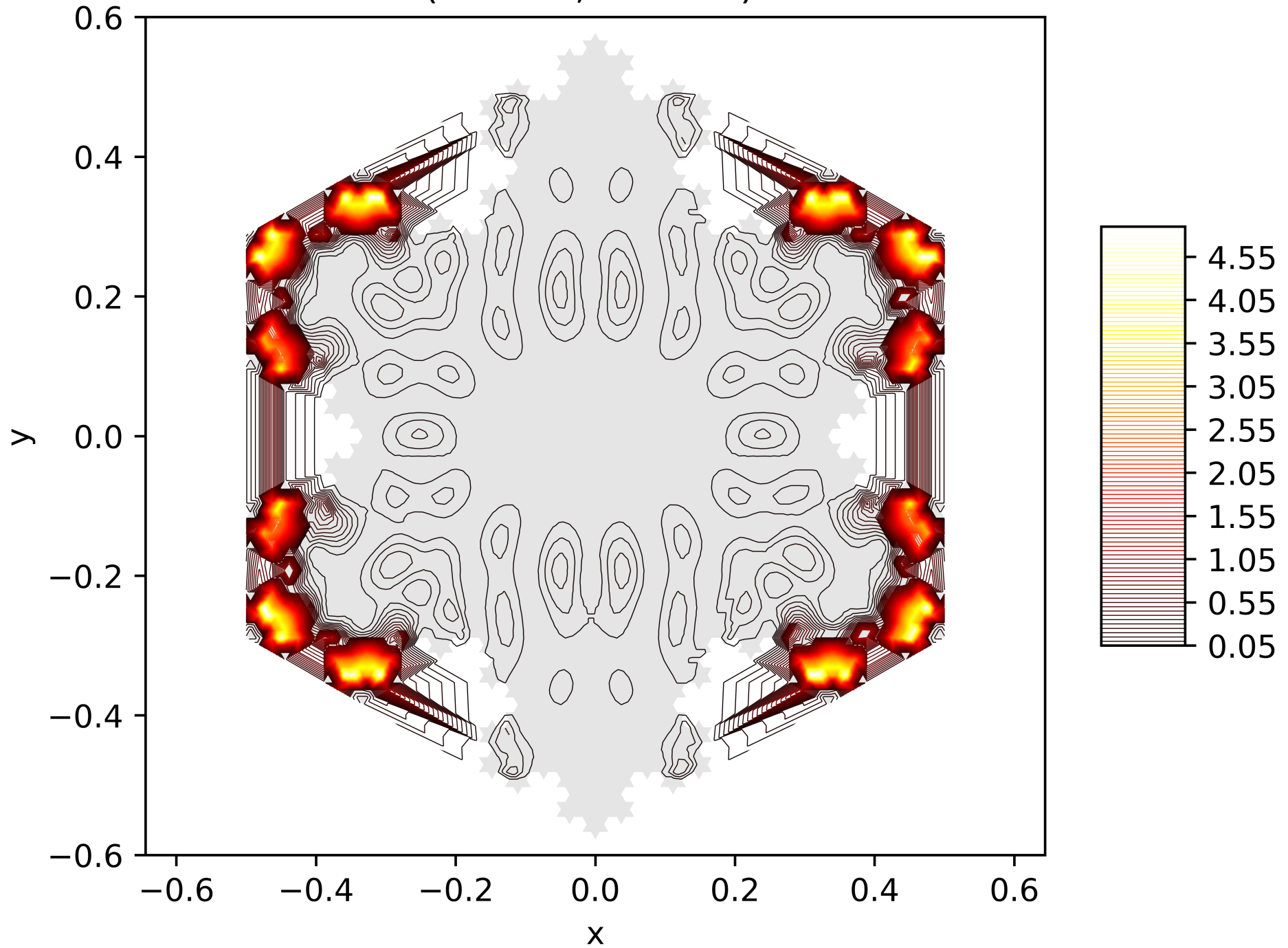
Contour Lines of the Energy Function of the 100. Eigenfunction on the Snowflake (Level 5, Res. 81) with Neumann BC
