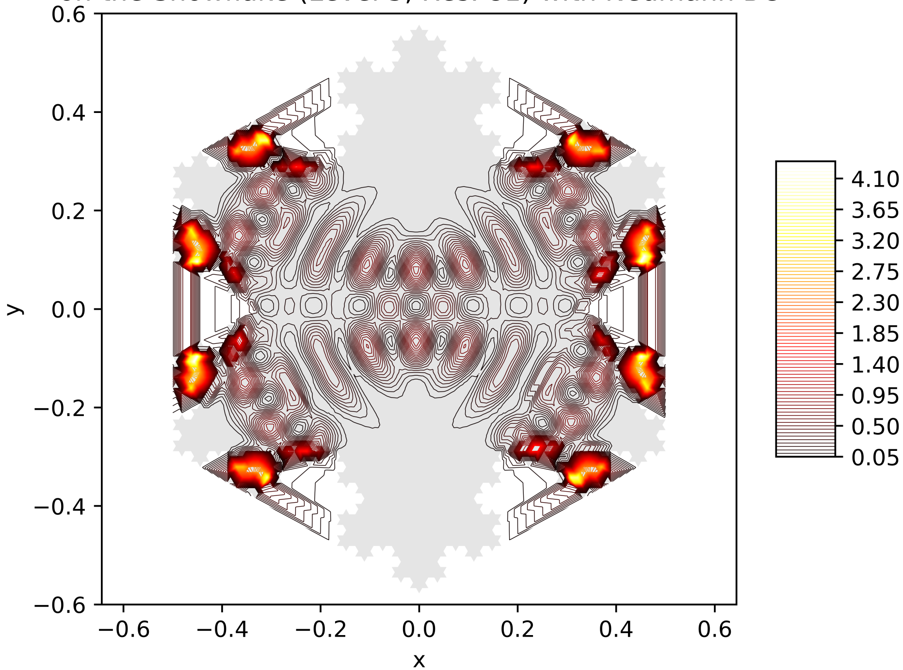
Contour Lines of the Energy Function of the 94. Eigenfunction on the Snowflake (Level 5, Res. 81) with Neumann BC
