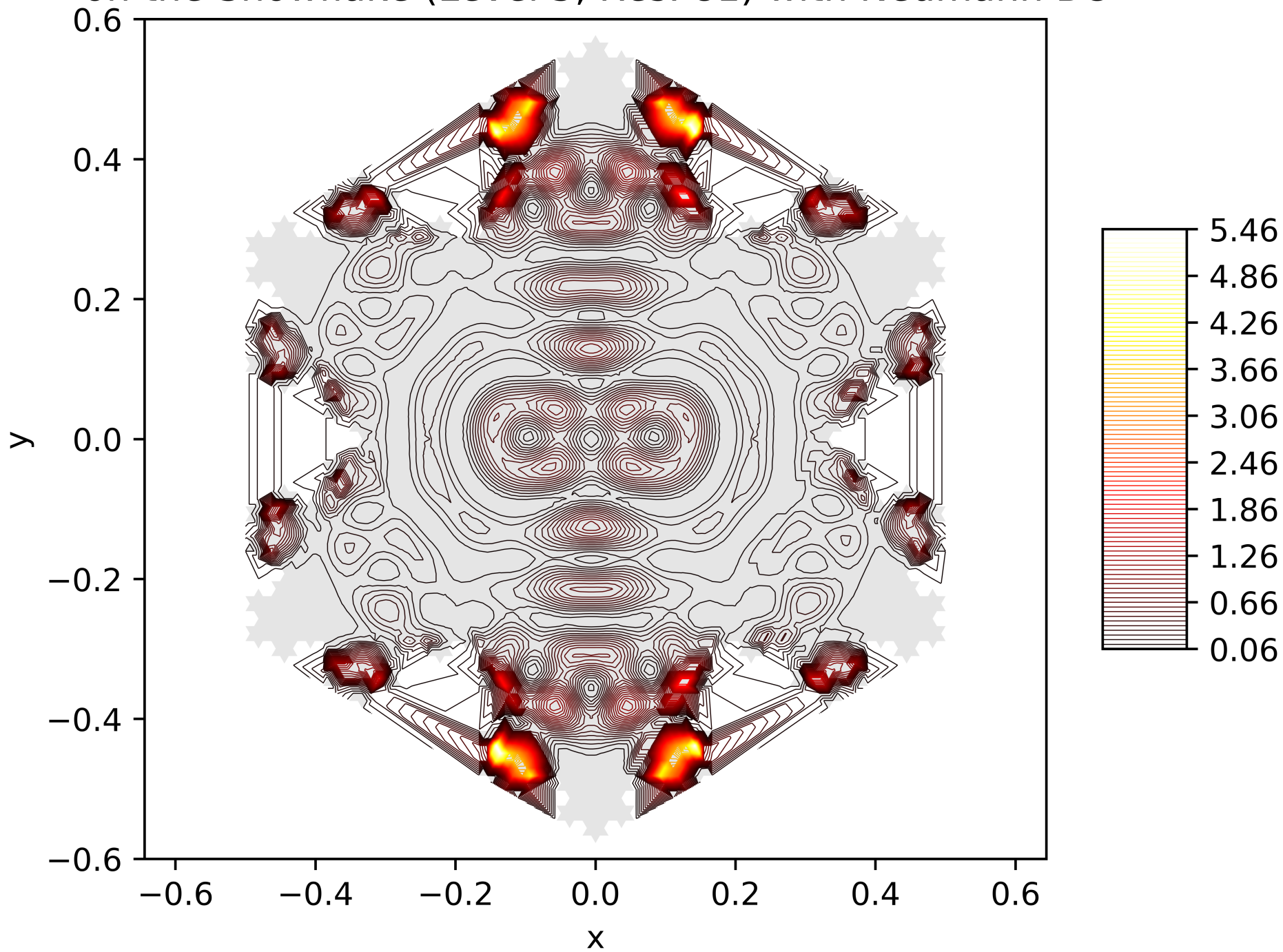
Contour Lines of the Energy Function of the 93. Eigenfunction on the Snowflake (Level 5, Res. 81) with Neumann BC
