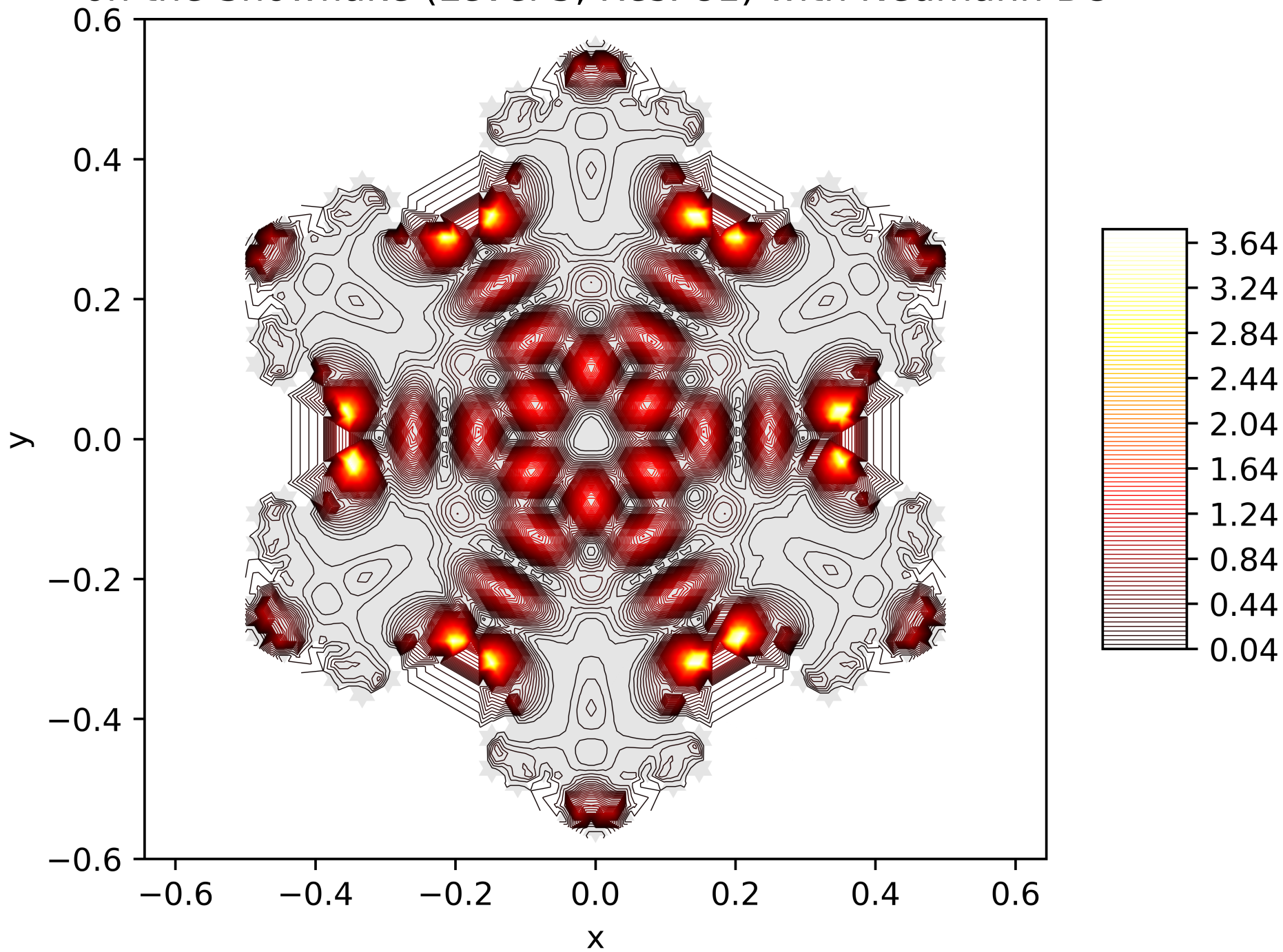
Contour Lines of the Energy Function of the 98. Eigenfunction on the Snowflake (Level 5, Res. 81) with Neumann BC
