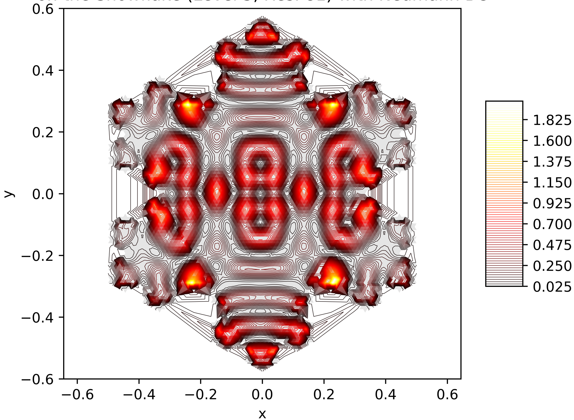
Contour Lines of the Energy Function of the 81. Eigenfunction on the Snowflake (Level 5, Res. 81) with Neumann BC
