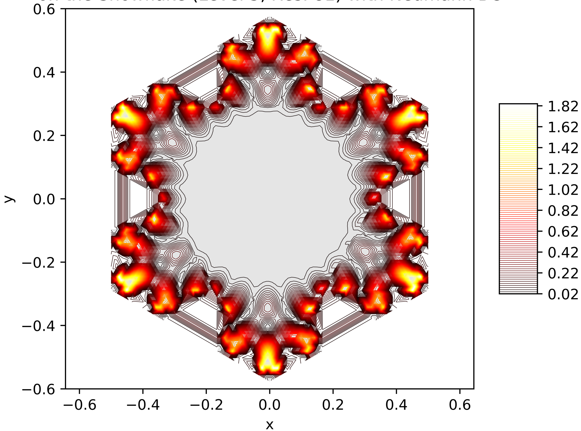
Contour Lines of the Energy Function of the 84. Eigenfunction on the Snowflake (Level 5, Res. 81) with Neumann BC
