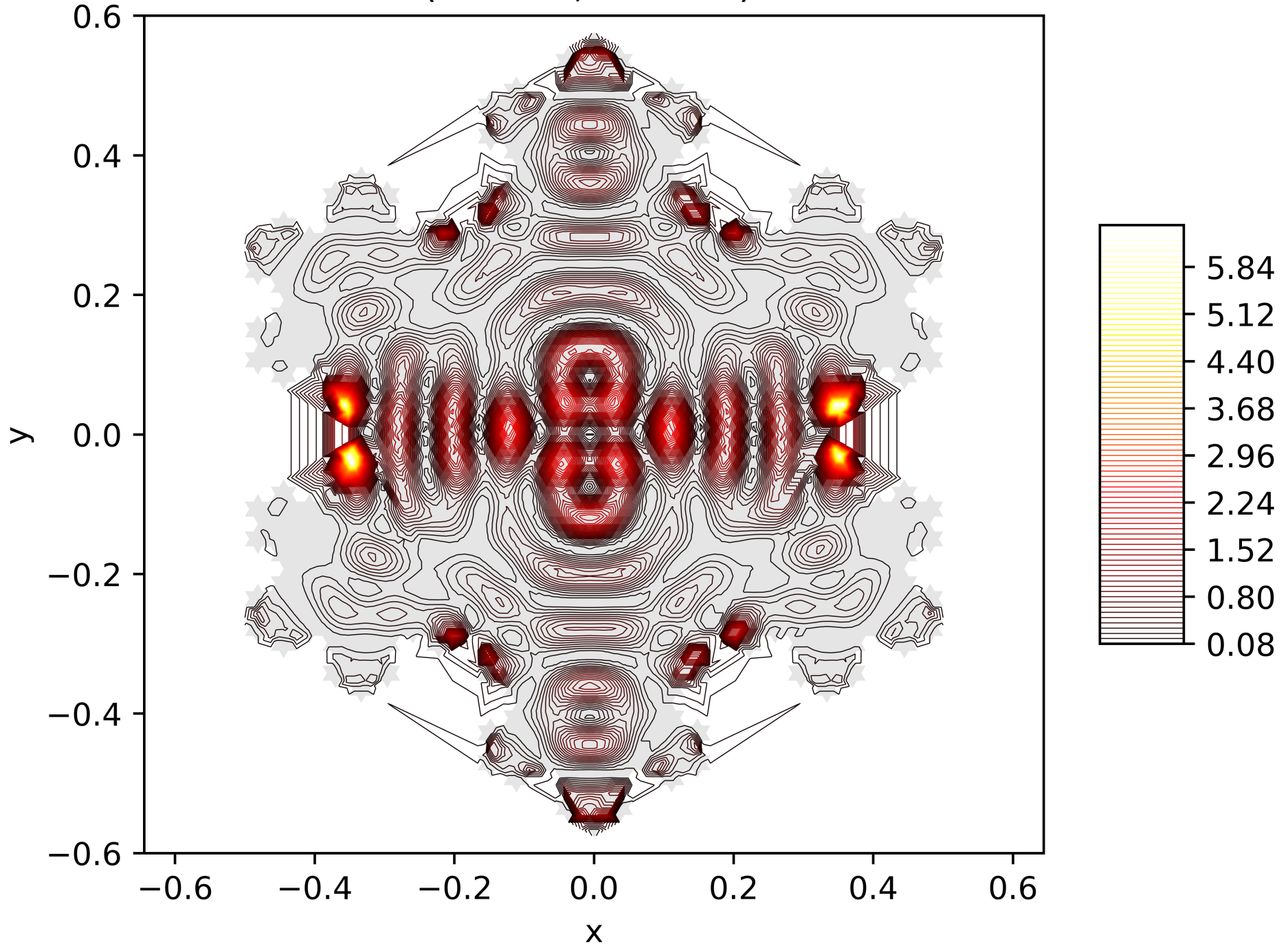
Contour Lines of the Energy Function of the 122. Eigenfunction on the Snowflake (Level 5, Res. 81) with Neumann BC
