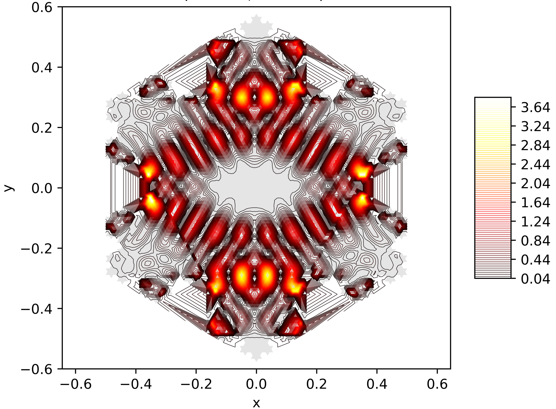
Contour Lines of the Energy Function of the 130. Eigenfunction on the Snowflake (Level 5, Res. 81) with Neumann BC
