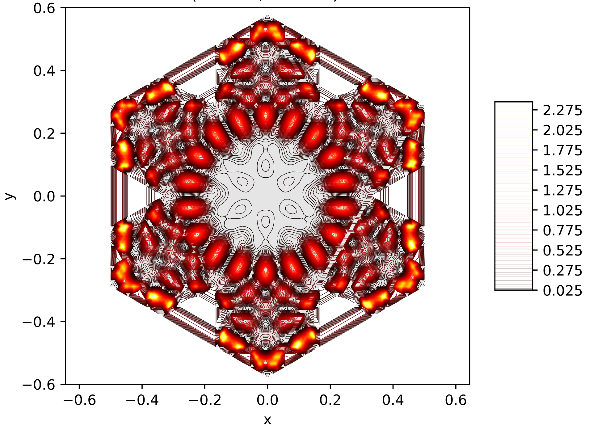
Contour Lines of the Energy Function of the 126. Eigenfunction on the Snowflake (Level 5, Res. 81) with Neumann BC
