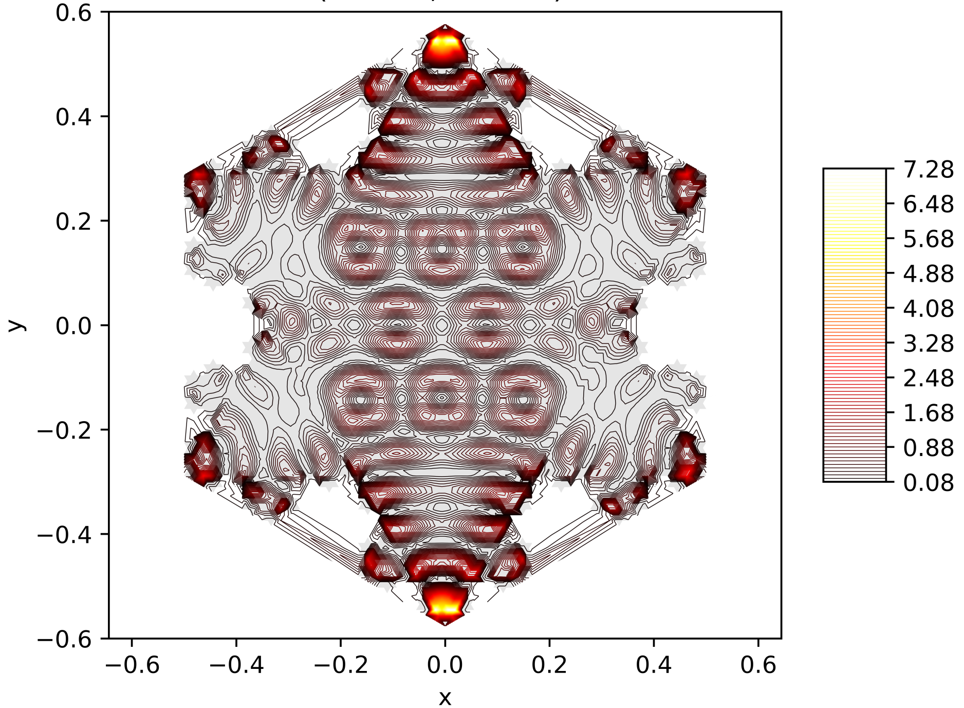
Contour Lines of the Energy Function of the 136. Eigenfunction on the Snowflake (Level 5, Res. 81) with Neumann BC
