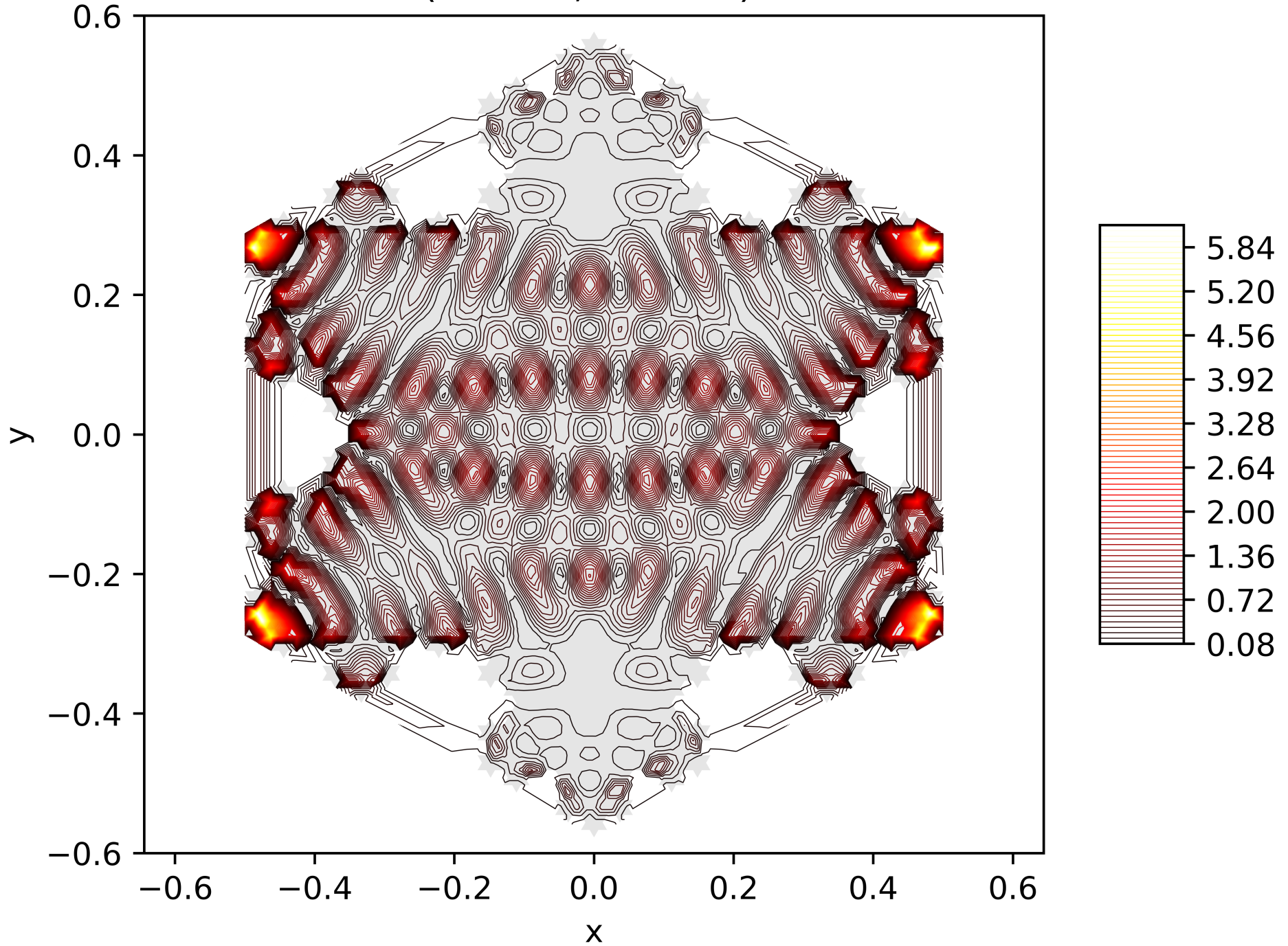
Contour Lines of the Energy Function of the 137. Eigenfunction on the Snowflake (Level 5, Res. 81) with Neumann BC
