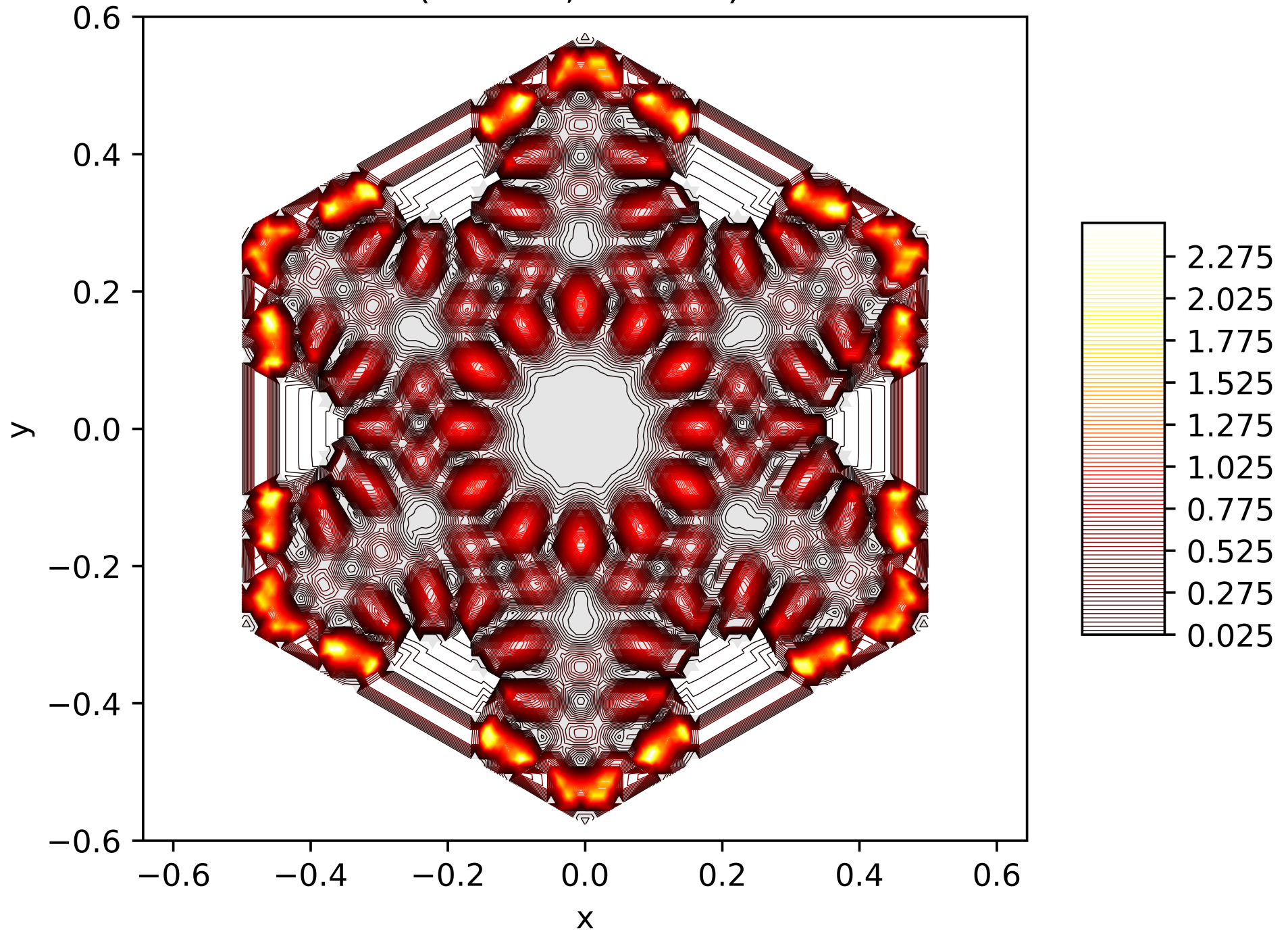
Contour Lines of the Energy Function of the 121. Eigenfunction on the Snowflake (Level 5, Res. 81) with Neumann BC
