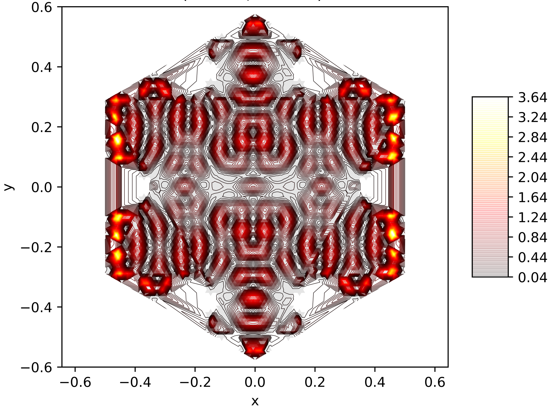
Contour Lines of the Energy Function of the 135. Eigenfunction on the Snowflake (Level 5, Res. 81) with Neumann BC
