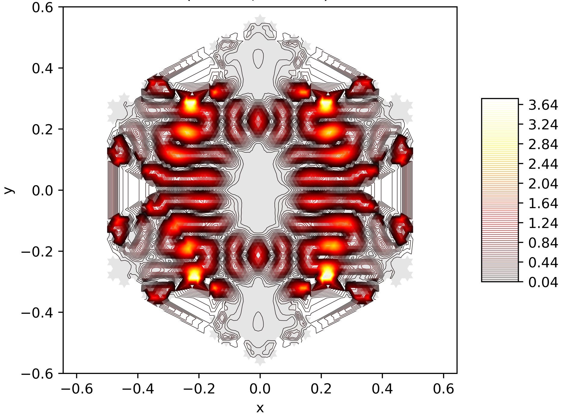
Contour Lines of the Energy Function of the 131. Eigenfunction on the Snowflake (Level 5, Res. 81) with Neumann BC
