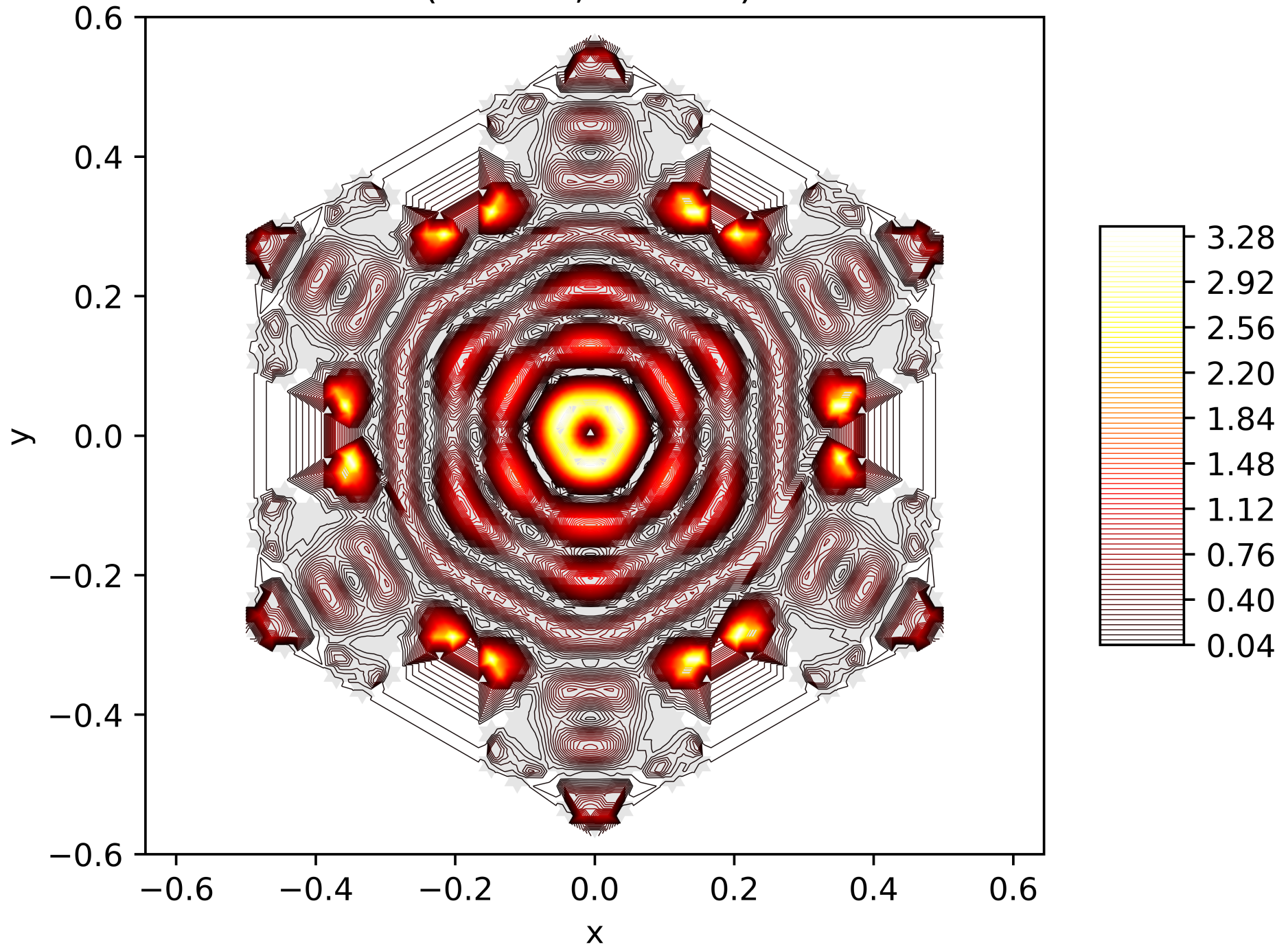
Contour Lines of the Energy Function of the 127. Eigenfunction on the Snowflake (Level 5, Res. 81) with Neumann BC
