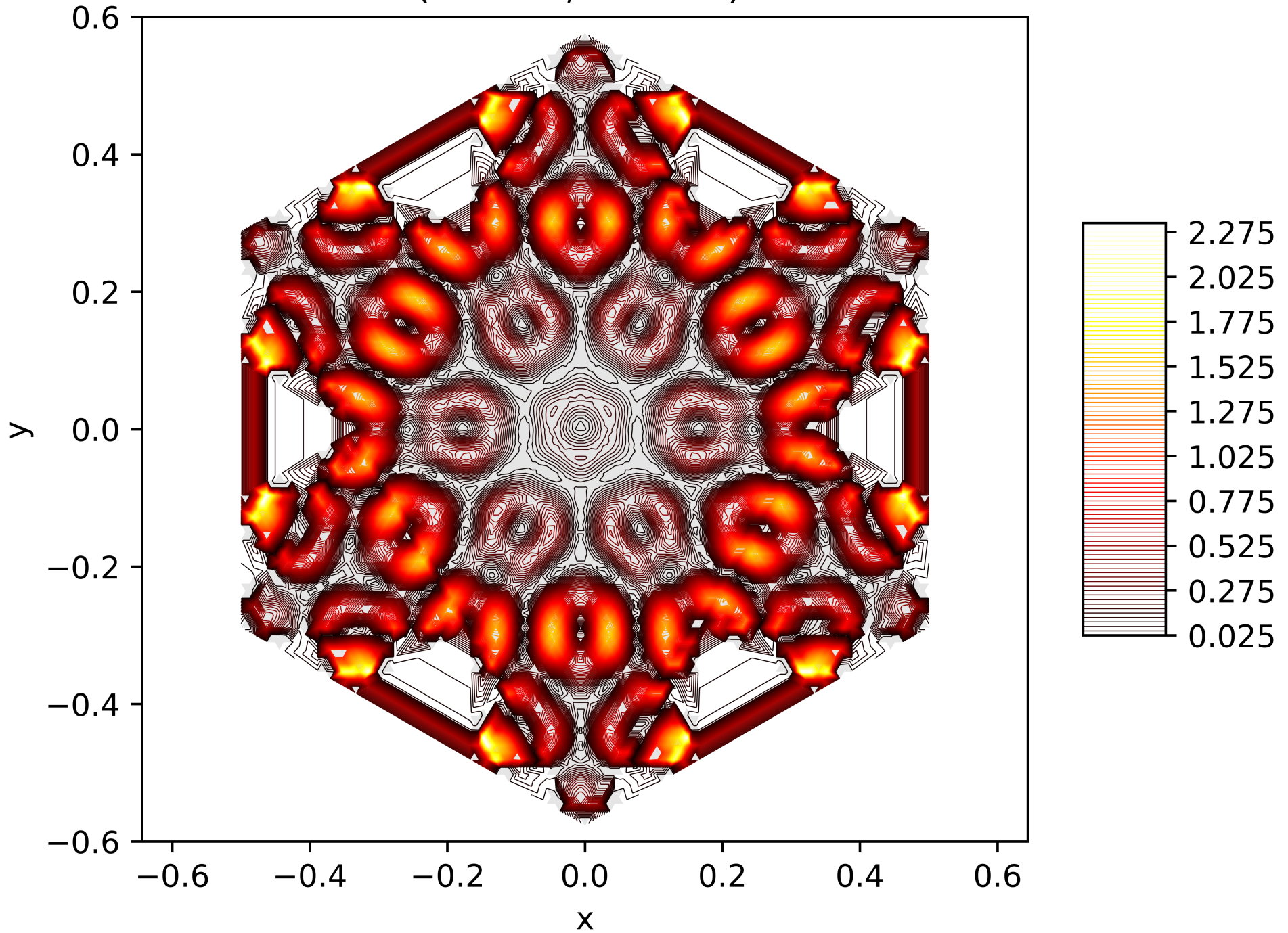
Contour Lines of the Energy Function of the 132. Eigenfunction on the Snowflake (Level 5, Res. 81) with Neumann BC
