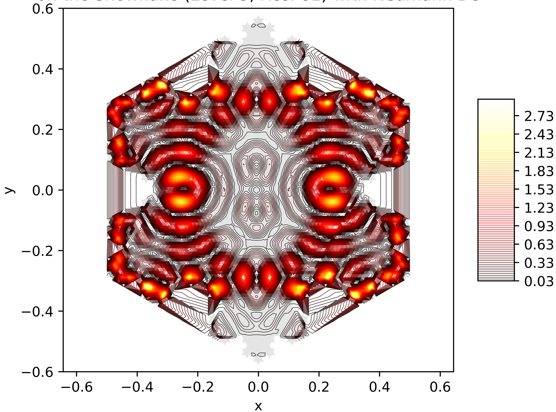
Contour Lines of the Energy Function of the 129. Eigenfunction on the Snowflake (Level 5, Res. 81) with Neumann BC
