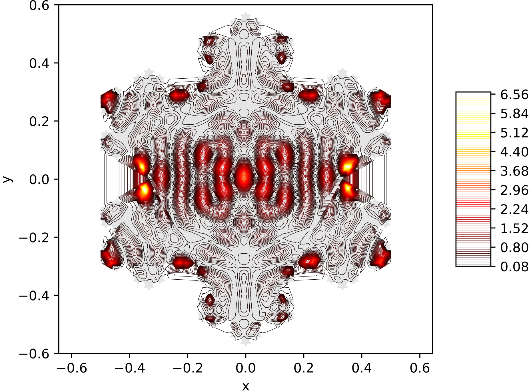
Contour Lines of the Energy Function of the 140. Eigenfunction on the Snowflake (Level 5, Res. 81) with Neumann BC
