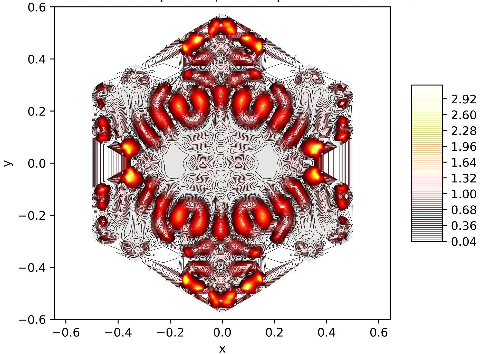
Contour Lines of the Energy Function of the 128. Eigenfunction on the Snowflake (Level 5, Res. 81) with Neumann BC
