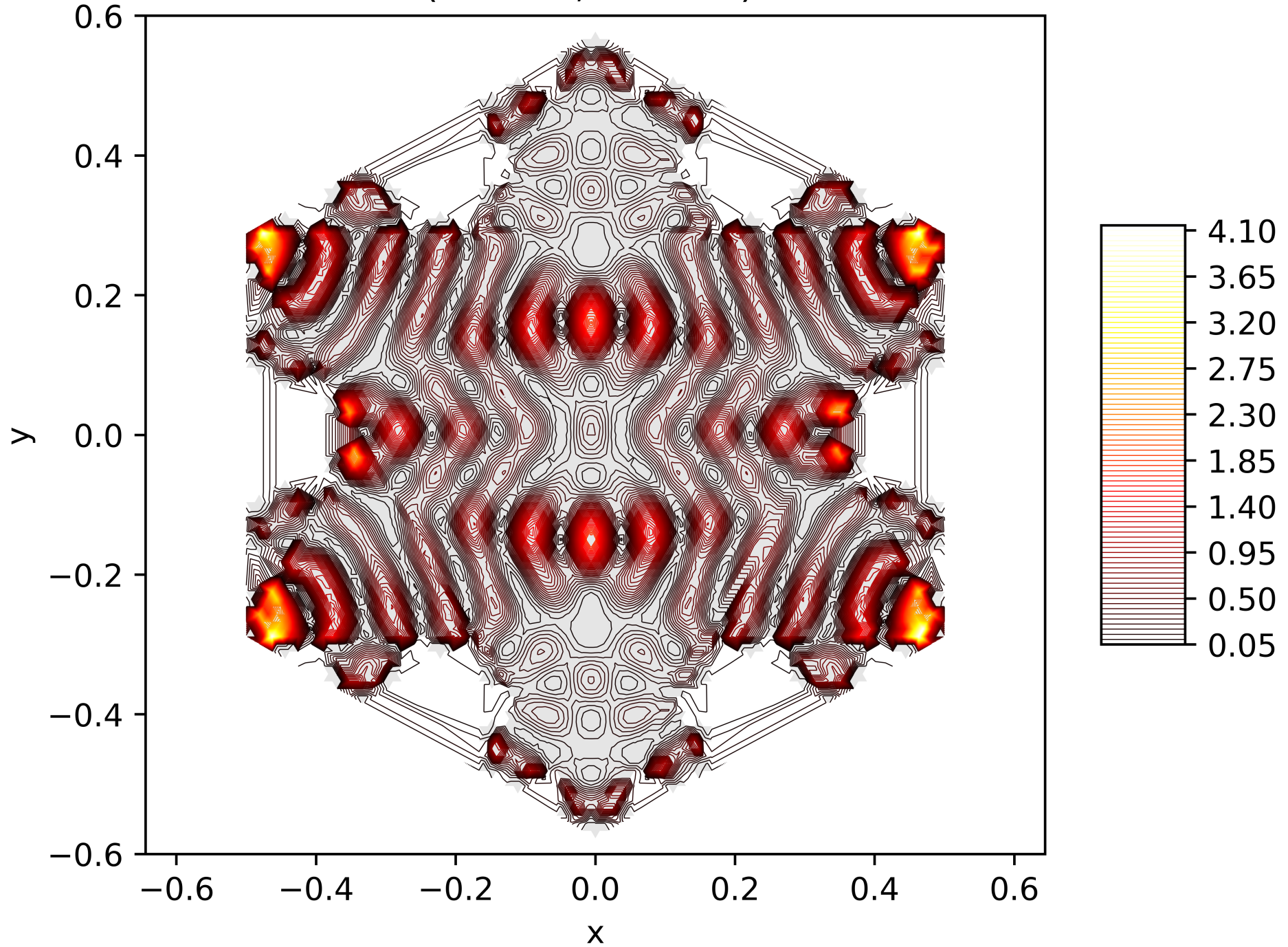
Contour Lines of the Energy Function of the 125. Eigenfunction on the Snowflake (Level 5, Res. 81) with Neumann BC
