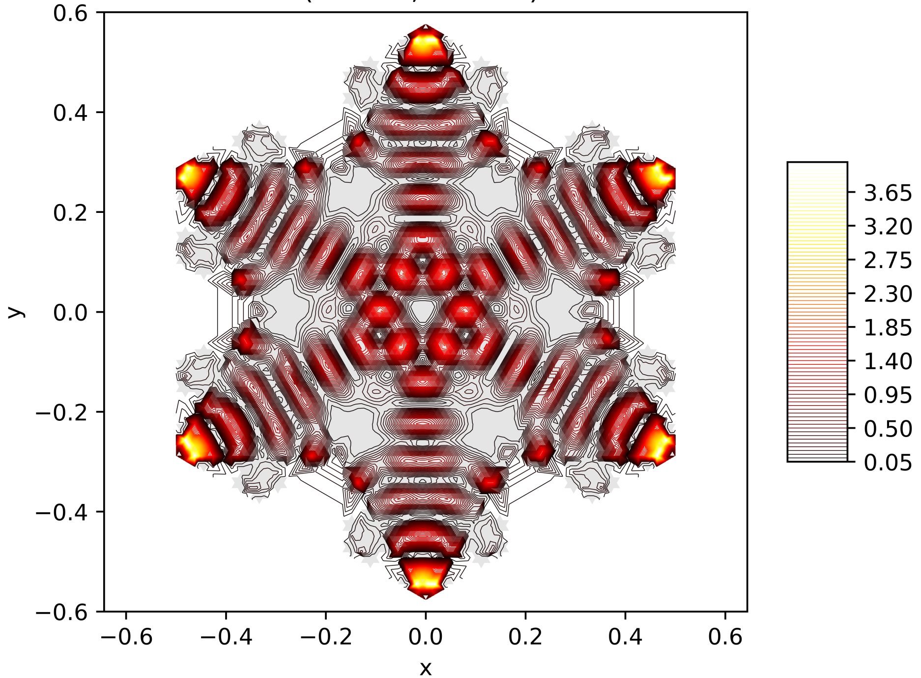
Contour Lines of the Energy Function of the 133. Eigenfunction on the Snowflake (Level 5, Res. 81) with Neumann BC
