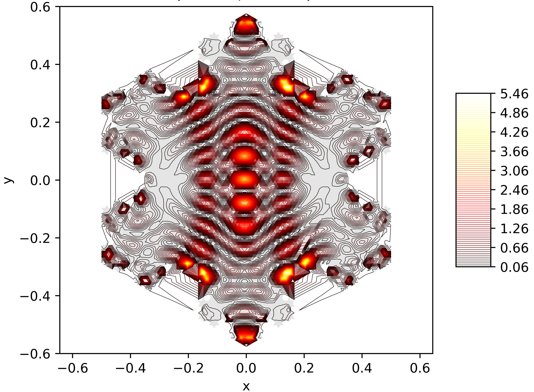
Contour Lines of the Energy Function of the 139. Eigenfunction on the Snowflake (Level 5, Res. 81) with Neumann BC
