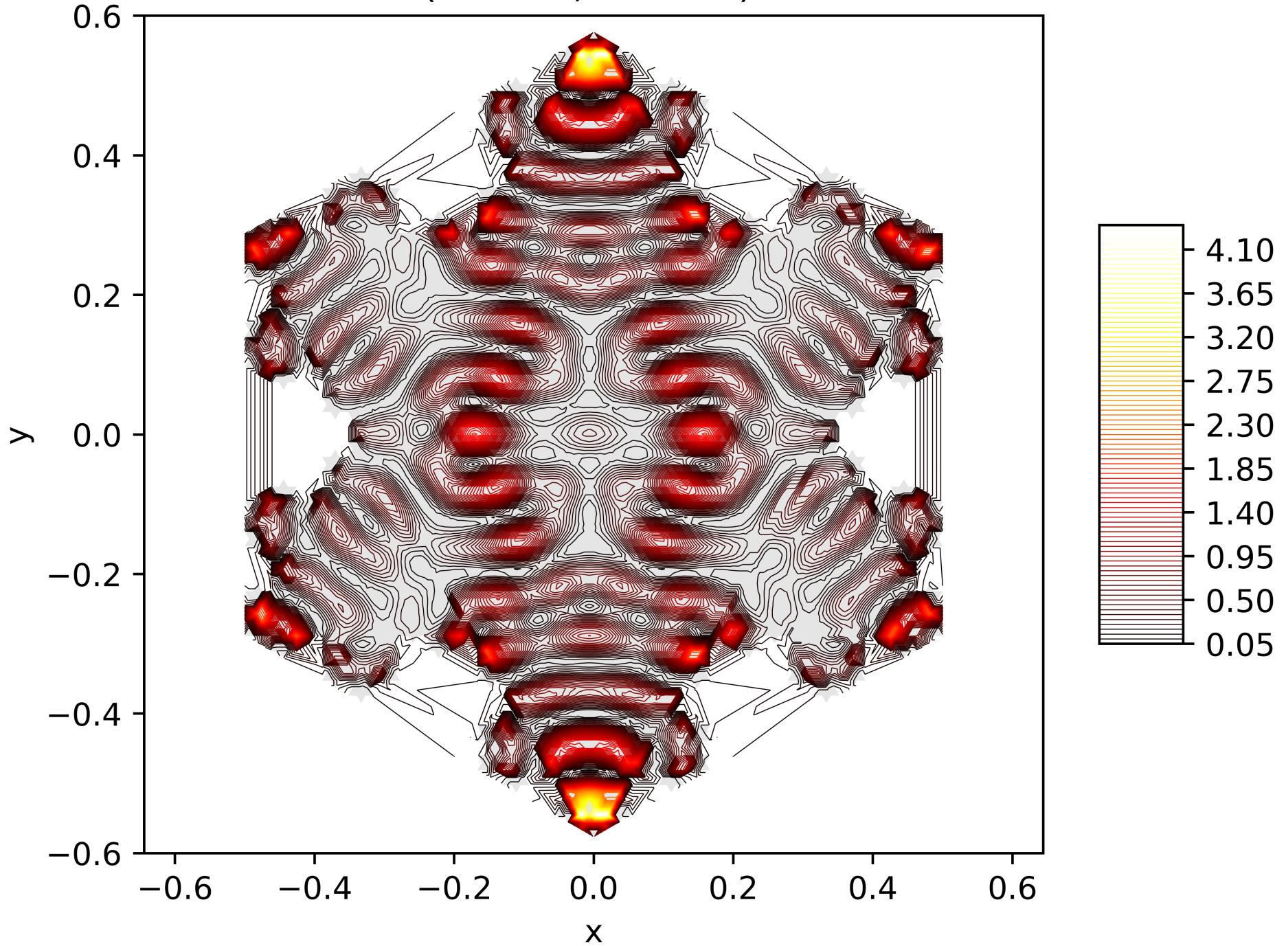
Contour Lines of the Energy Function of the 124. Eigenfunction on the Snowflake (Level 5, Res. 81) with Neumann BC
