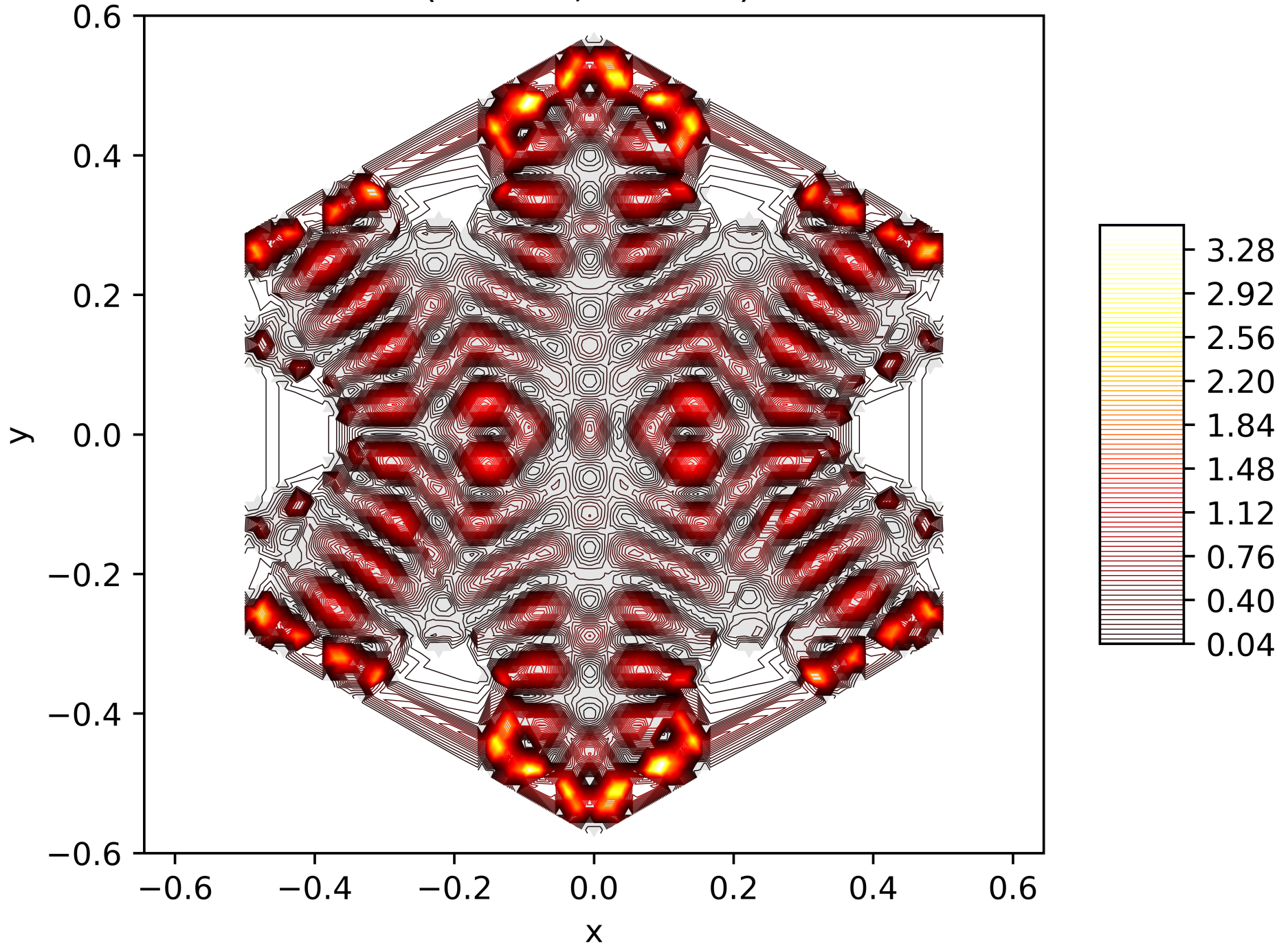
Contour Lines of the Energy Function of the 134. Eigenfunction on the Snowflake (Level 5, Res. 81) with Neumann BC
