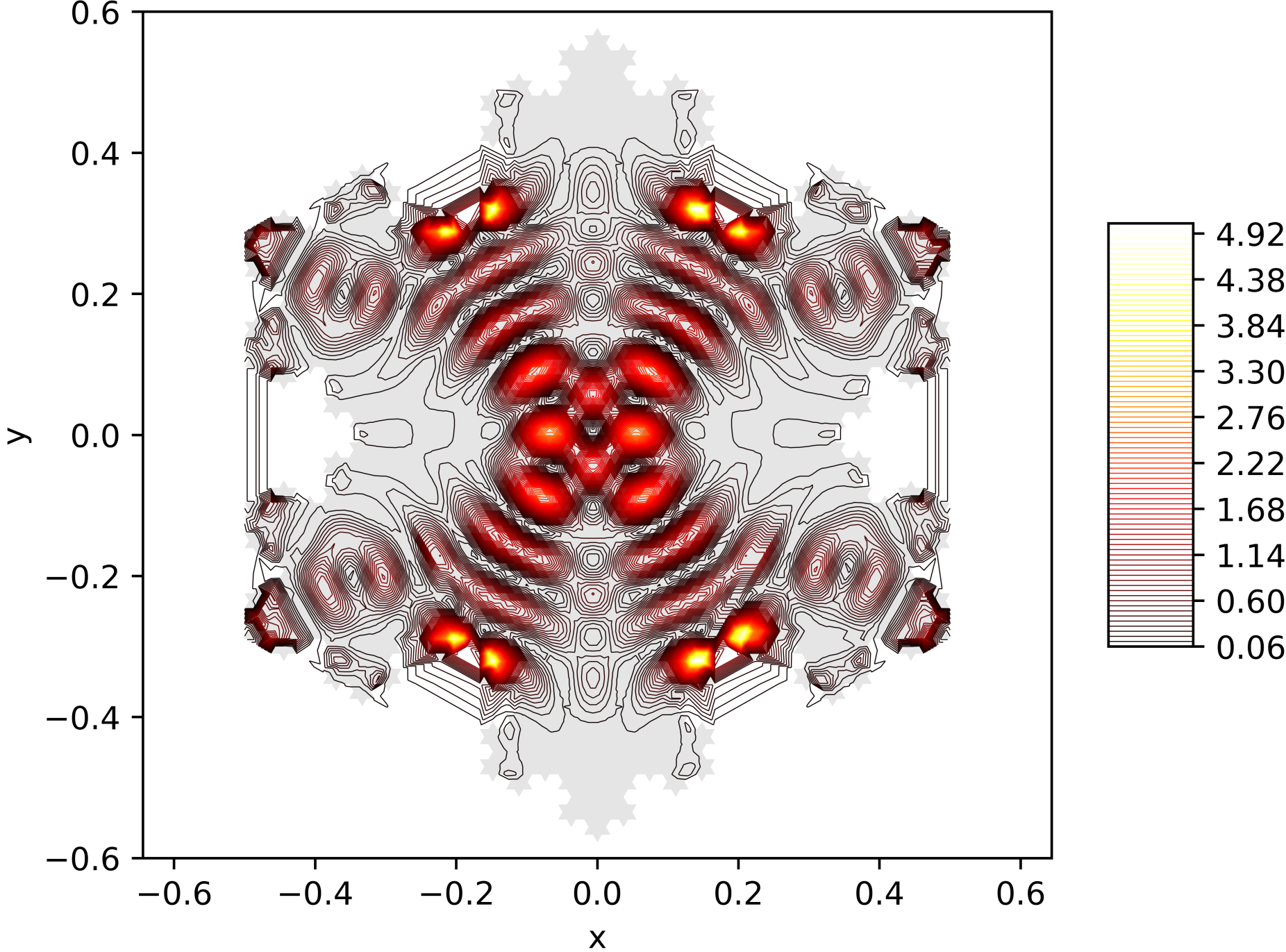
Contour Lines of the Energy Function of the 123. Eigenfunction on the Snowflake (Level 5, Res. 81) with Neumann BC
