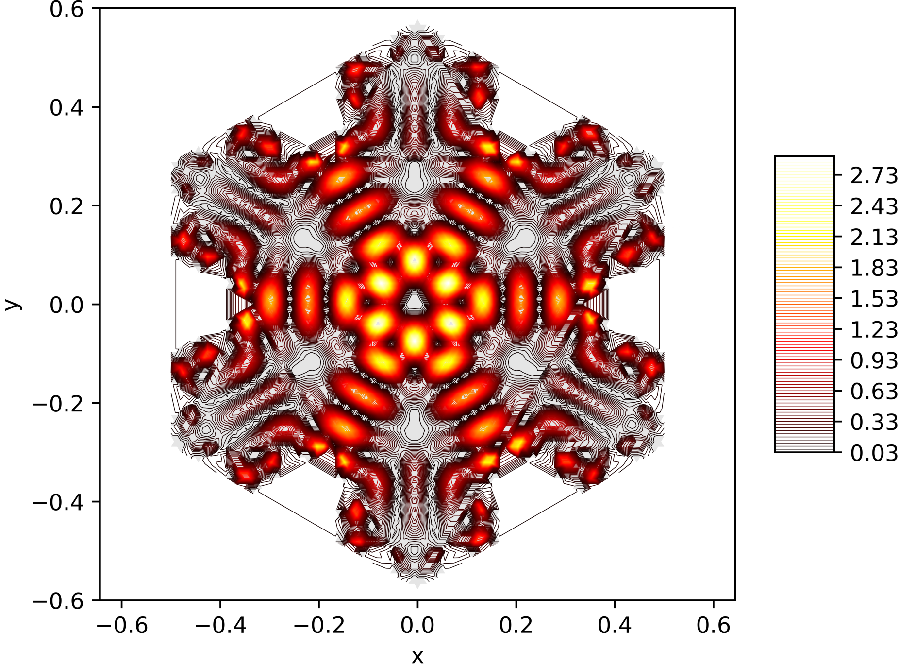
Contour Lines of the Energy Function of the 138. Eigenfunction on the Snowflake (Level 5, Res. 81) with Neumann BC
