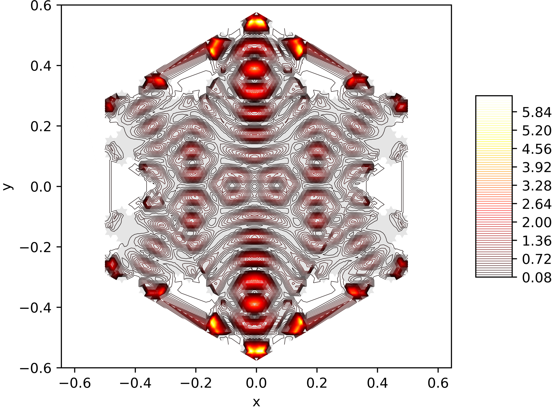
Contour Lines of the Energy Function of the 153. Eigenfunction on the Snowflake (Level 5, Res. 81) with Neumann BC
