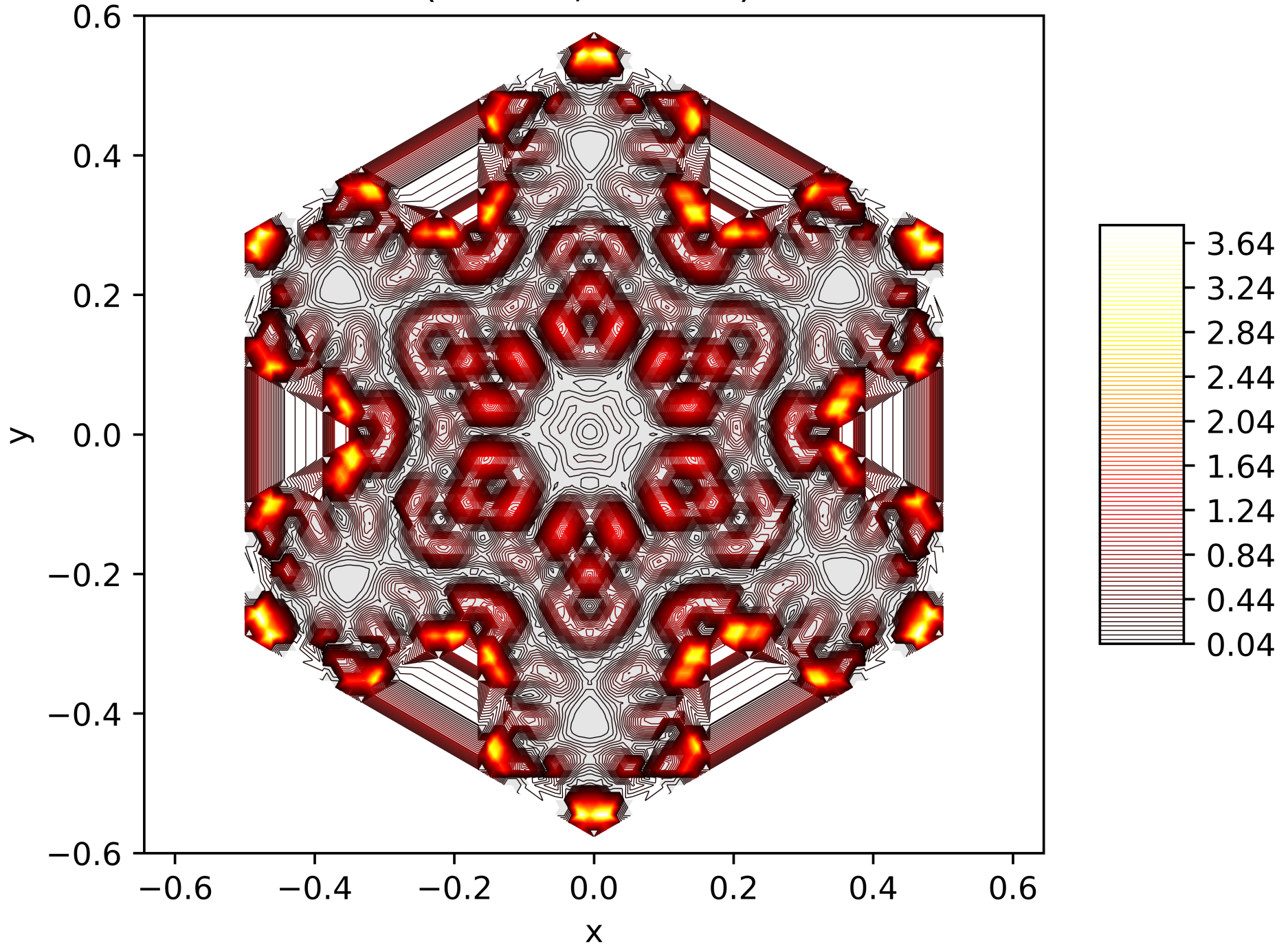
Contour Lines of the Energy Function of the 158. Eigenfunction on the Snowflake (Level 5, Res. 81) with Neumann BC
