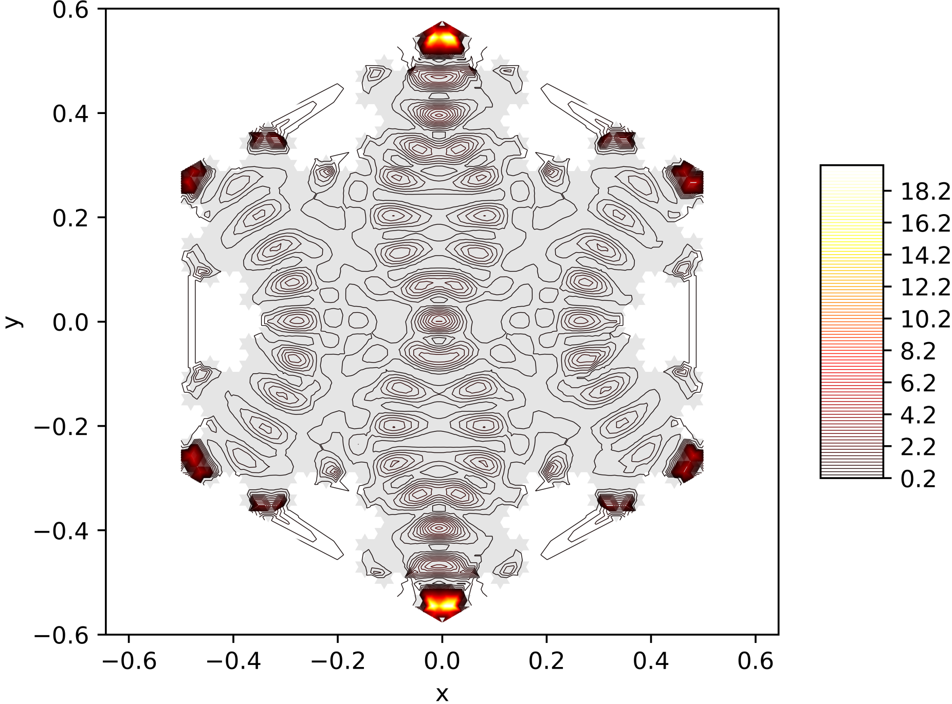
Contour Lines of the Energy Function of the 160. Eigenfunction on the Snowflake (Level 5, Res. 81) with Neumann BC
