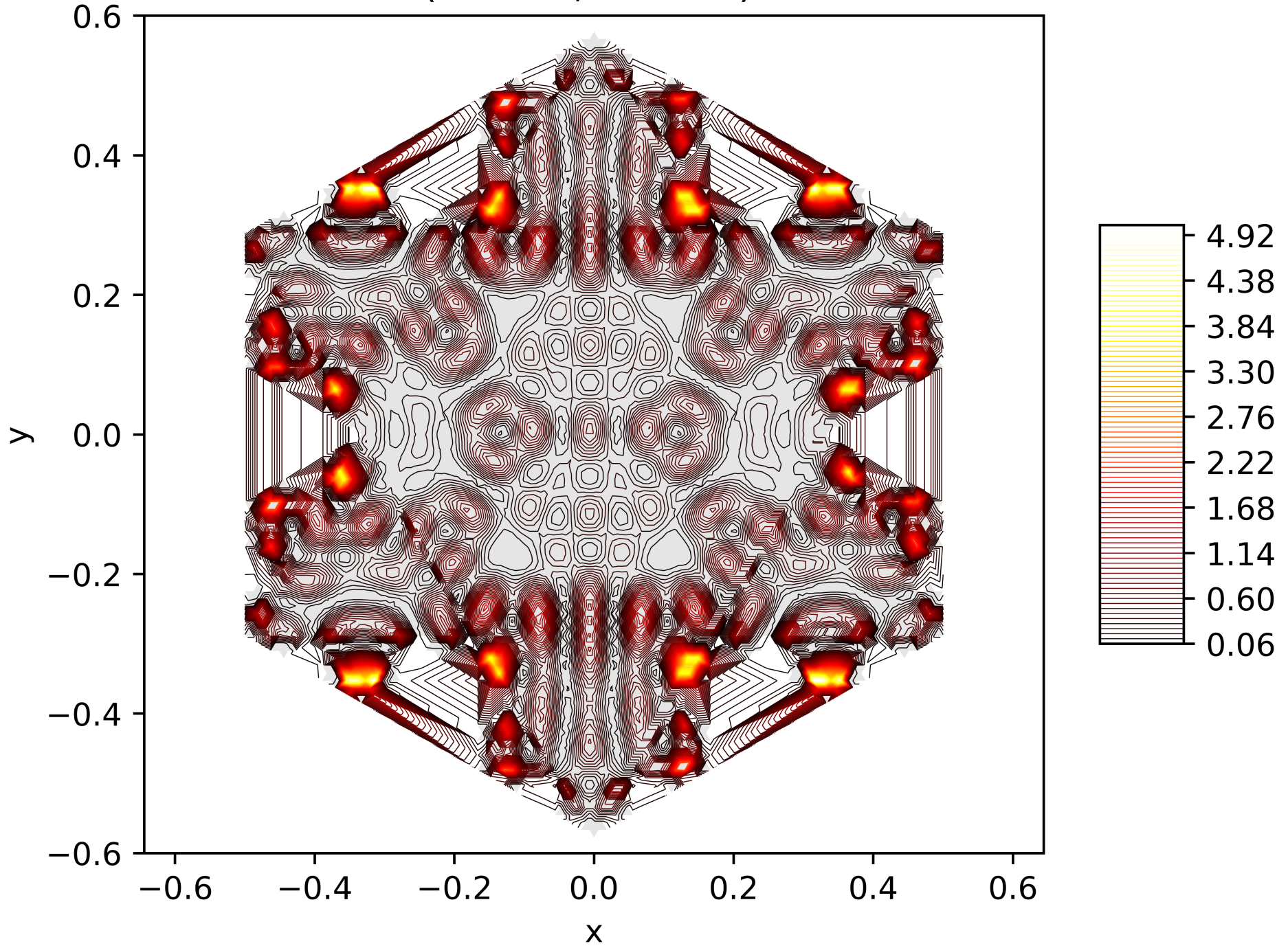
Contour Lines of the Energy Function of the 146. Eigenfunction on the Snowflake (Level 5, Res. 81) with Neumann BC
