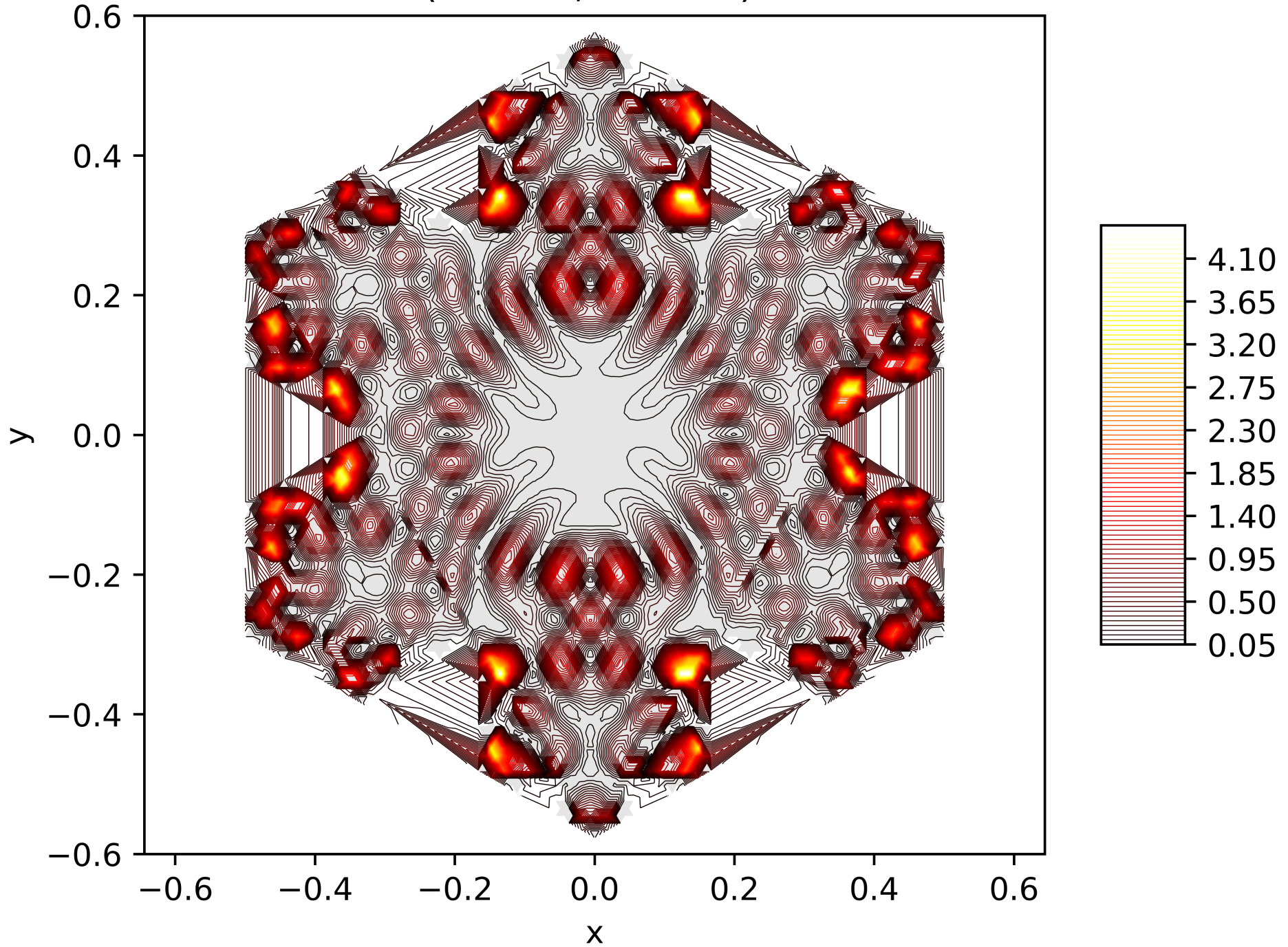
Contour Lines of the Energy Function of the 142. Eigenfunction on the Snowflake (Level 5, Res. 81) with Neumann BC
