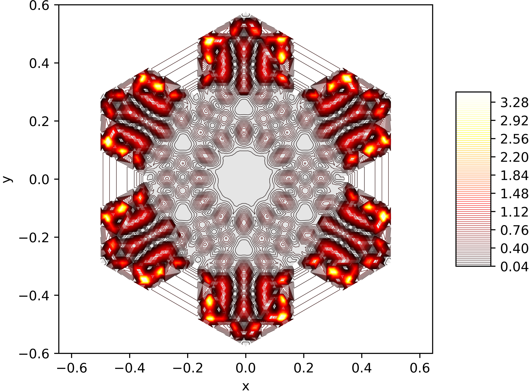
Contour Lines of the Energy Function of the 145. Eigenfunction on the Snowflake (Level 5, Res. 81) with Neumann BC
