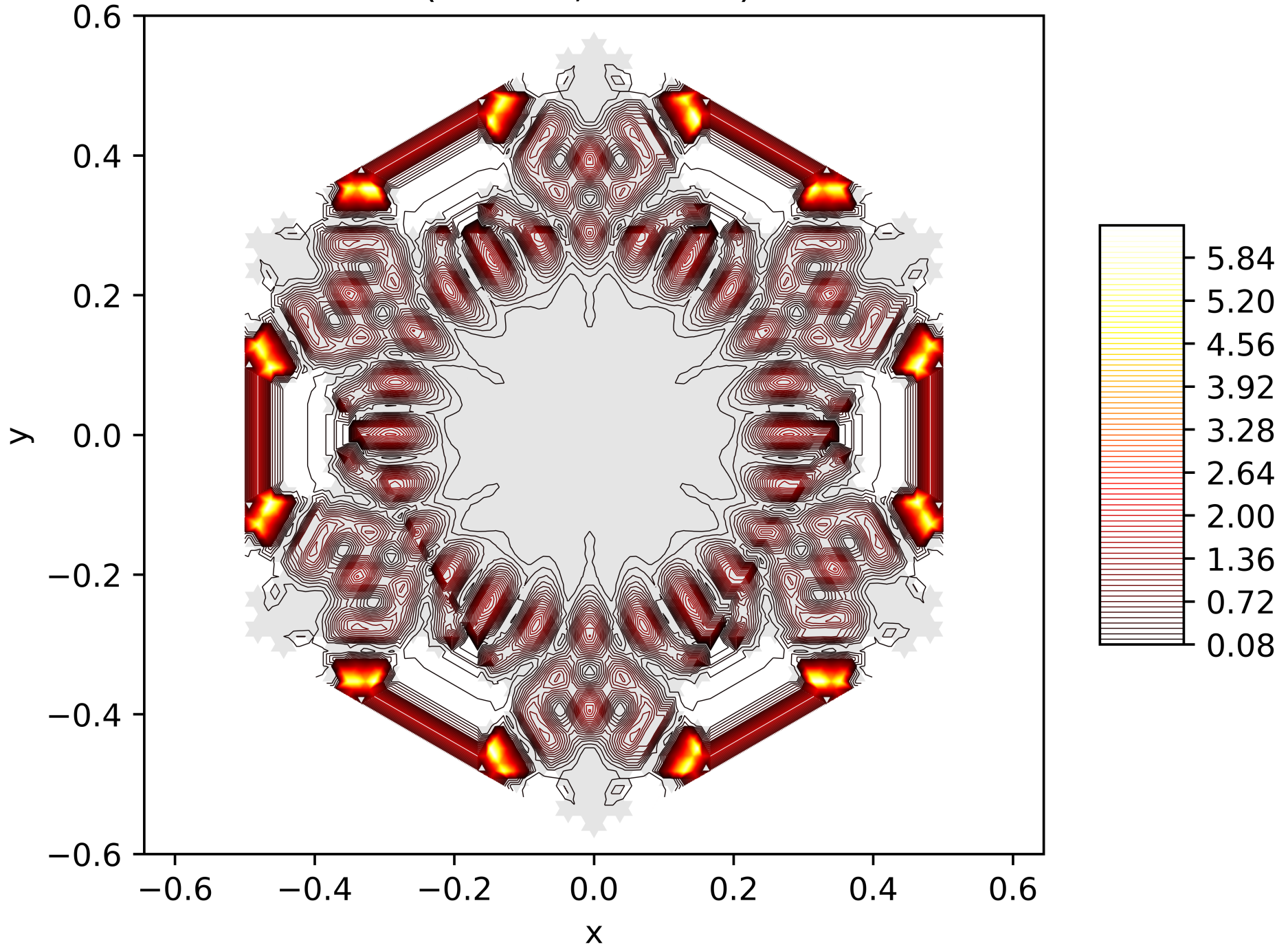
Contour Lines of the Energy Function of the 157. Eigenfunction on the Snowflake (Level 5, Res. 81) with Neumann BC
