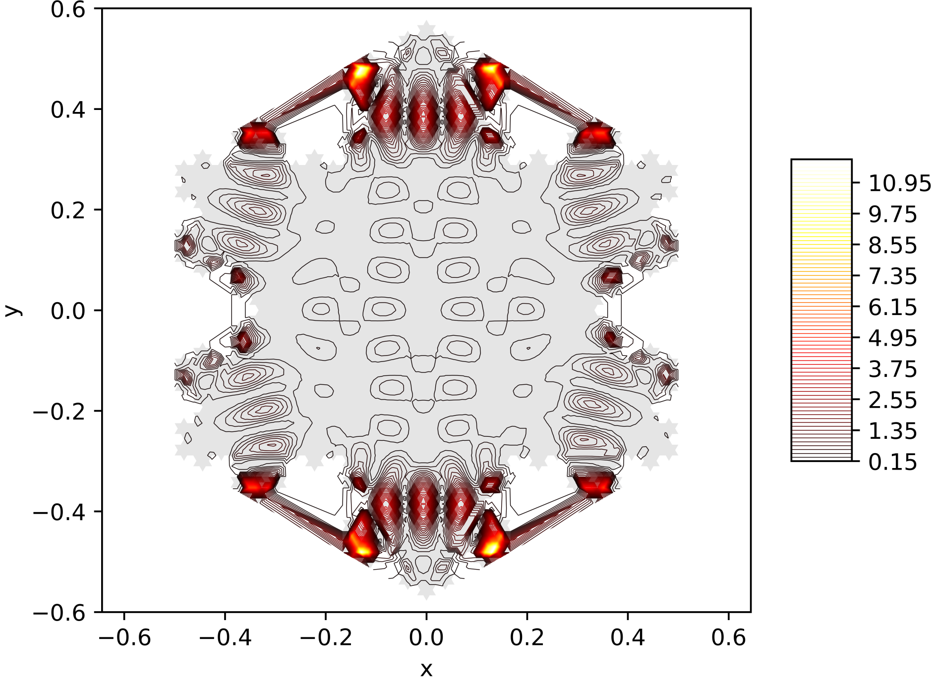
Contour Lines of the Energy Function of the 148. Eigenfunction on the Snowflake (Level 5, Res. 81) with Neumann BC
