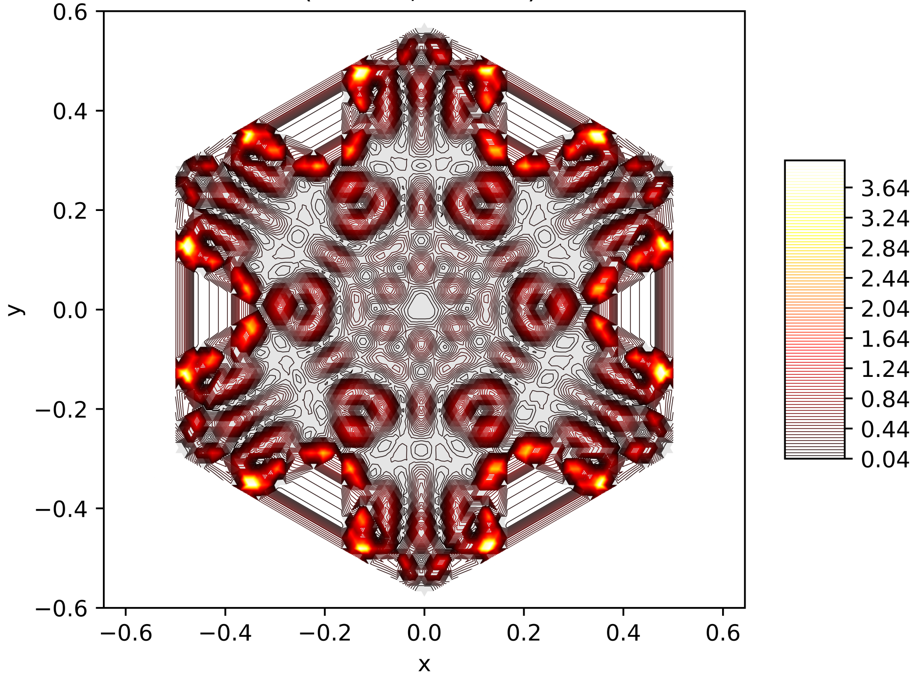
Contour Lines of the Energy Function of the 150. Eigenfunction on the Snowflake (Level 5, Res. 81) with Neumann BC
