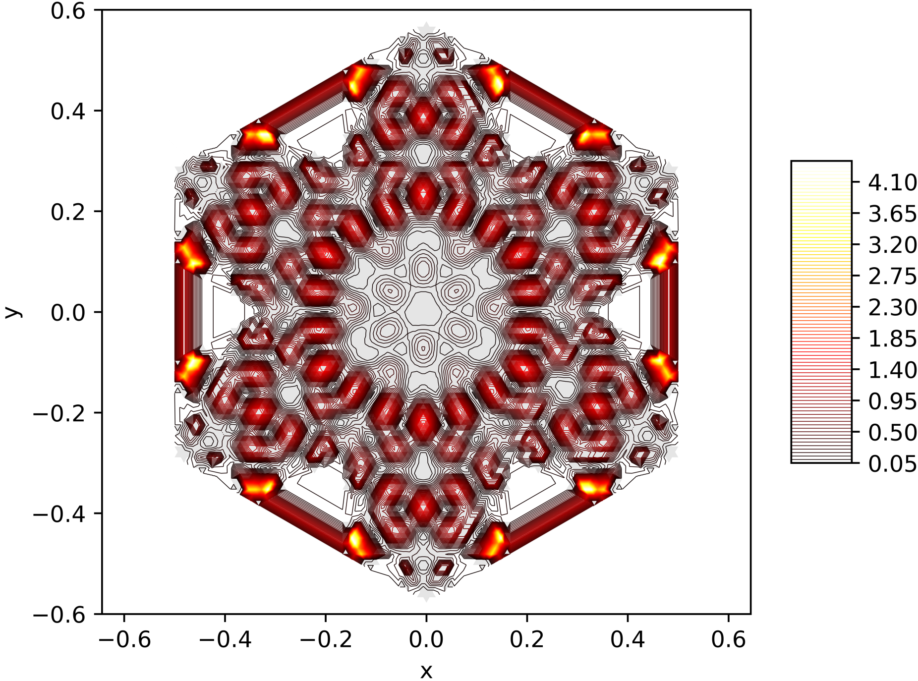
Contour Lines of the Energy Function of the 155. Eigenfunction on the Snowflake (Level 5, Res. 81) with Neumann BC
