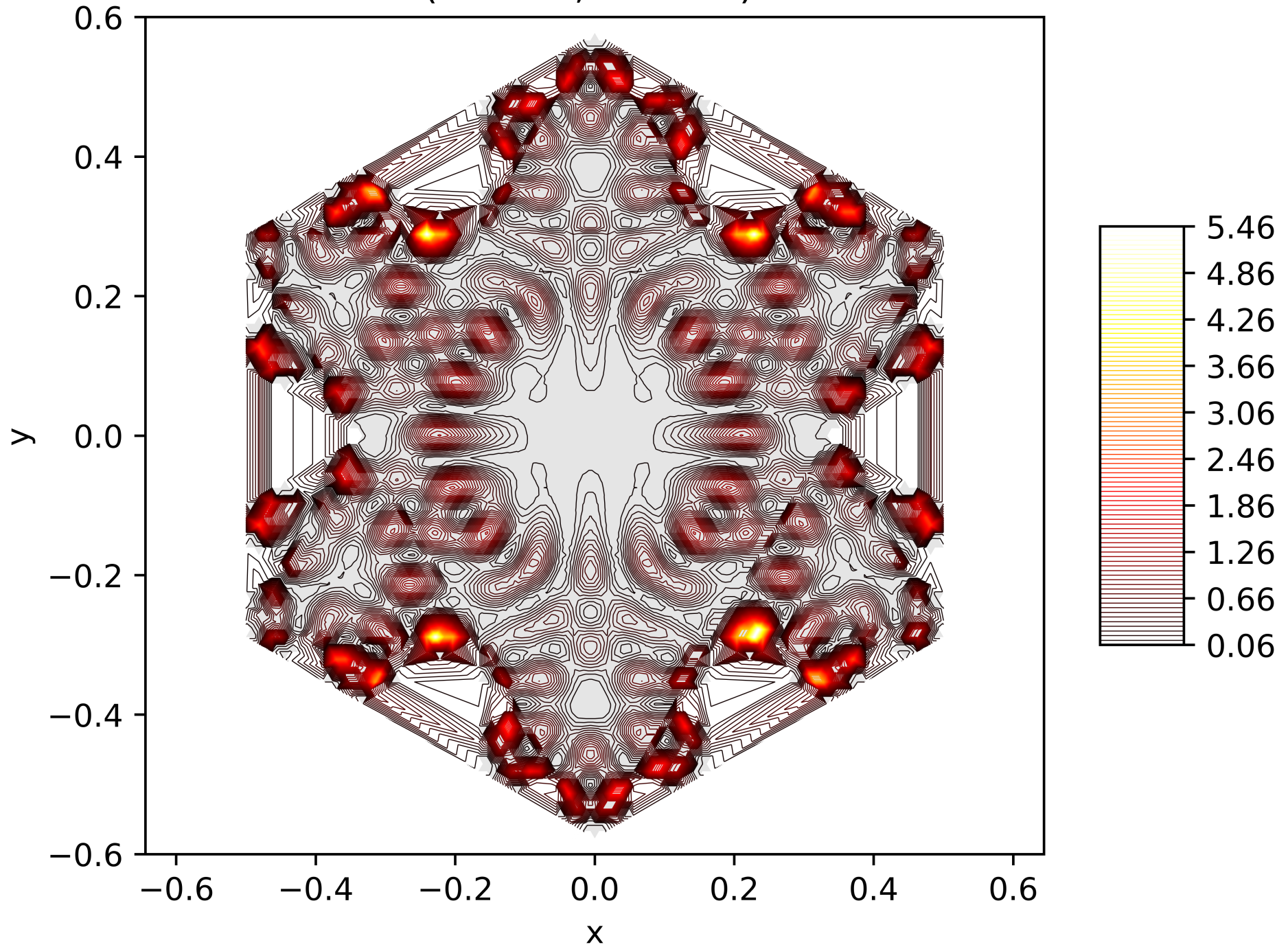
Contour Lines of the Energy Function of the 141. Eigenfunction on the Snowflake (Level 5, Res. 81) with Neumann BC
