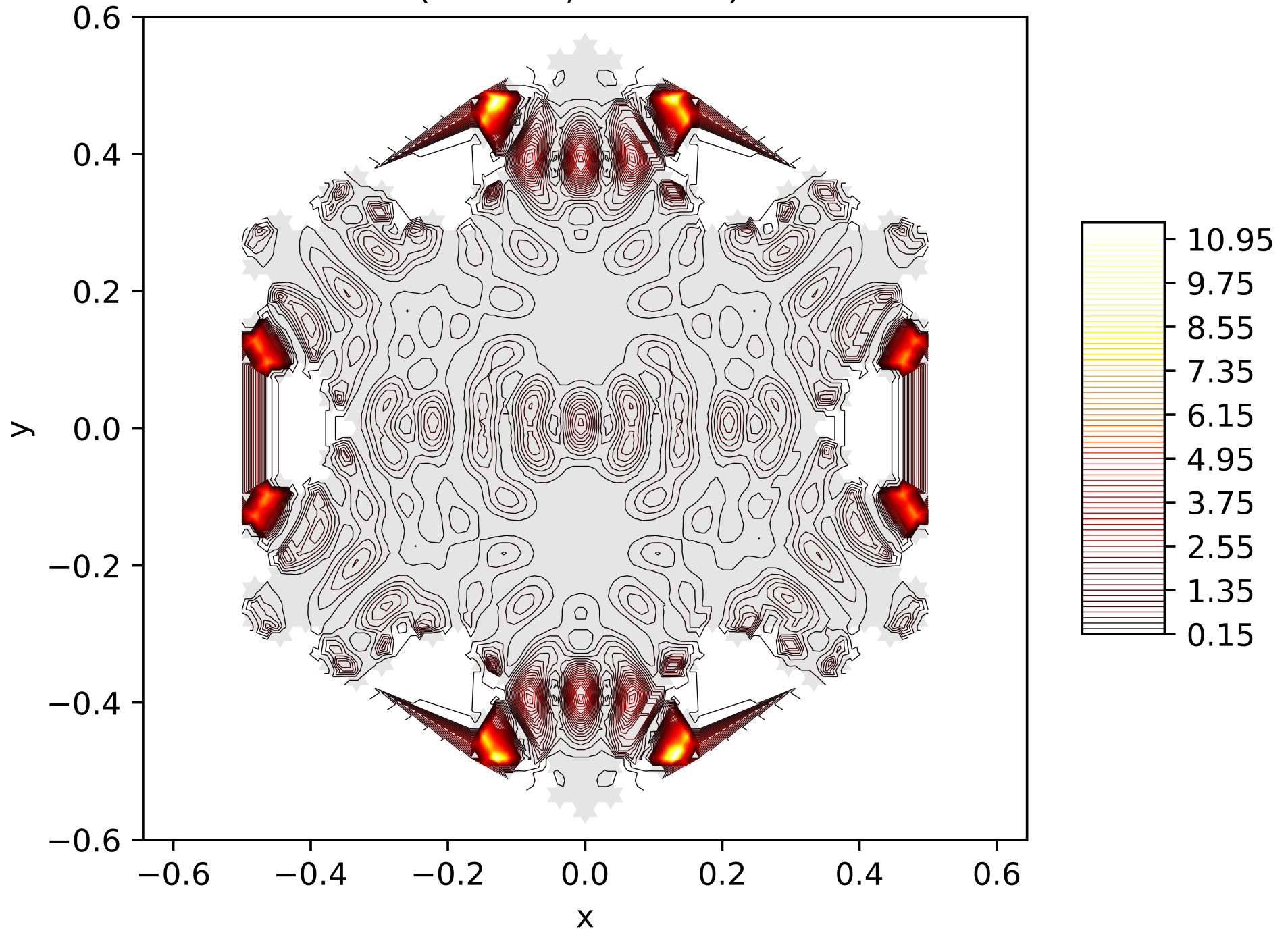
Contour Lines of the Energy Function of the 152. Eigenfunction on the Snowflake (Level 5, Res. 81) with Neumann BC
