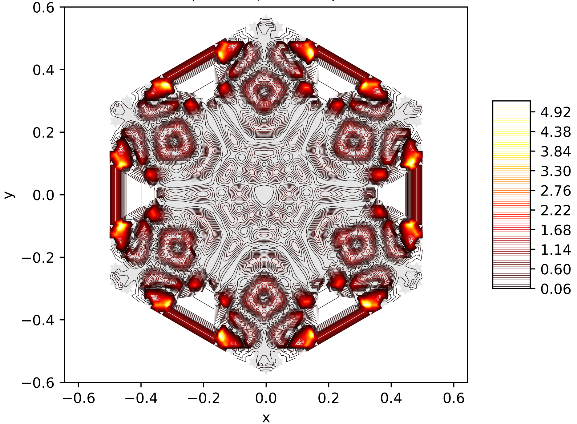
Contour Lines of the Energy Function of the 144. Eigenfunction on the Snowflake (Level 5, Res. 81) with Neumann BC
