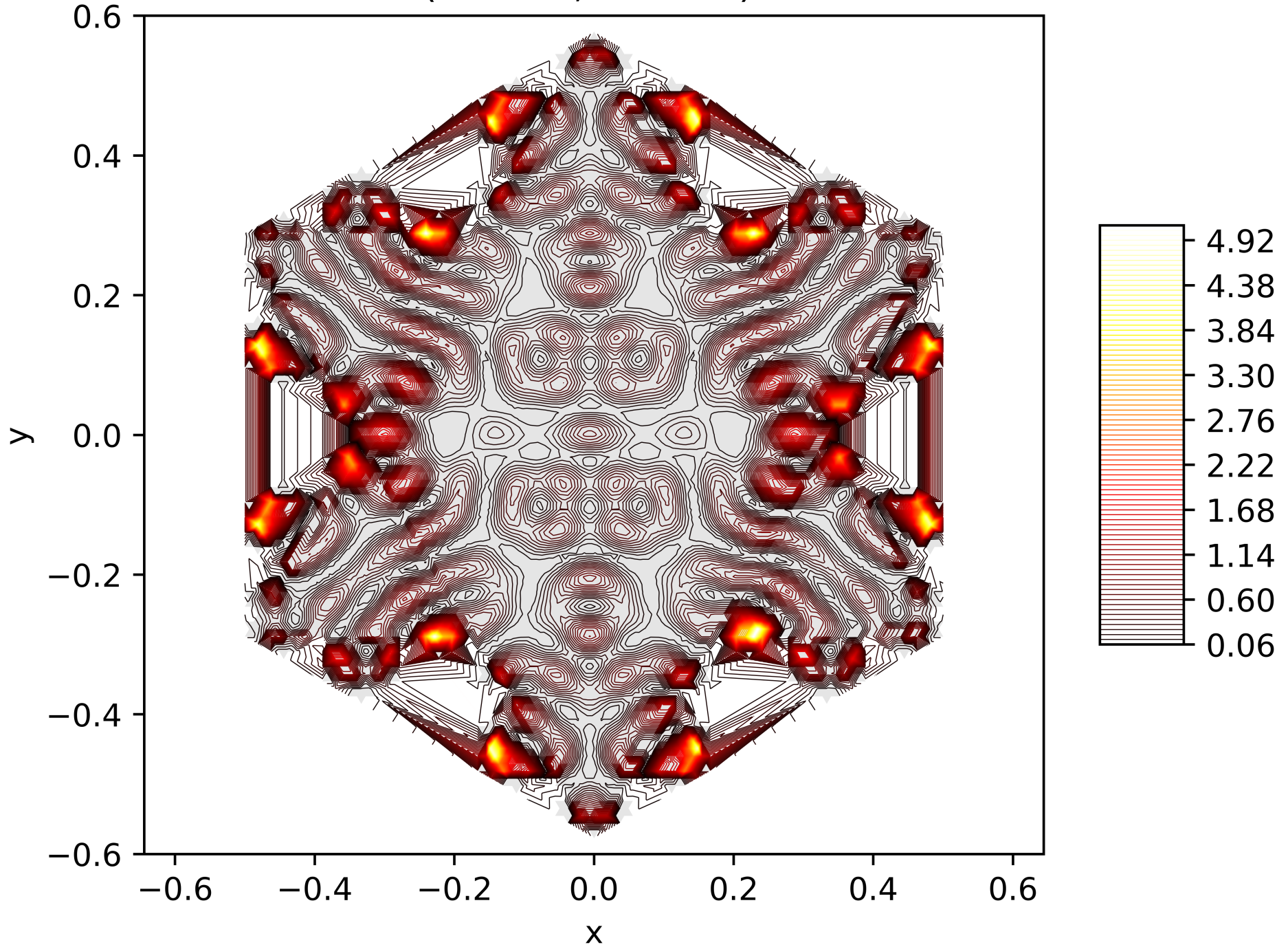
Contour Lines of the Energy Function of the 147. Eigenfunction on the Snowflake (Level 5, Res. 81) with Neumann BC
