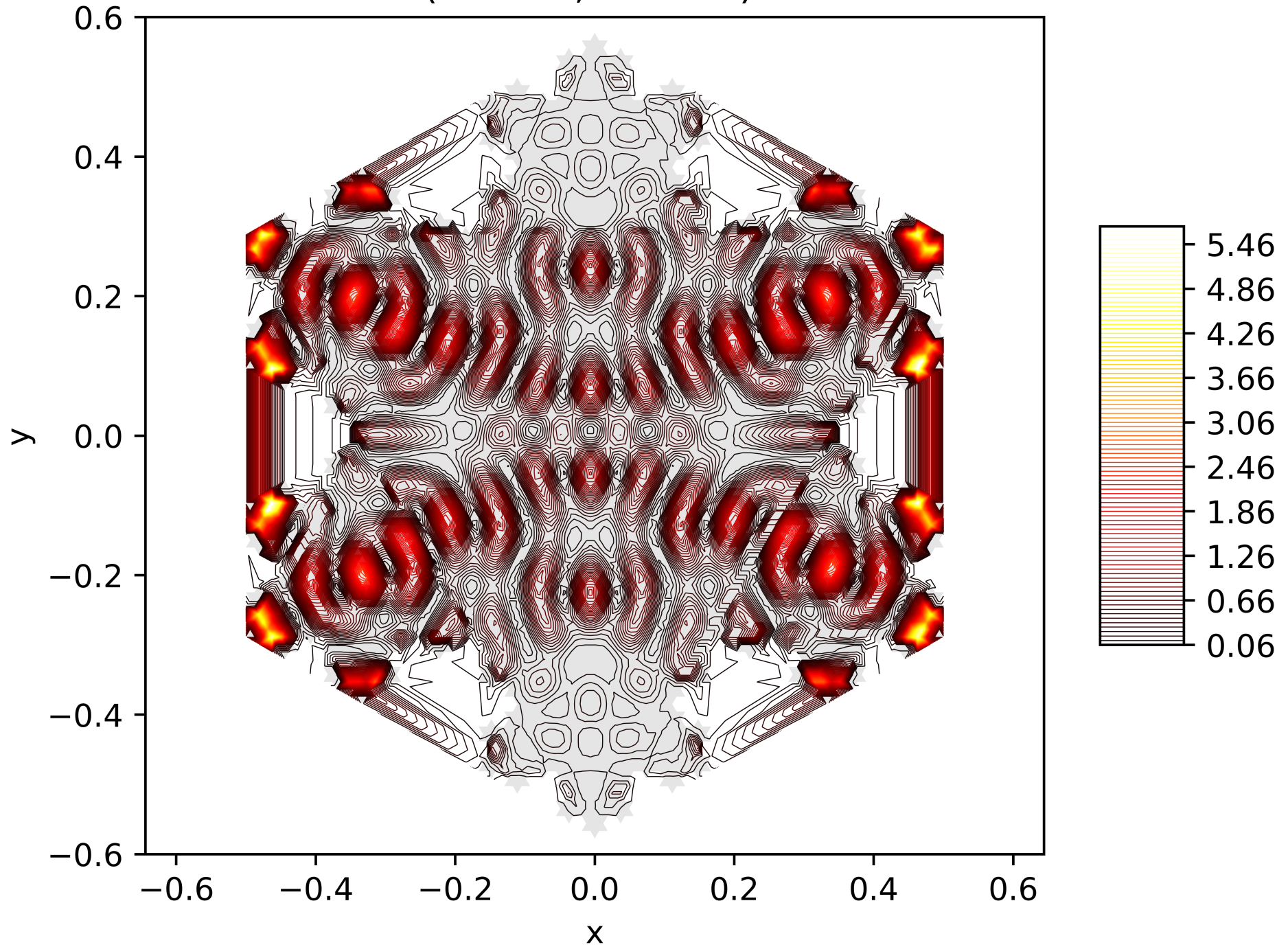
Contour Lines of the Energy Function of the 154. Eigenfunction on the Snowflake (Level 5, Res. 81) with Neumann BC
