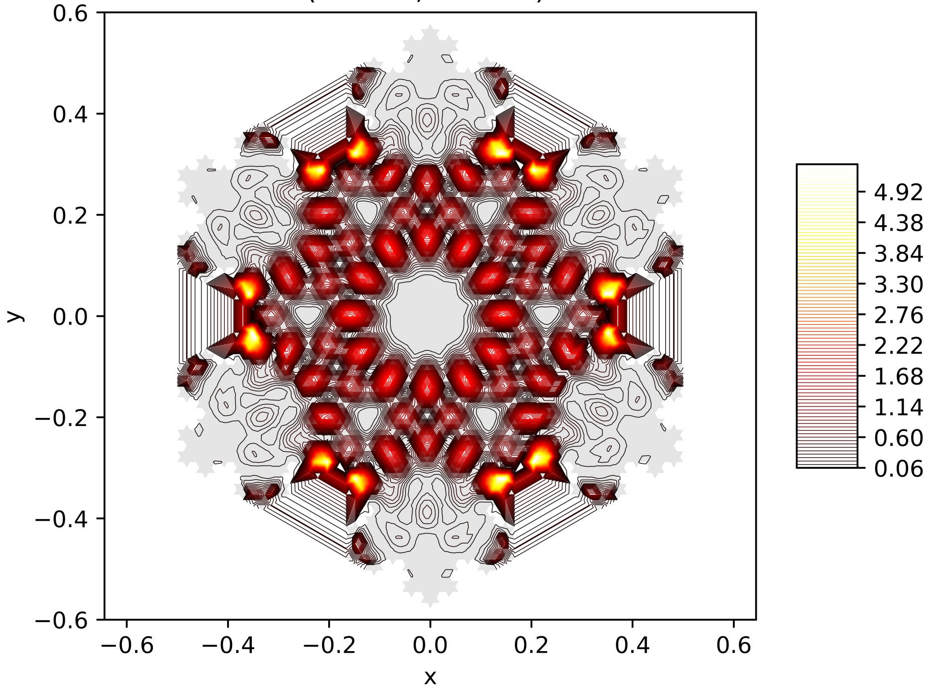
Contour Lines of the Energy Function of the 159. Eigenfunction on the Snowflake (Level 5, Res. 81) with Neumann BC
