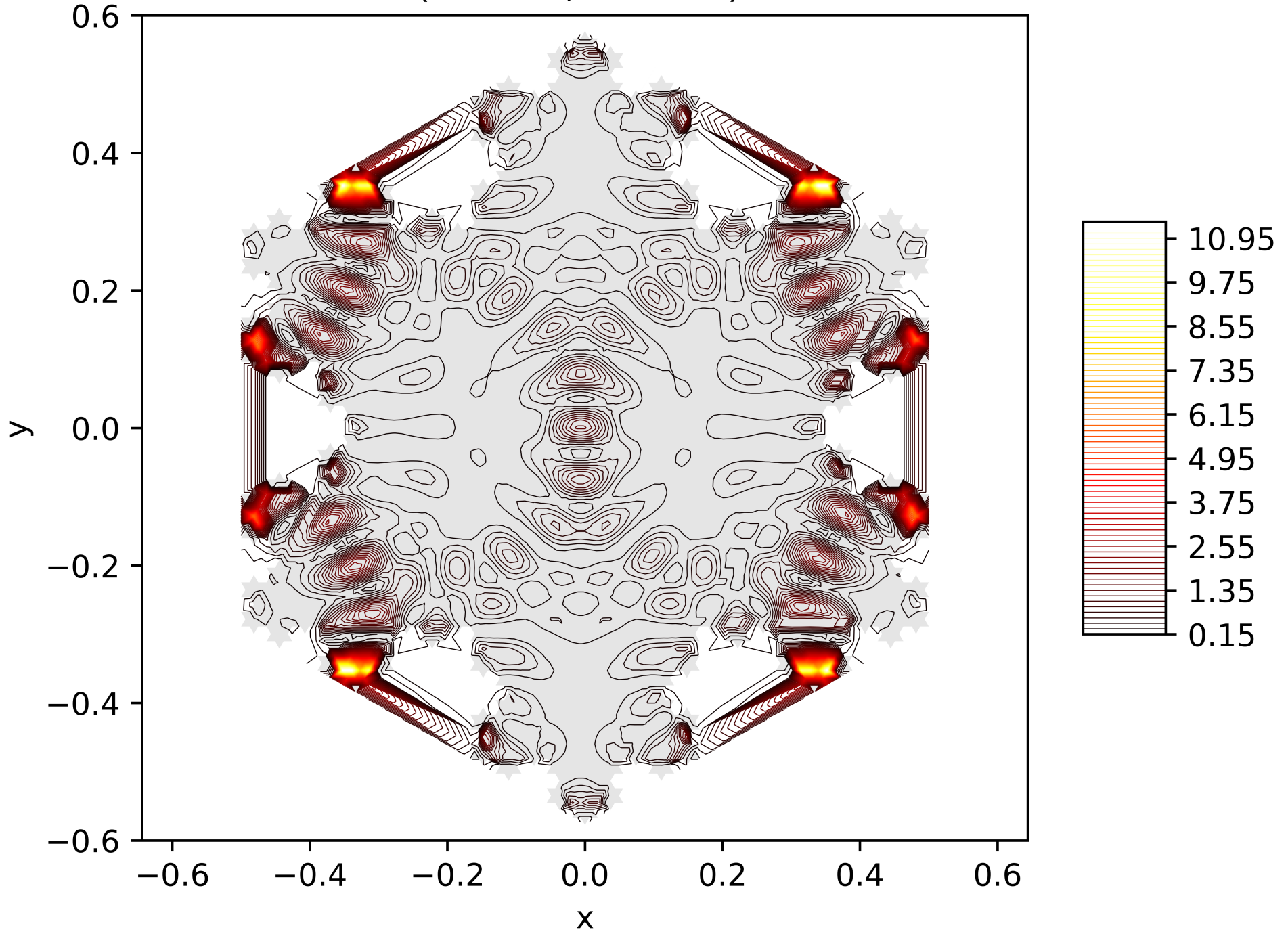
Contour Lines of the Energy Function of the 151. Eigenfunction on the Snowflake (Level 5, Res. 81) with Neumann BC
