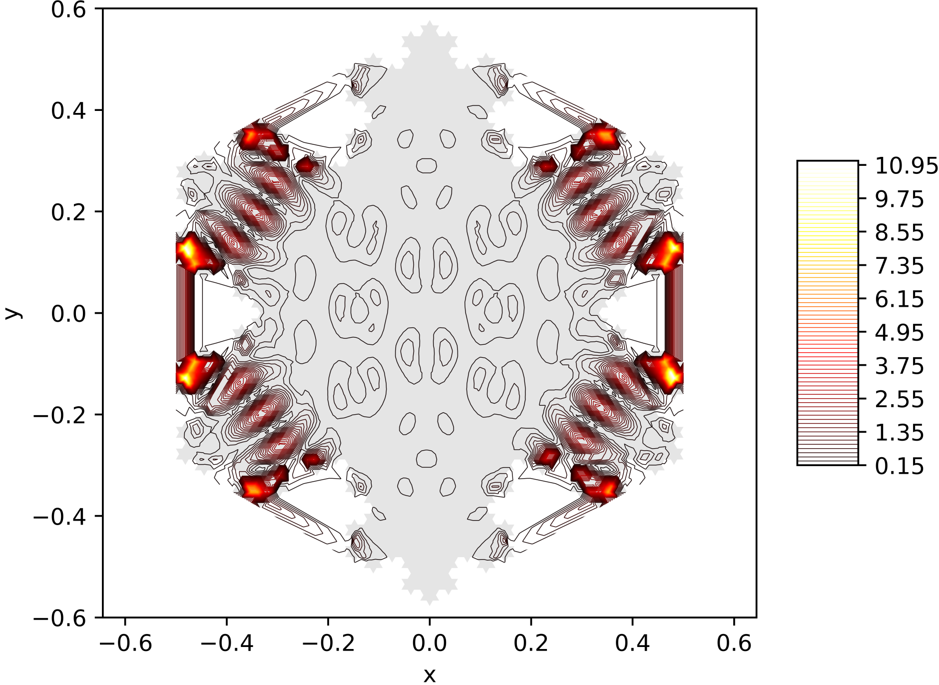
Contour Lines of the Energy Function of the 149. Eigenfunction on the Snowflake (Level 5, Res. 81) with Neumann BC
