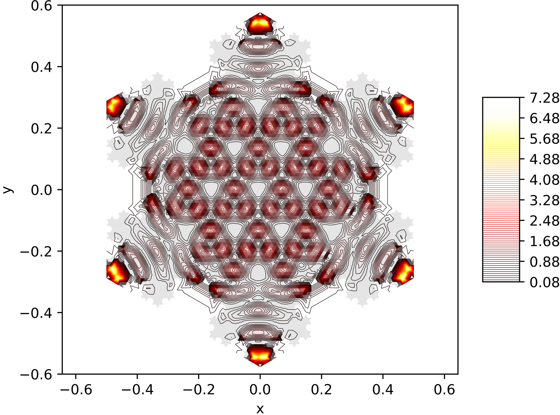
Contour Lines of the Energy Function of the 156. Eigenfunction on the Snowflake (Level 5, Res. 81) with Neumann BC
