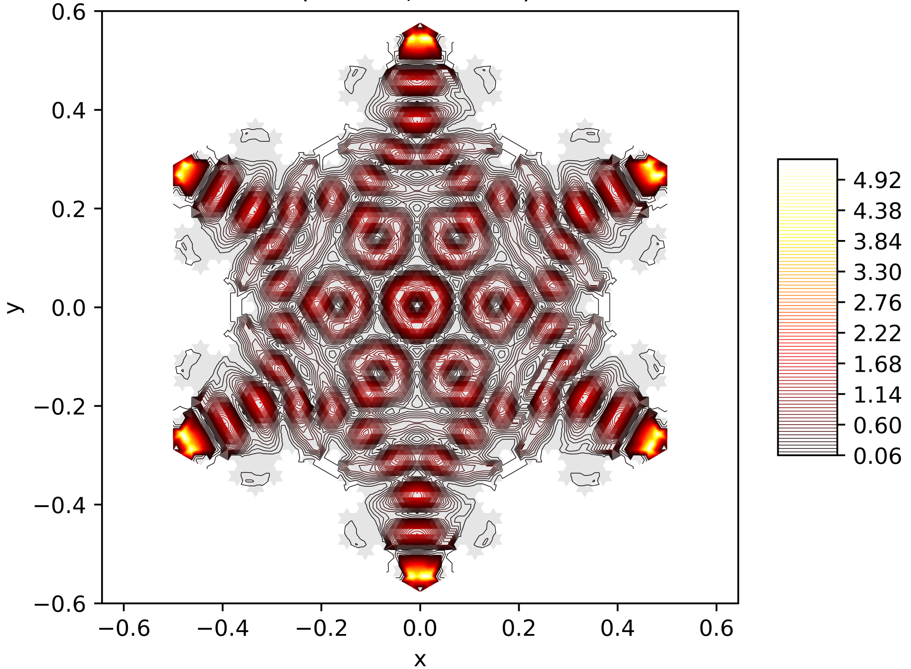
Contour Lines of the Energy Function of the 143. Eigenfunction on the Snowflake (Level 5, Res. 81) with Neumann BC
