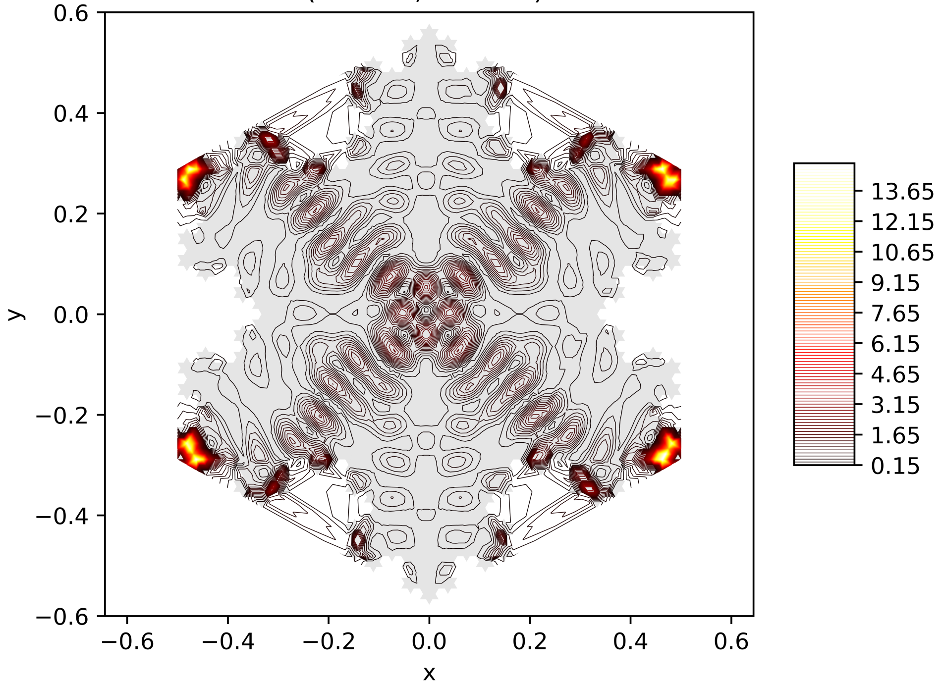
Contour Lines of the Energy Function of the 168. Eigenfunction on the Snowflake (Level 5, Res. 81) with Neumann BC
