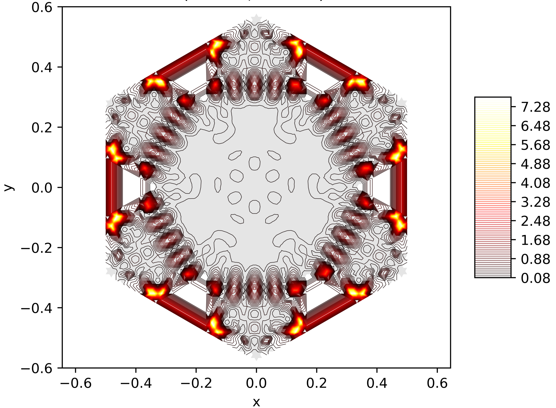
Contour Lines of the Energy Function of the 175. Eigenfunction on the Snowflake (Level 5, Res. 81) with Neumann BC
