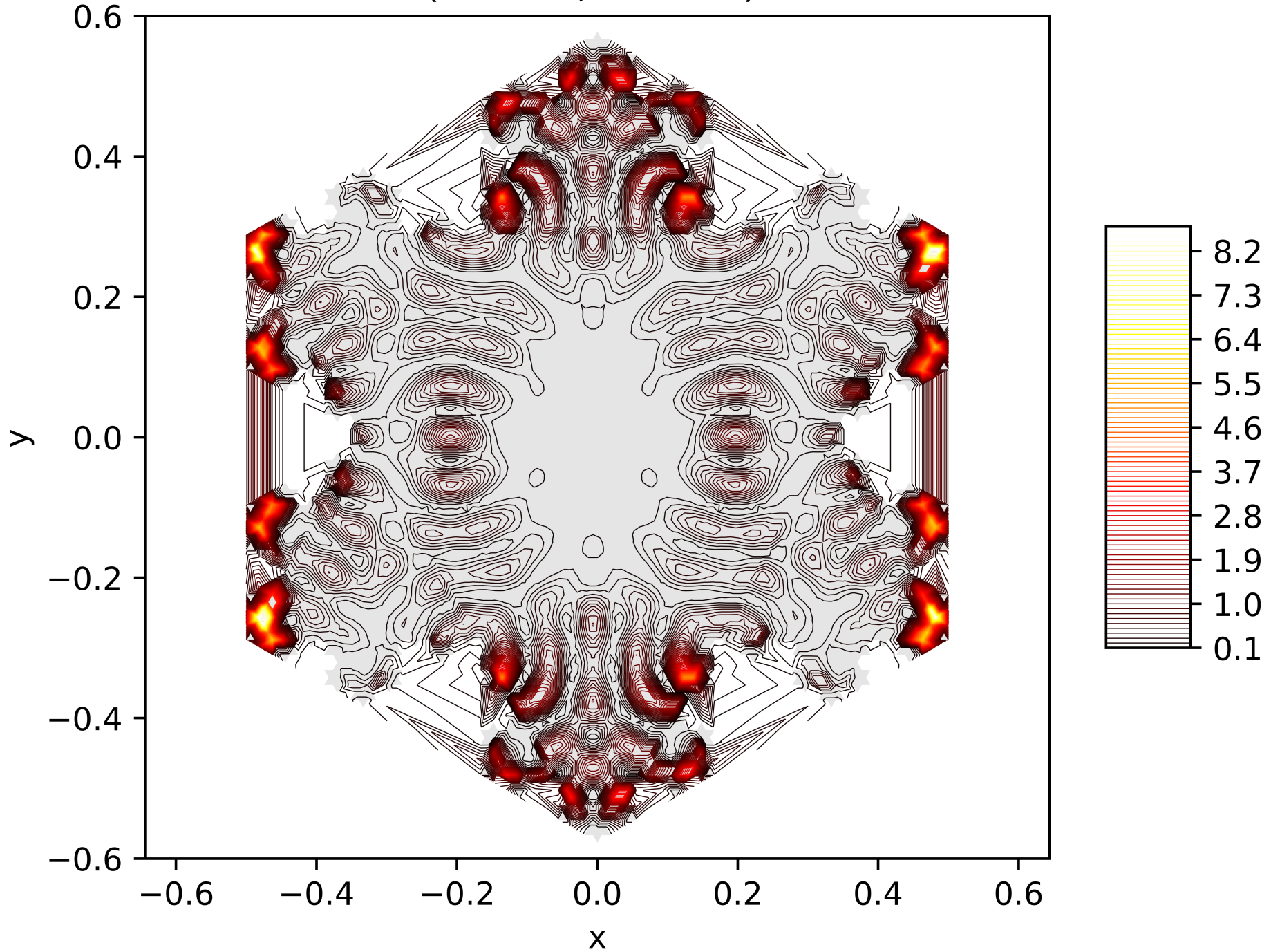
Contour Lines of the Energy Function of the 173. Eigenfunction on the Snowflake (Level 5, Res. 81) with Neumann BC
