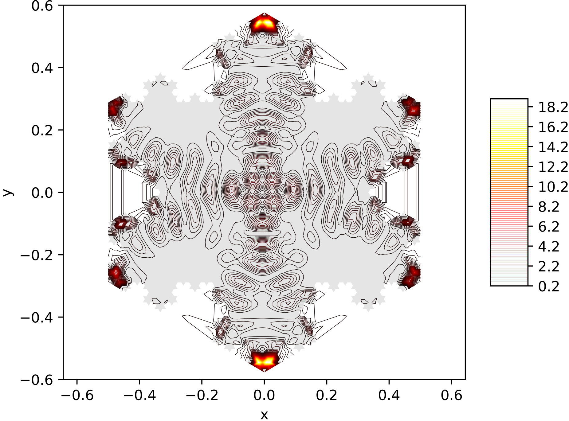
Contour Lines of the Energy Function of the 167. Eigenfunction on the Snowflake (Level 5, Res. 81) with Neumann BC
