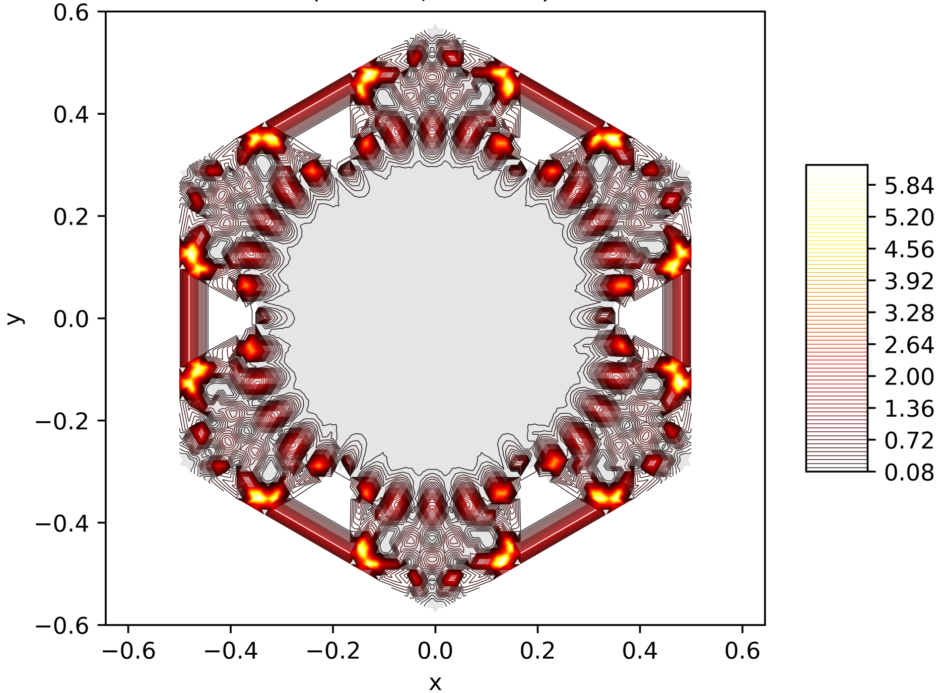
Contour Lines of the Energy Function of the 178. Eigenfunction on the Snowflake (Level 5, Res. 81) with Neumann BC
