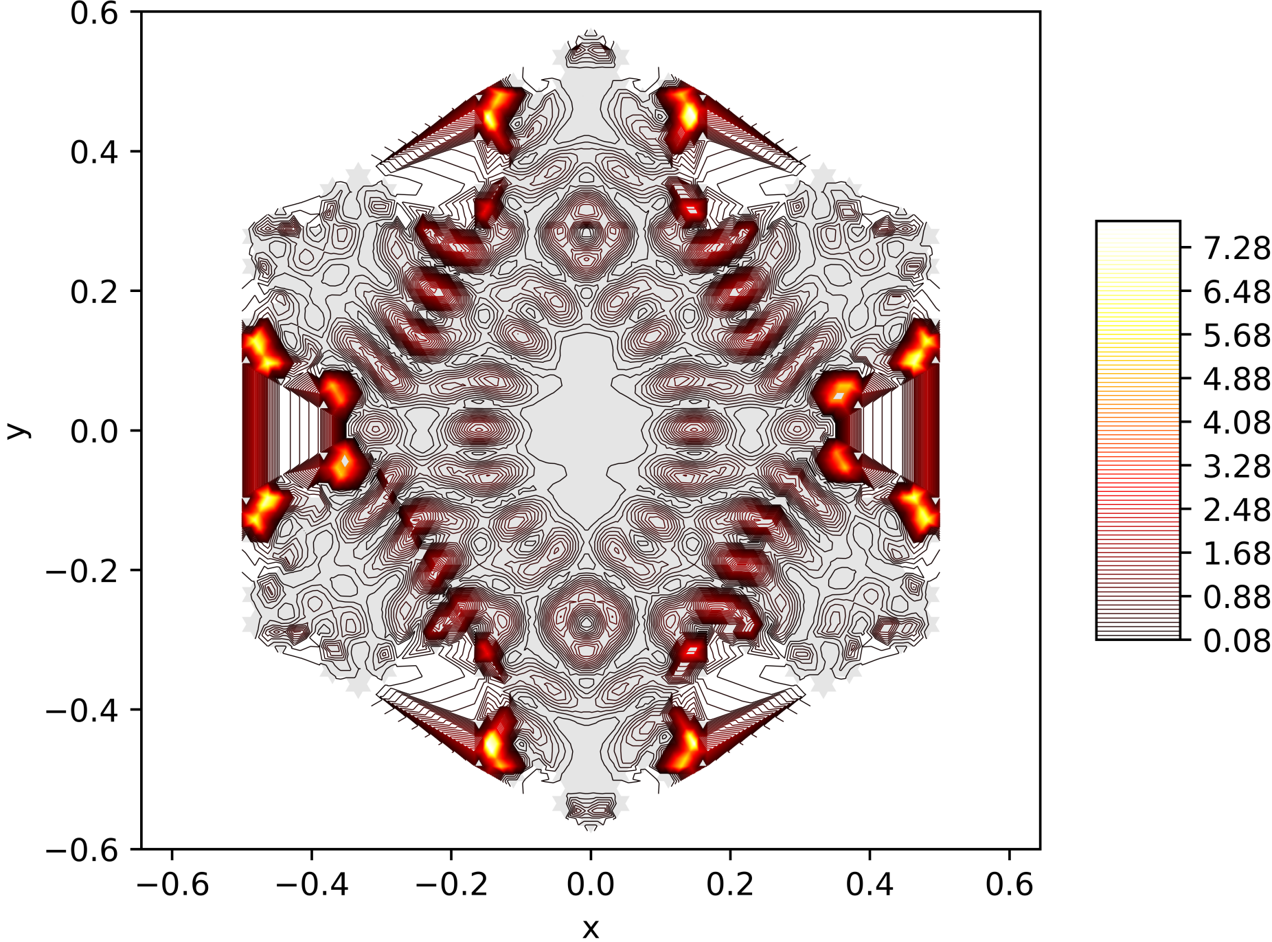
Contour Lines of the Energy Function of the 166. Eigenfunction on the Snowflake (Level 5, Res. 81) with Neumann BC
