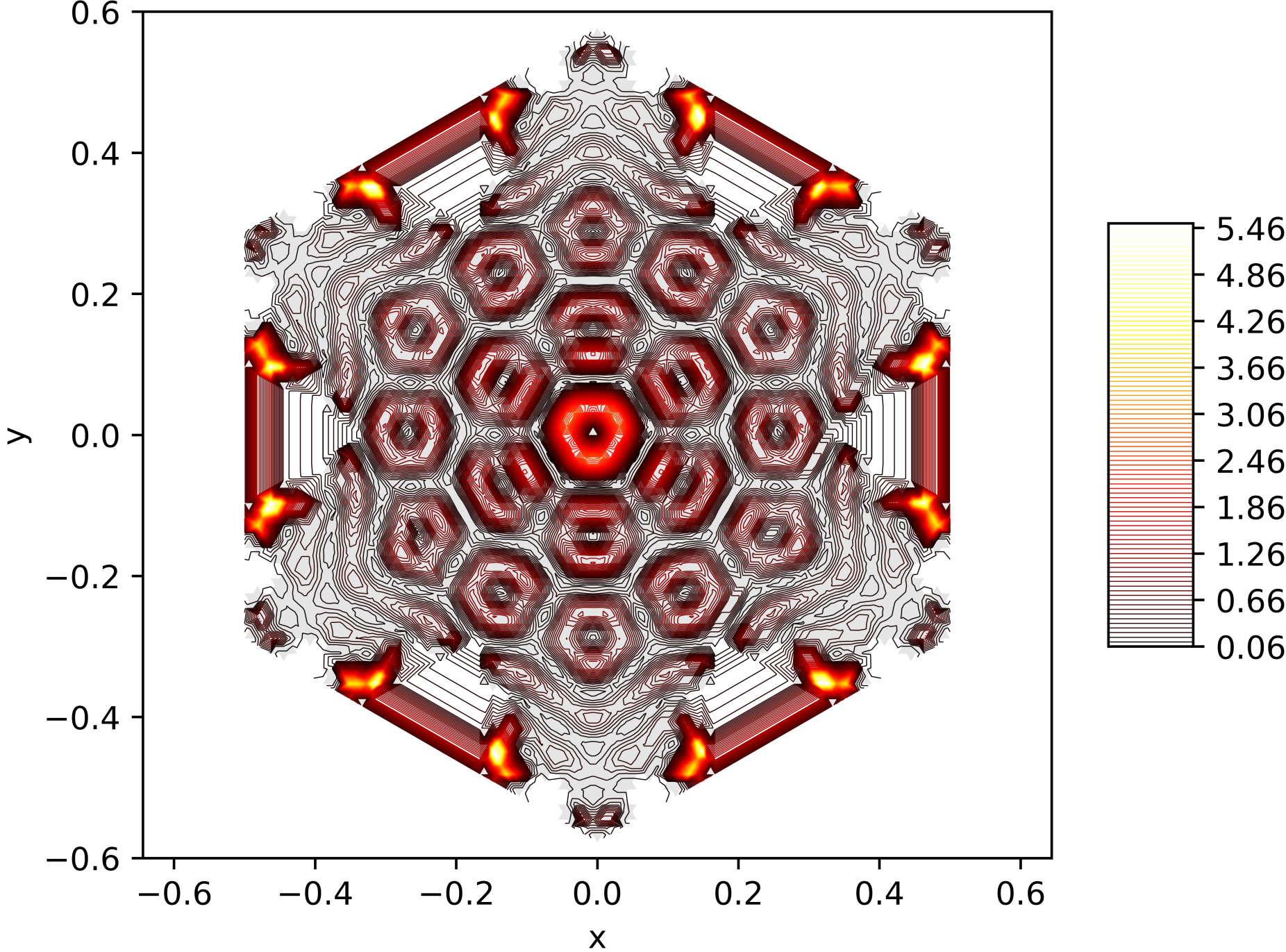
Contour Lines of the Energy Function of the 164. Eigenfunction on the Snowflake (Level 5, Res. 81) with Neumann BC
