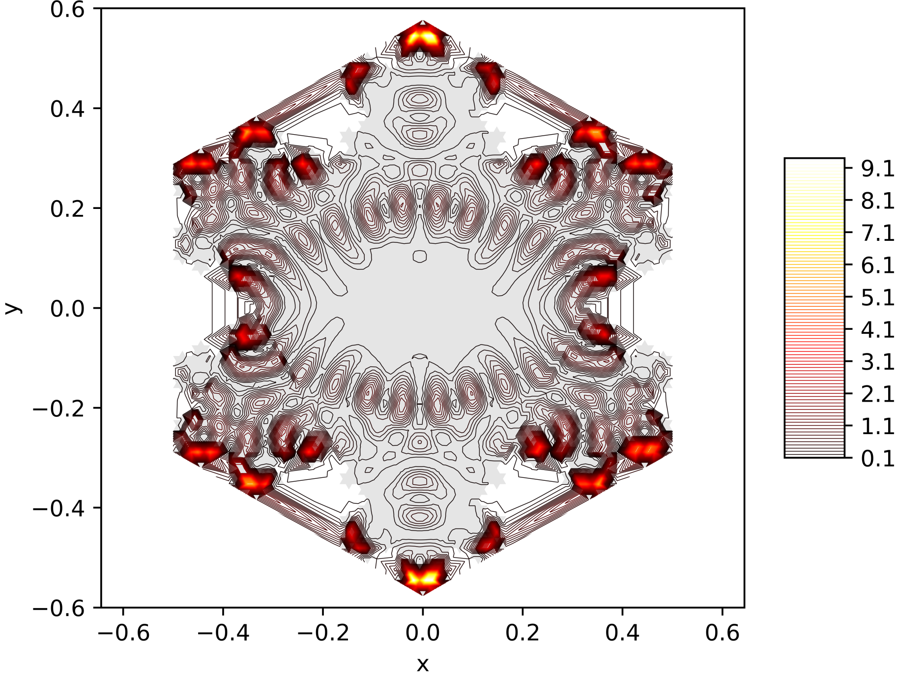
Contour Lines of the Energy Function of the 174. Eigenfunction on the Snowflake (Level 5, Res. 81) with Neumann BC
