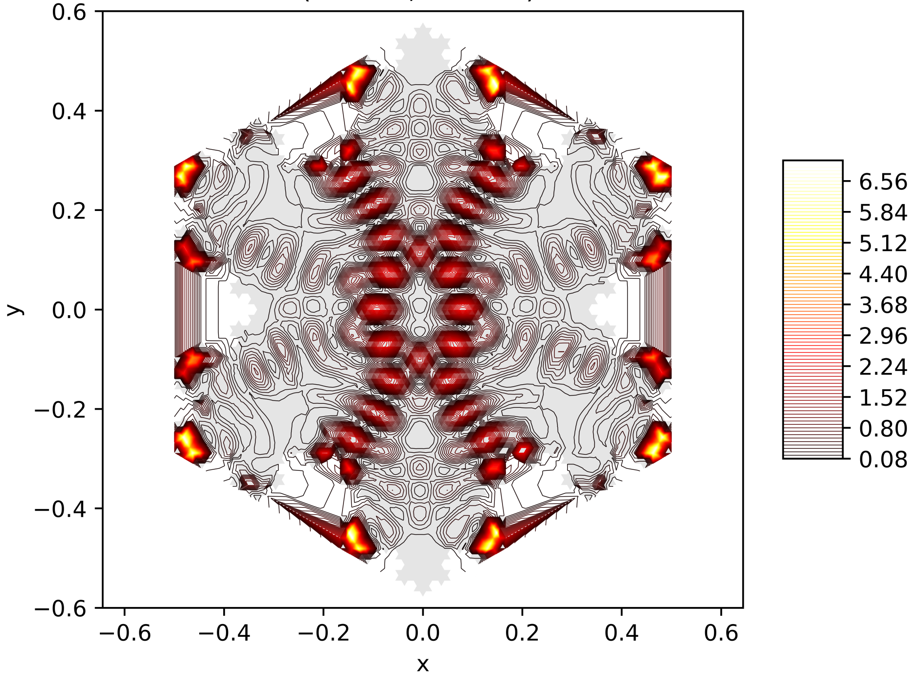
Contour Lines of the Energy Function of the 163. Eigenfunction on the Snowflake (Level 5, Res. 81) with Neumann BC
