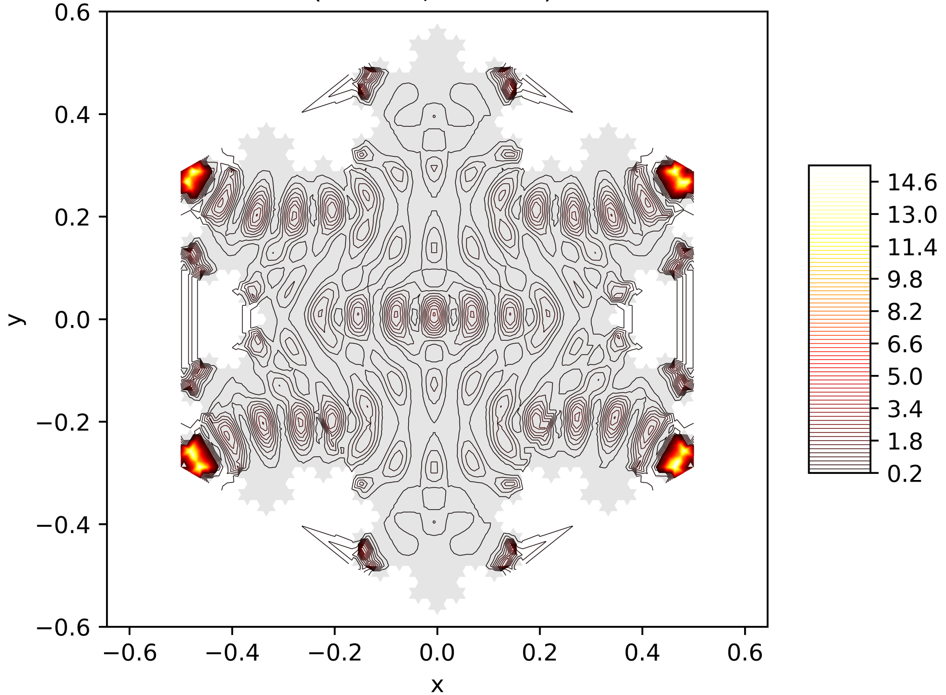
Contour Lines of the Energy Function of the 161. Eigenfunction on the Snowflake (Level 5, Res. 81) with Neumann BC
