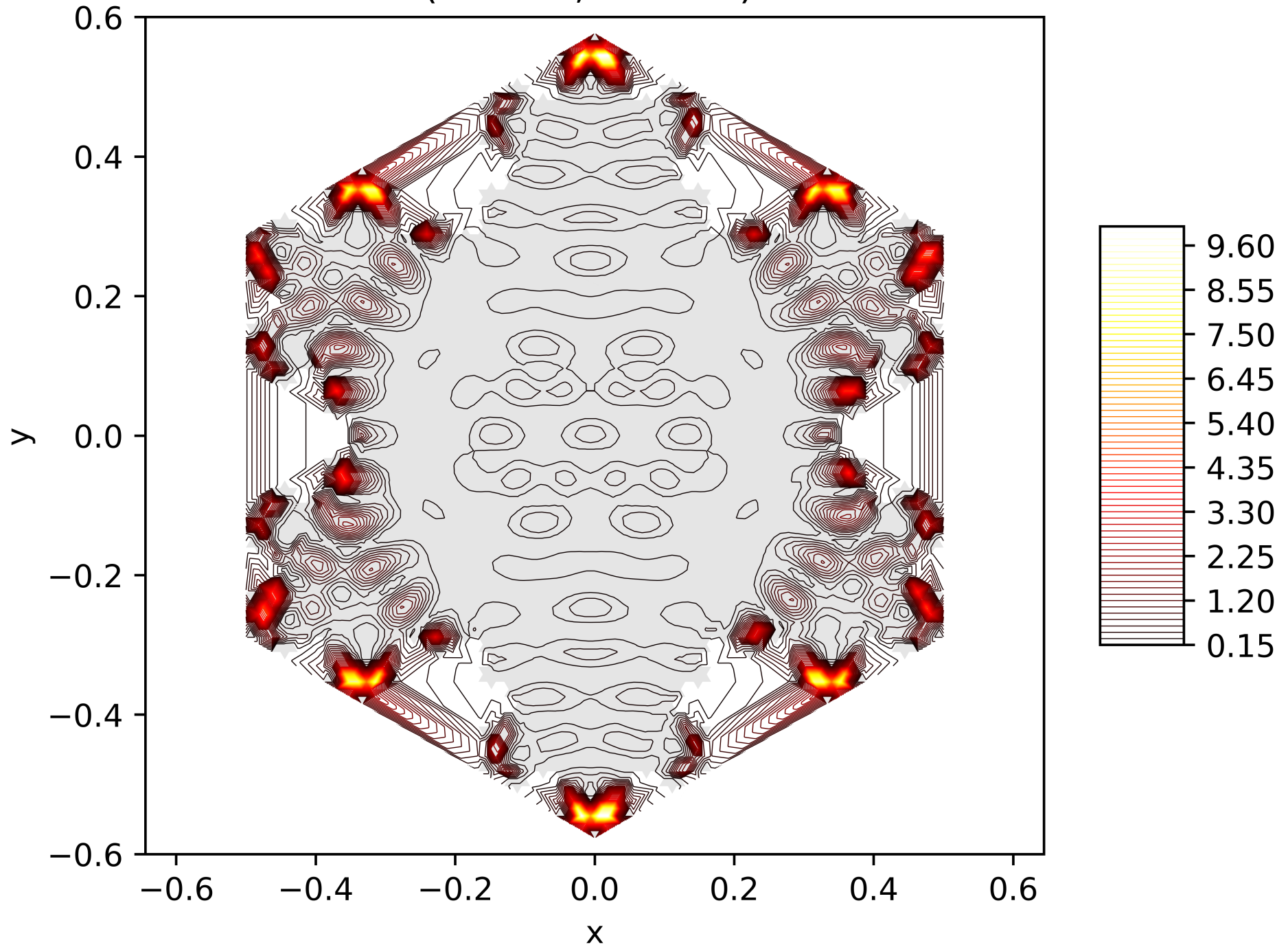
Contour Lines of the Energy Function of the 179. Eigenfunction on the Snowflake (Level 5, Res. 81) with Neumann BC
