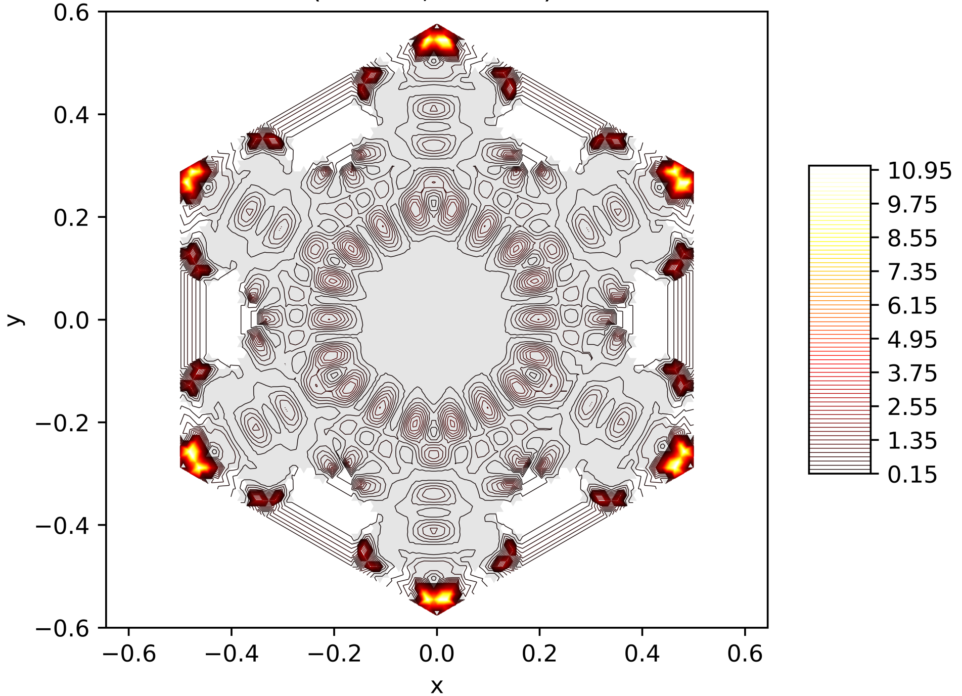
Contour Lines of the Energy Function of the 169. Eigenfunction on the Snowflake (Level 5, Res. 81) with Neumann BC
