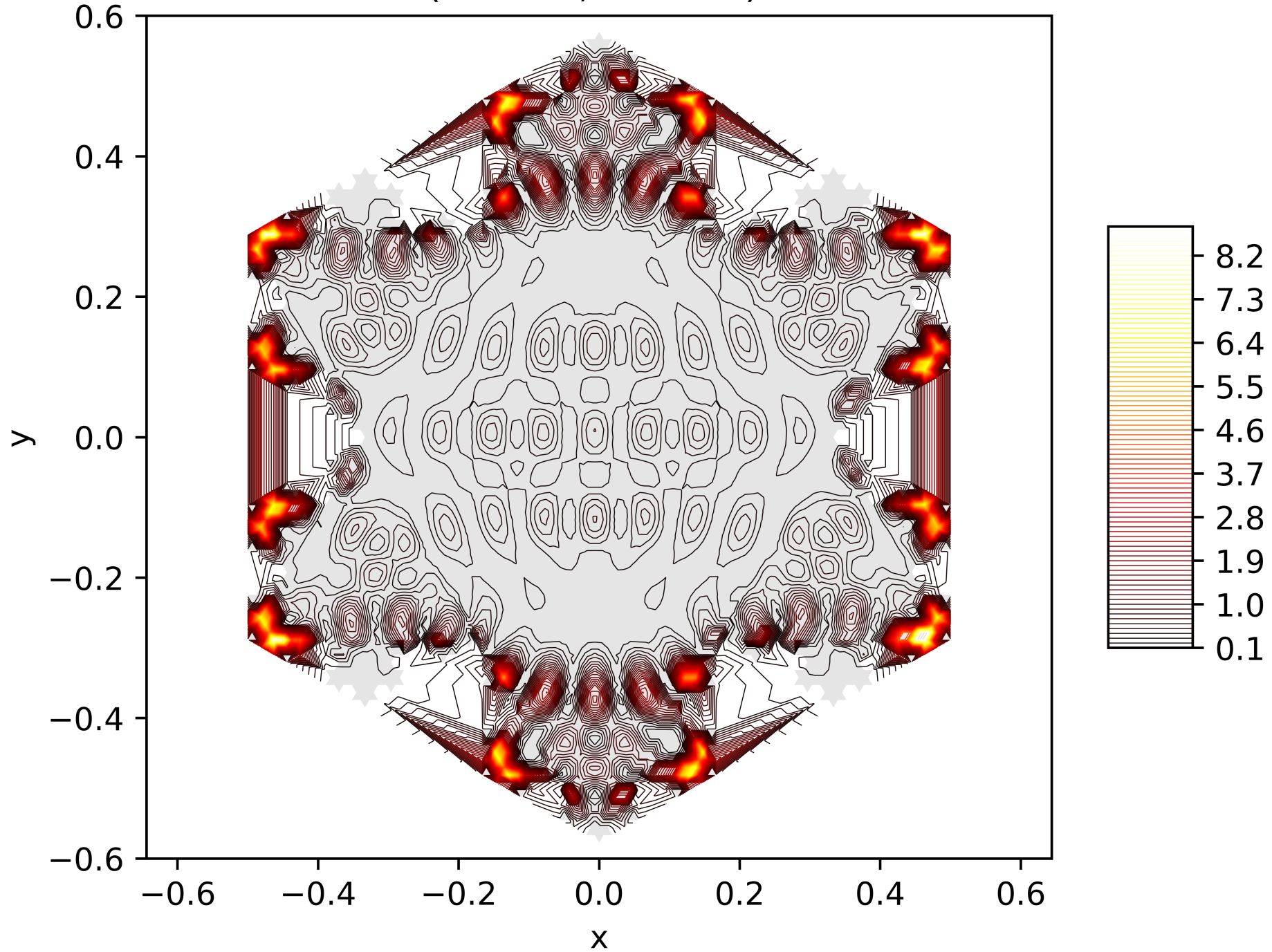
Contour Lines of the Energy Function of the 180. Eigenfunction on the Snowflake (Level 5, Res. 81) with Neumann BC
