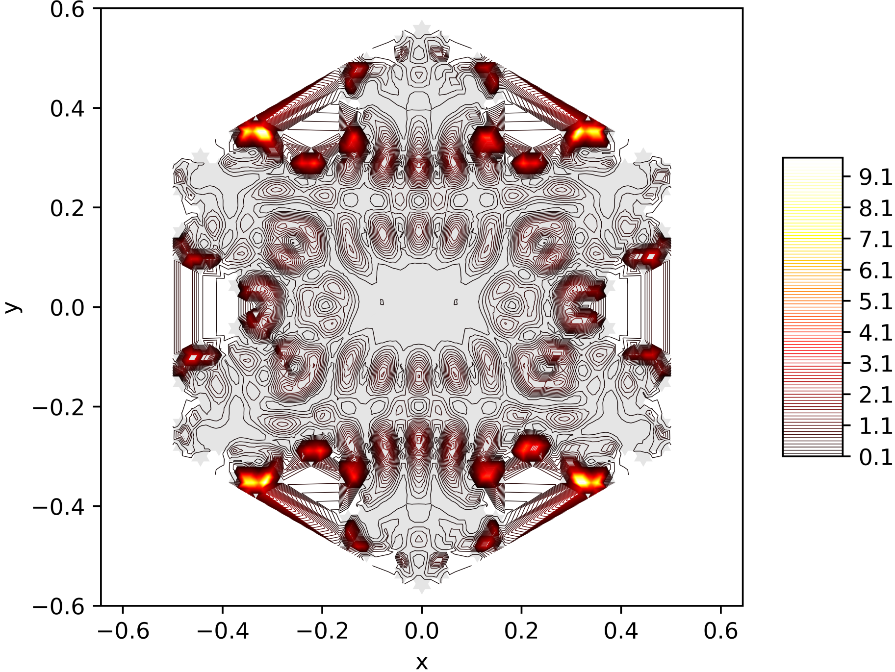
Contour Lines of the Energy Function of the 165. Eigenfunction on the Snowflake (Level 5, Res. 81) with Neumann BC
