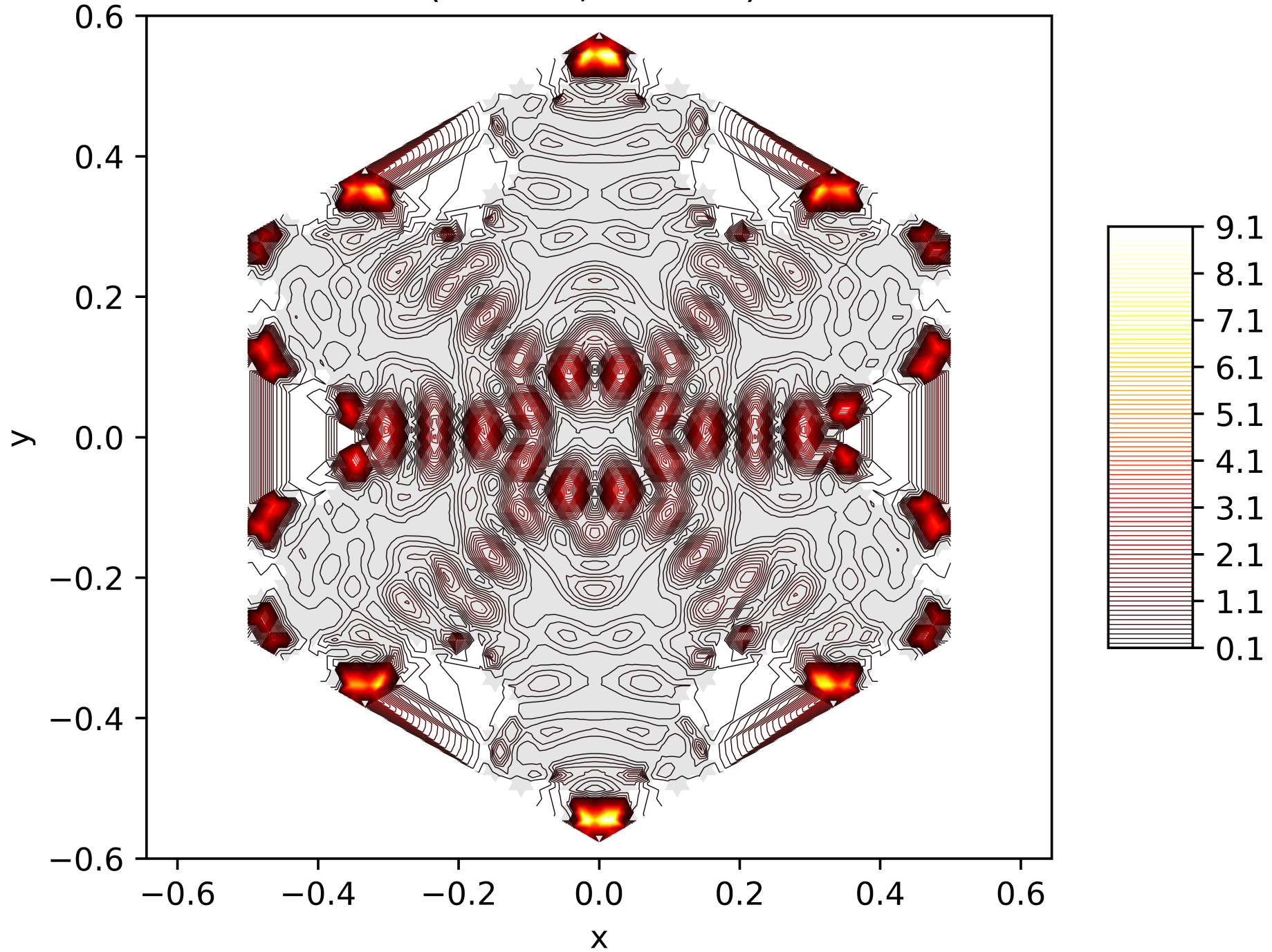
Contour Lines of the Energy Function of the 162. Eigenfunction on the Snowflake (Level 5, Res. 81) with Neumann BC
