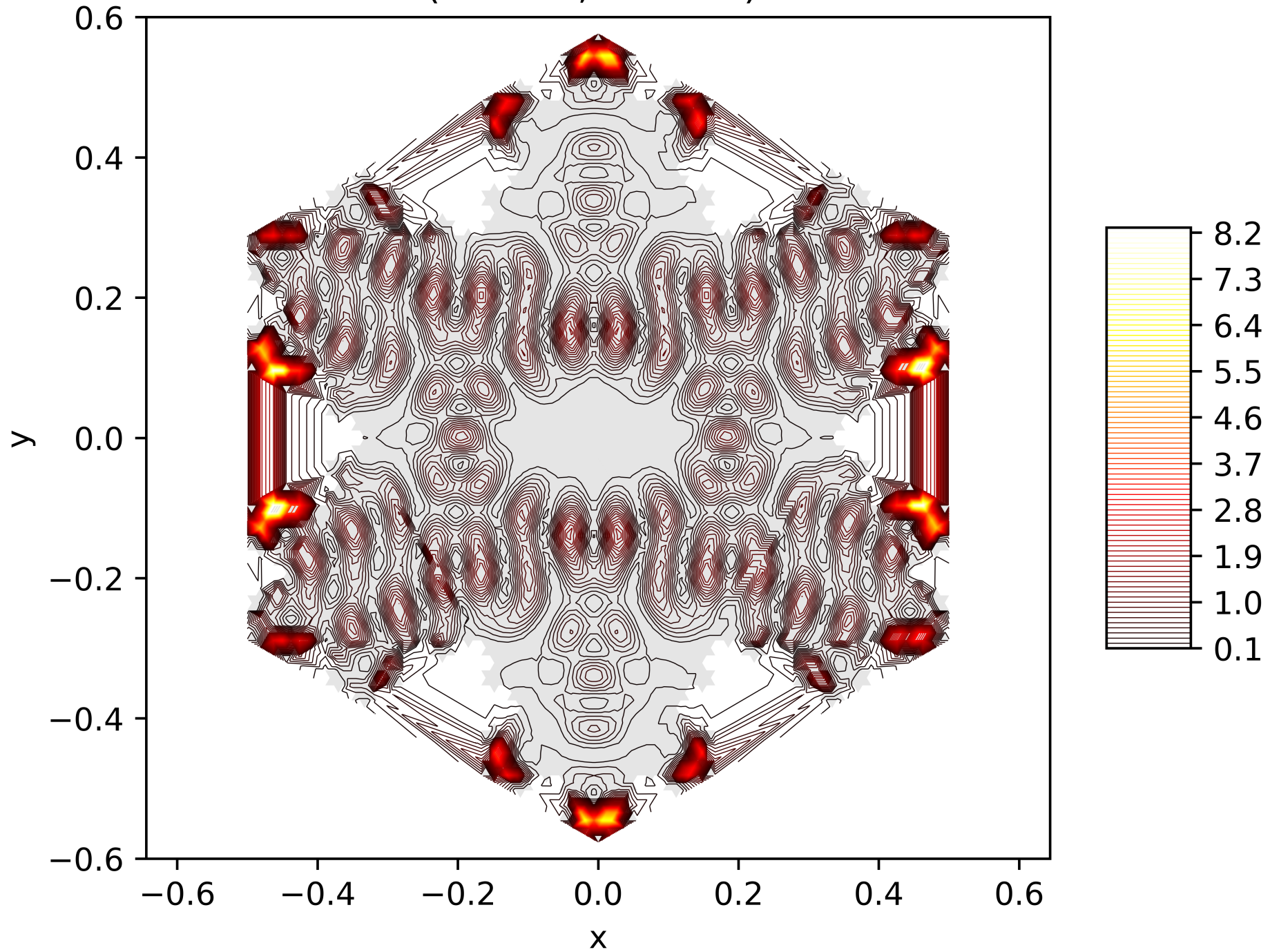
Contour Lines of the Energy Function of the 171. Eigenfunction on the Snowflake (Level 5, Res. 81) with Neumann BC
