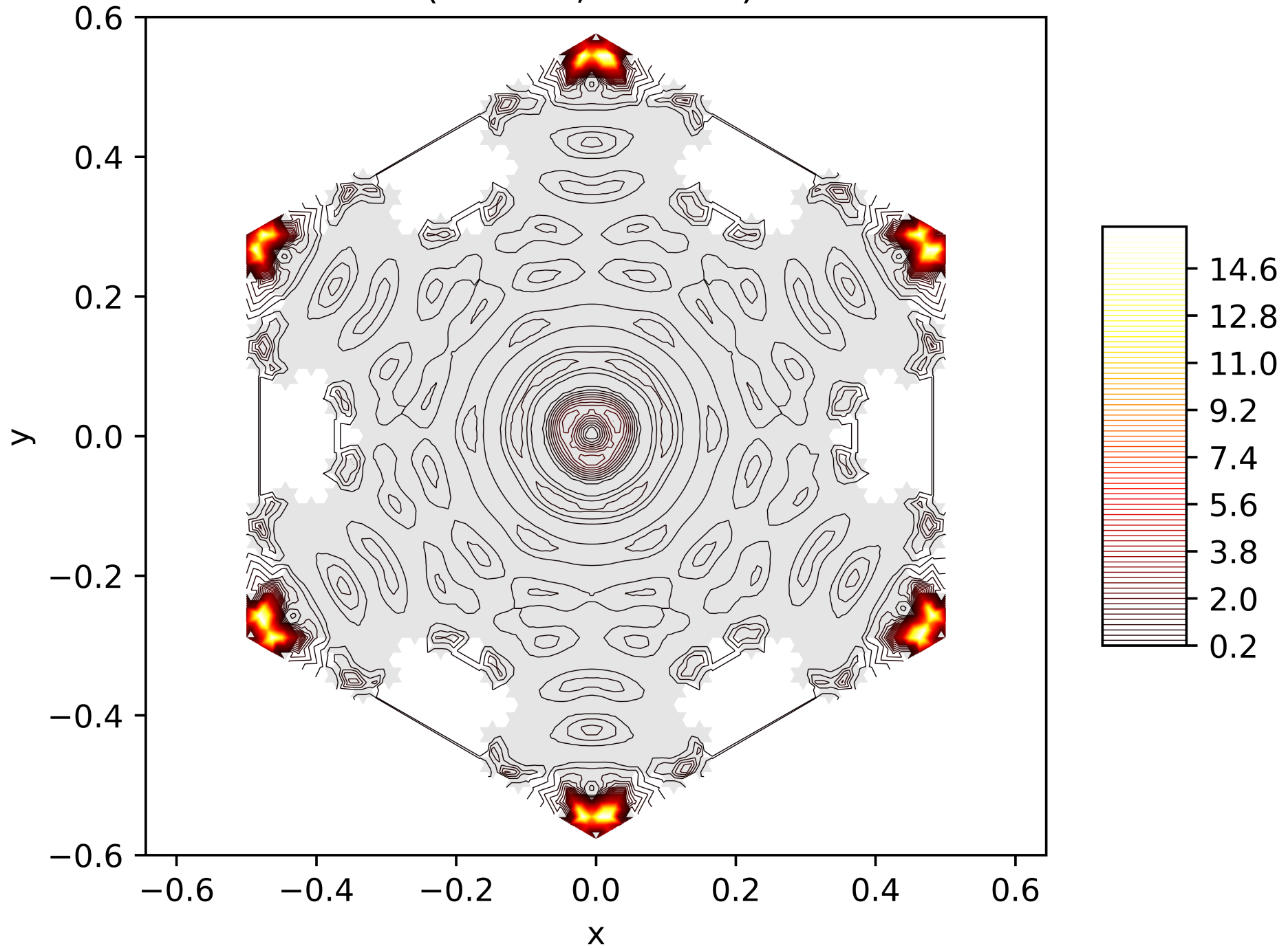
Contour Lines of the Energy Function of the 172. Eigenfunction on the Snowflake (Level 5, Res. 81) with Neumann BC
