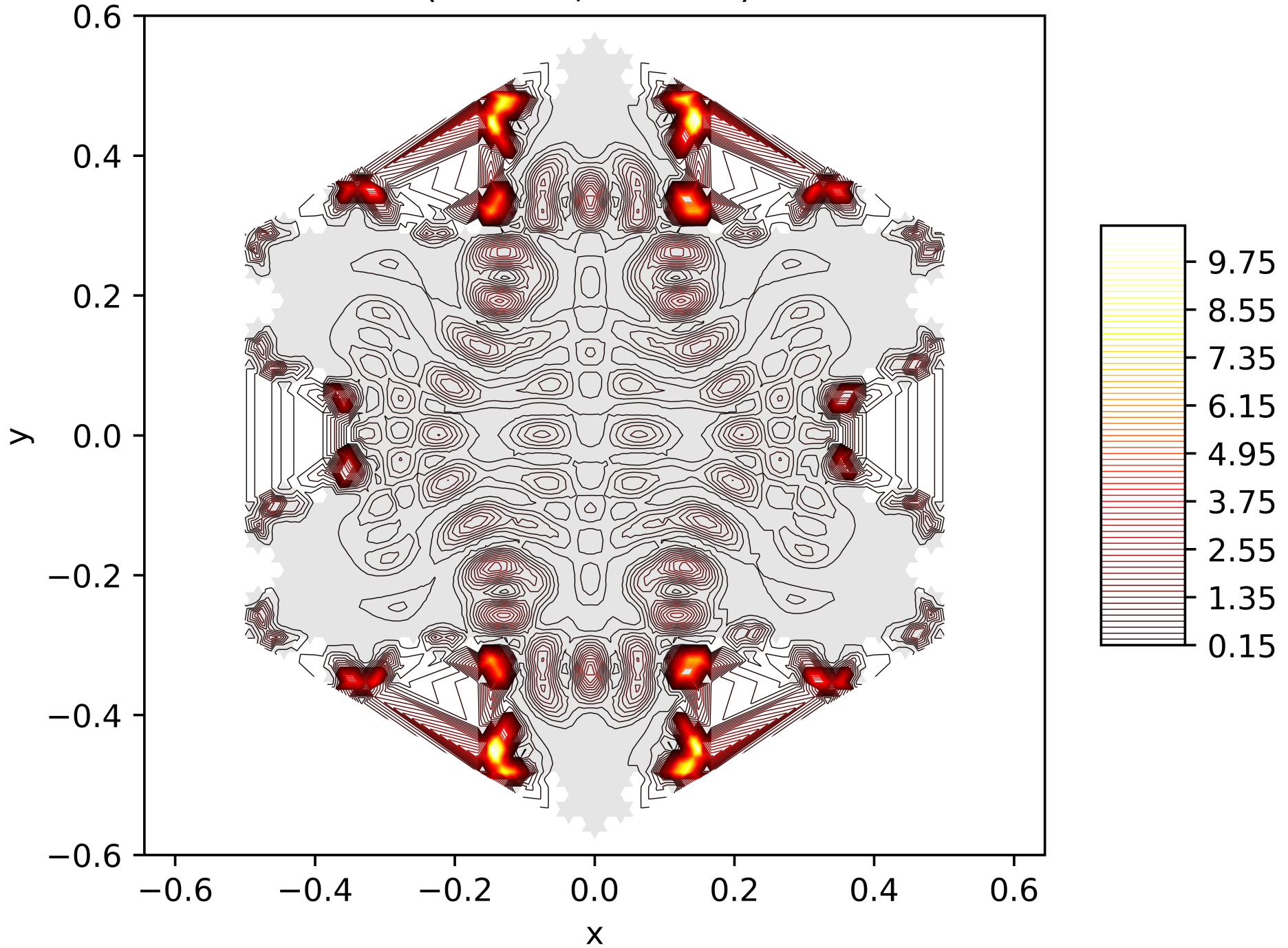
Contour Lines of the Energy Function of the 176. Eigenfunction on the Snowflake (Level 5, Res. 81) with Neumann BC
