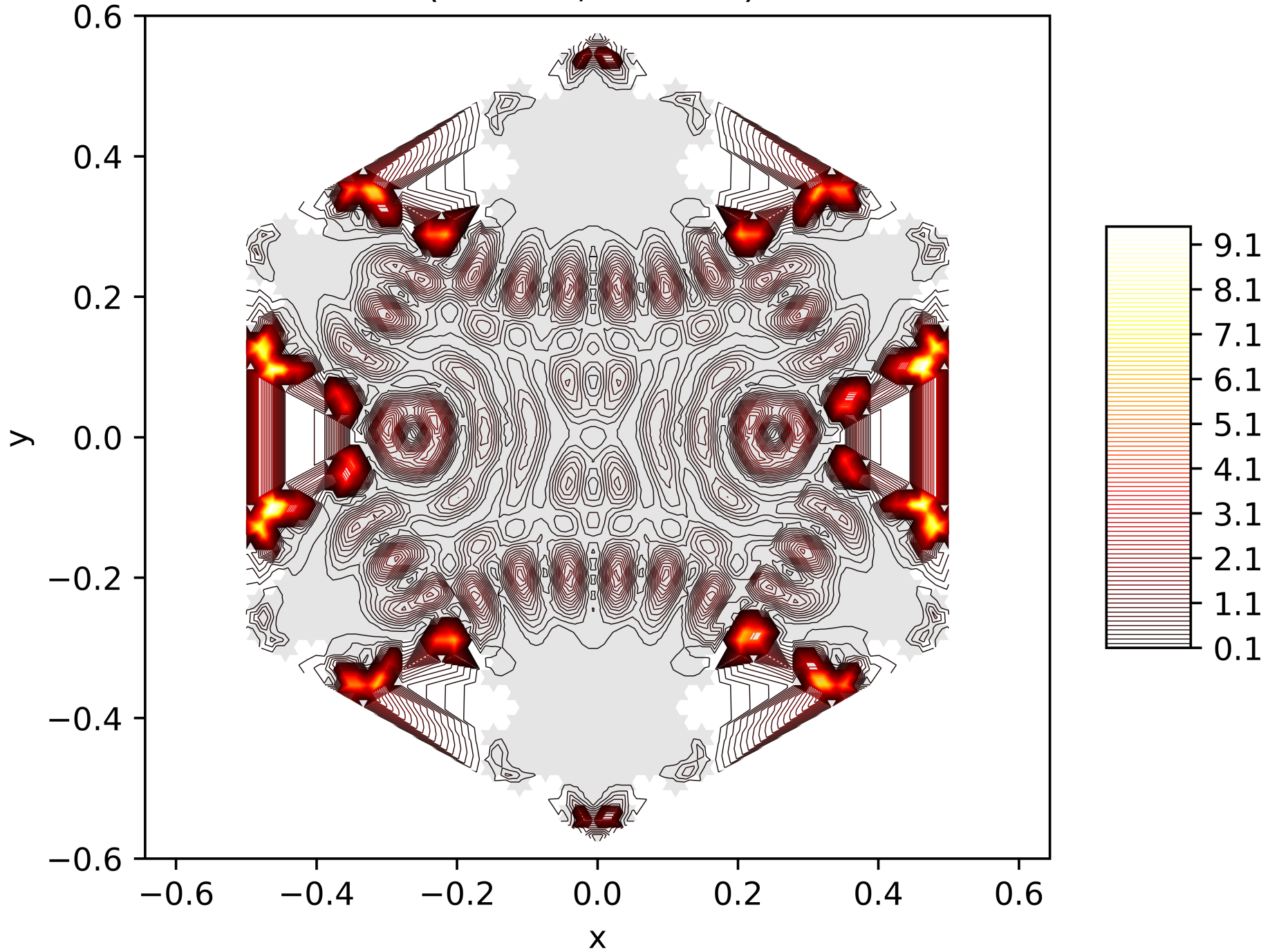
Contour Lines of the Energy Function of the 177. Eigenfunction on the Snowflake (Level 5, Res. 81) with Neumann BC
