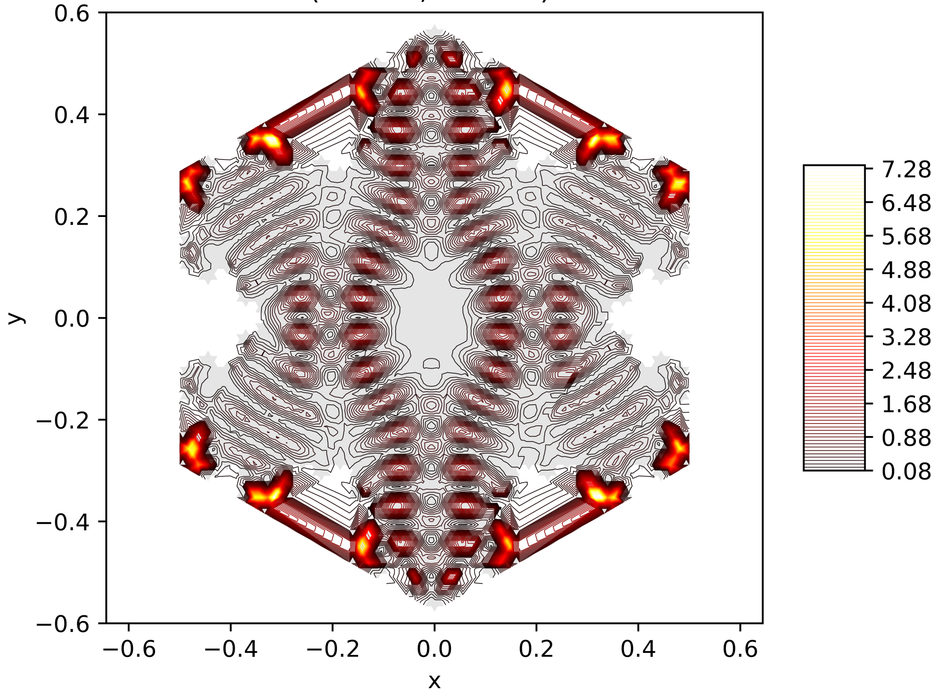
Contour Lines of the Energy Function of the 170. Eigenfunction on the Snowflake (Level 5, Res. 81) with Neumann BC
