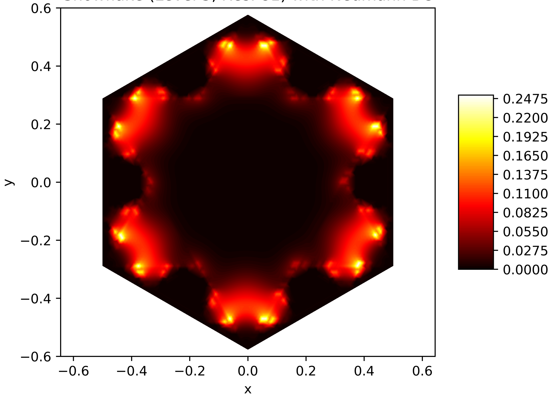
Energy Function of the 15. Eigenfunction on the Snowflake (Level 5, Res. 81) with Neumann BC
