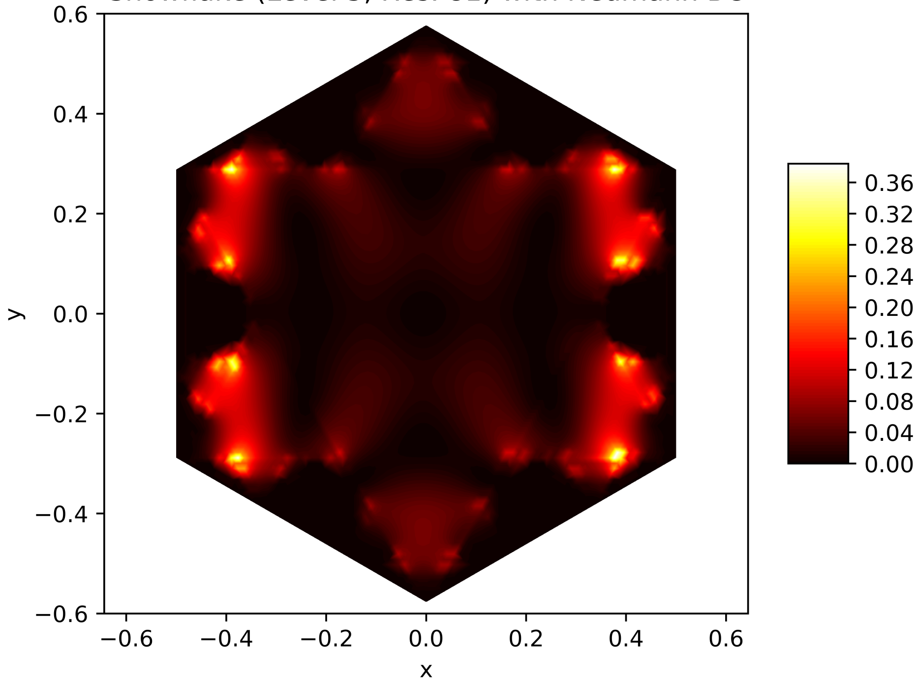
Energy Function of the 18. Eigenfunction on the Snowflake (Level 5, Res. 81) with Neumann BC
