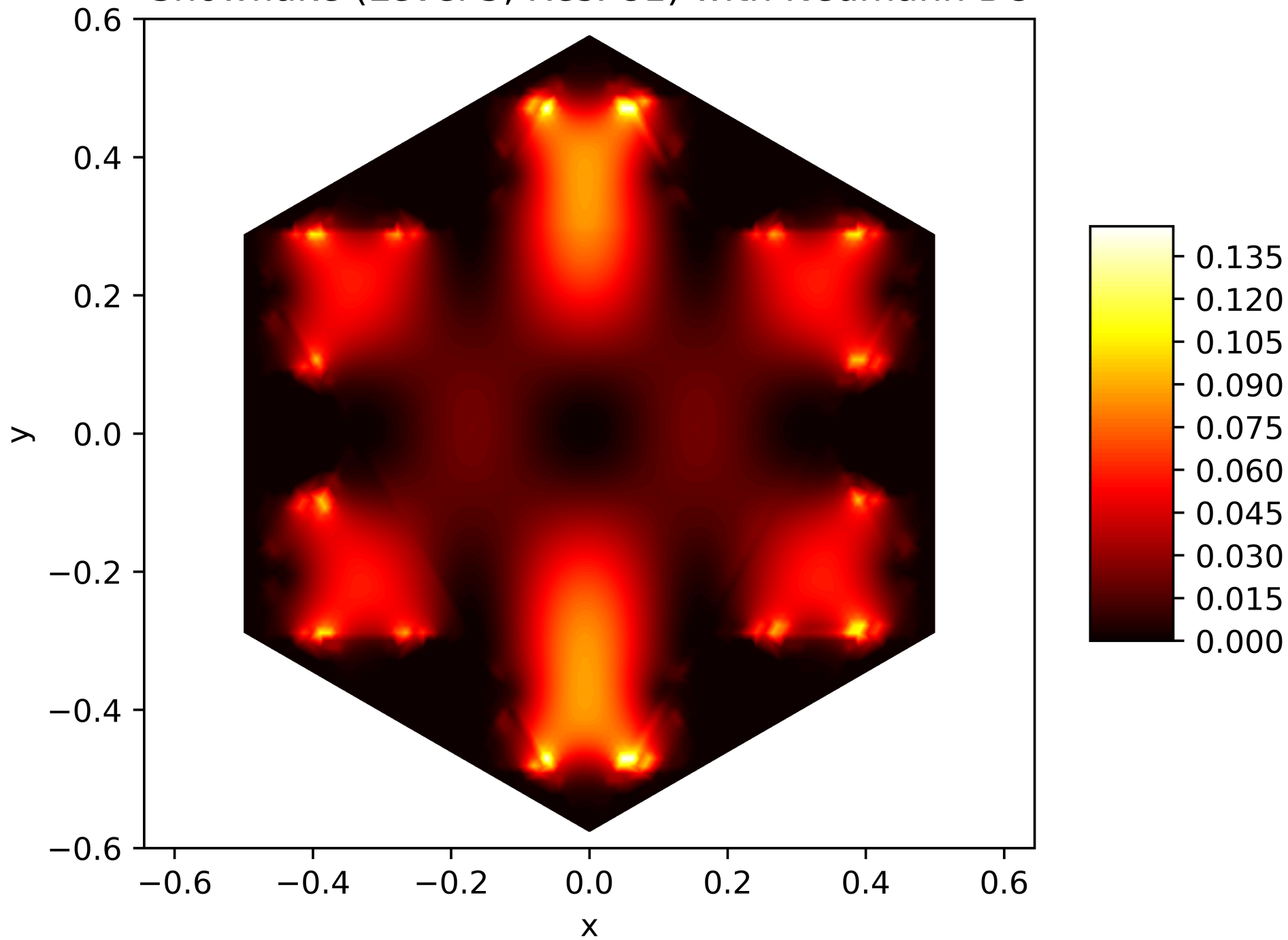
Energy Function of the 11. Eigenfunction on the Snowflake (Level 5, Res. 81) with Neumann BC
