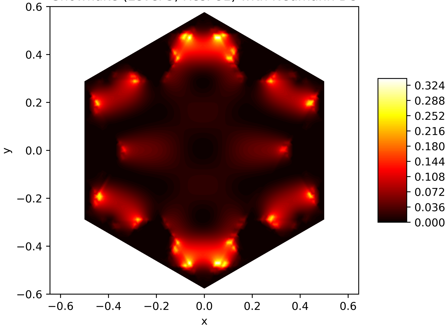
Energy Function of the 17. Eigenfunction on the Snowflake (Level 5, Res. 81) with Neumann BC
