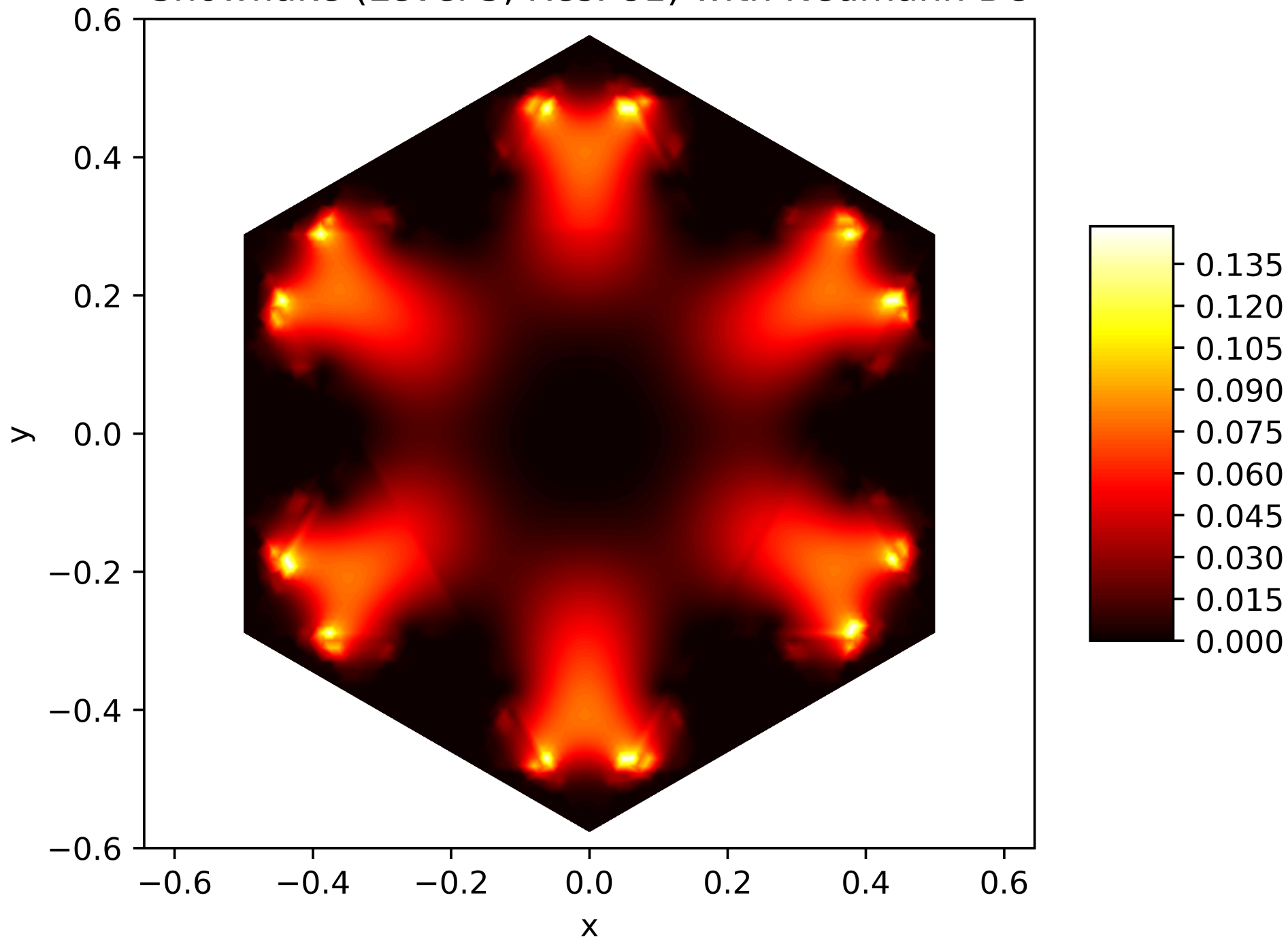
Energy Function of the 12. Eigenfunction on the Snowflake (Level 5, Res. 81) with Neumann BC
