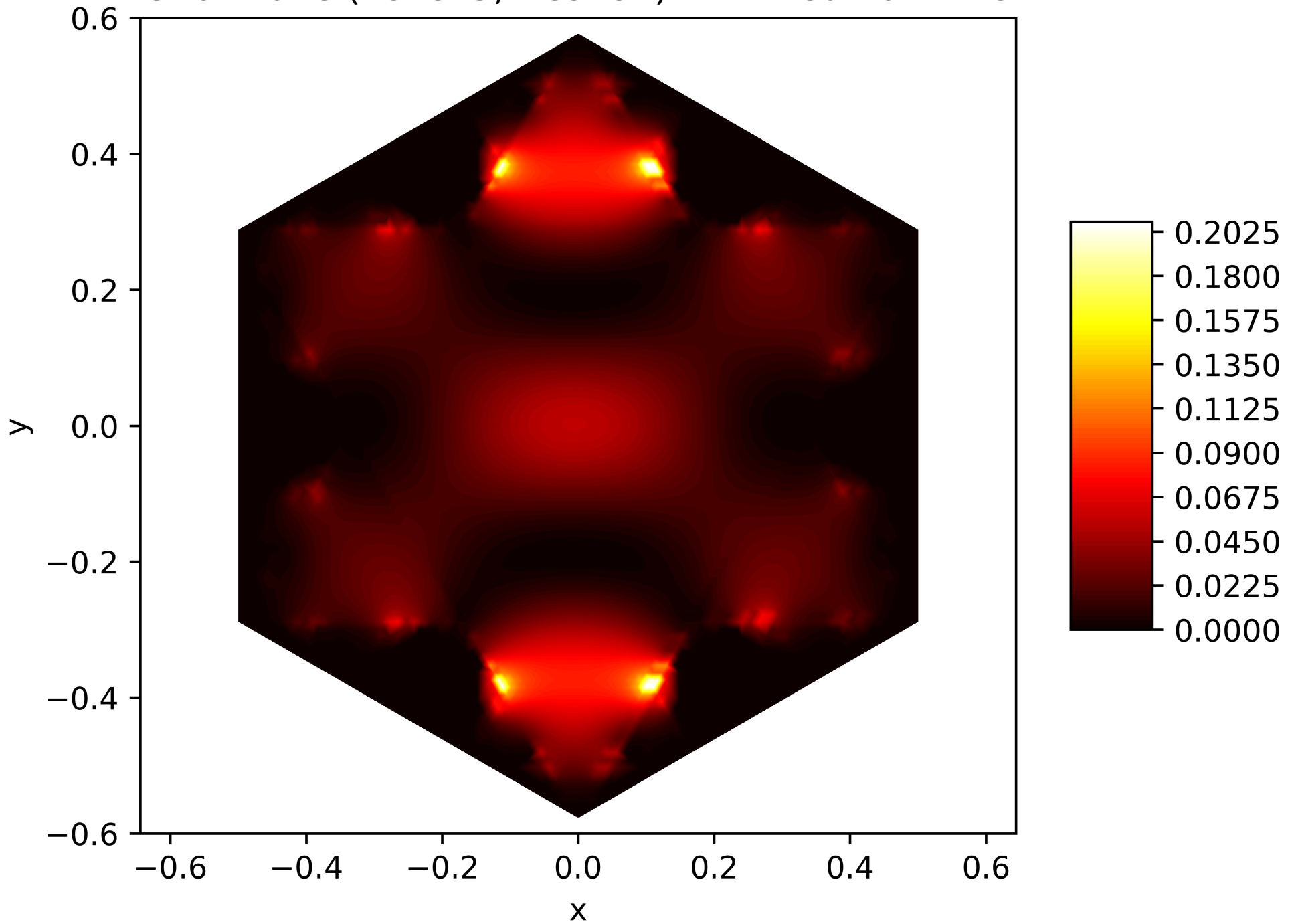
Energy Function of the 8. Eigenfunction on the Snowflake (Level 5, Res. 81) with Neumann BC
