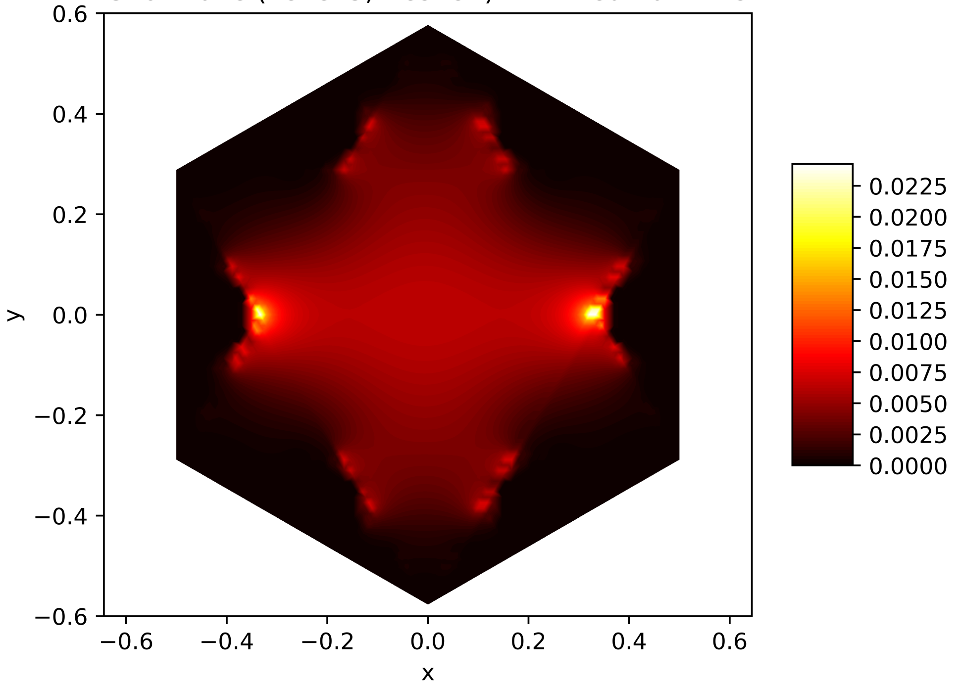
Energy Function of the 2. Eigenfunction on the Snowflake (Level 5, Res. 81) with Neumann BC
