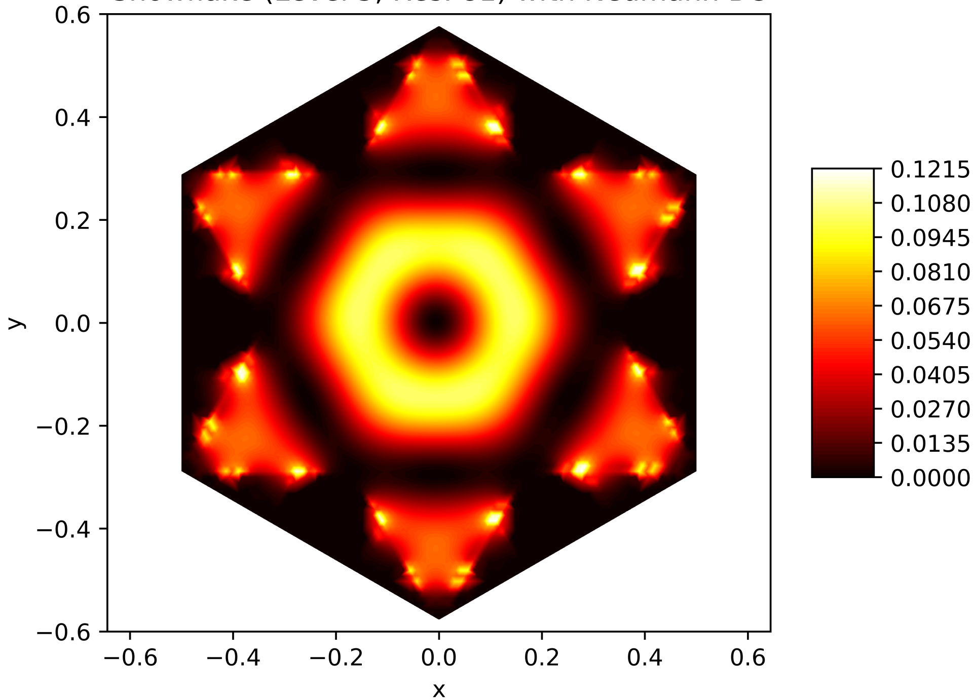
Energy Function of the 16. Eigenfunction on the Snowflake (Level 5, Res. 81) with Neumann BC
