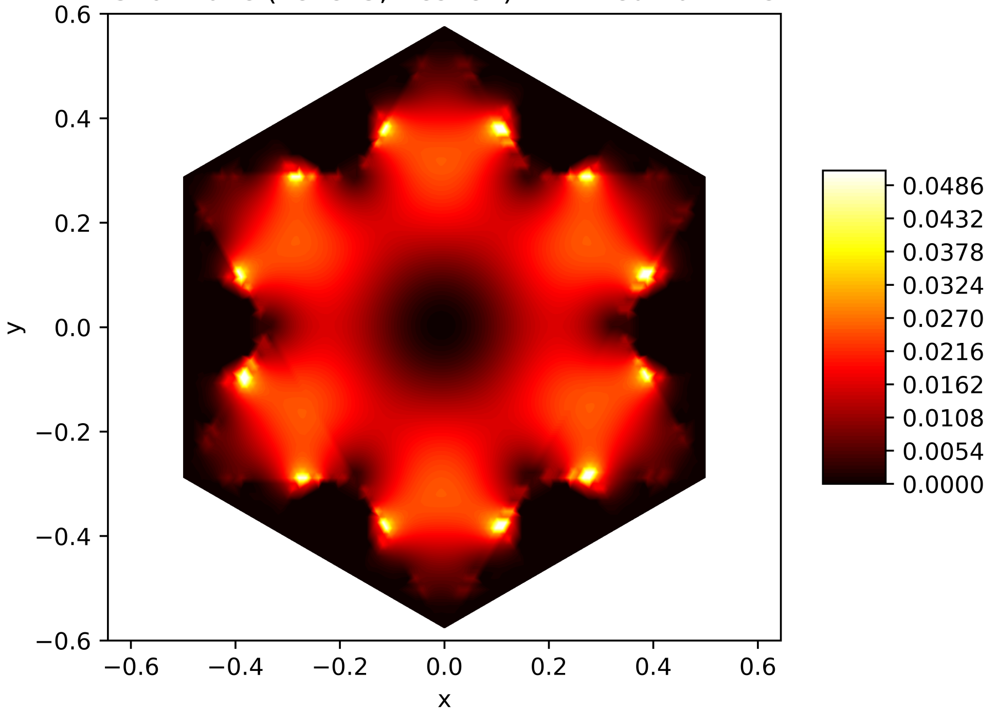
Energy Function of the 7. Eigenfunction on the Snowflake (Level 5, Res. 81) with Neumann BC
