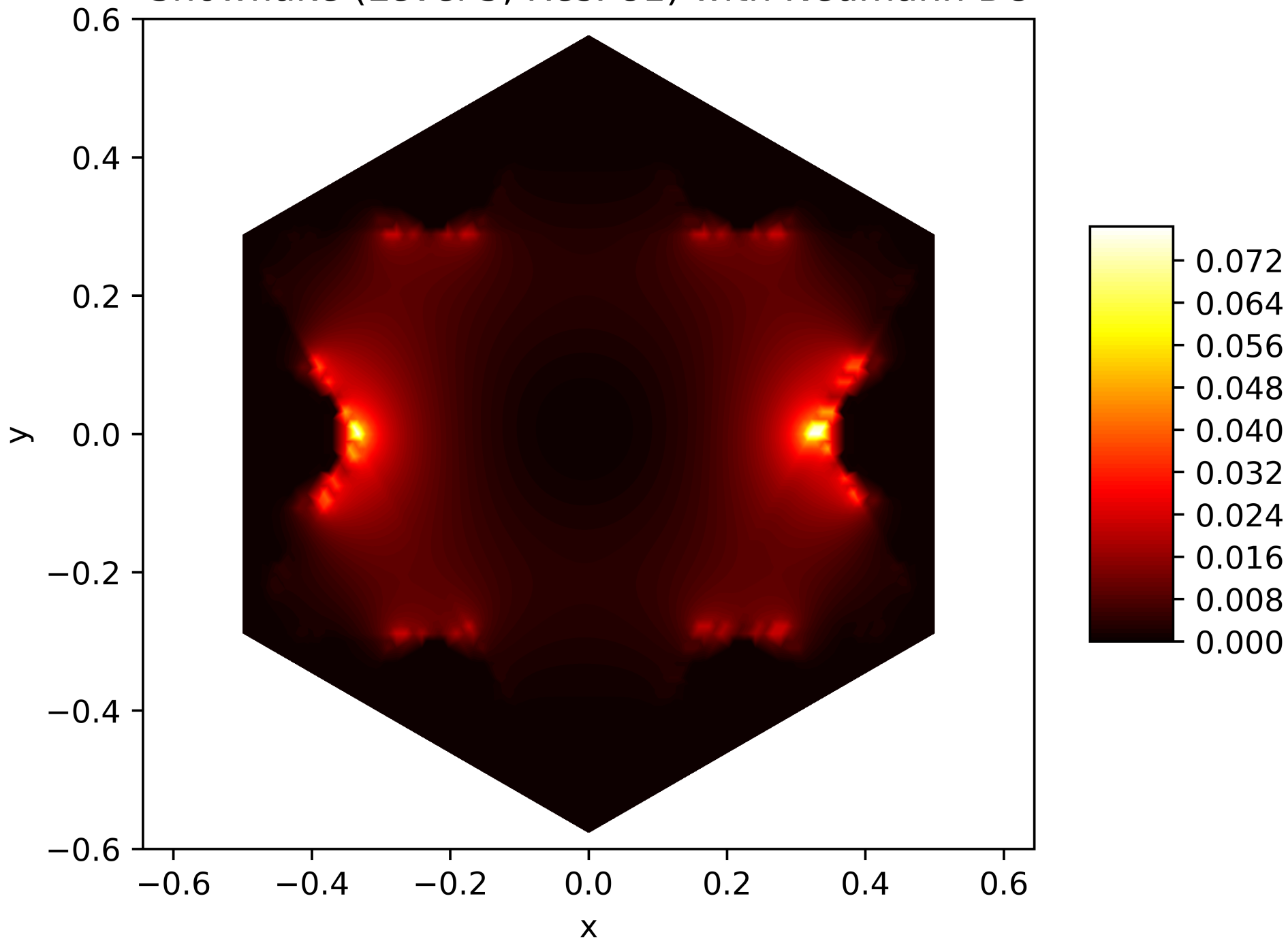
Energy Function of the 5. Eigenfunction on the Snowflake (Level 5, Res. 81) with Neumann BC
