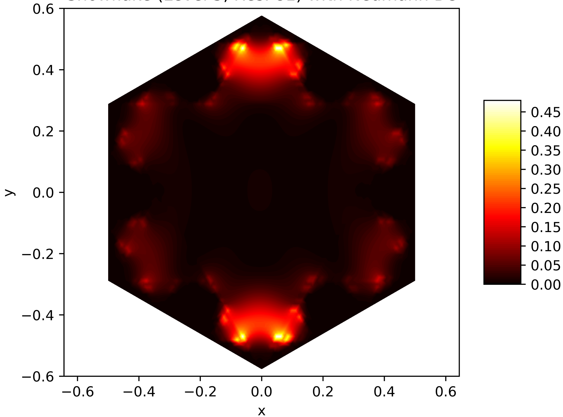
Energy Function of the 13. Eigenfunction on the Snowflake (Level 5, Res. 81) with Neumann BC
