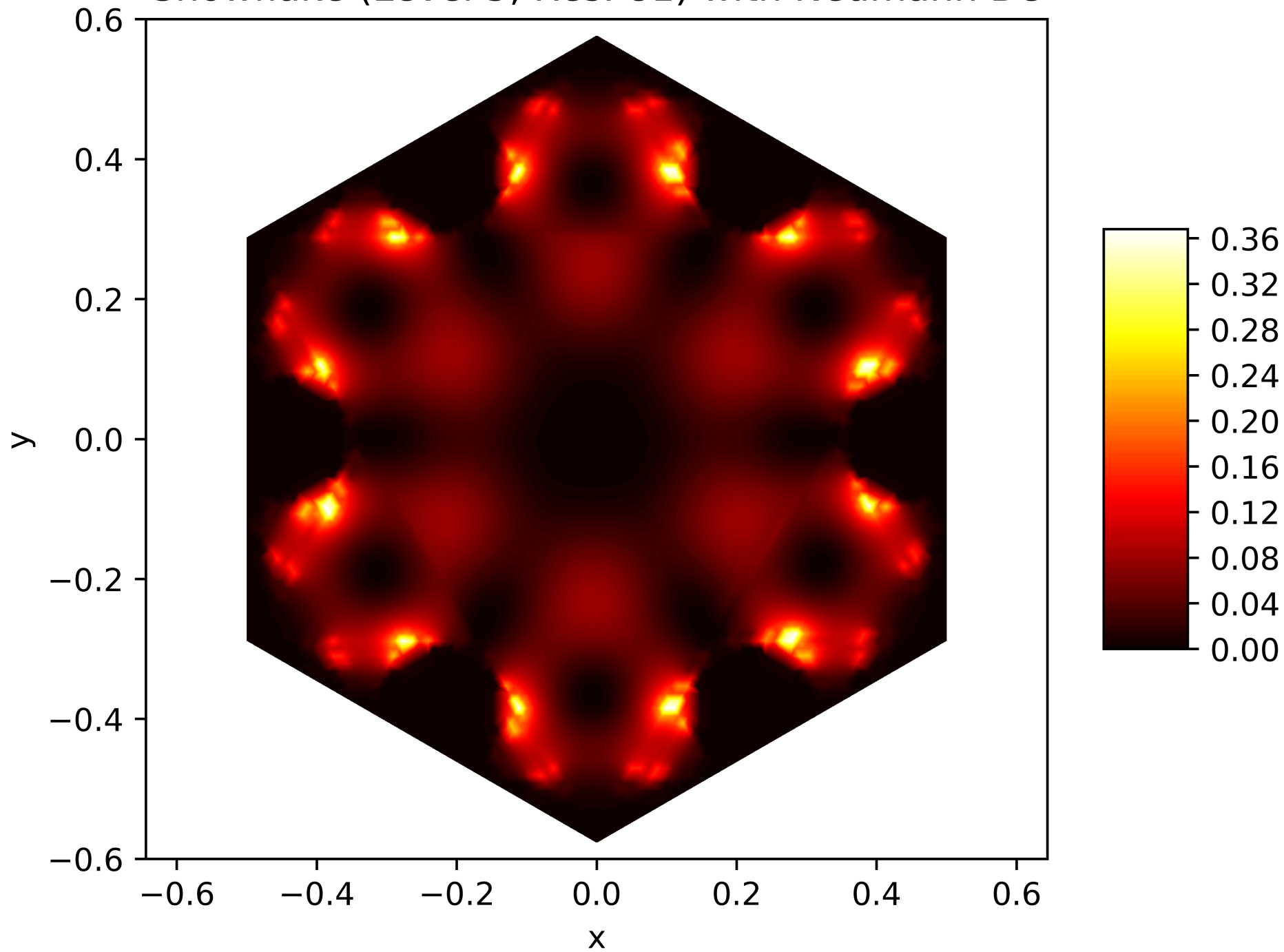
Energy Function of the 20. Eigenfunction on the Snowflake (Level 5, Res. 81) with Neumann BC
