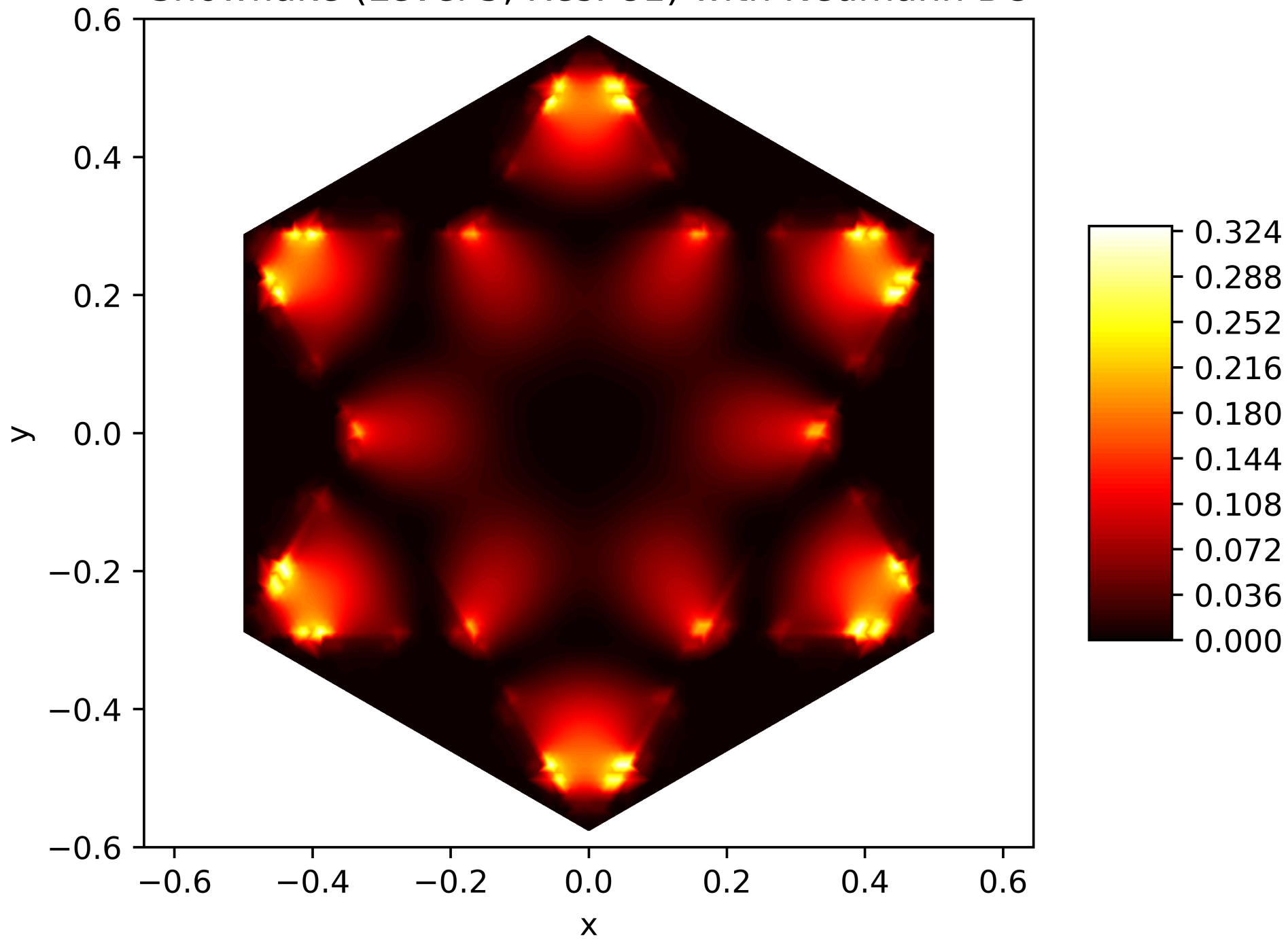
Energy Function of the 19. Eigenfunction on the Snowflake (Level 5, Res. 81) with Neumann BC
