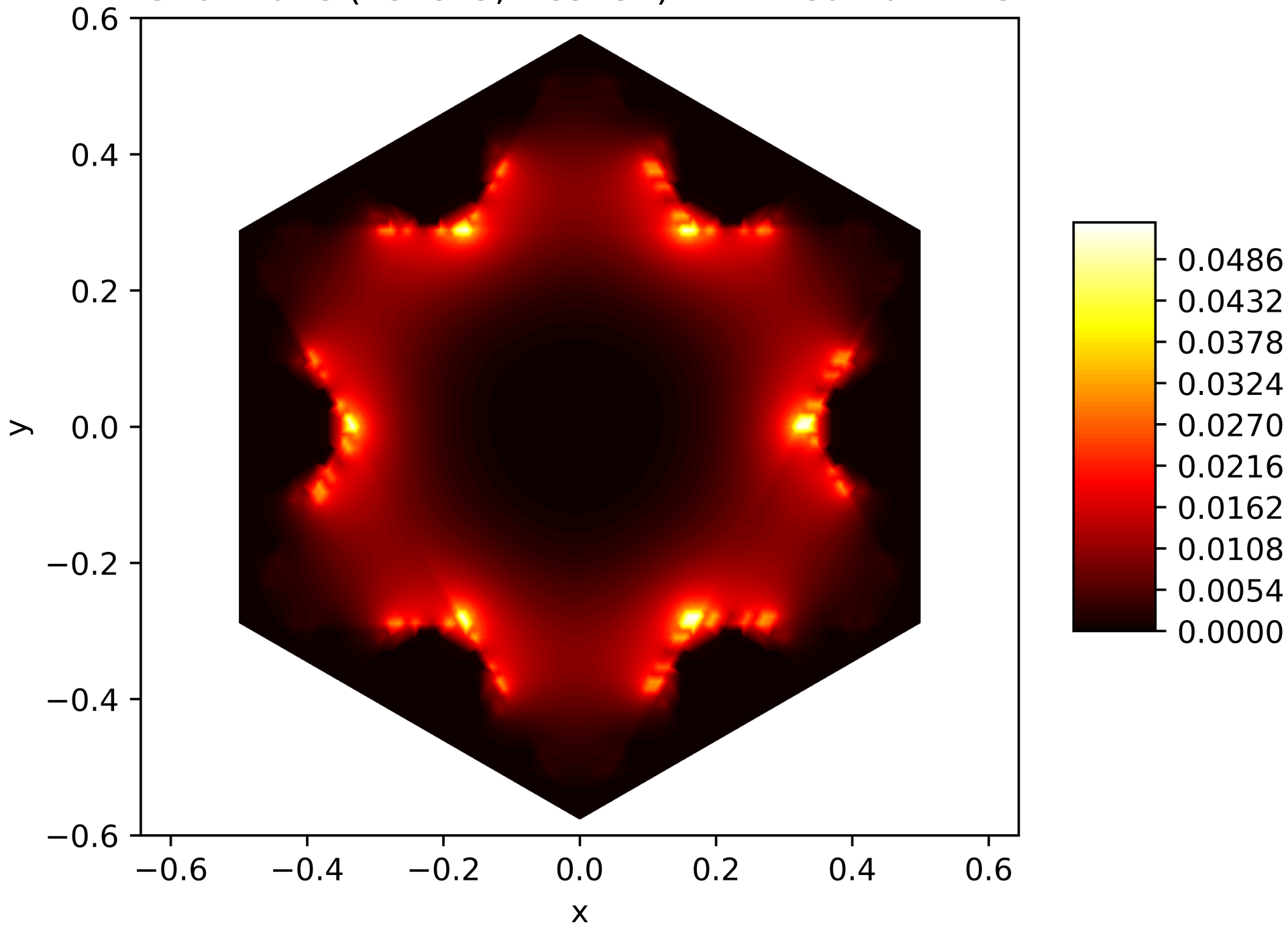
Energy Function of the 6. Eigenfunction on the Snowflake (Level 5, Res. 81) with Neumann BC
