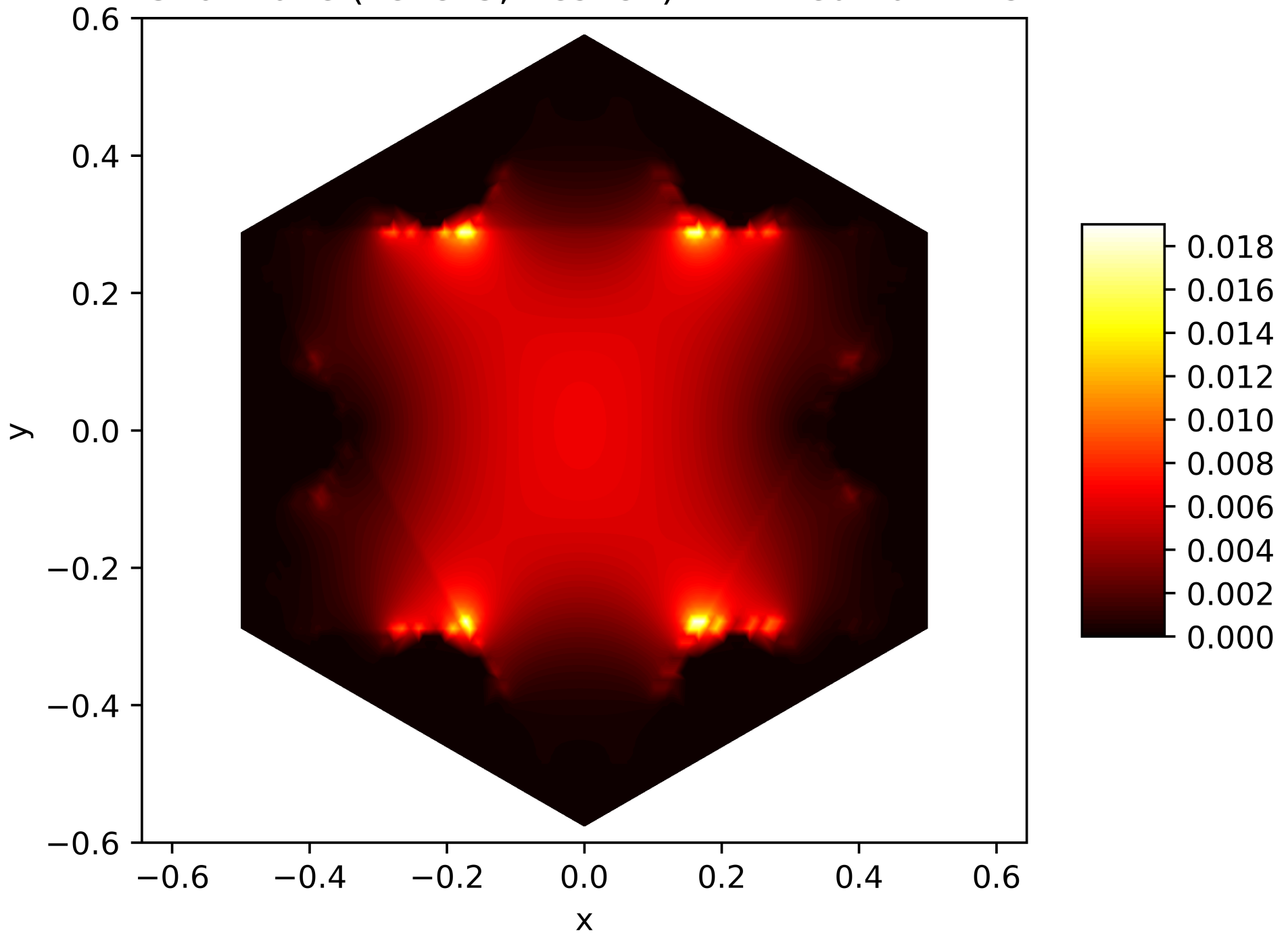
Energy Function of the 3. Eigenfunction on the Snowflake (Level 5, Res. 81) with Neumann BC
