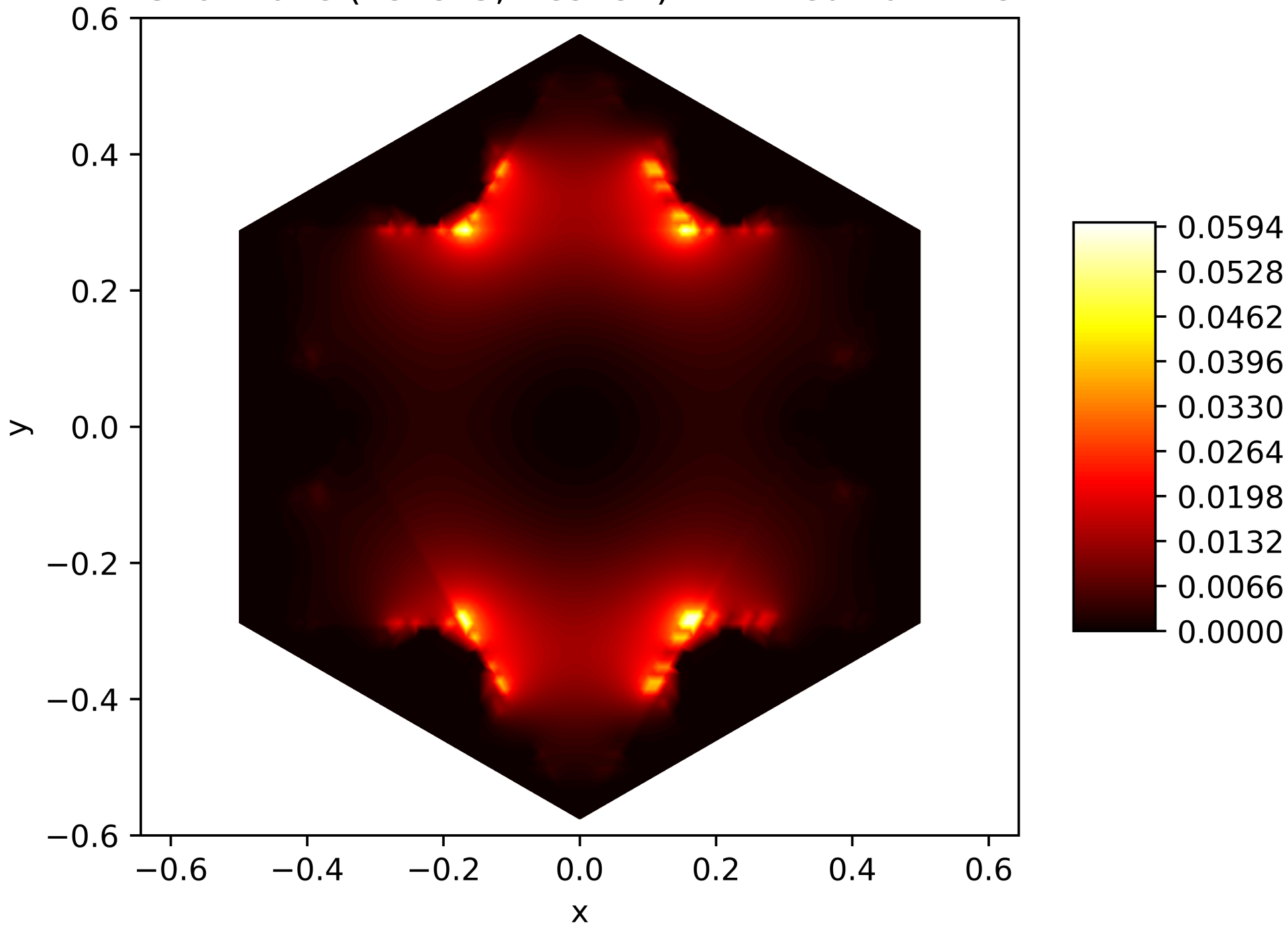
Energy Function of the 4. Eigenfunction on the Snowflake (Level 5, Res. 81) with Neumann BC
