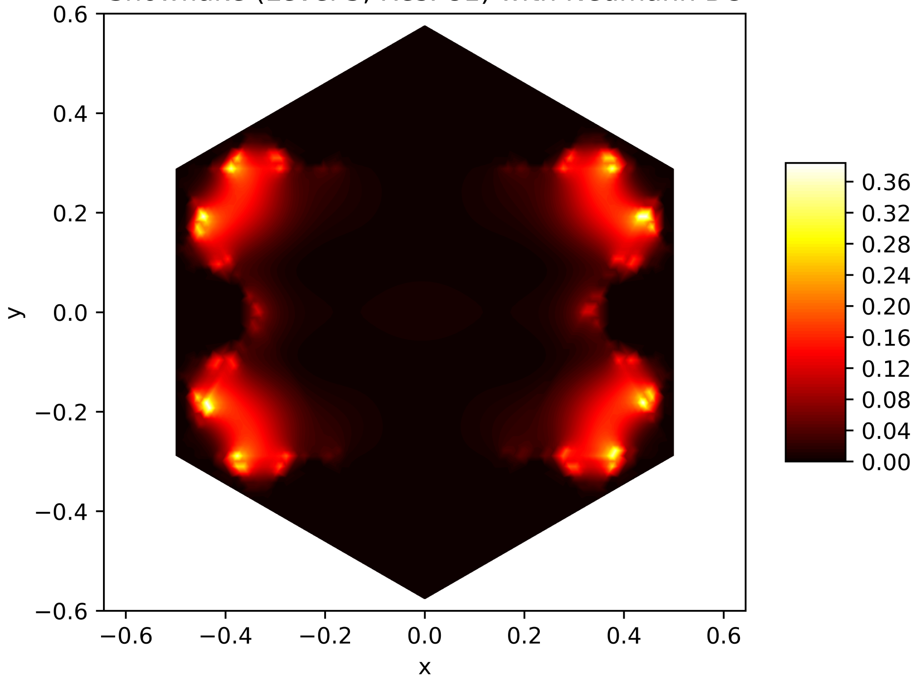
Energy Function of the 14. Eigenfunction on the Snowflake (Level 5, Res. 81) with Neumann BC
