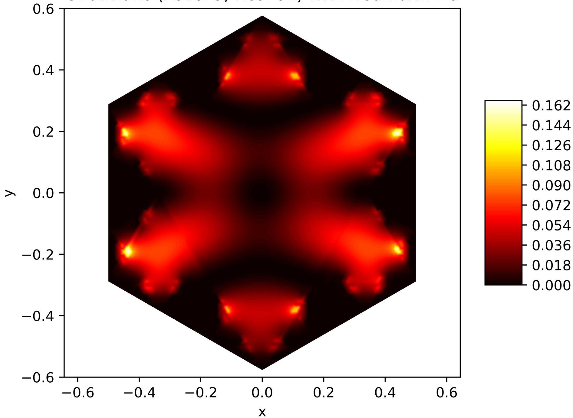
Energy Function of the 10. Eigenfunction on the Snowflake (Level 5, Res. 81) with Neumann BC
