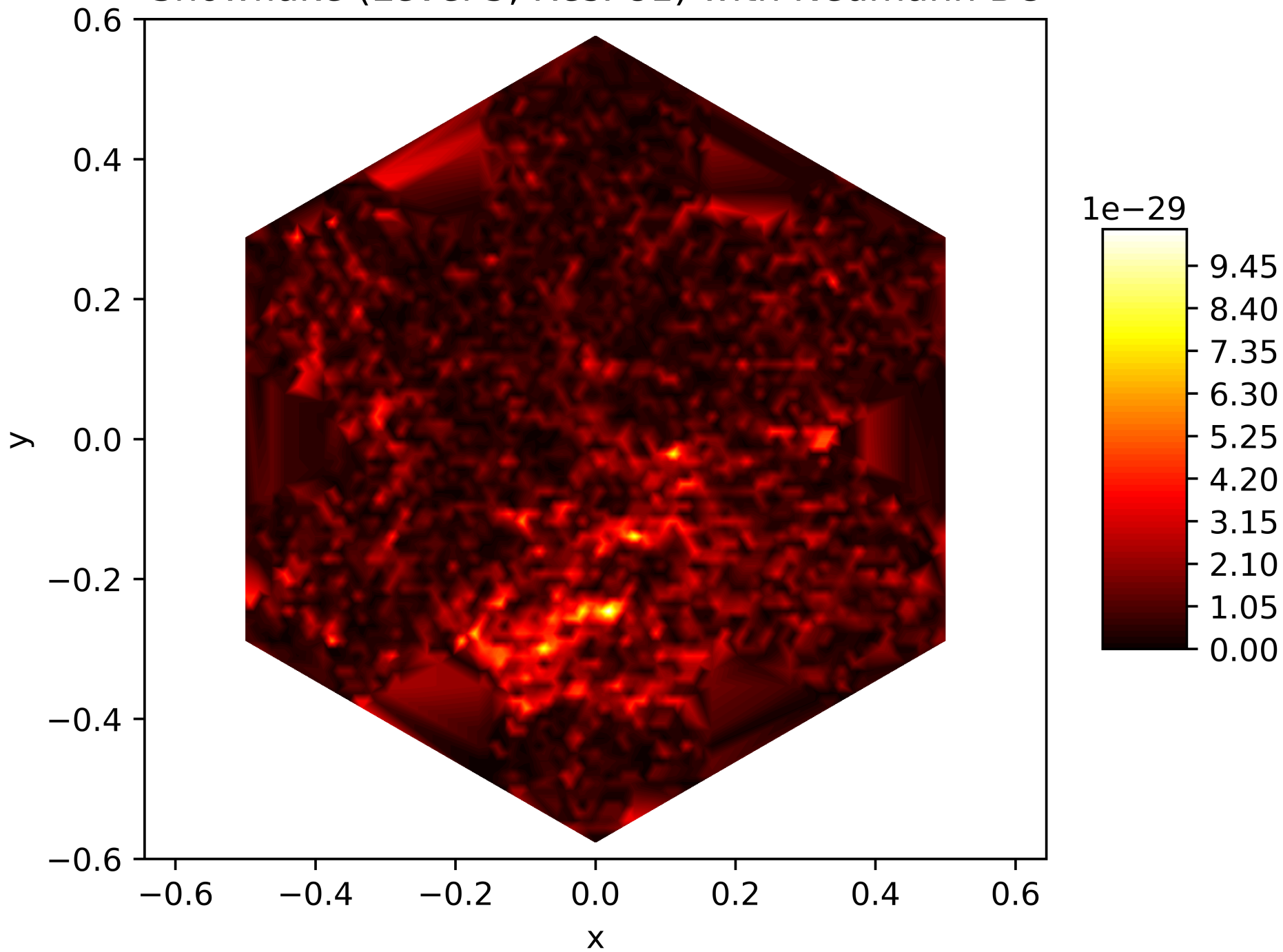
Energy Function of the 1. Eigenfunction on the Snowflake (Level 5, Res. 81) with Neumann BC
