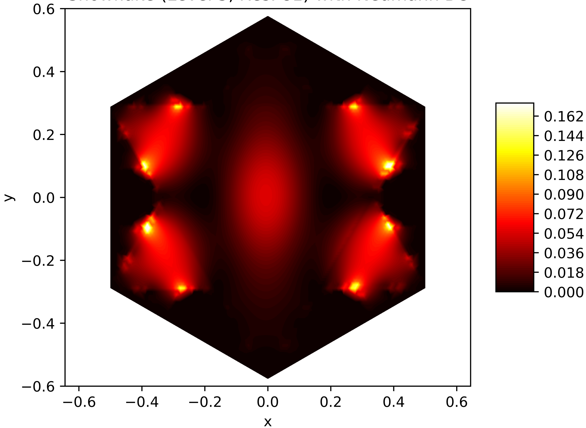
Energy Function of the 9. Eigenfunction on the Snowflake (Level 5, Res. 81) with Neumann BC
