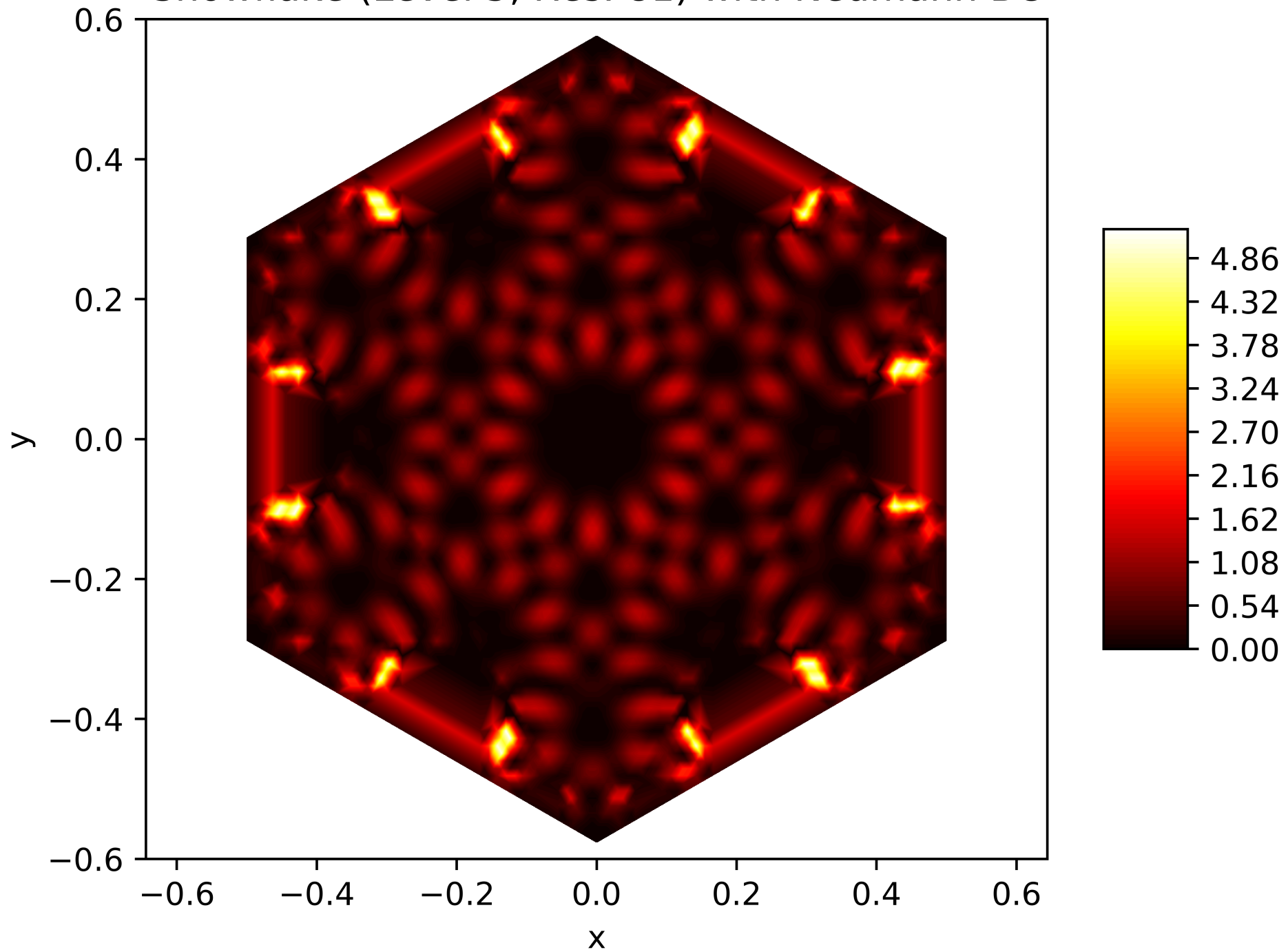
Energy Function of the 193. Eigenfunction on the Snowflake (Level 5, Res. 81) with Neumann BC
