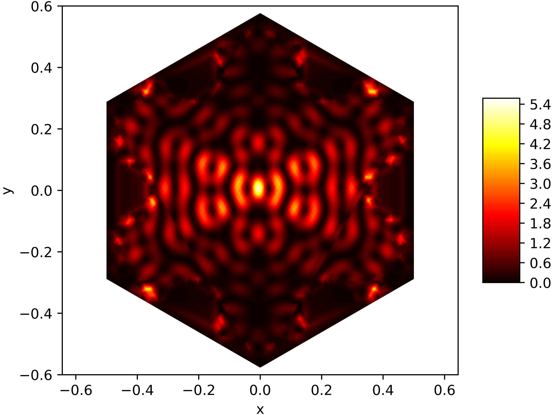
Energy Function of the 197. Eigenfunction on the Snowflake (Level 5, Res. 81) with Neumann BC
