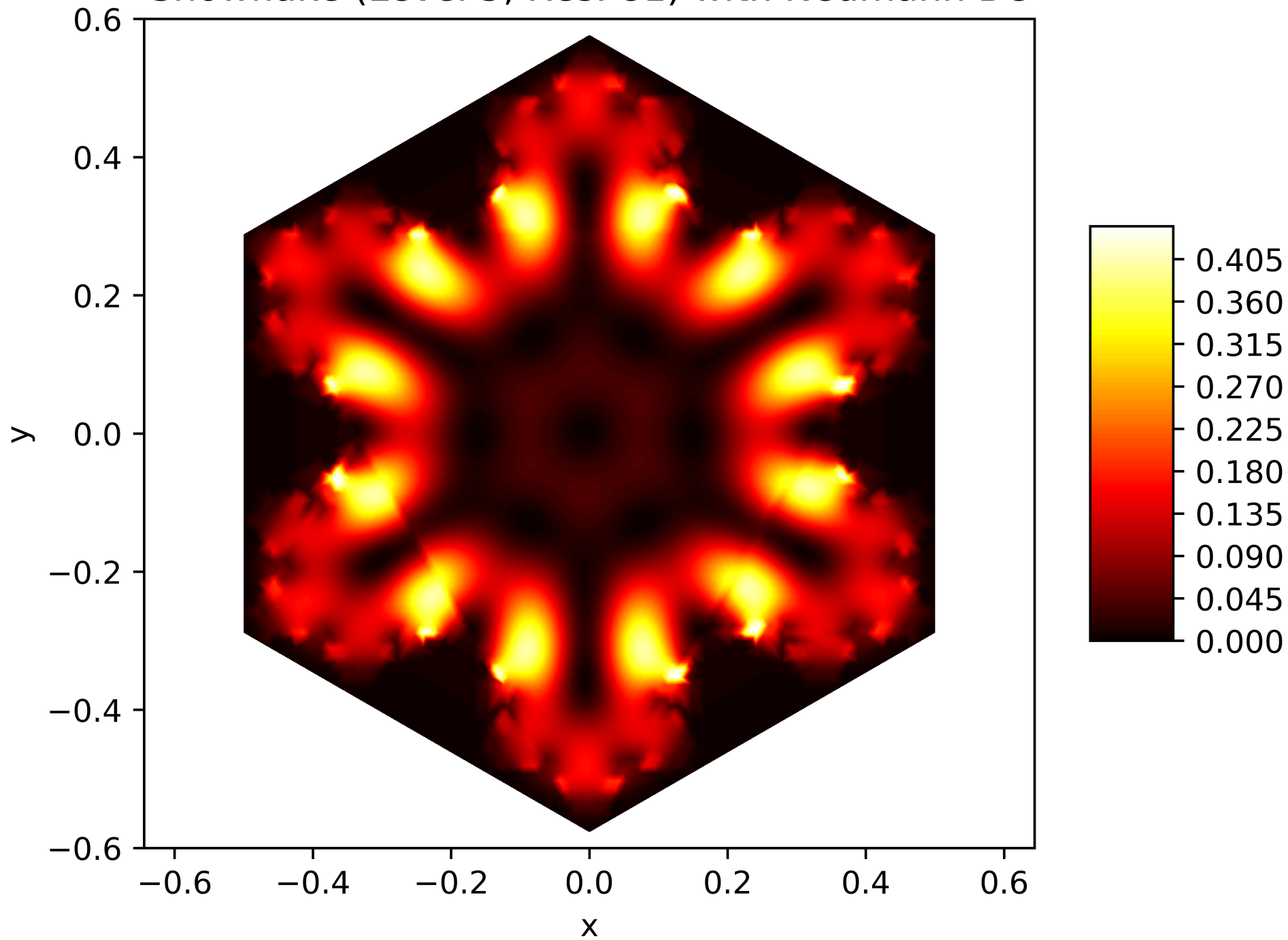
Energy Function of the 38. Eigenfunction on the Snowflake (Level 5, Res. 81) with Neumann BC
