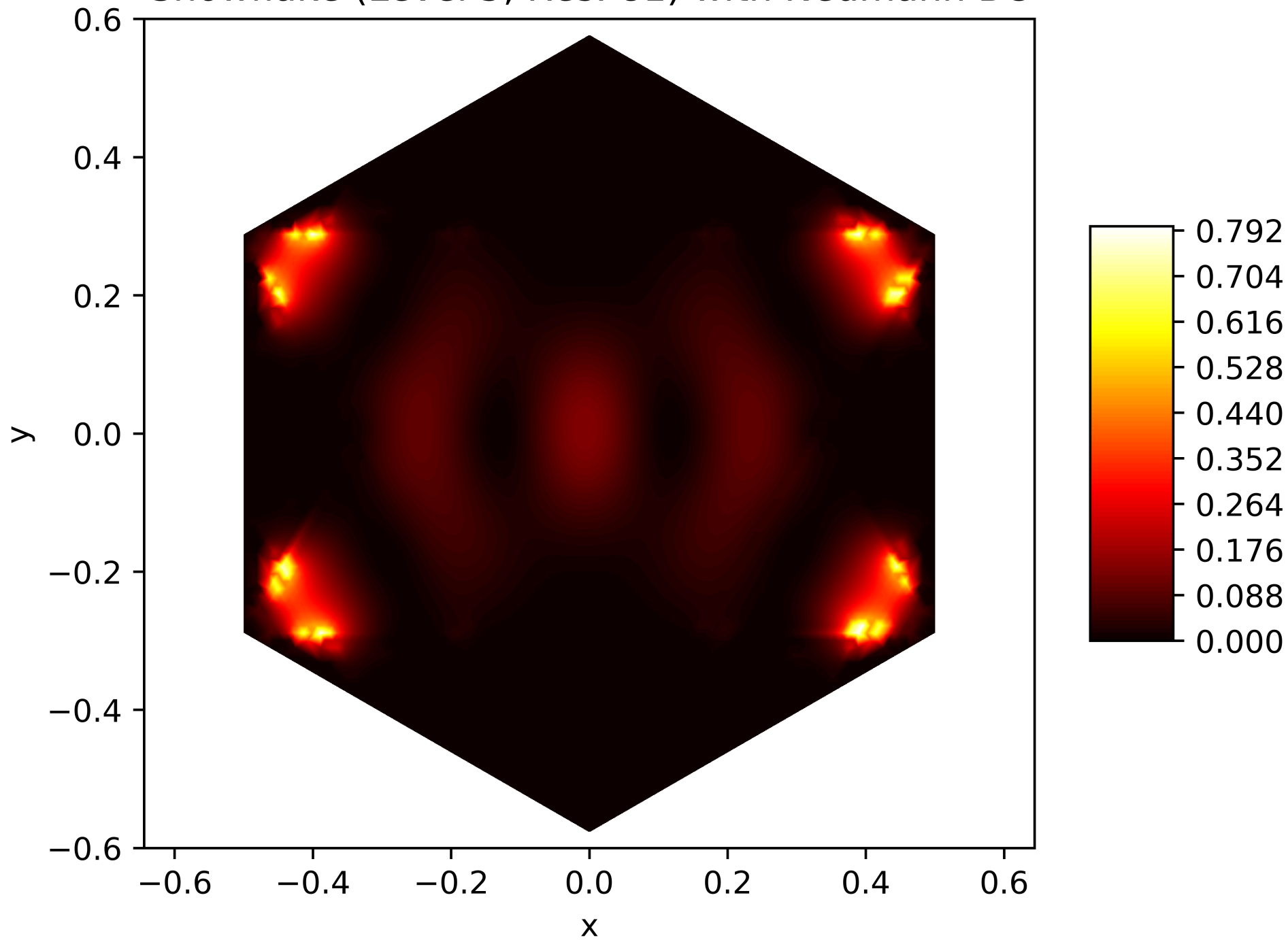
Energy Function of the 22. Eigenfunction on the Snowflake (Level 5, Res. 81) with Neumann BC
