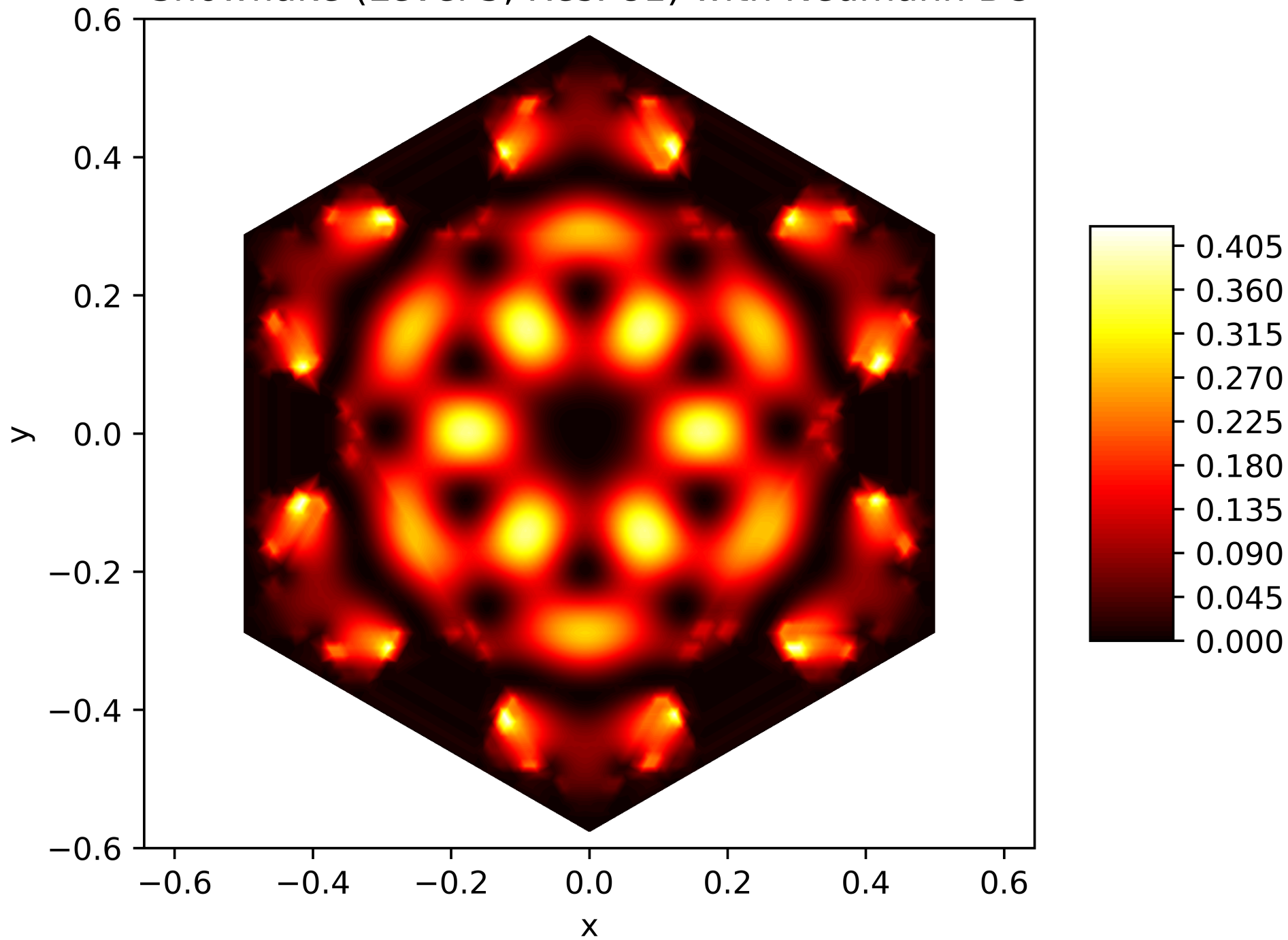
Energy Function of the 37. Eigenfunction on the Snowflake (Level 5, Res. 81) with Neumann BC
