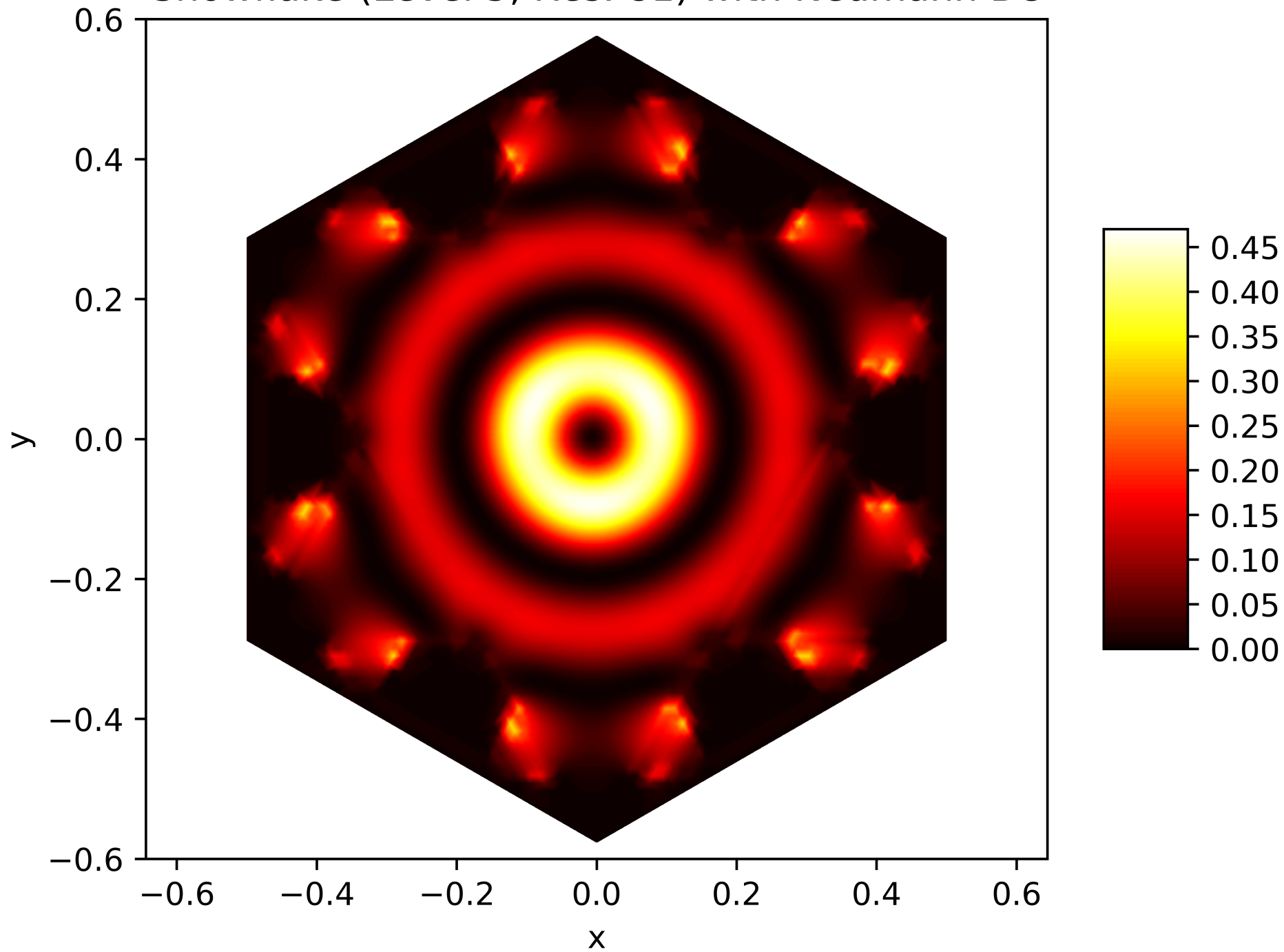
Energy Function of the 35. Eigenfunction on the Snowflake (Level 5, Res. 81) with Neumann BC
