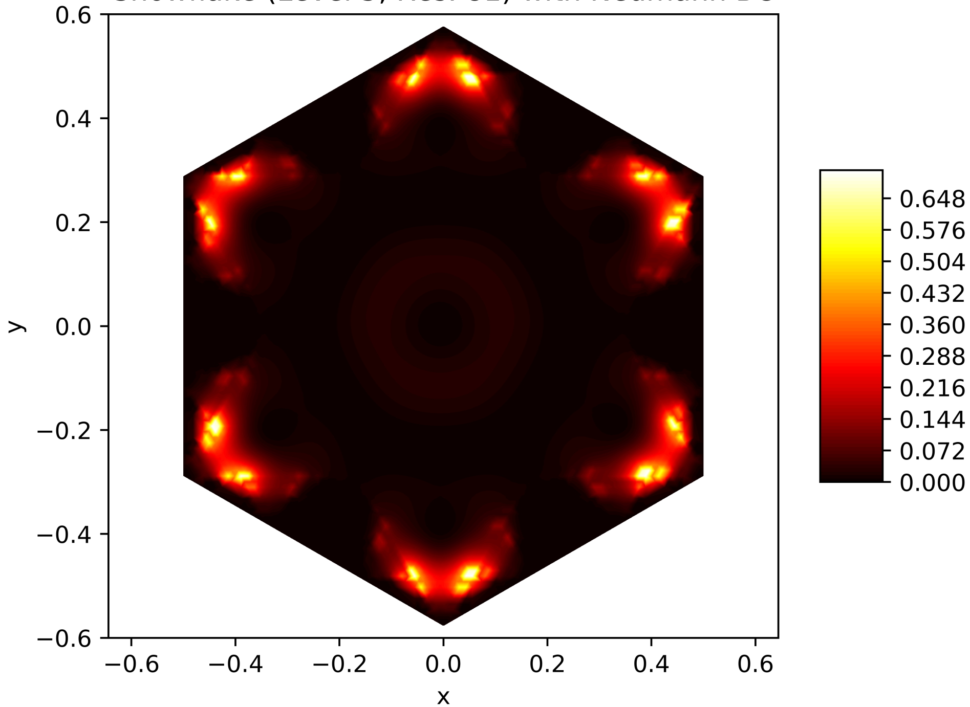
Energy Function of the 25. Eigenfunction on the Snowflake (Level 5, Res. 81) with Neumann BC
