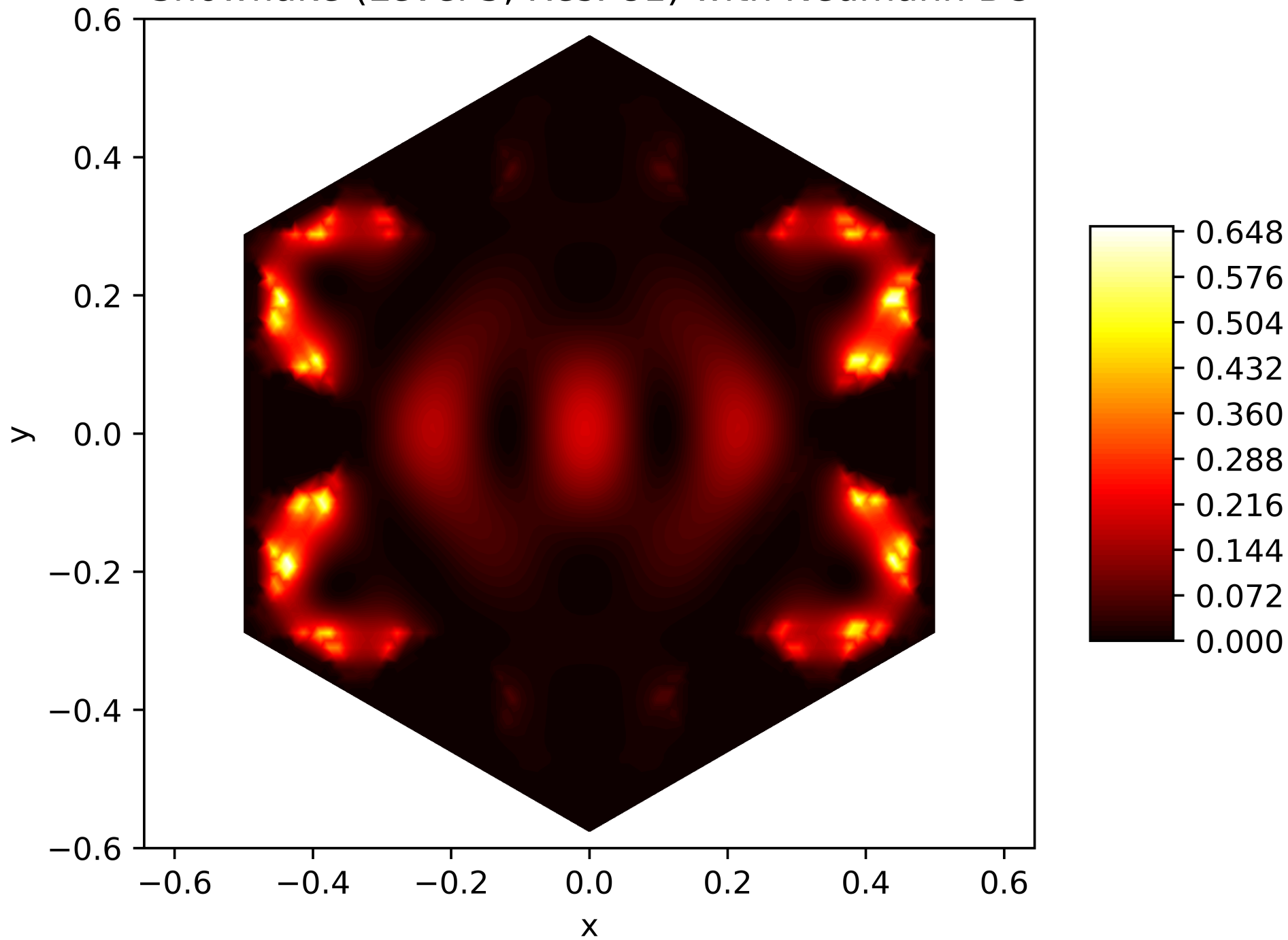
Energy Function of the 28. Eigenfunction on the Snowflake (Level 5, Res. 81) with Neumann BC
