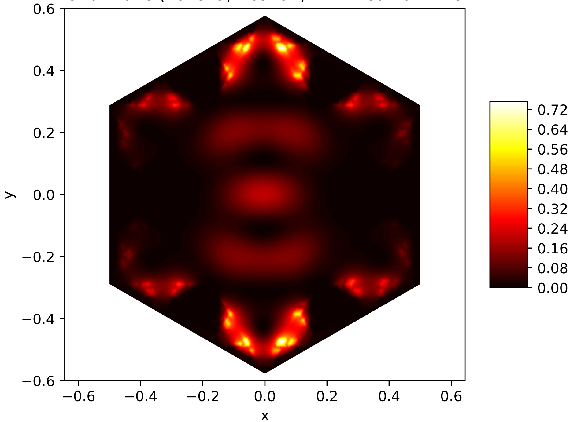
Energy Function of the 27. Eigenfunction on the Snowflake (Level 5, Res. 81) with Neumann BC
