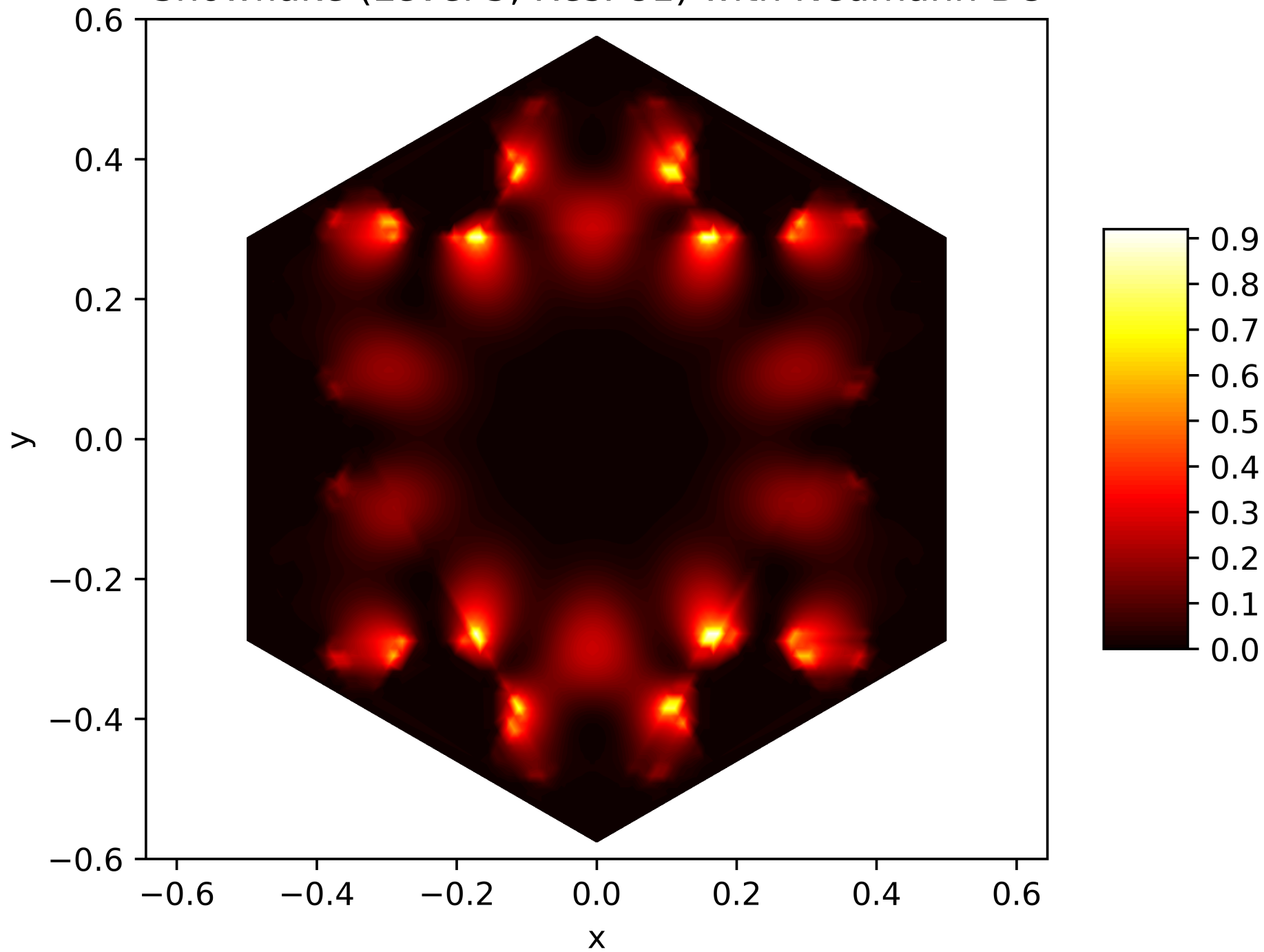
Energy Function of the 31. Eigenfunction on the Snowflake (Level 5, Res. 81) with Neumann BC
