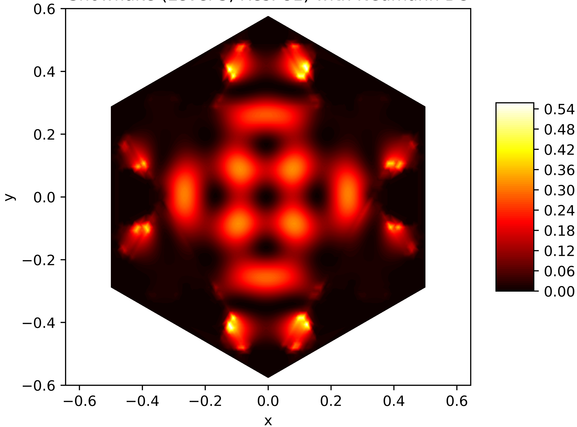
Energy Function of the 33. Eigenfunction on the Snowflake (Level 5, Res. 81) with Neumann BC
