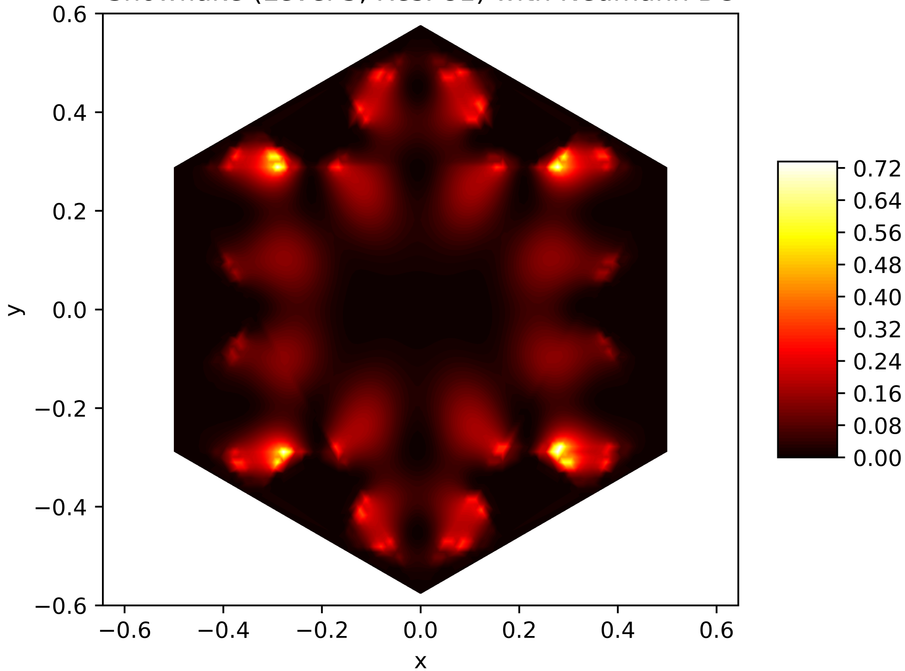
Energy Function of the 29. Eigenfunction on the Snowflake (Level 5, Res. 81) with Neumann BC
