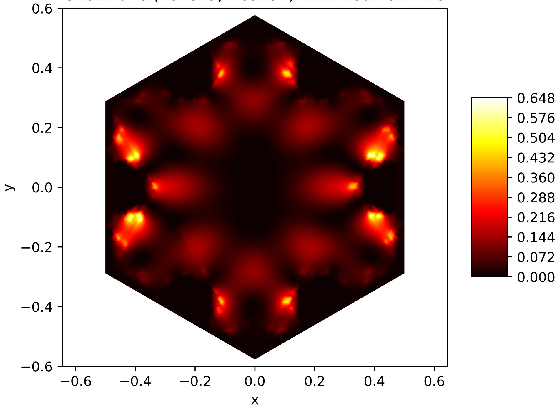
Energy Function of the 30. Eigenfunction on the Snowflake (Level 5, Res. 81) with Neumann BC
