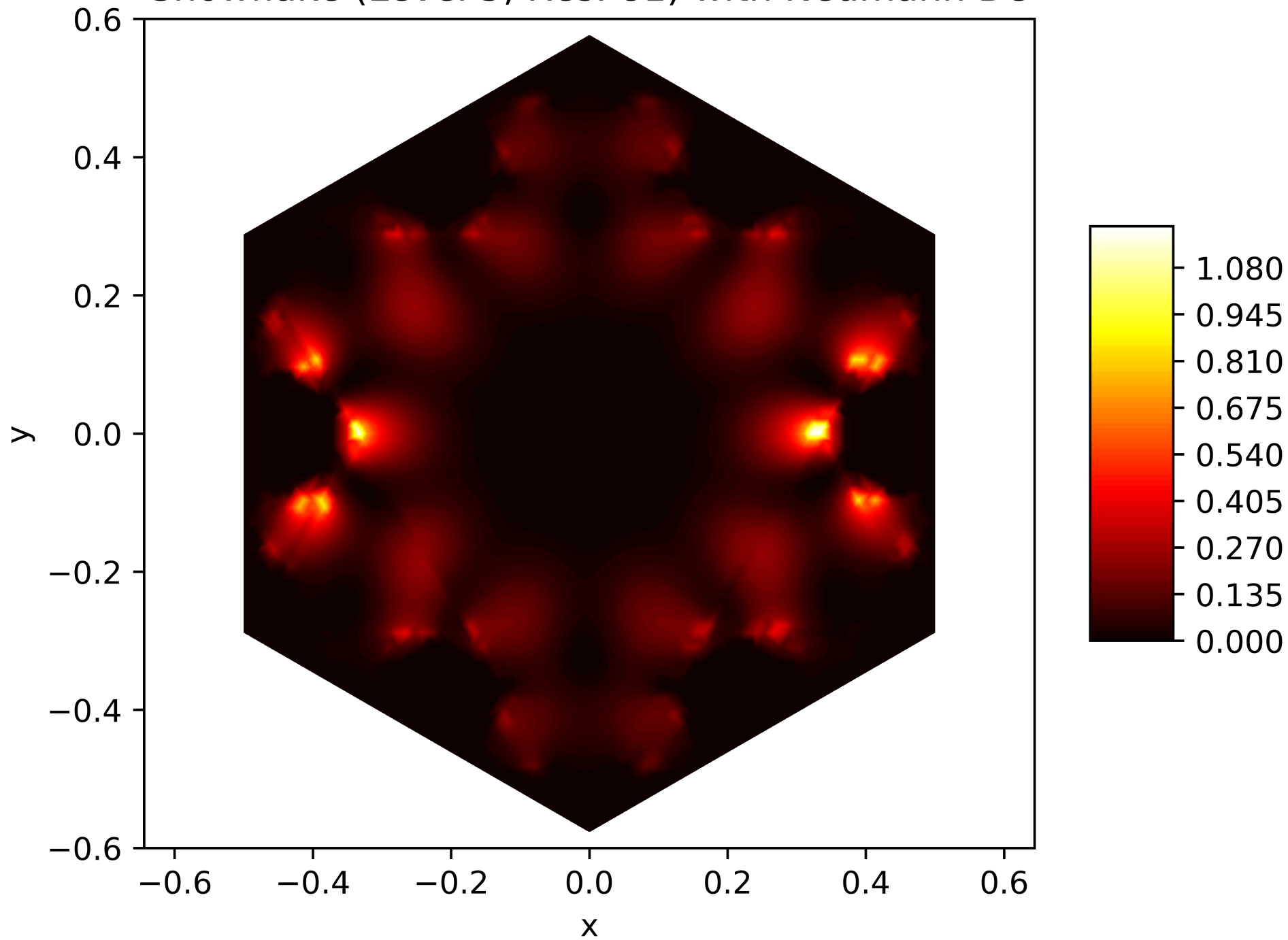
Energy Function of the 32. Eigenfunction on the Snowflake (Level 5, Res. 81) with Neumann BC
