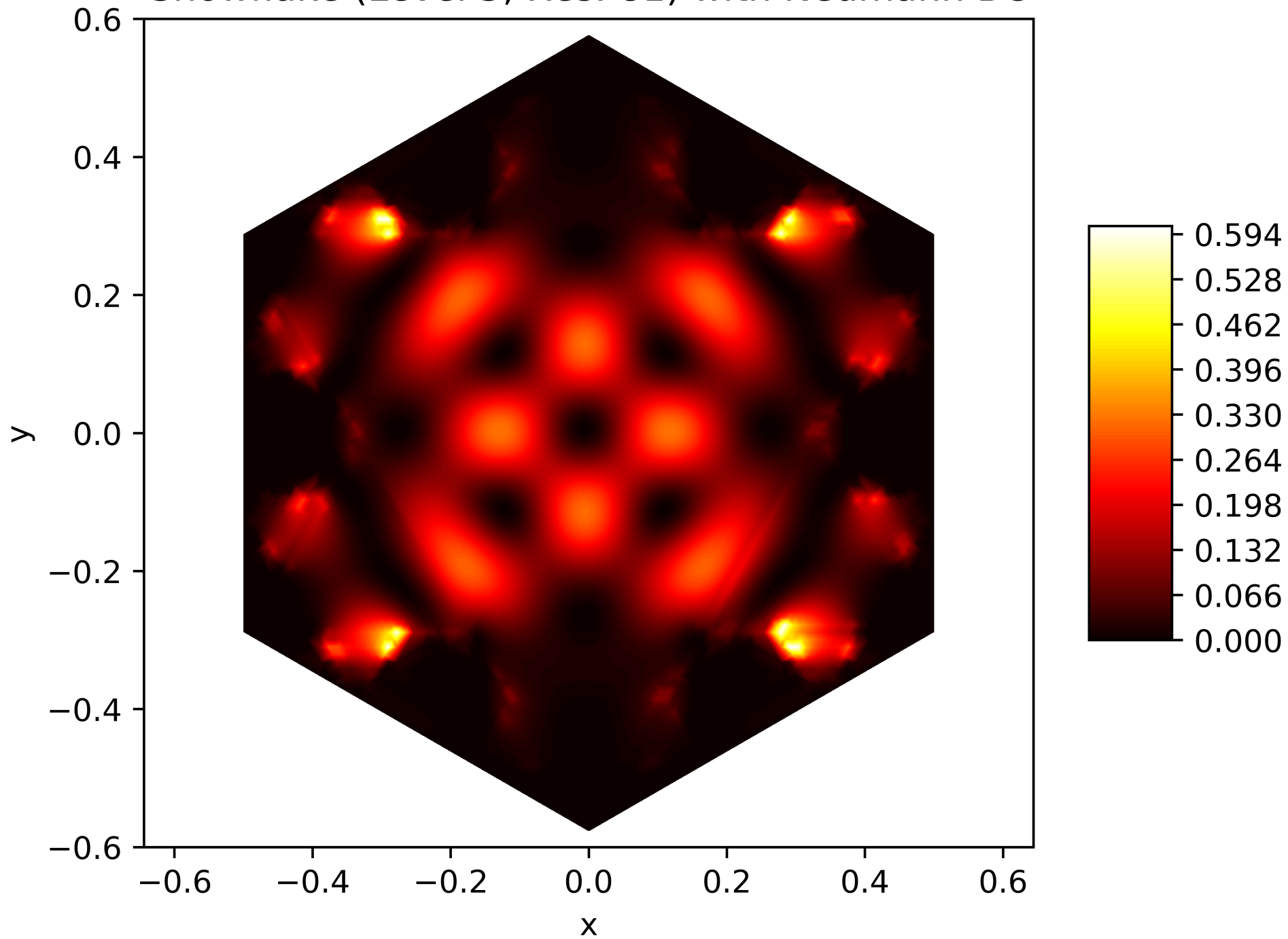
Energy Function of the 34. Eigenfunction on the Snowflake (Level 5, Res. 81) with Neumann BC
