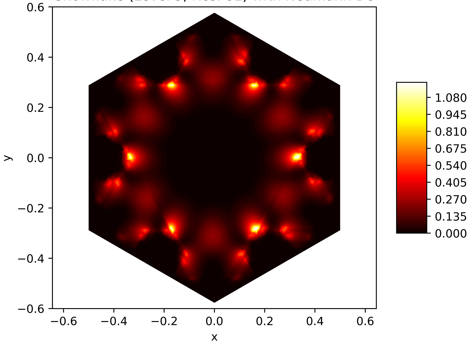
Energy Function of the 36. Eigenfunction on the Snowflake (Level 5, Res. 81) with Neumann BC
