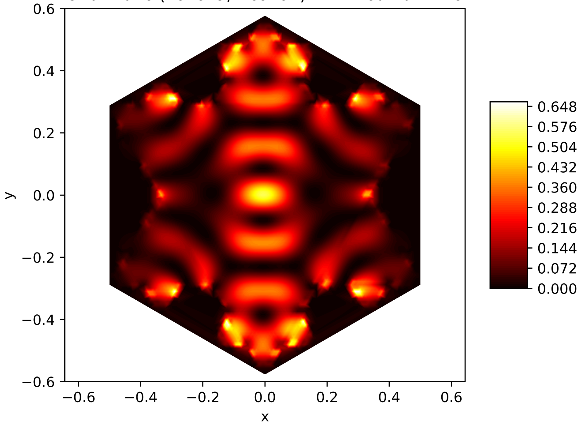
Energy Function of the 40. Eigenfunction on the Snowflake (Level 5, Res. 81) with Neumann BC
