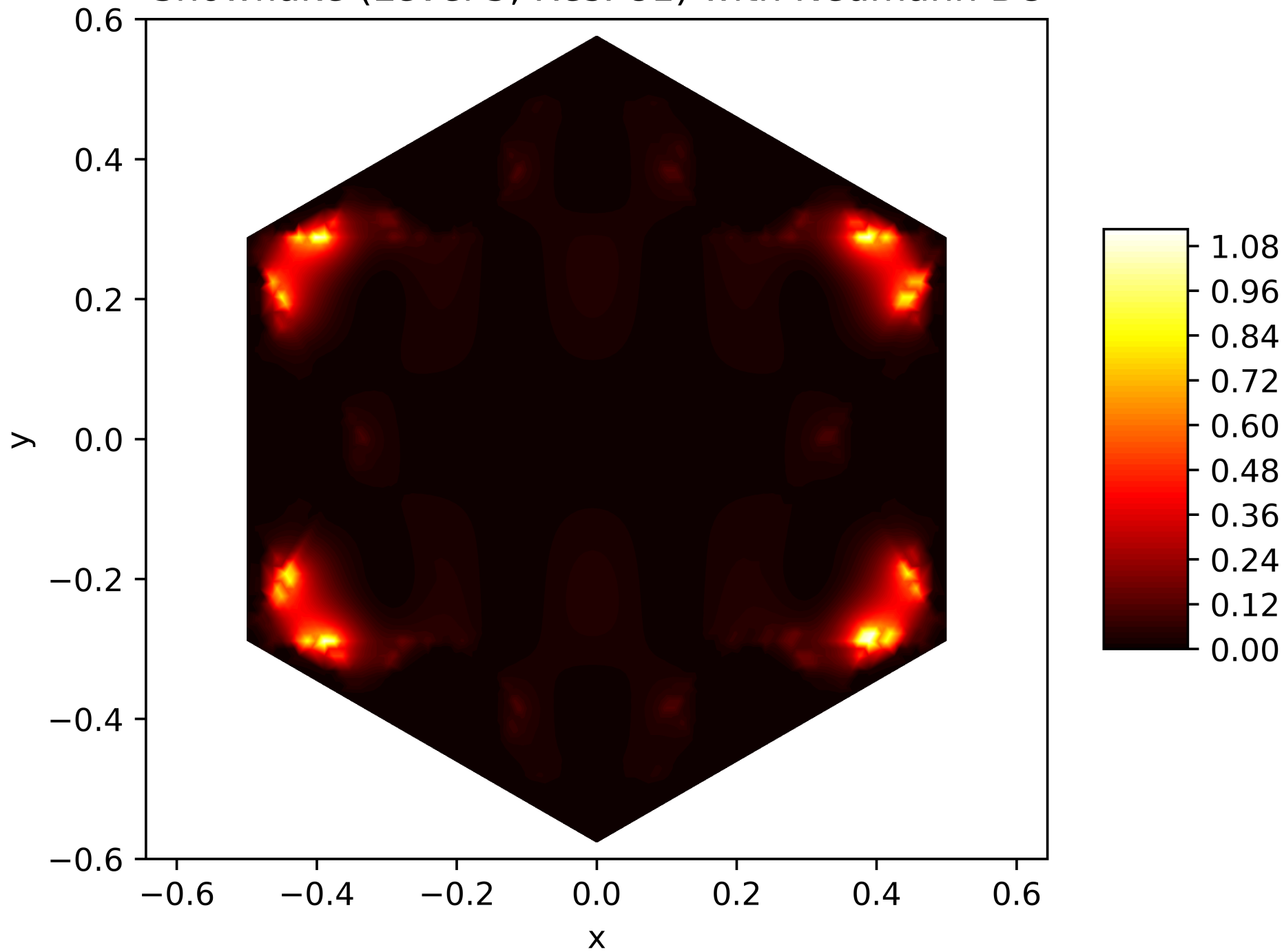
Energy Function of the 24. Eigenfunction on the Snowflake (Level 5, Res. 81) with Neumann BC
