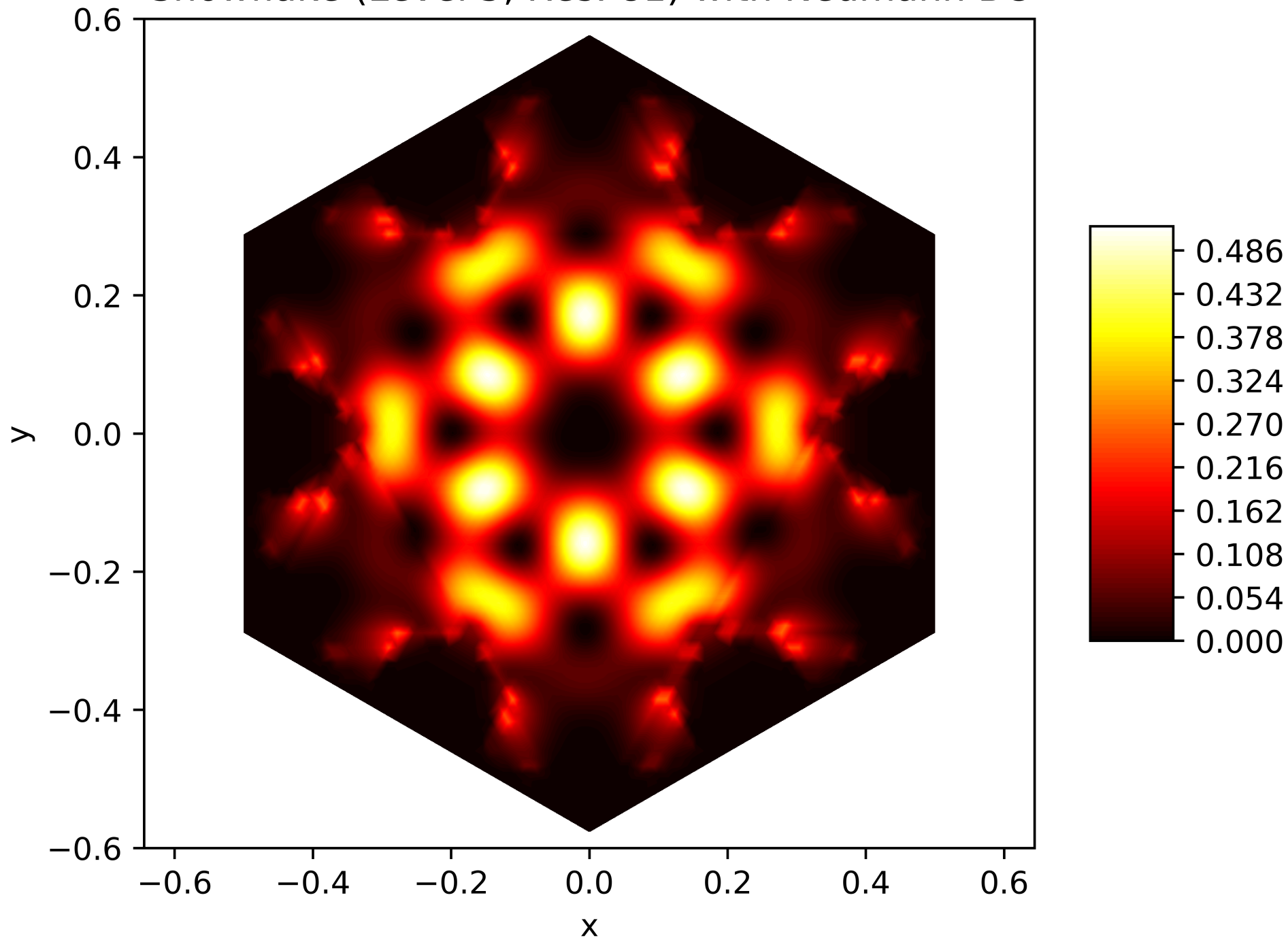
Energy Function of the 39. Eigenfunction on the Snowflake (Level 5, Res. 81) with Neumann BC
