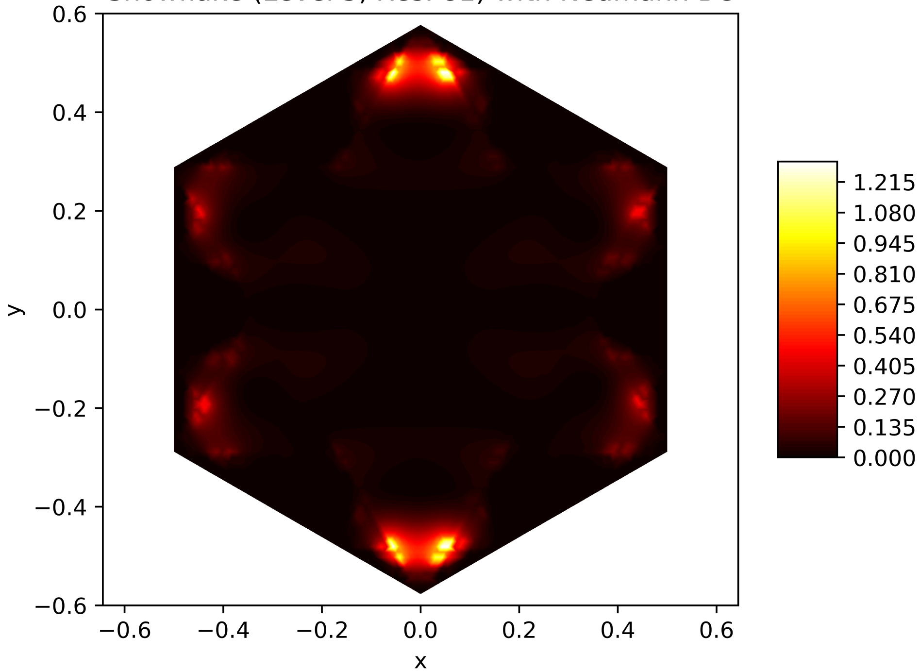
Energy Function of the 23. Eigenfunction on the Snowflake (Level 5, Res. 81) with Neumann BC
