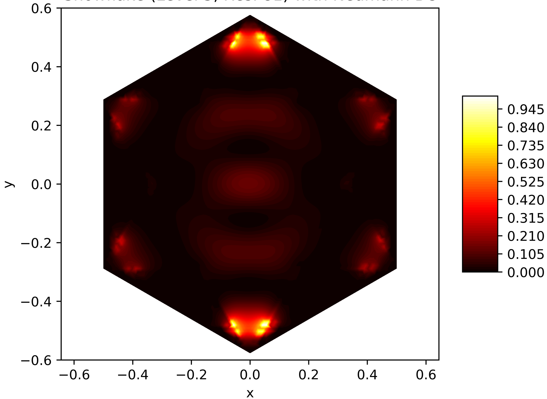
Energy Function of the 21. Eigenfunction on the Snowflake (Level 5, Res. 81) with Neumann BC
