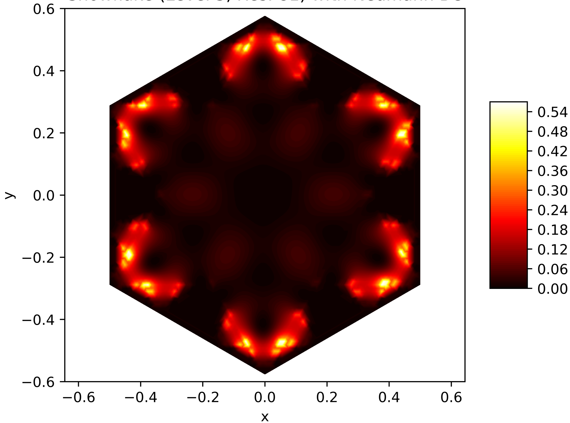
Energy Function of the 26. Eigenfunction on the Snowflake (Level 5, Res. 81) with Neumann BC
