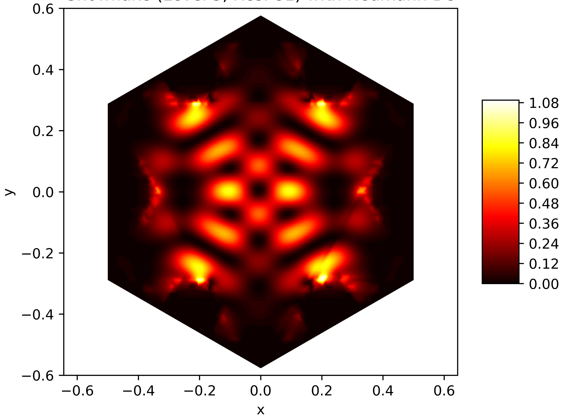
Energy Function of the 51. Eigenfunction on the Snowflake (Level 5, Res. 81) with Neumann BC
