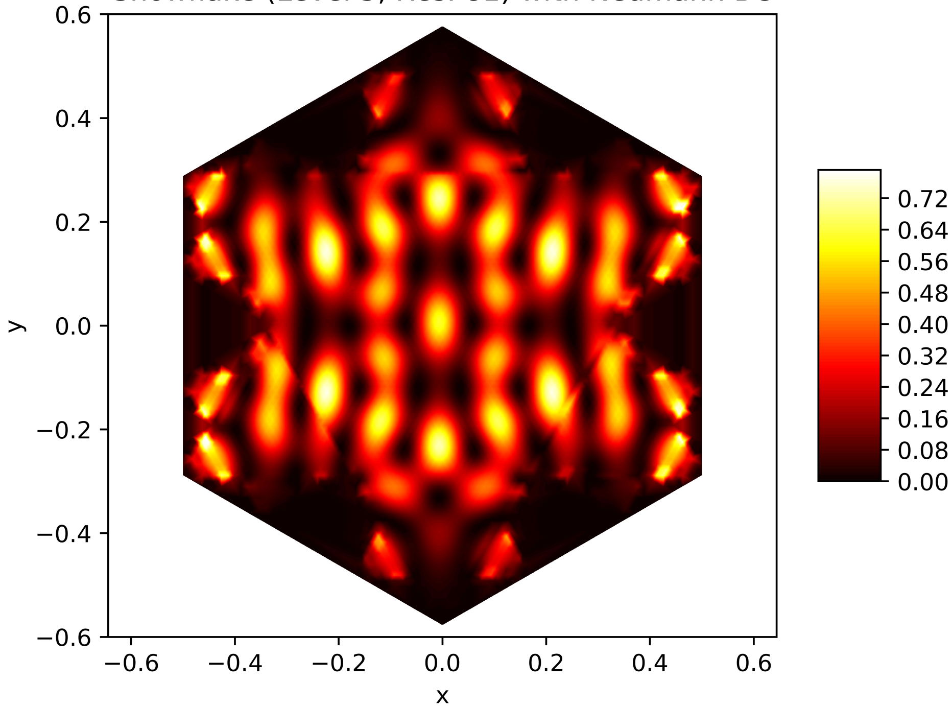
Energy Function of the 60. Eigenfunction on the Snowflake (Level 5, Res. 81) with Neumann BC
