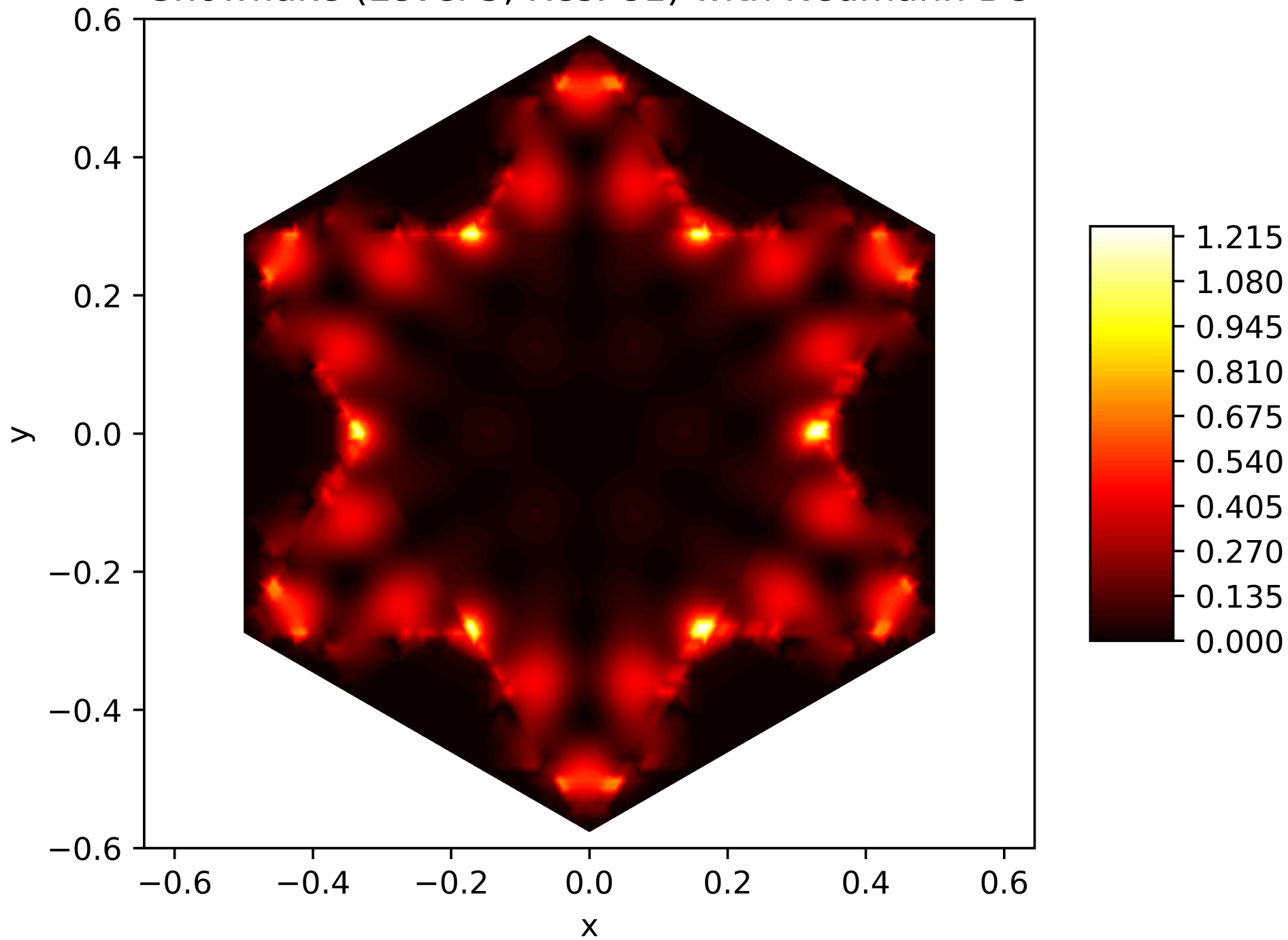
Energy Function of the 48. Eigenfunction on the Snowflake (Level 5, Res. 81) with Neumann BC
