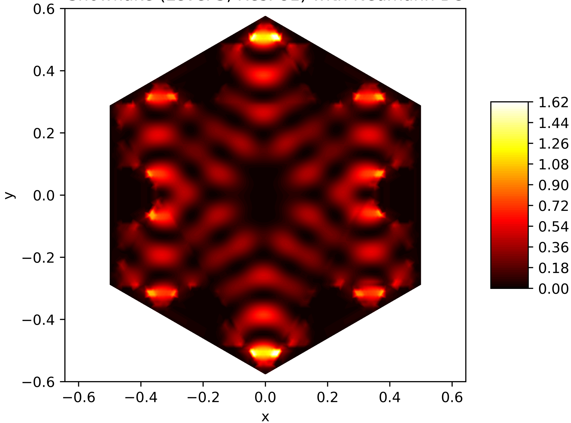
Energy Function of the 57. Eigenfunction on the Snowflake (Level 5, Res. 81) with Neumann BC
