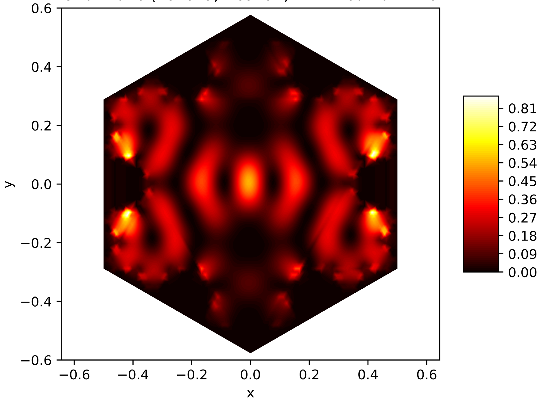
Energy Function of the 41. Eigenfunction on the Snowflake (Level 5, Res. 81) with Neumann BC
