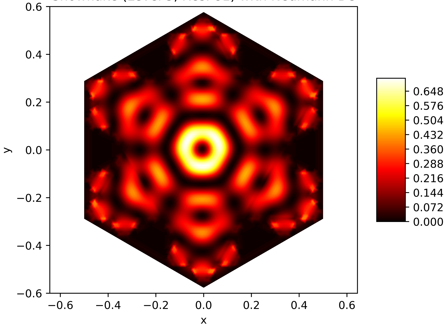
Energy Function of the 49. Eigenfunction on the Snowflake (Level 5, Res. 81) with Neumann BC
