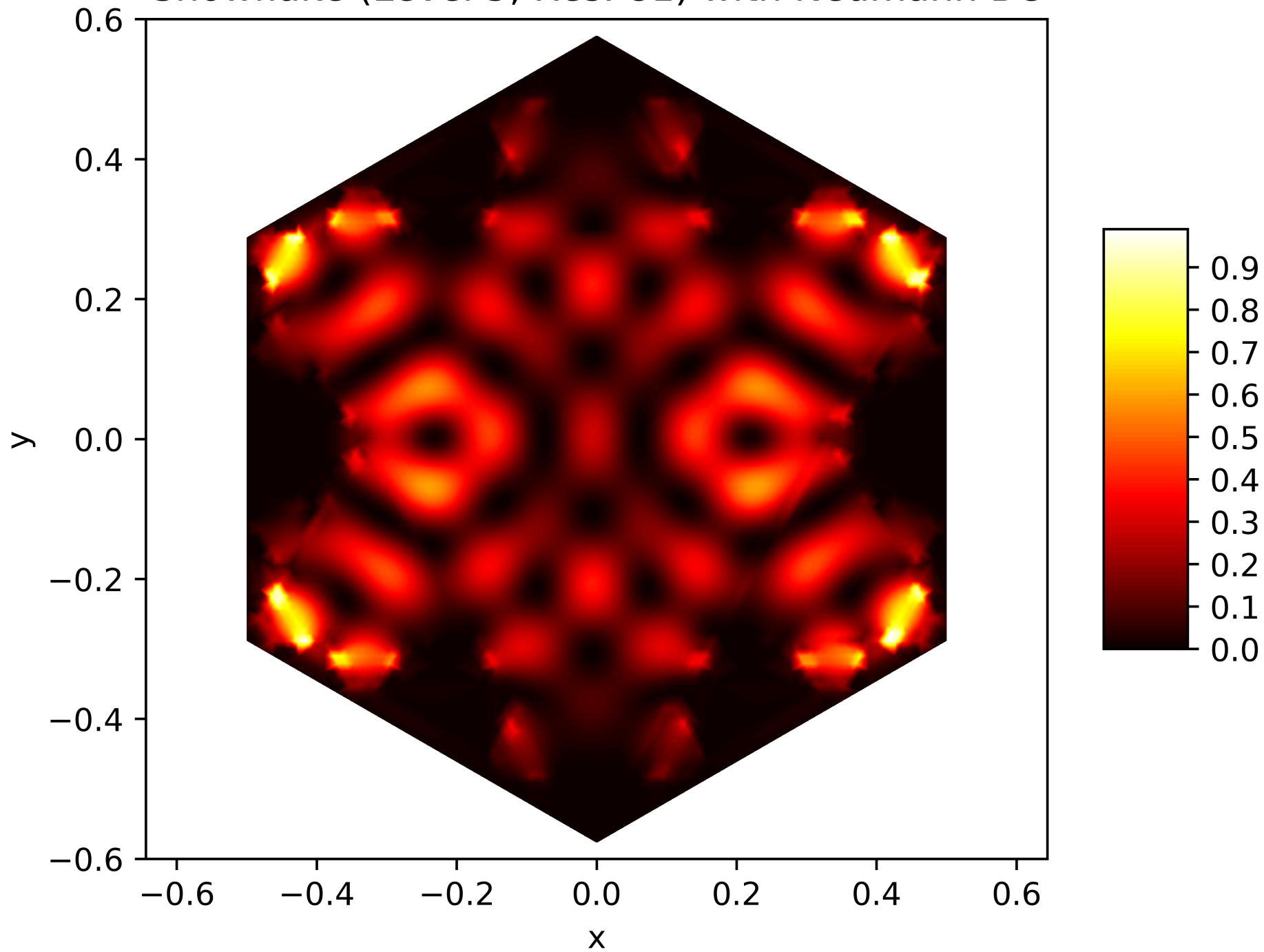
Energy Function of the 53. Eigenfunction on the Snowflake (Level 5, Res. 81) with Neumann BC
