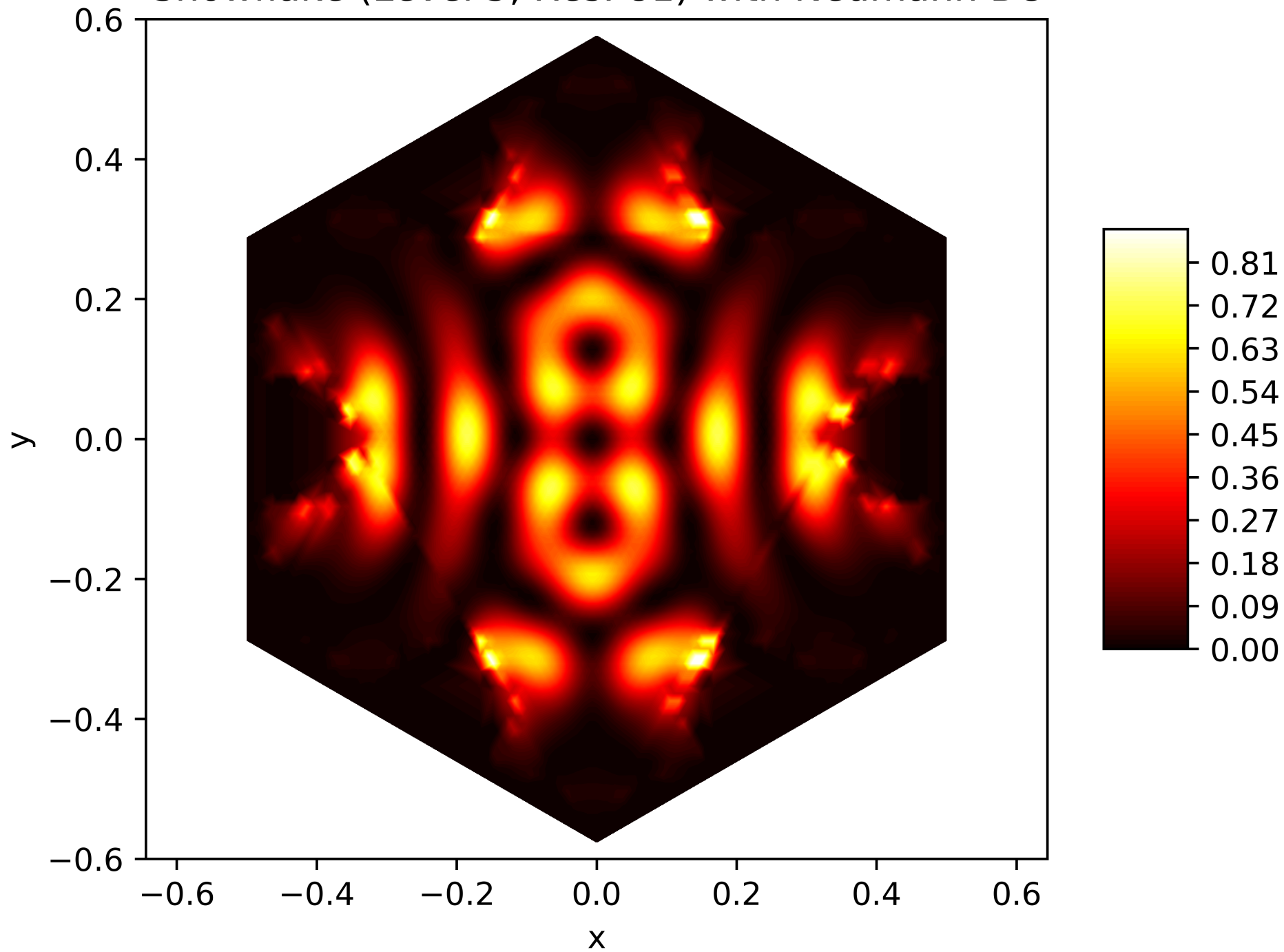
Energy Function of the 50. Eigenfunction on the Snowflake (Level 5, Res. 81) with Neumann BC
