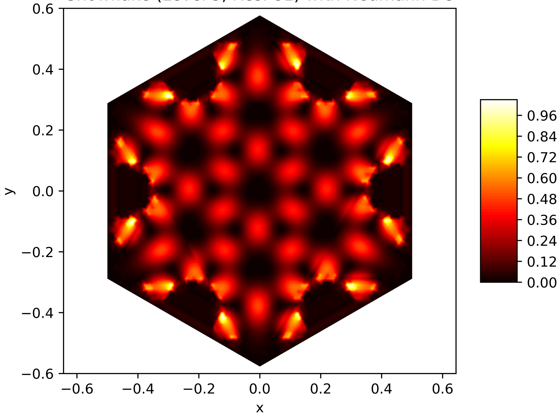
Energy Function of the 55. Eigenfunction on the Snowflake (Level 5, Res. 81) with Neumann BC
