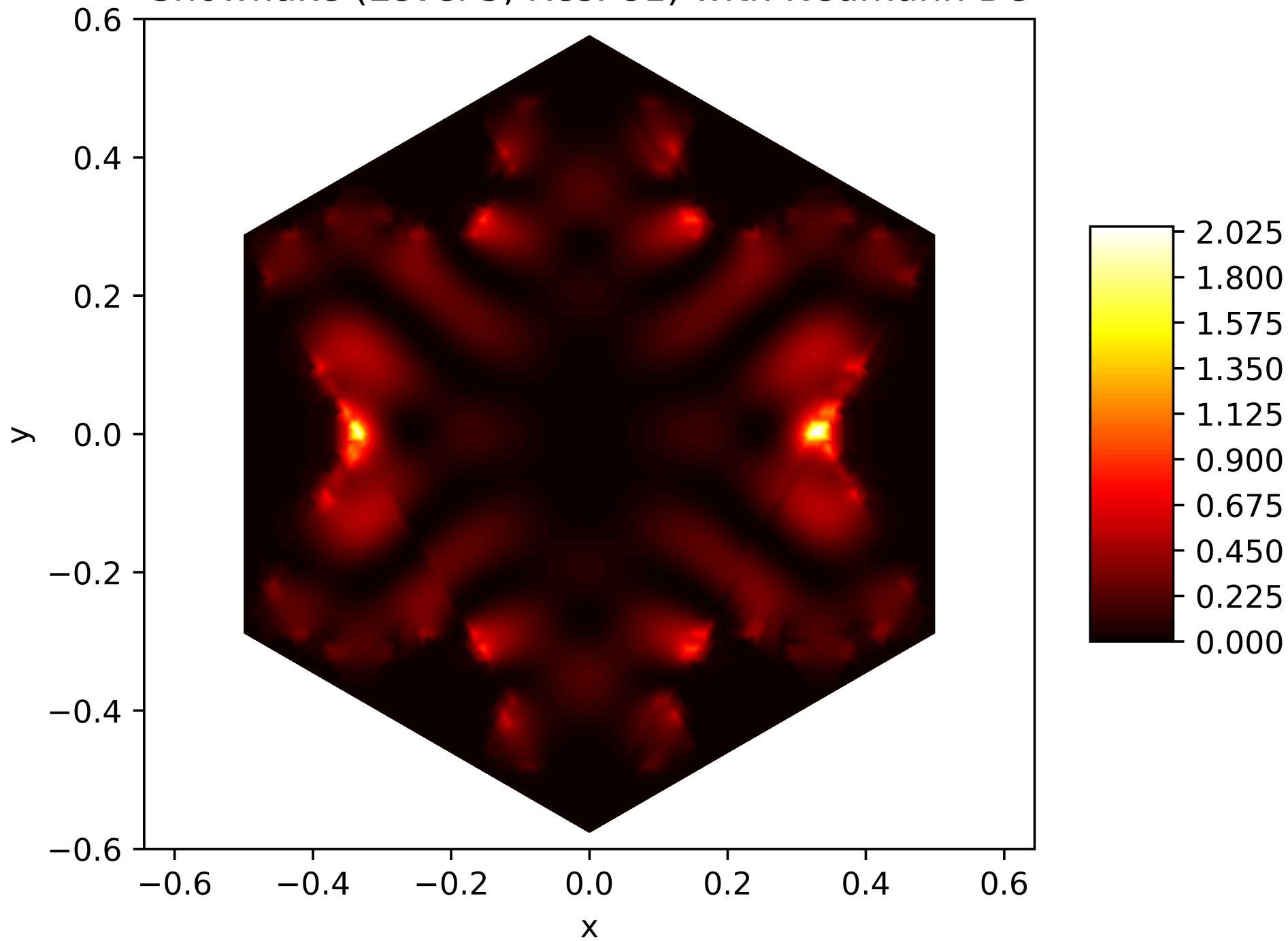
Energy Function of the 46. Eigenfunction on the Snowflake (Level 5, Res. 81) with Neumann BC
