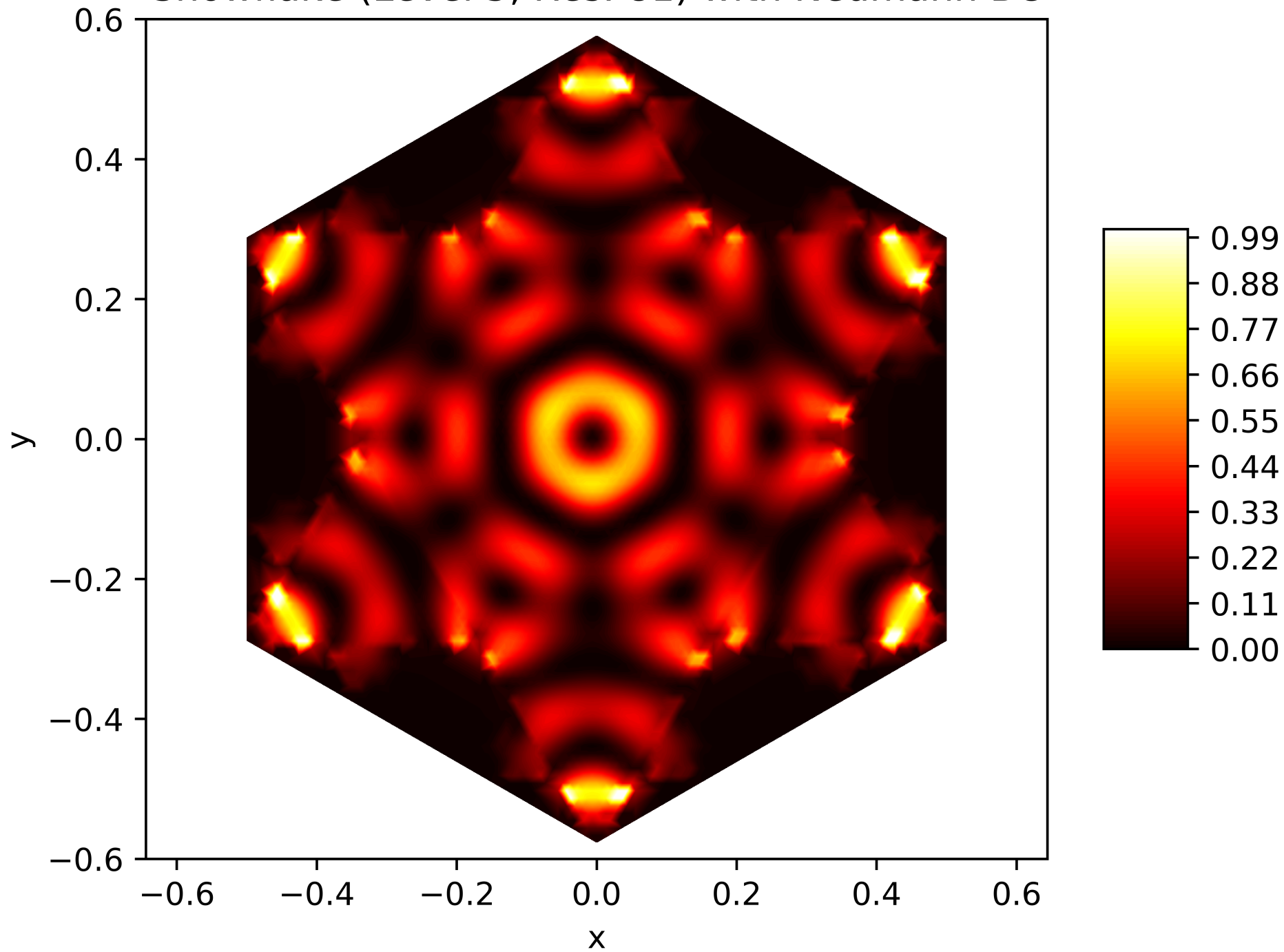
Energy Function of the 56. Eigenfunction on the Snowflake (Level 5, Res. 81) with Neumann BC
