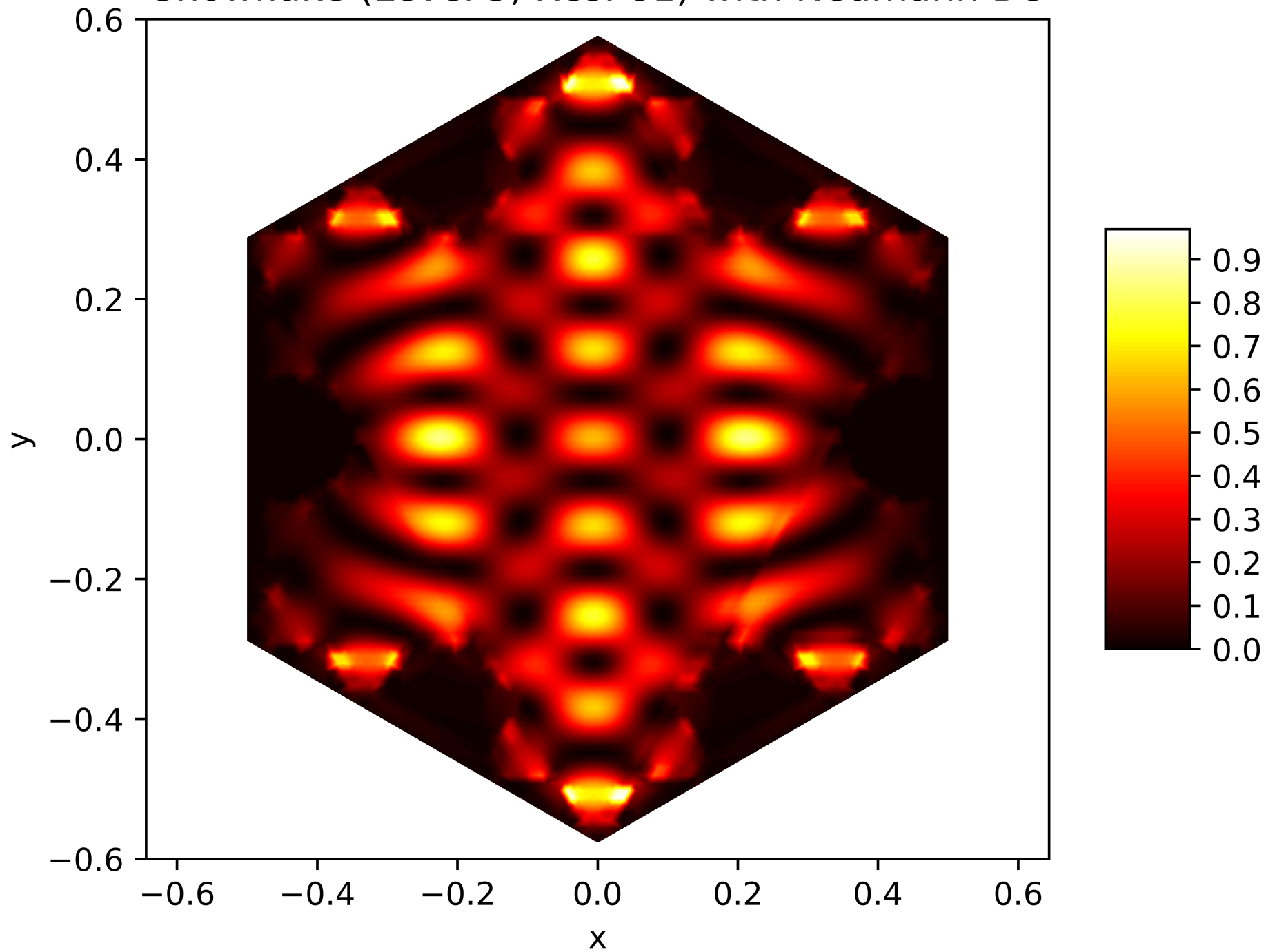
Energy Function of the 59. Eigenfunction on the Snowflake (Level 5, Res. 81) with Neumann BC
