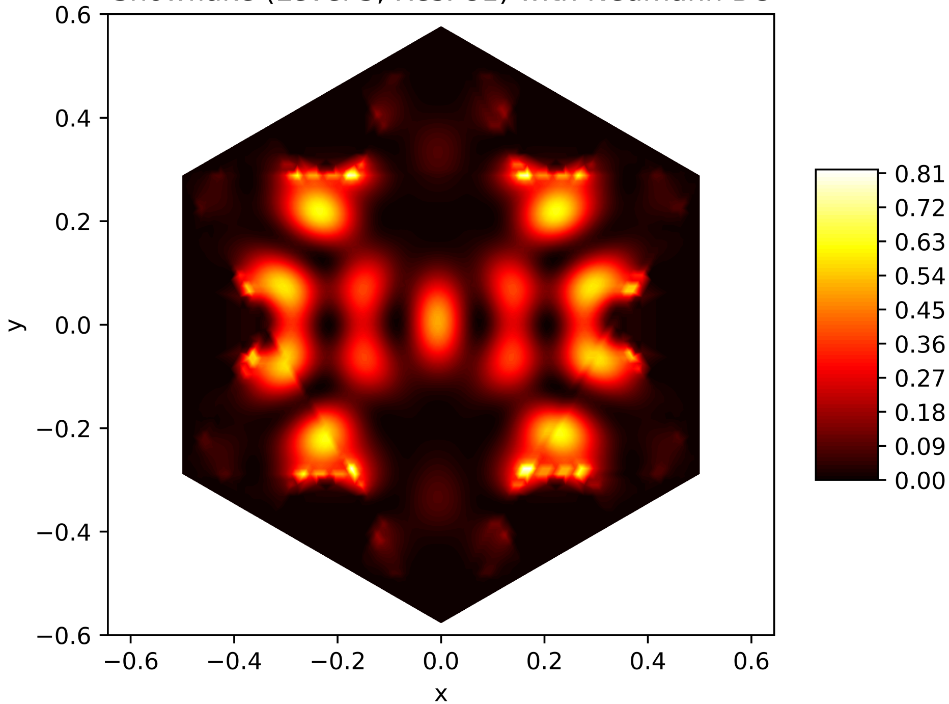
Energy Function of the 43. Eigenfunction on the Snowflake (Level 5, Res. 81) with Neumann BC
