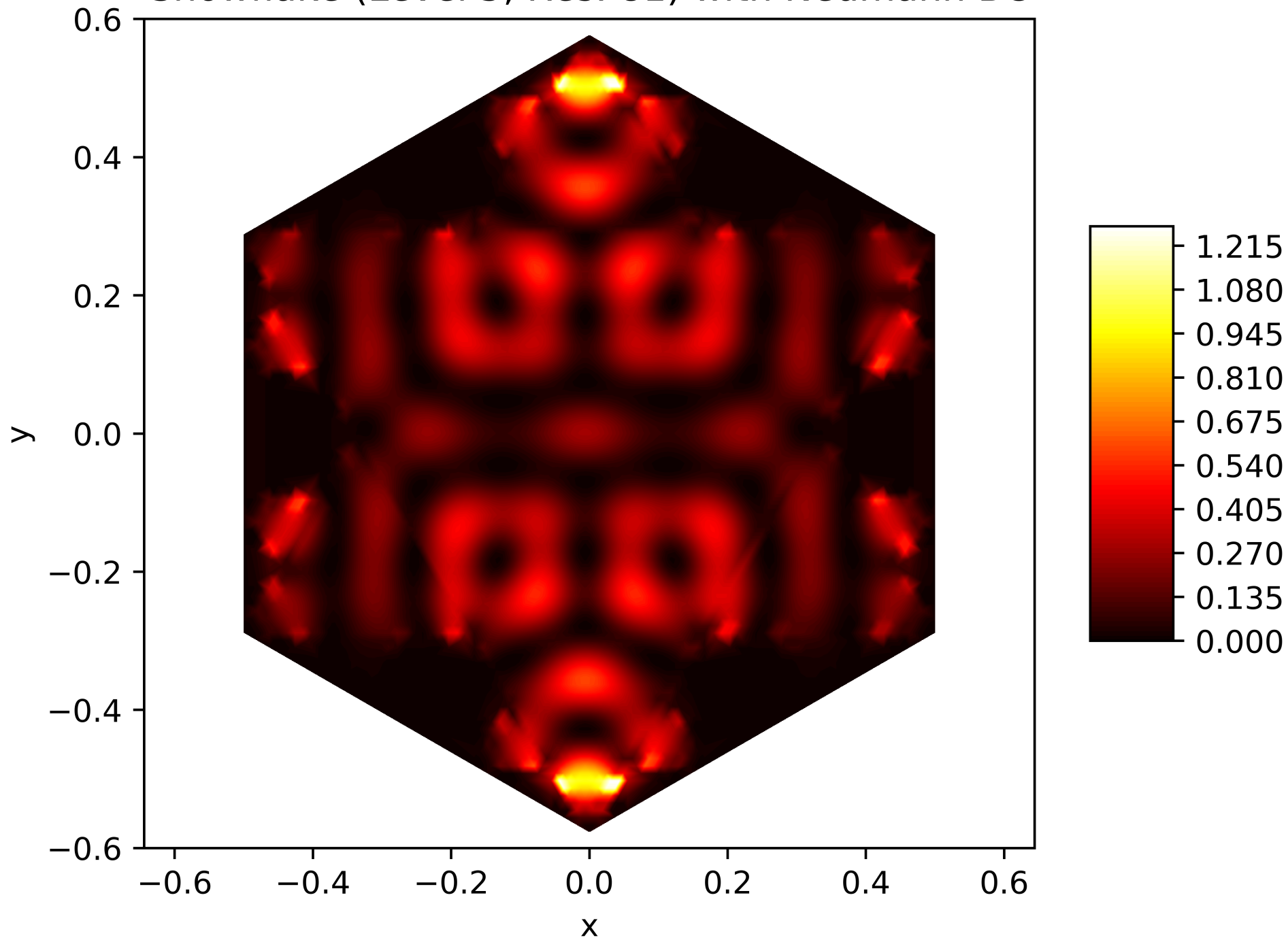
Energy Function of the 52. Eigenfunction on the Snowflake (Level 5, Res. 81) with Neumann BC
