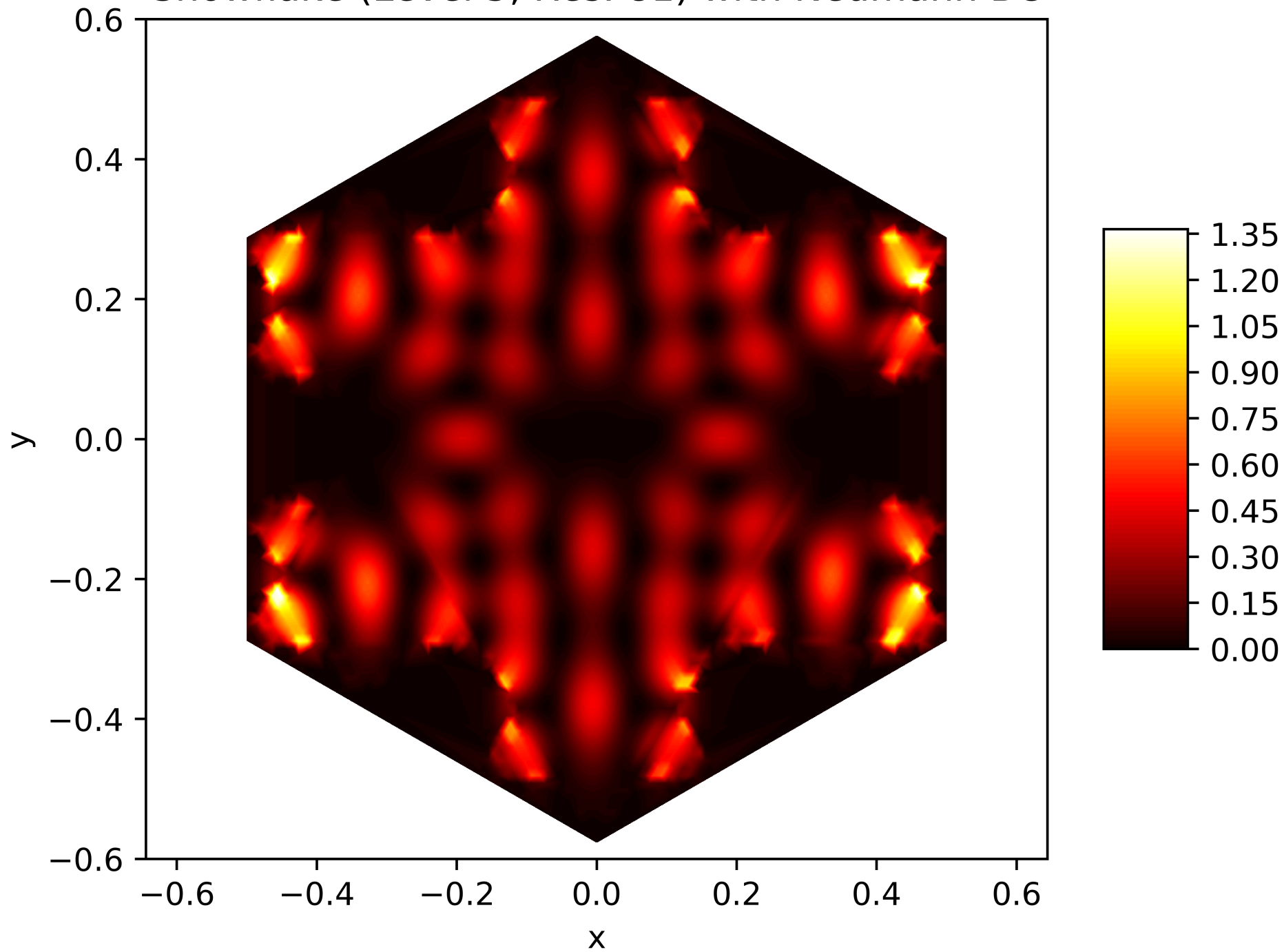
Energy Function of the 58. Eigenfunction on the Snowflake (Level 5, Res. 81) with Neumann BC
