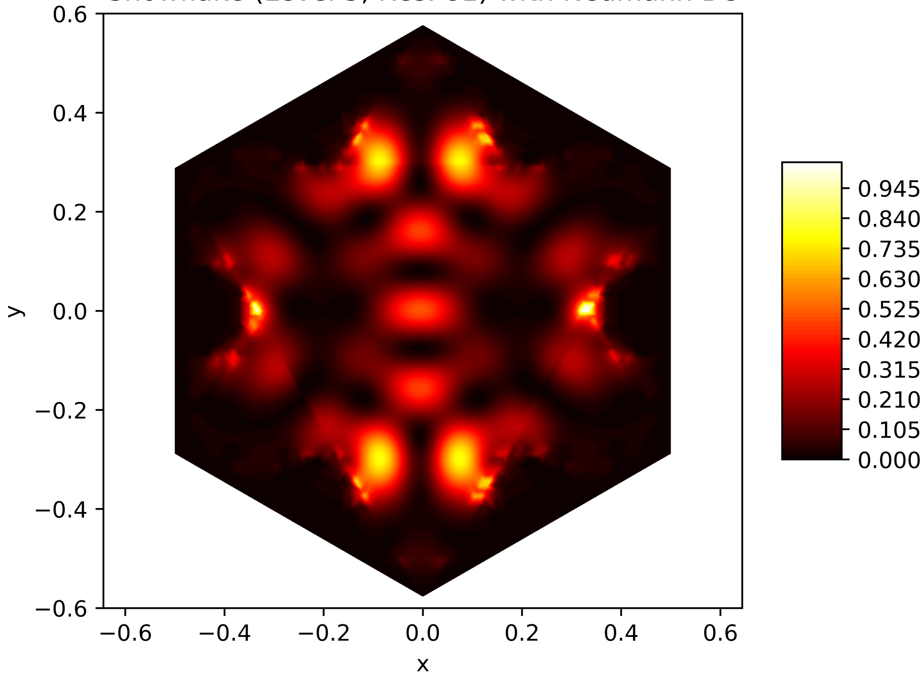
Energy Function of the 42. Eigenfunction on the Snowflake (Level 5, Res. 81) with Neumann BC
