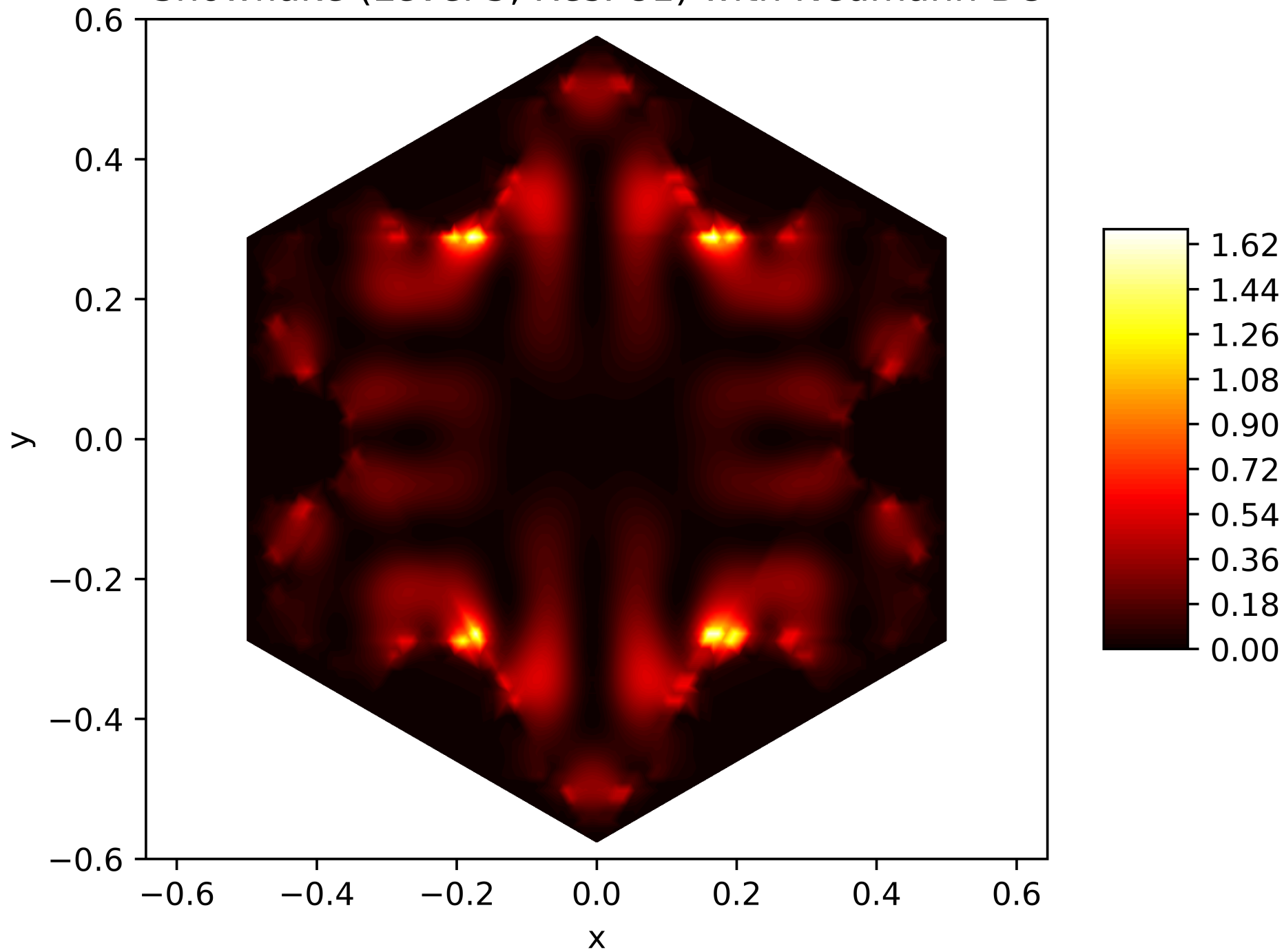
Energy Function of the 47. Eigenfunction on the Snowflake (Level 5, Res. 81) with Neumann BC
