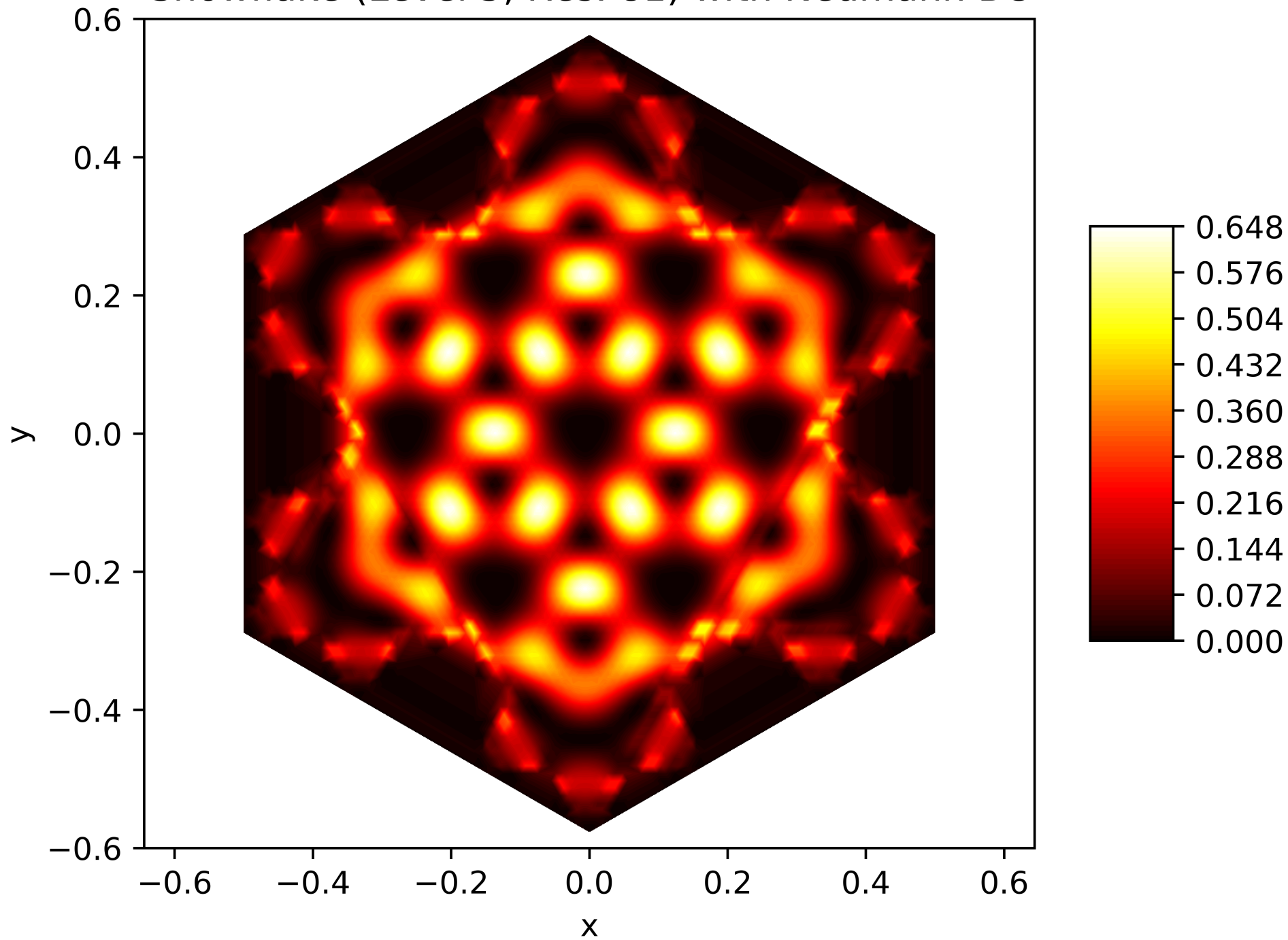
Energy Function of the 54. Eigenfunction on the Snowflake (Level 5, Res. 81) with Neumann BC
