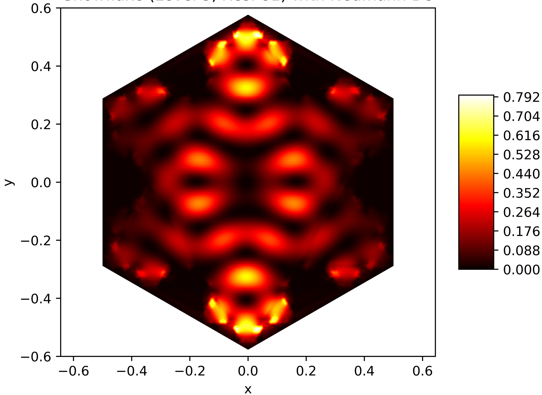
Energy Function of the 44. Eigenfunction on the Snowflake (Level 5, Res. 81) with Neumann BC
