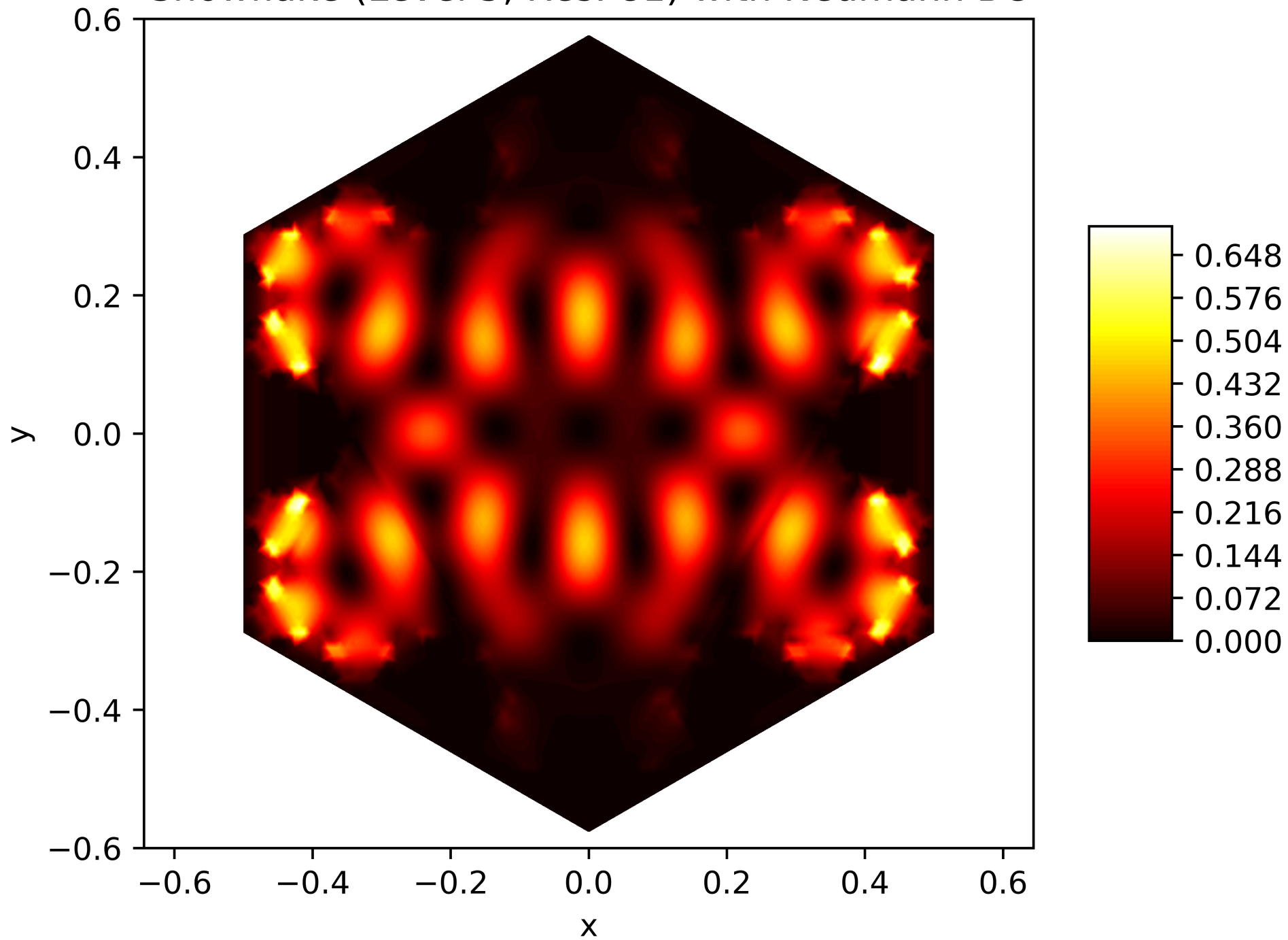
Energy Function of the 45. Eigenfunction on the Snowflake (Level 5, Res. 81) with Neumann BC
