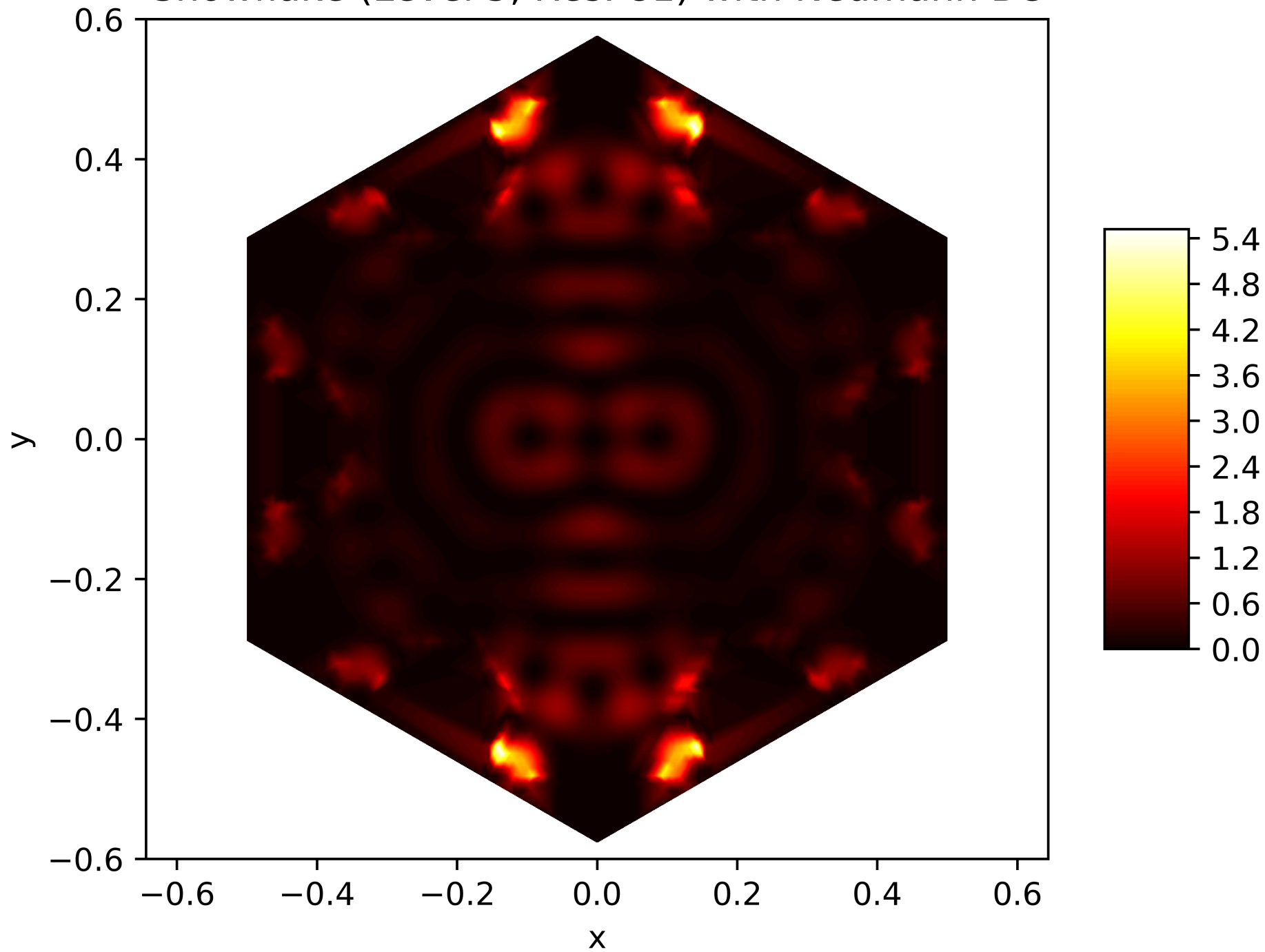
Energy Function of the 93. Eigenfunction on the Snowflake (Level 5, Res. 81) with Neumann BC
