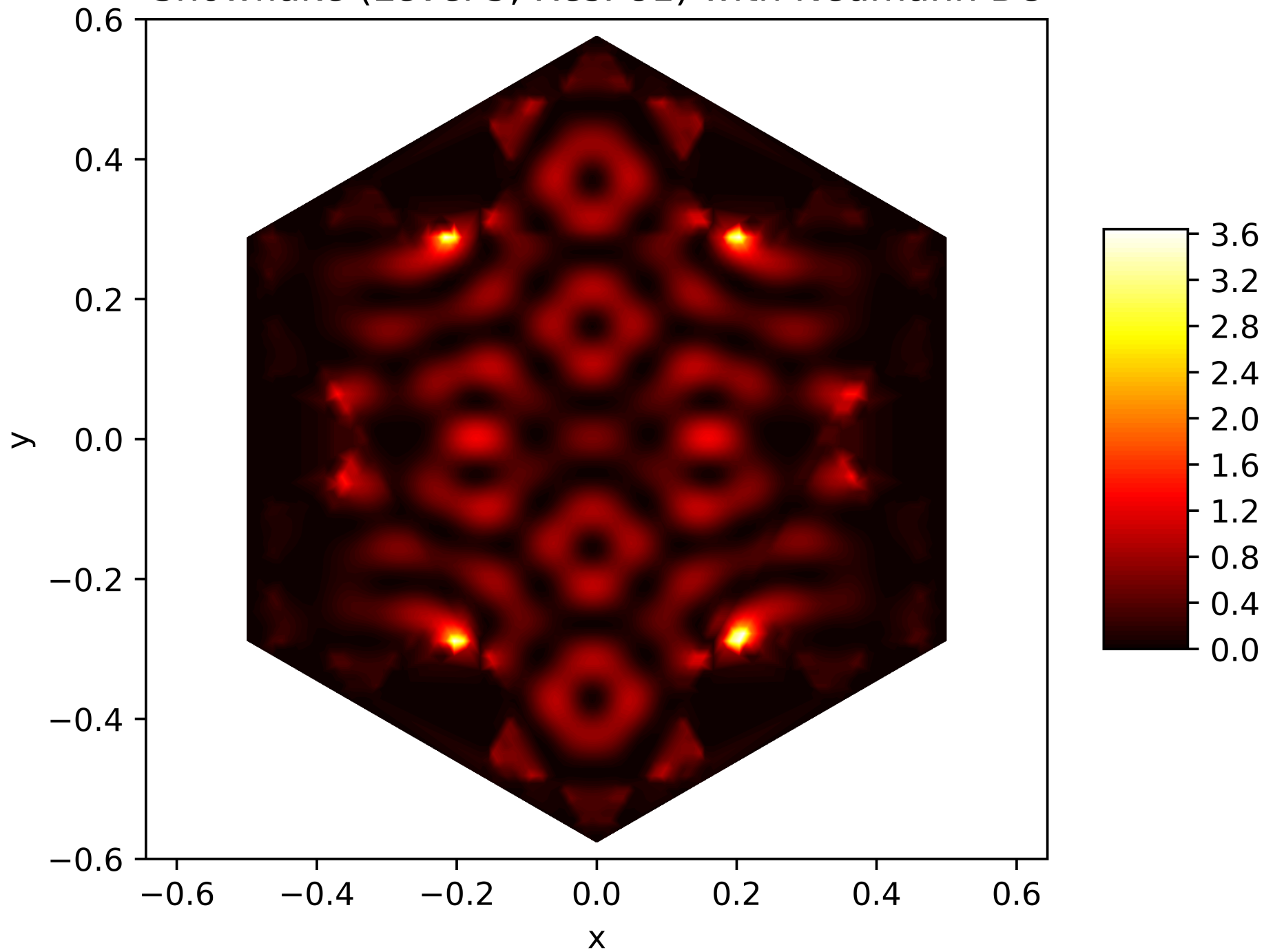
Energy Function of the 91. Eigenfunction on the Snowflake (Level 5, Res. 81) with Neumann BC
