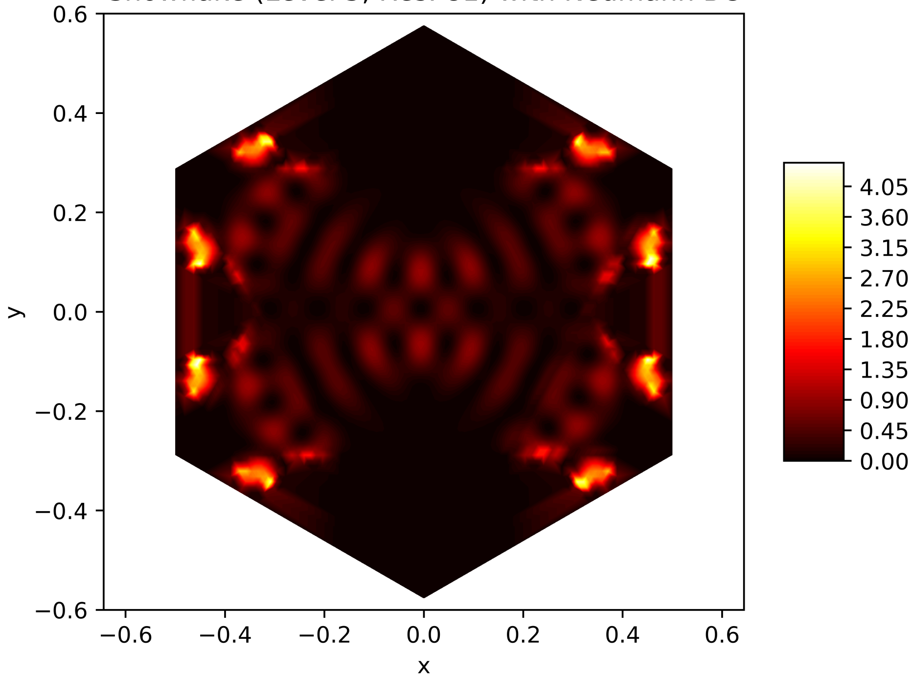
Energy Function of the 94. Eigenfunction on the Snowflake (Level 5, Res. 81) with Neumann BC
