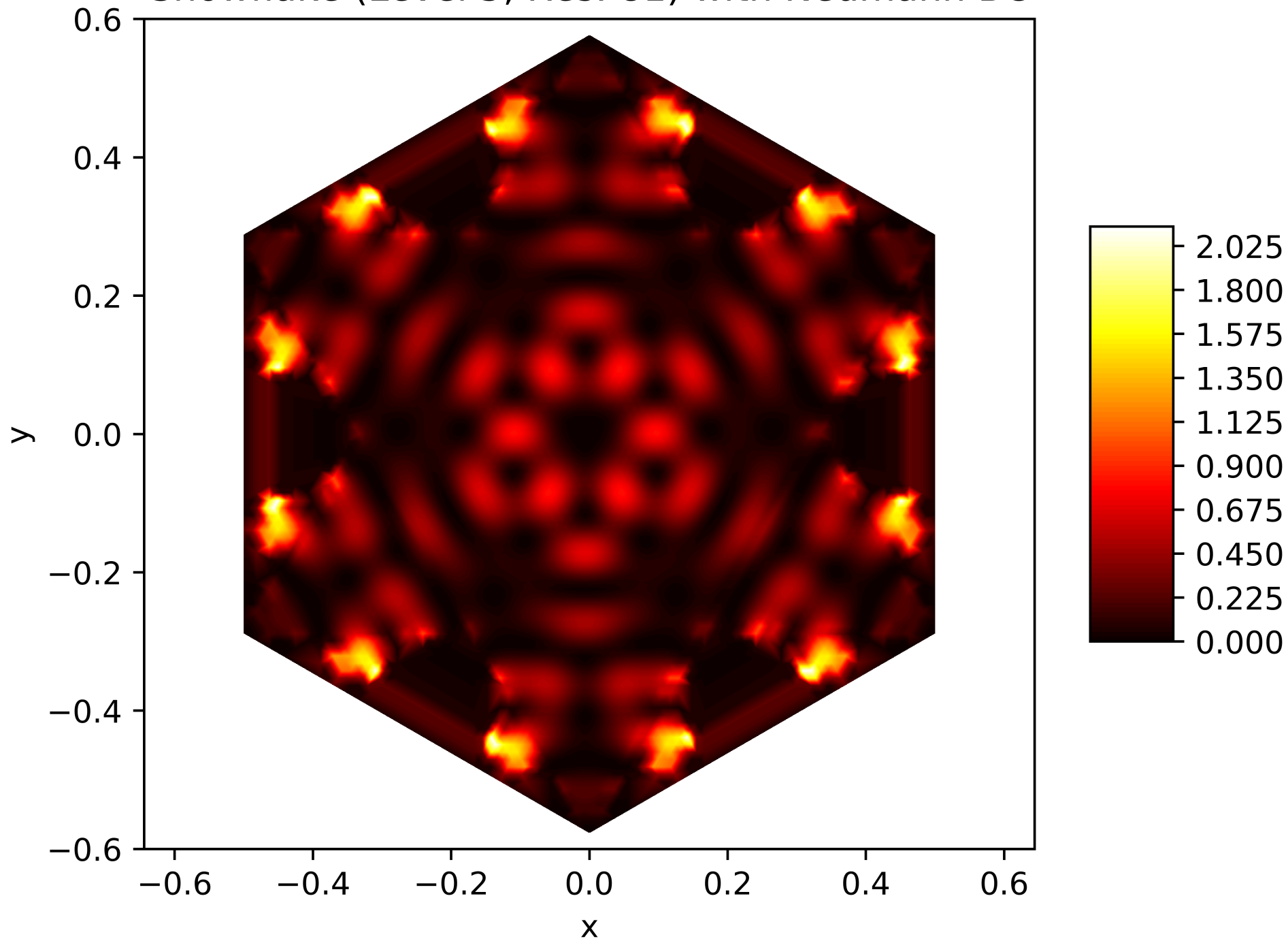
Energy Function of the 87. Eigenfunction on the Snowflake (Level 5, Res. 81) with Neumann BC
