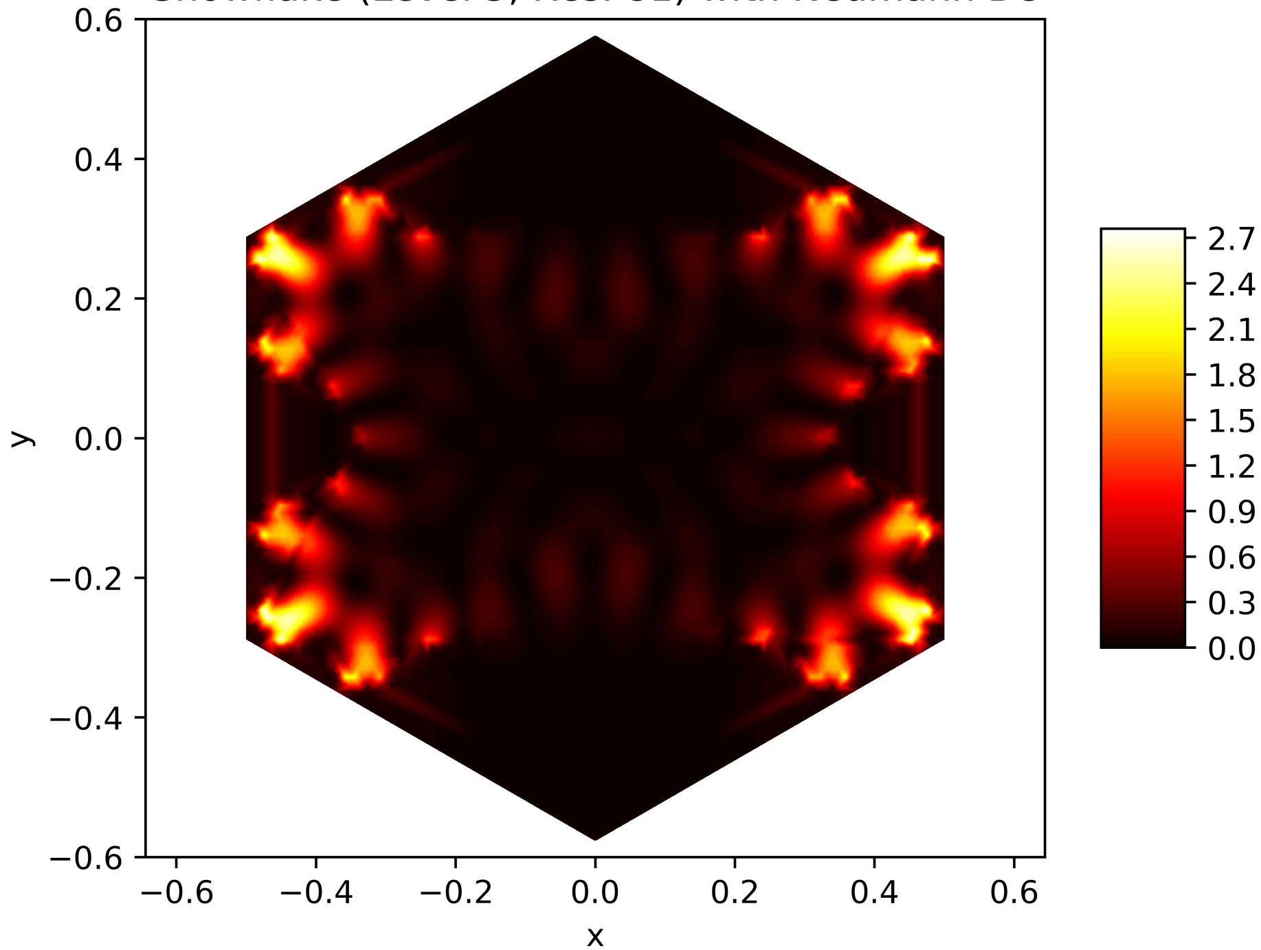
Energy Function of the 83. Eigenfunction on the Snowflake (Level 5, Res. 81) with Neumann BC
