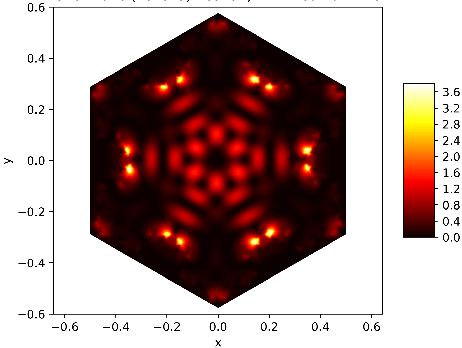
Energy Function of the 98. Eigenfunction on the Snowflake (Level 5, Res. 81) with Neumann BC
