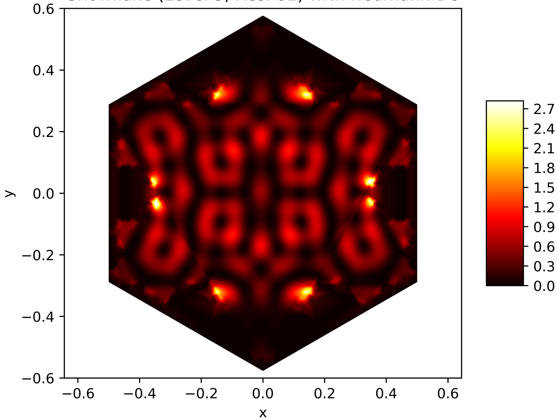
Energy Function of the 92. Eigenfunction on the Snowflake (Level 5, Res. 81) with Neumann BC
