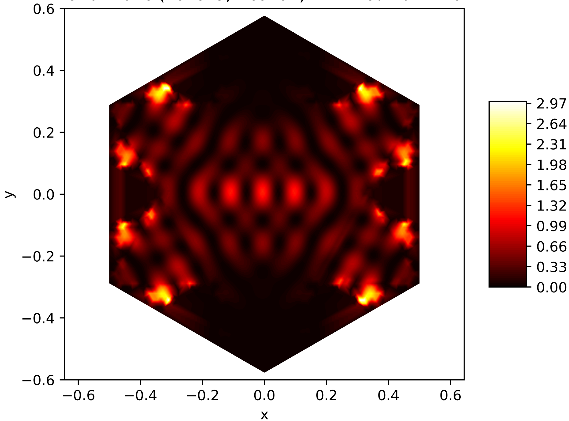
Energy Function of the 86. Eigenfunction on the Snowflake (Level 5, Res. 81) with Neumann BC
