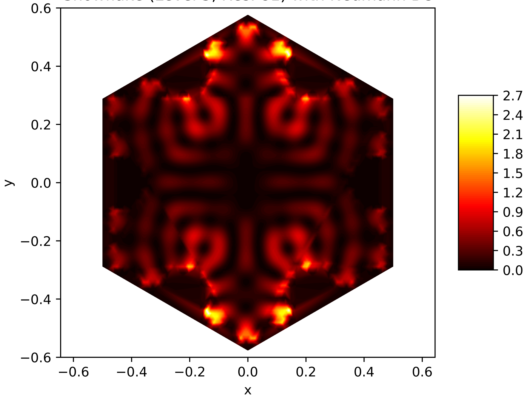
Energy Function of the 88. Eigenfunction on the Snowflake (Level 5, Res. 81) with Neumann BC
