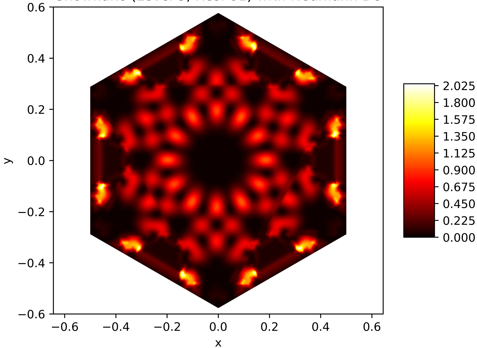
Energy Function of the 96. Eigenfunction on the Snowflake (Level 5, Res. 81) with Neumann BC
