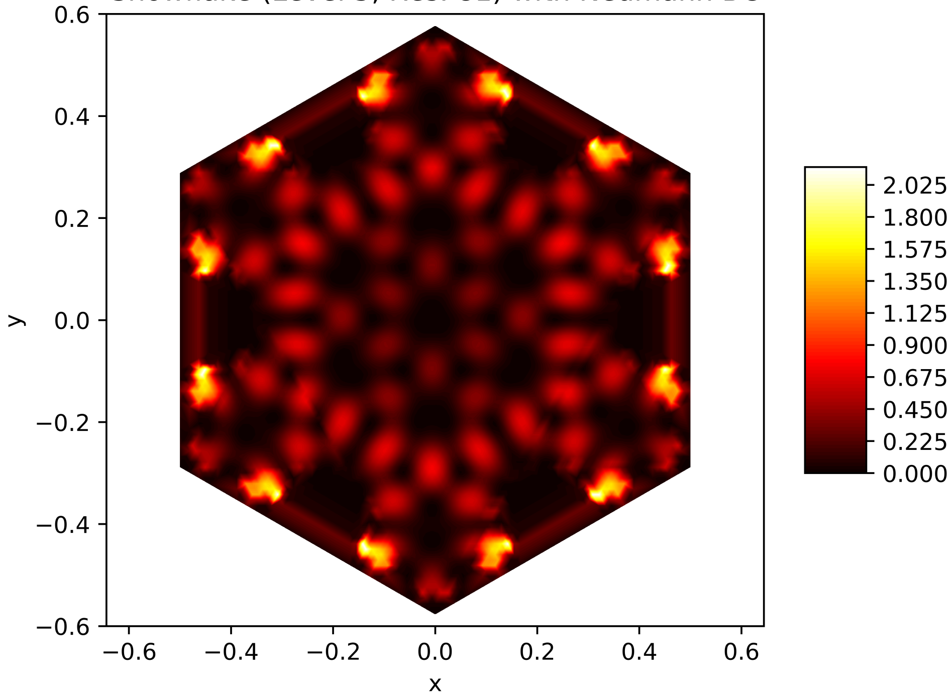
Energy Function of the 90. Eigenfunction on the Snowflake (Level 5, Res. 81) with Neumann BC
