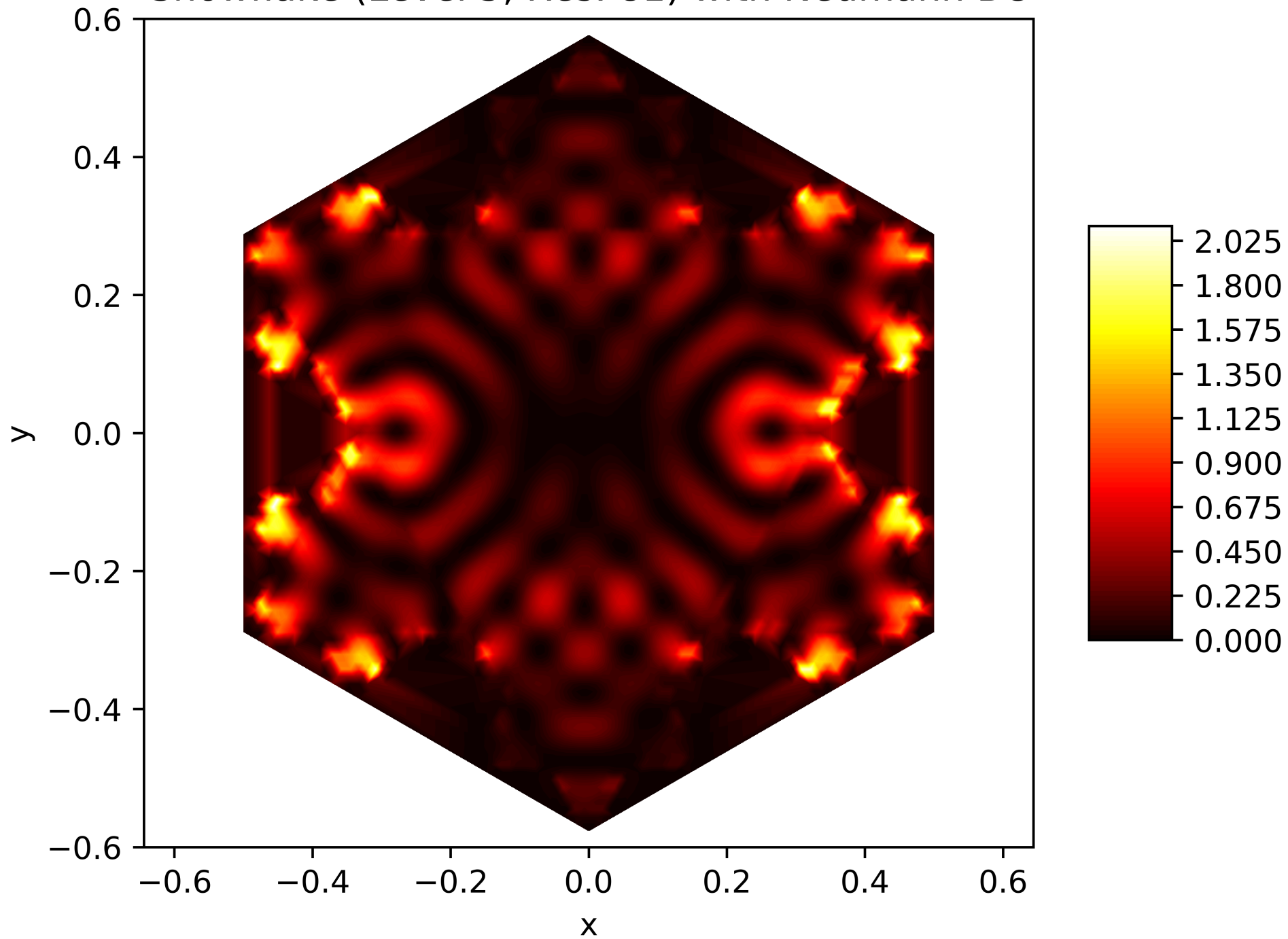
Energy Function of the 89. Eigenfunction on the Snowflake (Level 5, Res. 81) with Neumann BC
