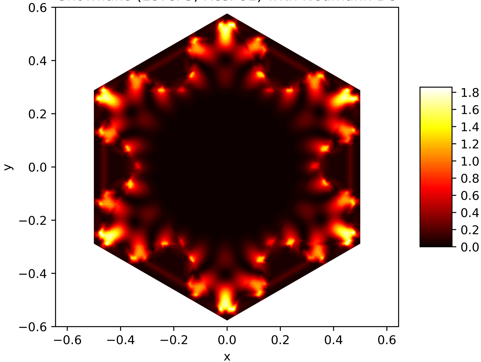
Energy Function of the 84. Eigenfunction on the Snowflake (Level 5, Res. 81) with Neumann BC
