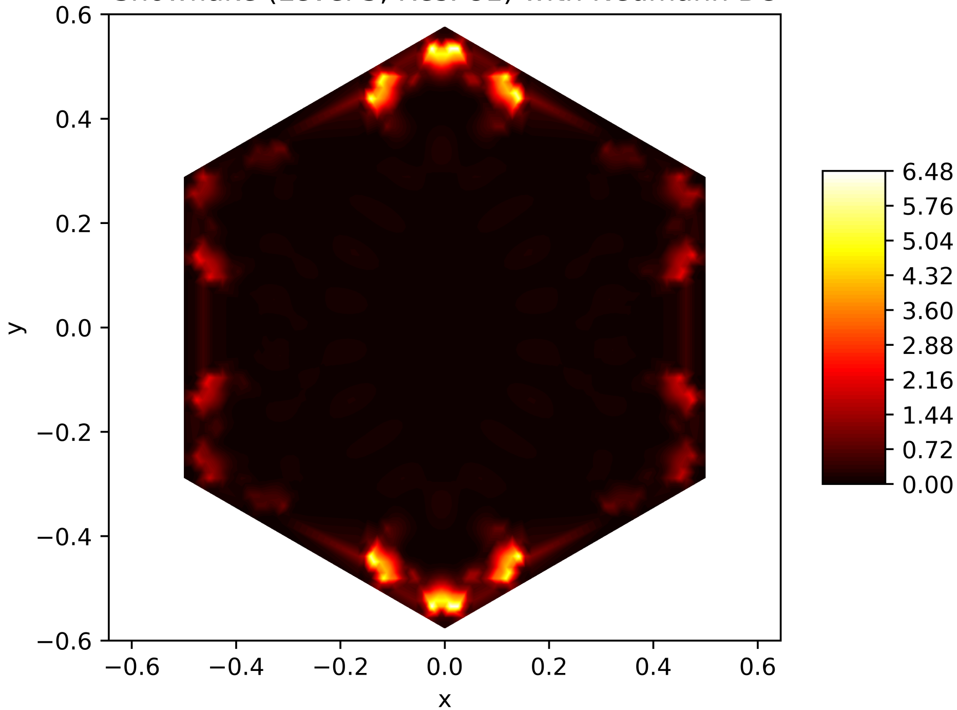
Energy Function of the 99. Eigenfunction on the Snowflake (Level 5, Res. 81) with Neumann BC
