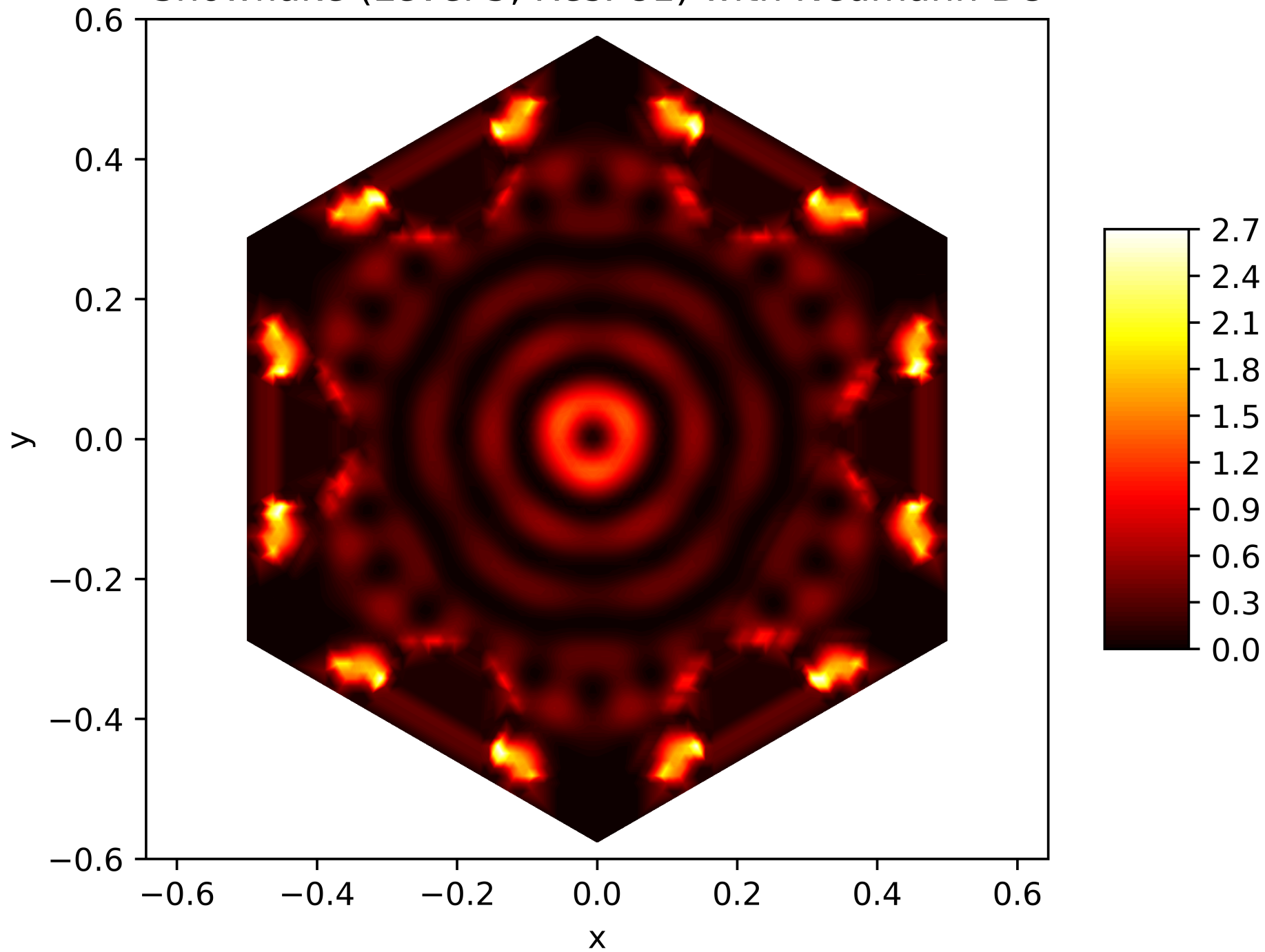
Energy Function of the 95. Eigenfunction on the Snowflake (Level 5, Res. 81) with Neumann BC
