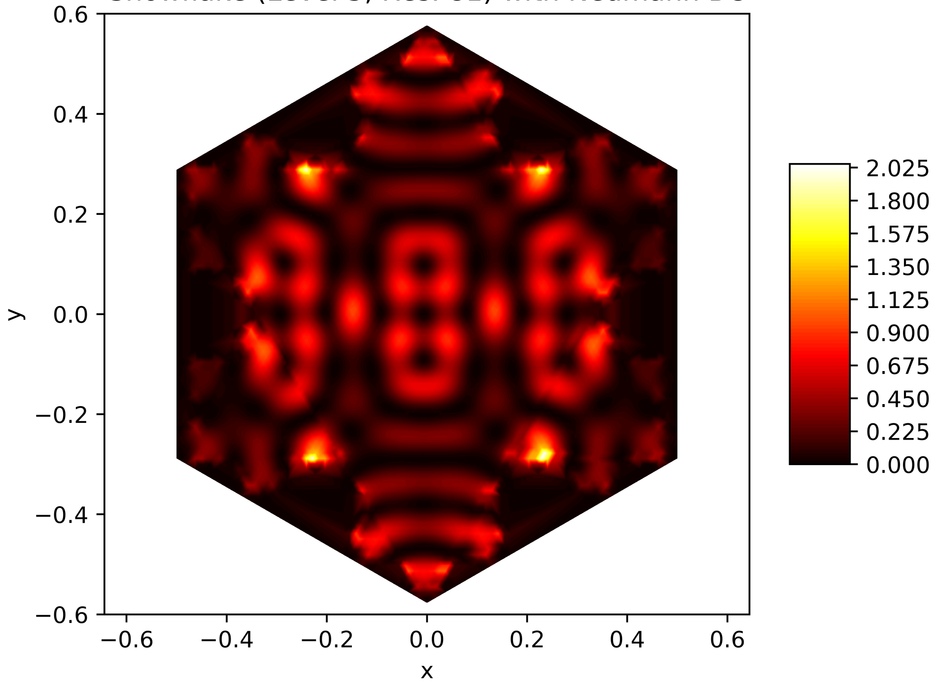
Energy Function of the 81. Eigenfunction on the Snowflake (Level 5, Res. 81) with Neumann BC
