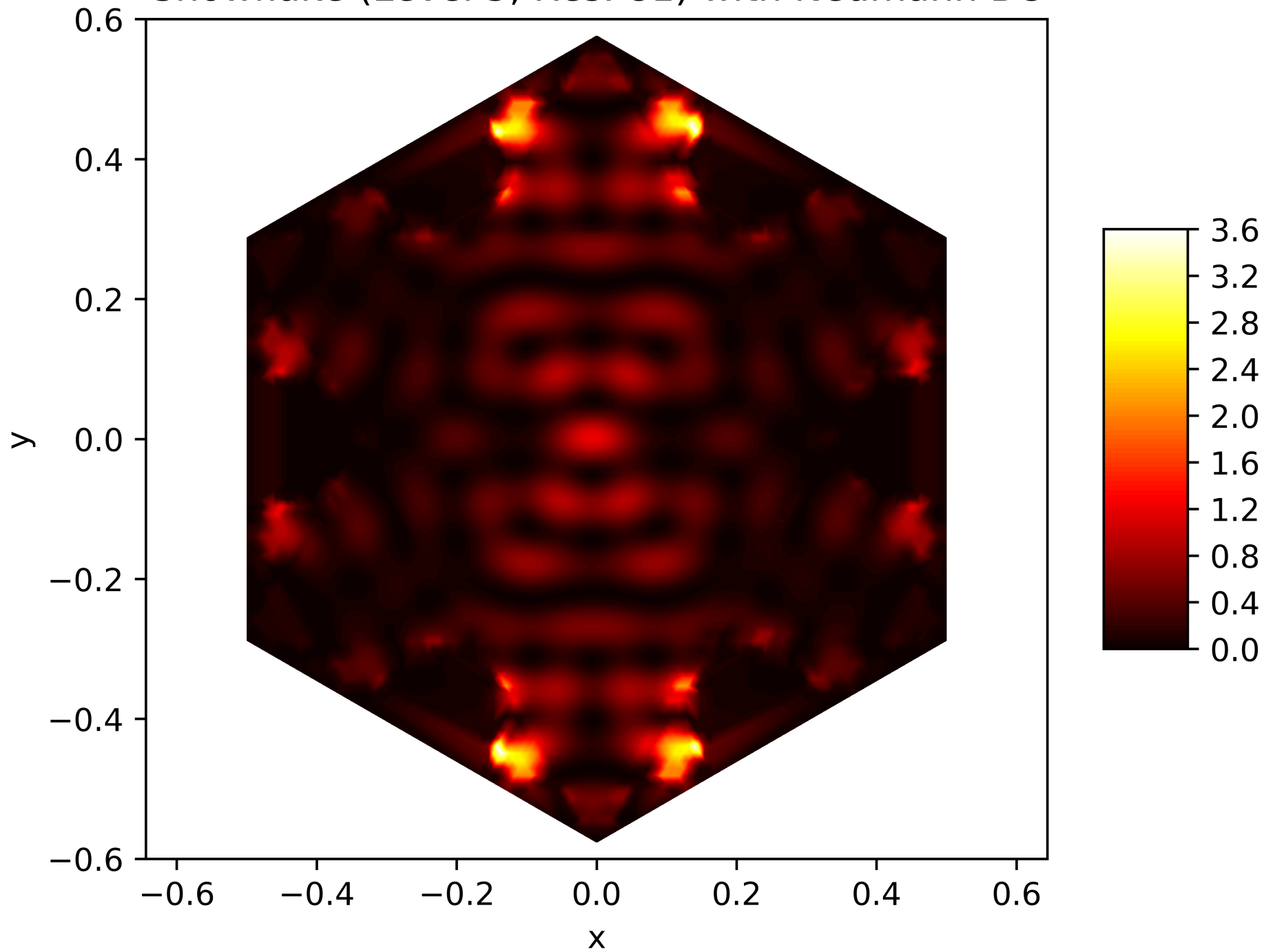
Energy Function of the 85. Eigenfunction on the Snowflake (Level 5, Res. 81) with Neumann BC
