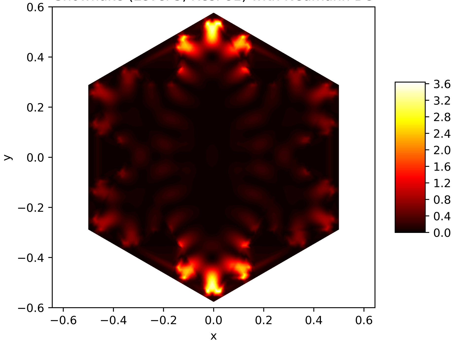
Energy Function of the 82. Eigenfunction on the Snowflake (Level 5, Res. 81) with Neumann BC
