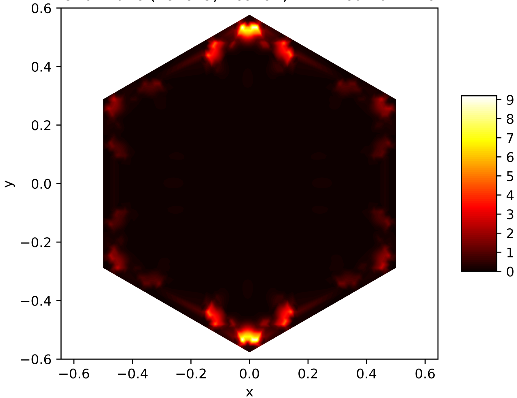
Energy Function of the 101. Eigenfunction on the Snowflake (Level 5, Res. 81) with Neumann BC
