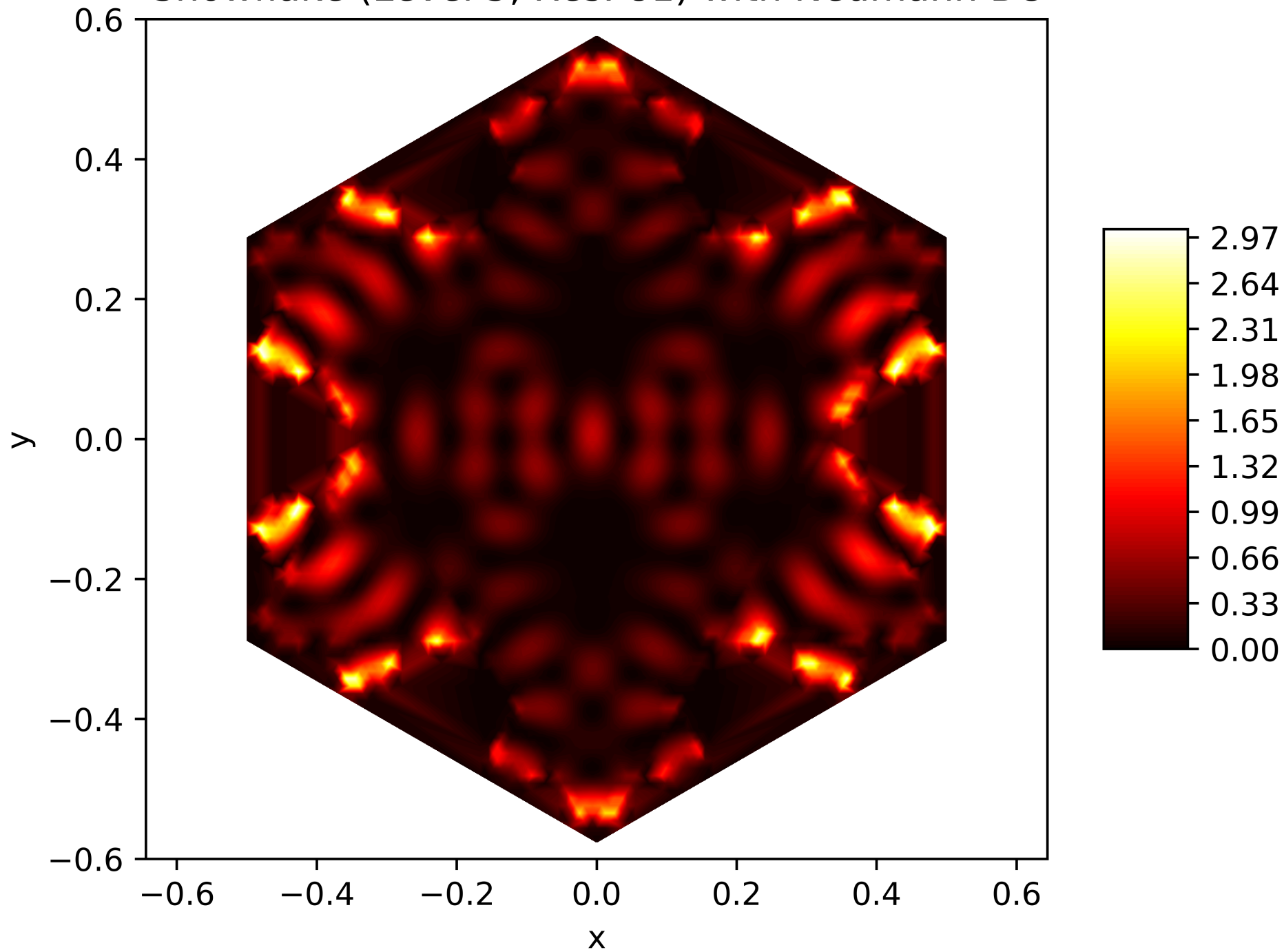
Energy Function of the 118. Eigenfunction on the Snowflake (Level 5, Res. 81) with Neumann BC
