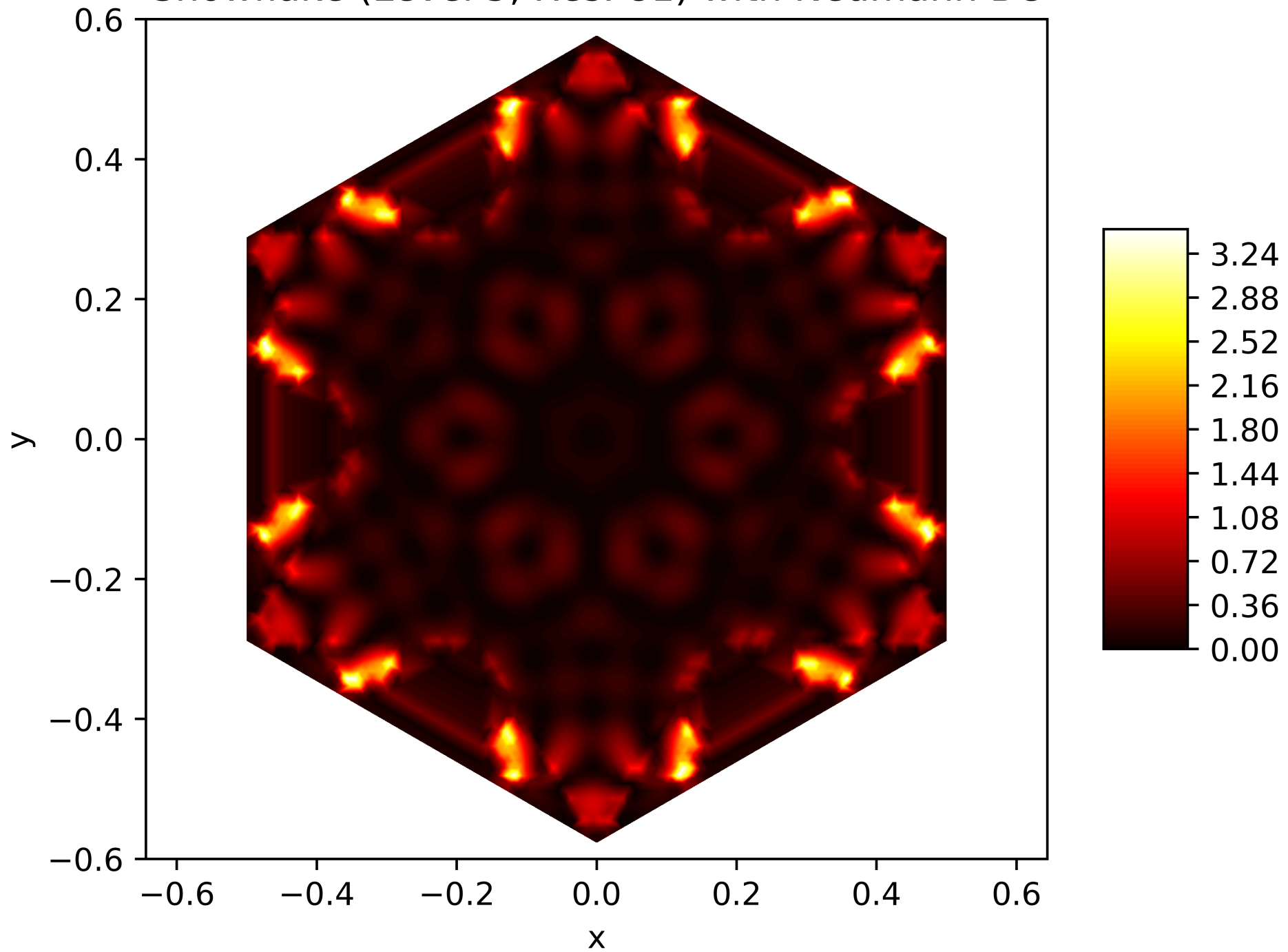
Energy Function of the 116. Eigenfunction on the Snowflake (Level 5, Res. 81) with Neumann BC
