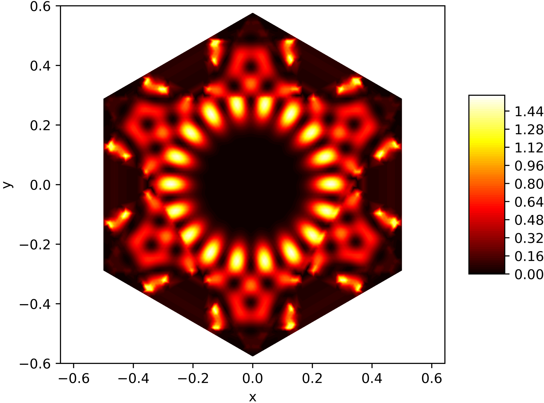
Energy Function of the 108. Eigenfunction on the Snowflake (Level 5, Res. 81) with Neumann BC
