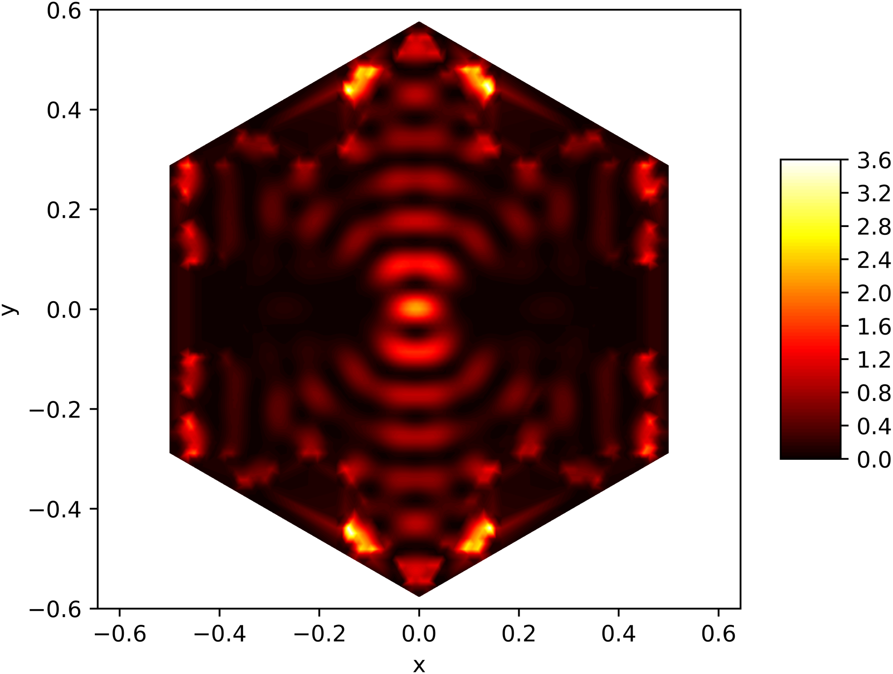
Energy Function of the 109. Eigenfunction on the Snowflake (Level 5, Res. 81) with Neumann BC
