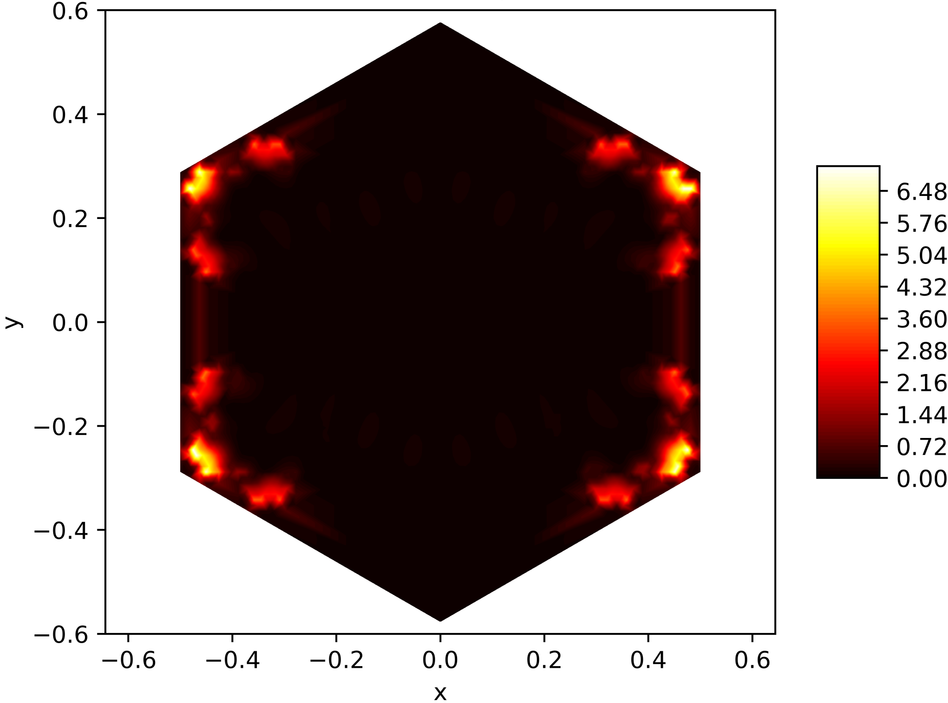
Energy Function of the 102. Eigenfunction on the Snowflake (Level 5, Res. 81) with Neumann BC
