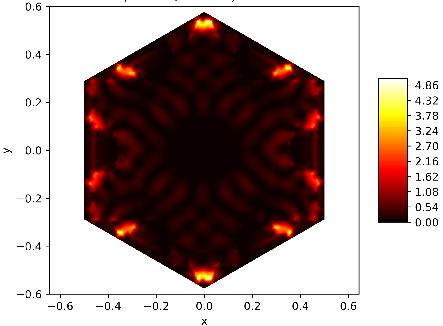
Energy Function of the 107. Eigenfunction on the Snowflake (Level 5, Res. 81) with Neumann BC
