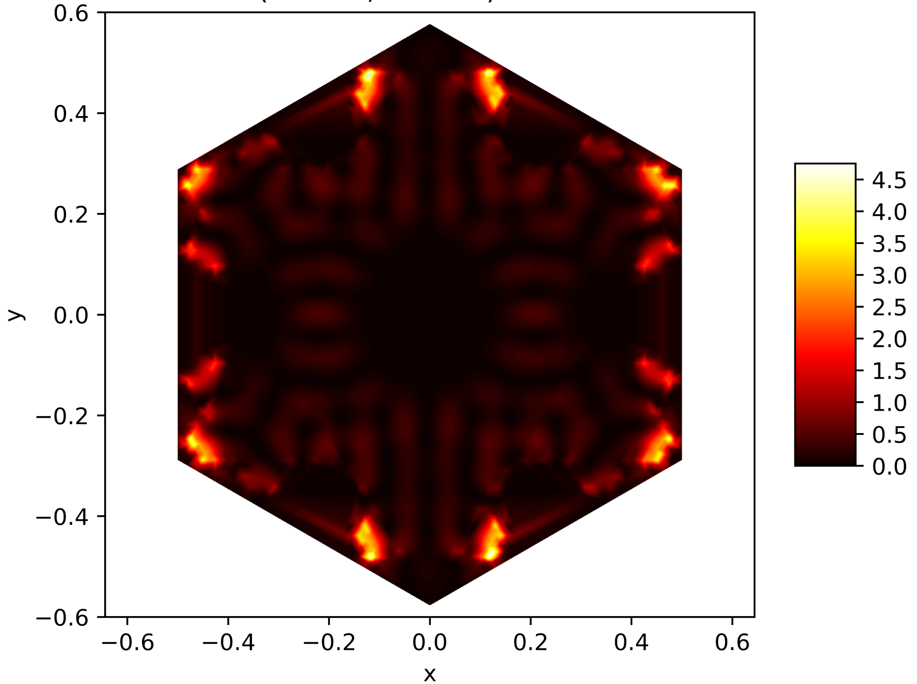
Energy Function of the 106. Eigenfunction on the Snowflake (Level 5, Res. 81) with Neumann BC
