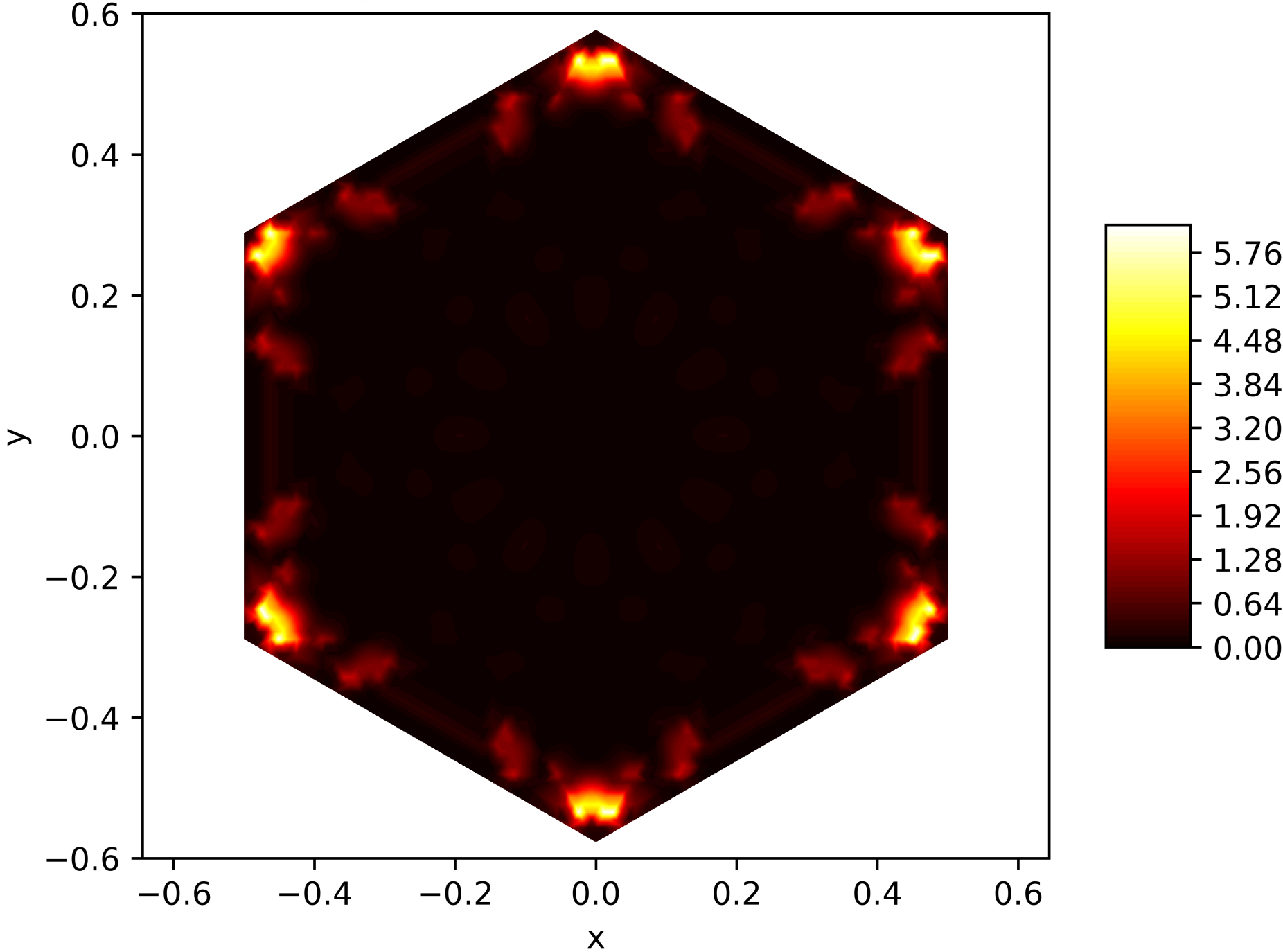
Energy Function of the 104. Eigenfunction on the Snowflake (Level 5, Res. 81) with Neumann BC
