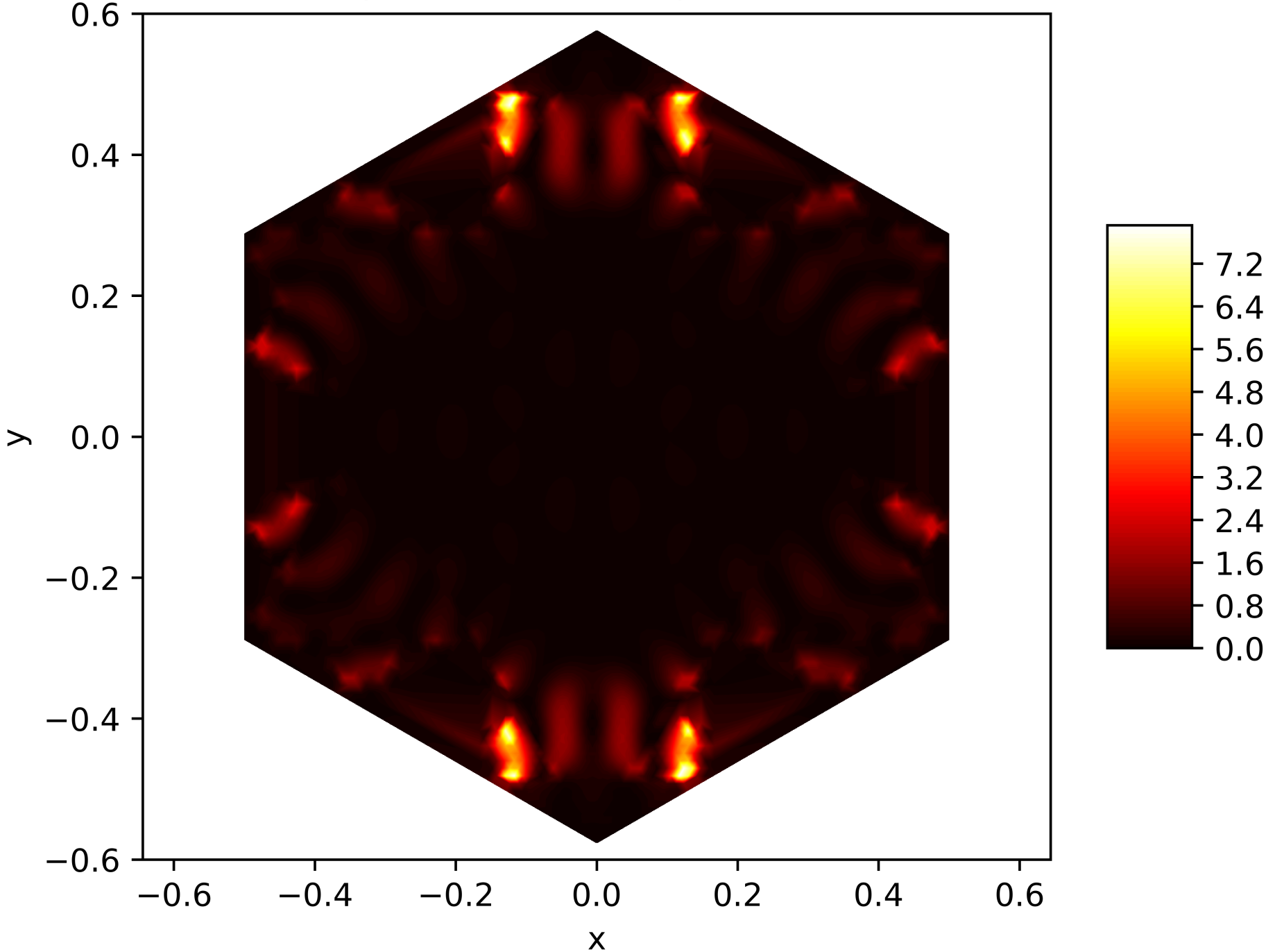
Energy Function of the 113. Eigenfunction on the Snowflake (Level 5, Res. 81) with Neumann BC
