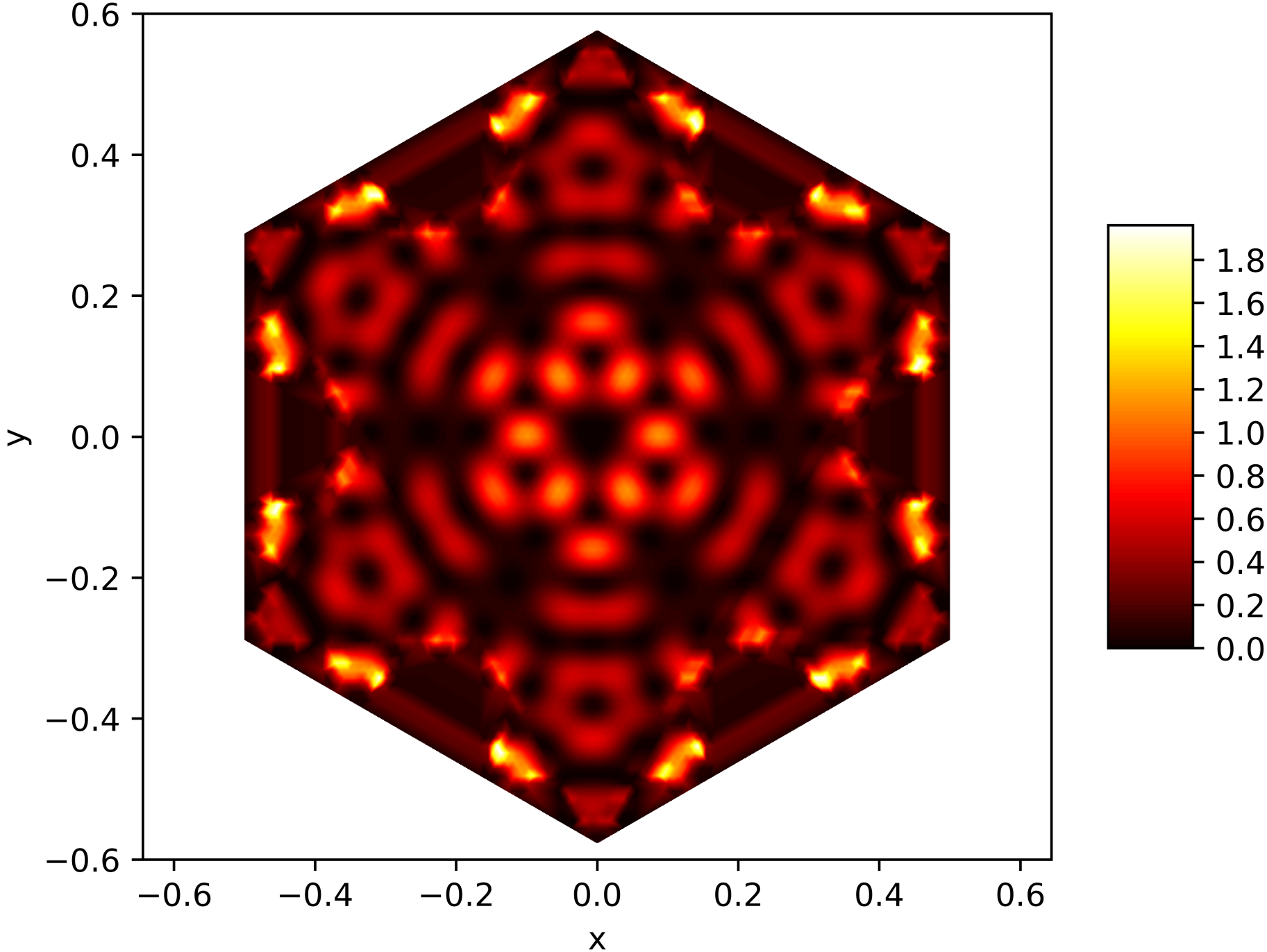
Energy Function of the 105. Eigenfunction on the Snowflake (Level 5, Res. 81) with Neumann BC
