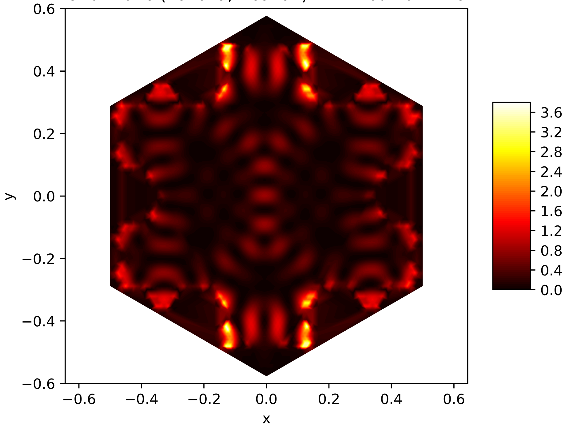
Energy Function of the 117. Eigenfunction on the Snowflake (Level 5, Res. 81) with Neumann BC
