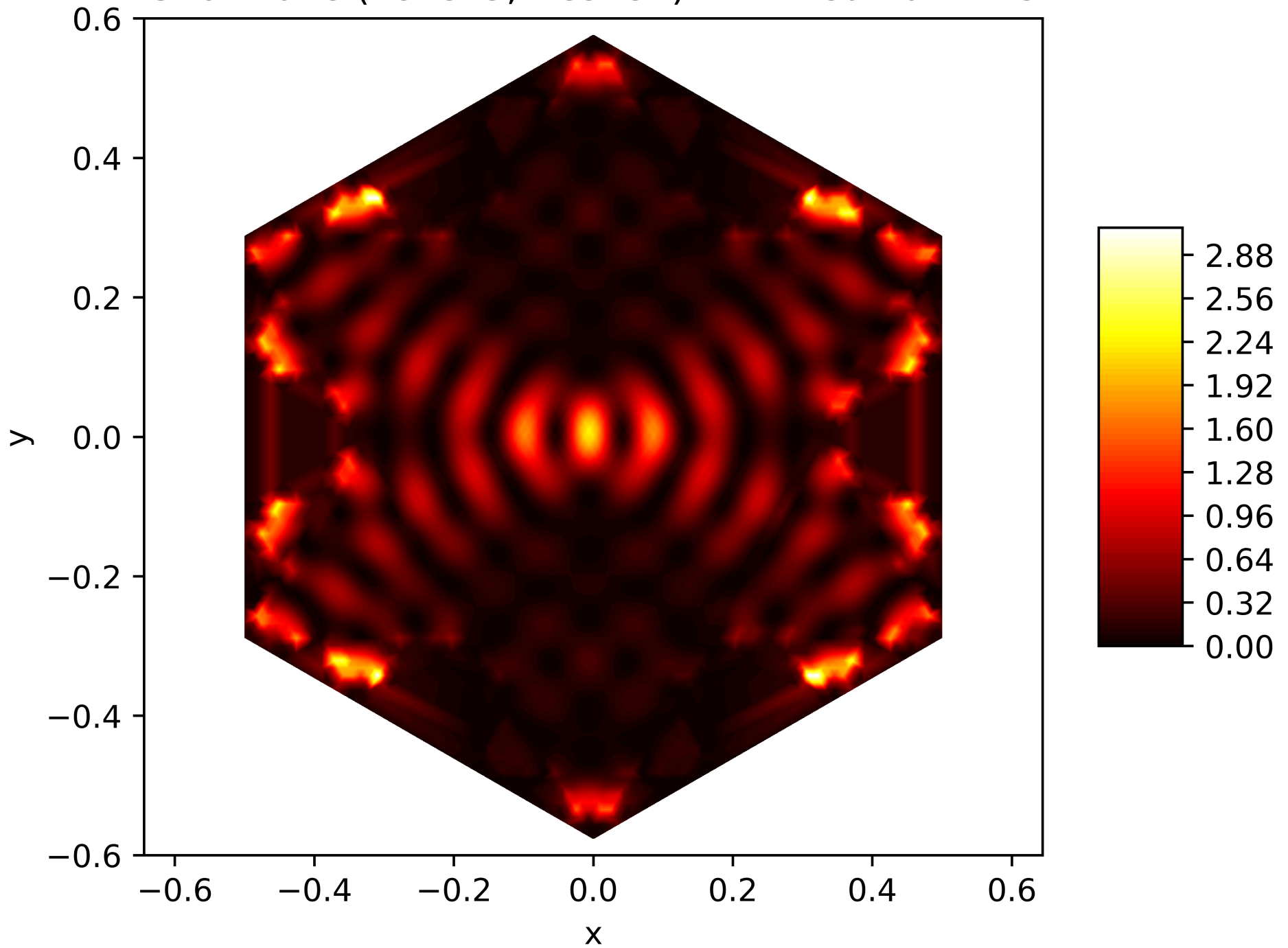
Energy Function of the 110. Eigenfunction on the Snowflake (Level 5, Res. 81) with Neumann BC
