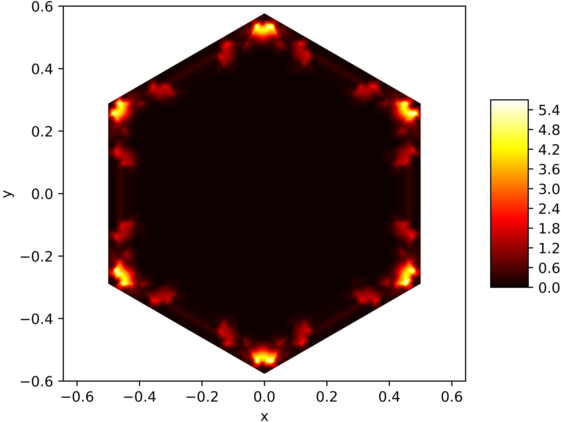
Energy Function of the 103. Eigenfunction on the Snowflake (Level 5, Res. 81) with Neumann BC
