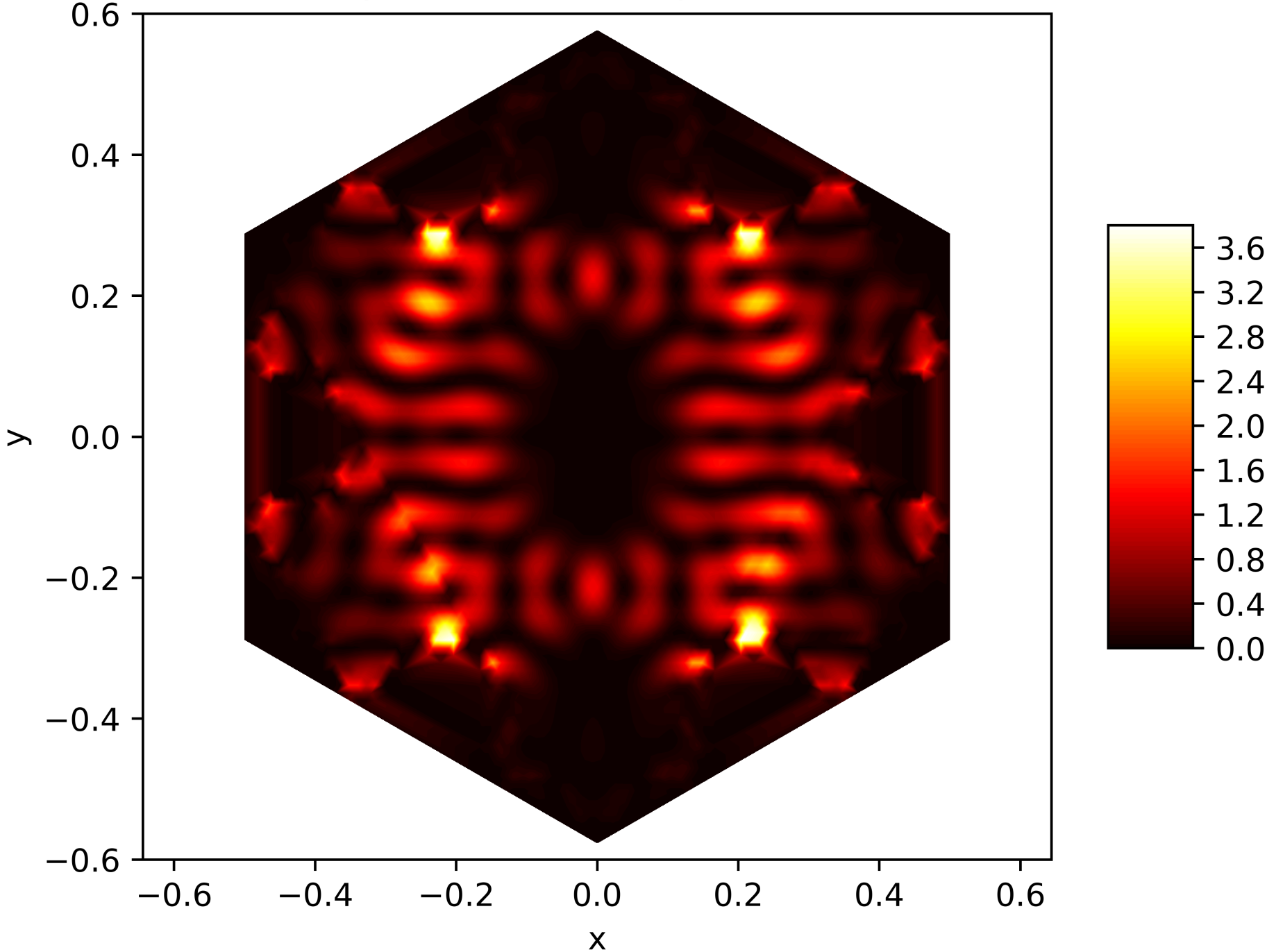
Energy Function of the 131. Eigenfunction on the Snowflake (Level 5, Res. 81) with Neumann BC
