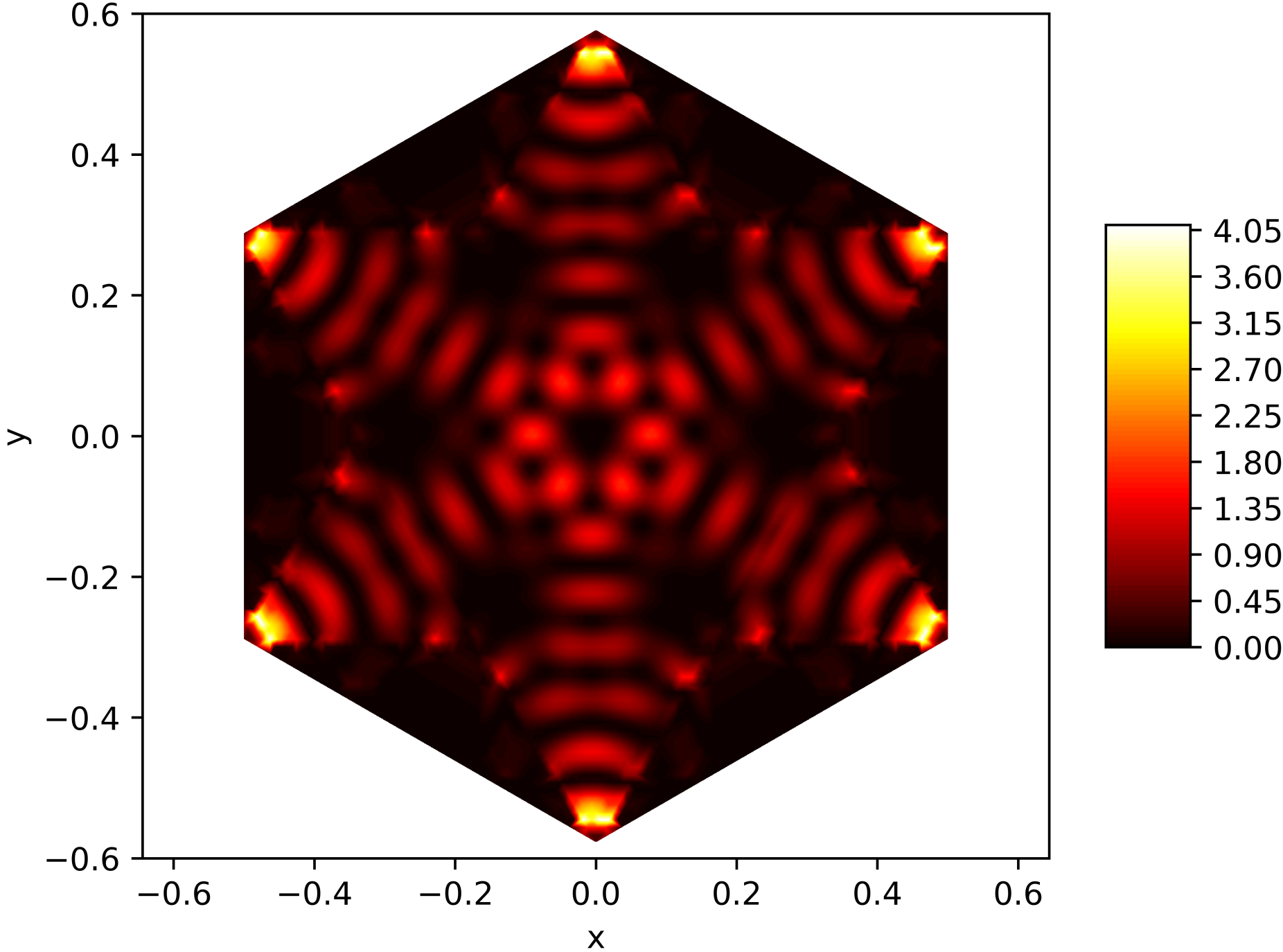
Energy Function of the 133. Eigenfunction on the Snowflake (Level 5, Res. 81) with Neumann BC
