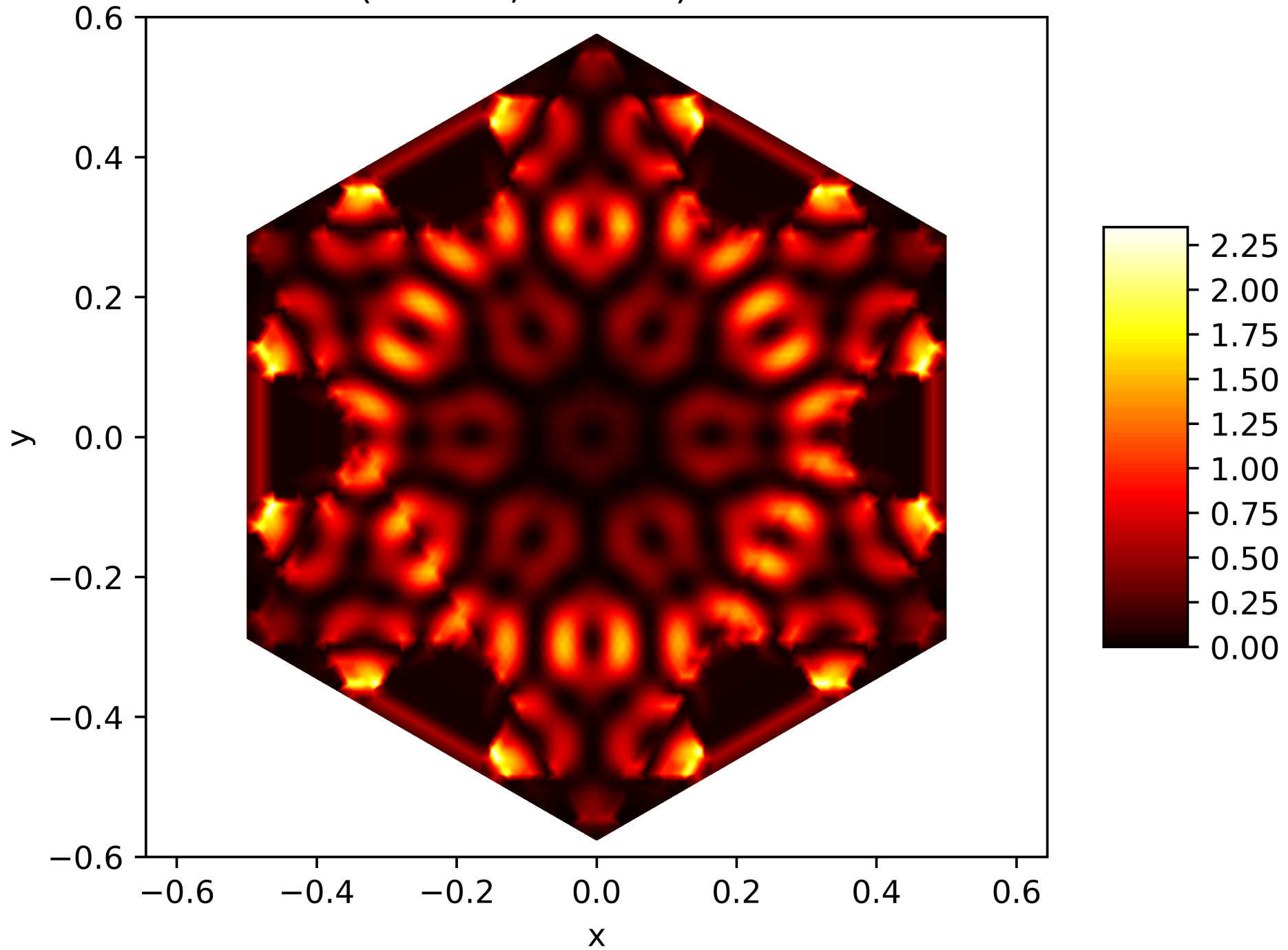
Energy Function of the 132. Eigenfunction on the Snowflake (Level 5, Res. 81) with Neumann BC
