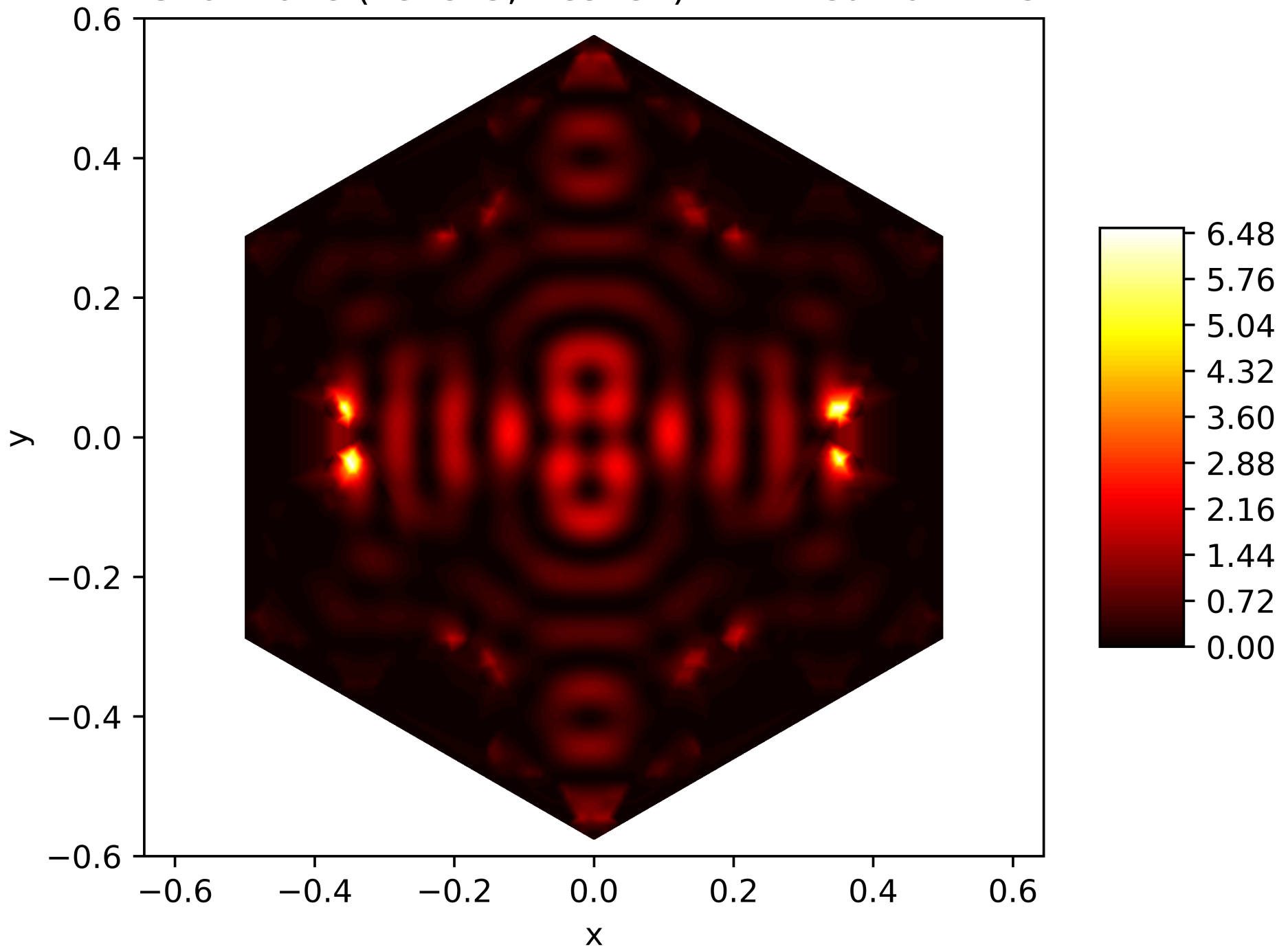
Energy Function of the 122. Eigenfunction on the Snowflake (Level 5, Res. 81) with Neumann BC
