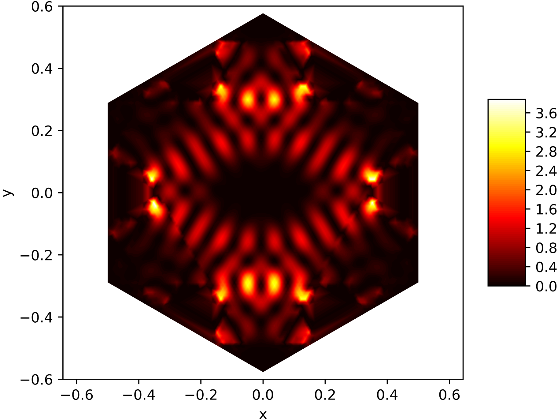
Energy Function of the 130. Eigenfunction on the Snowflake (Level 5, Res. 81) with Neumann BC
