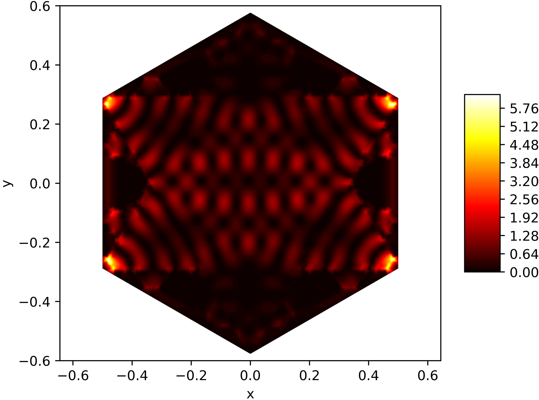
Energy Function of the 137. Eigenfunction on the Snowflake (Level 5, Res. 81) with Neumann BC
