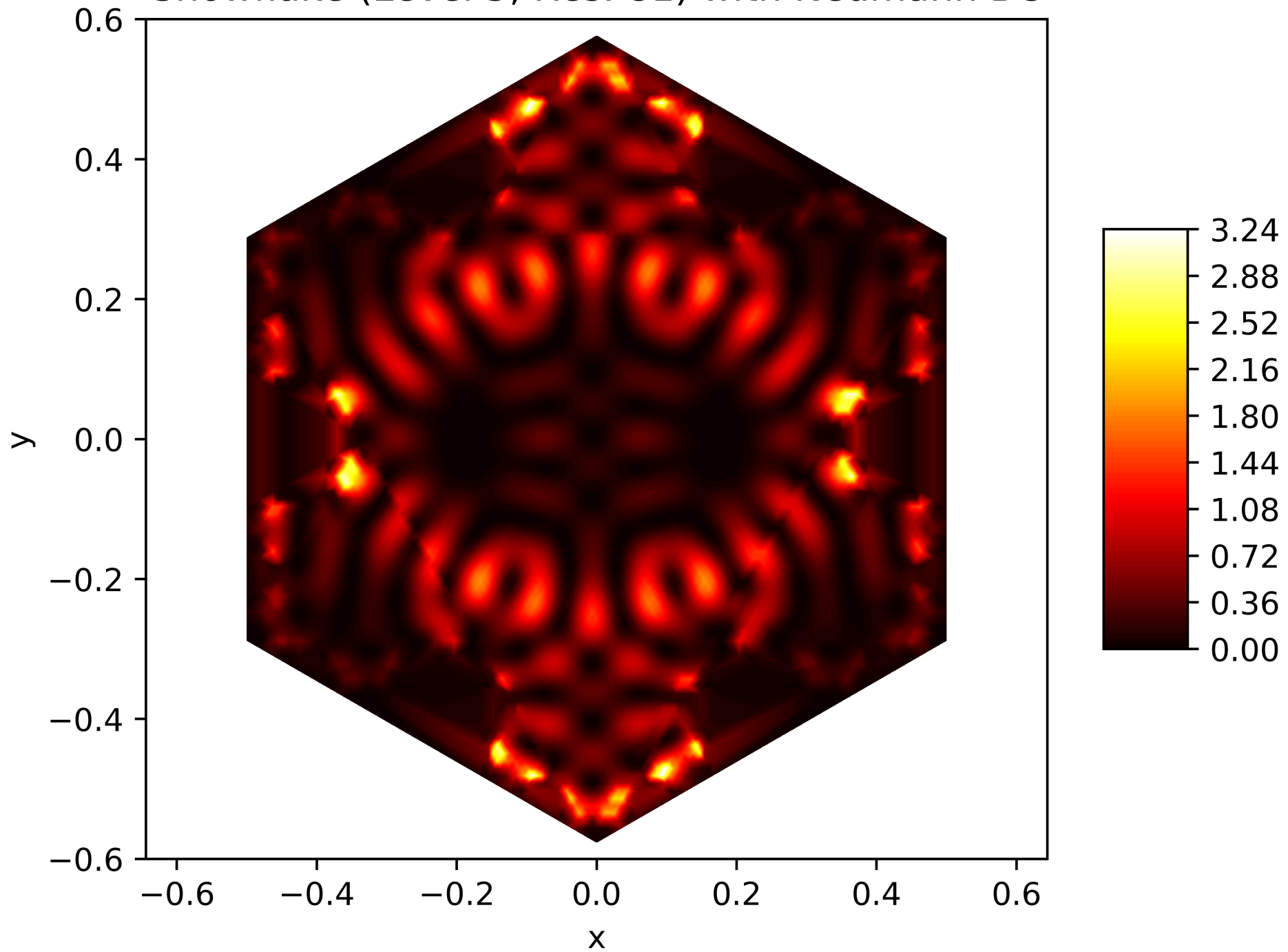
Energy Function of the 128. Eigenfunction on the Snowflake (Level 5, Res. 81) with Neumann BC
