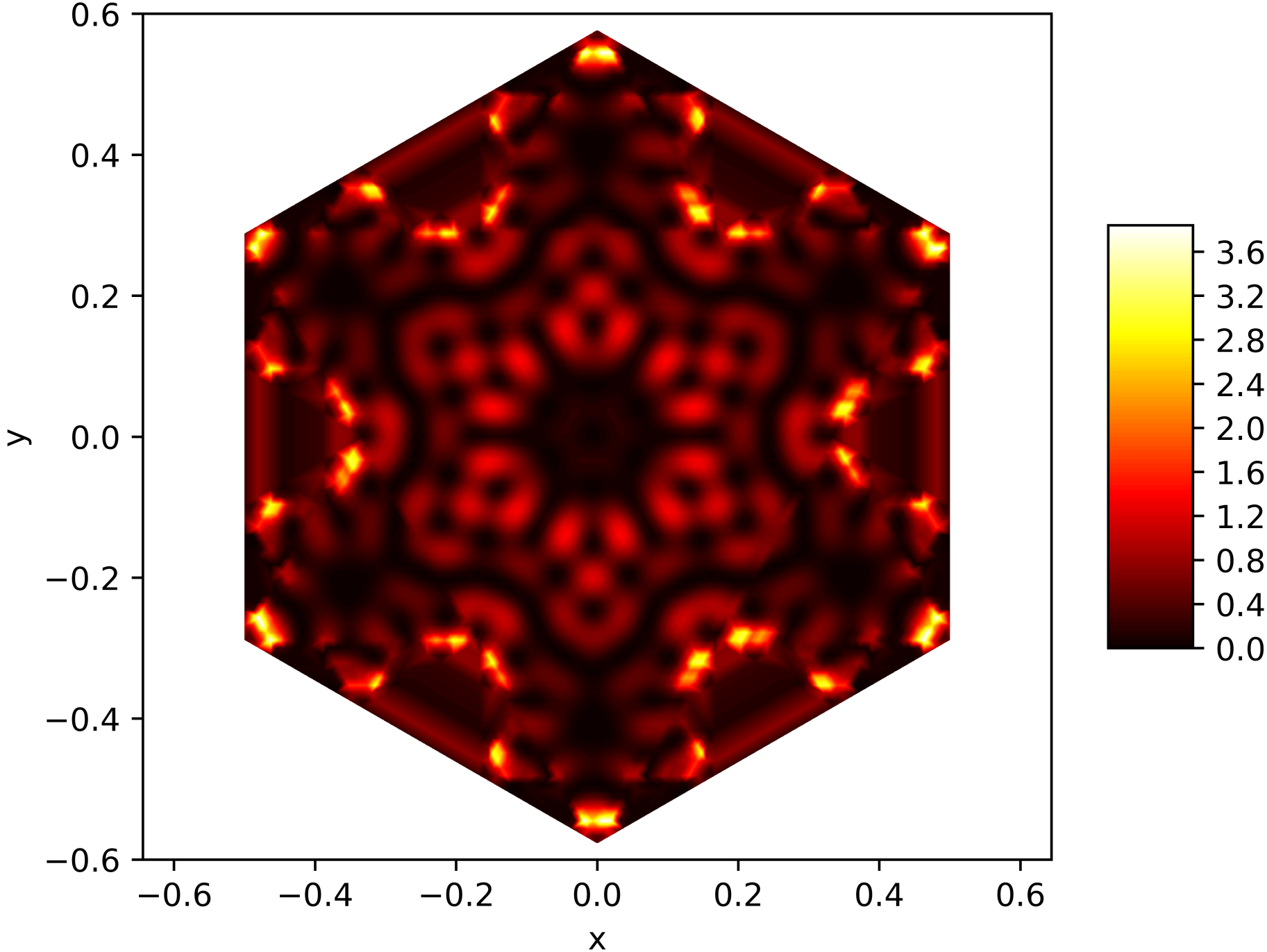
Energy Function of the 158. Eigenfunction on the Snowflake (Level 5, Res. 81) with Neumann BC
