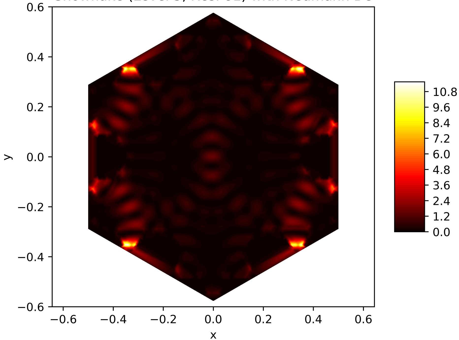
Energy Function of the 151. Eigenfunction on the Snowflake (Level 5, Res. 81) with Neumann BC
