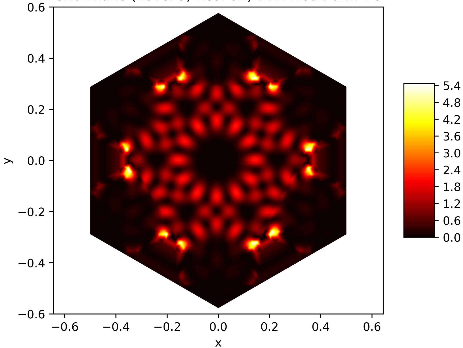
Energy Function of the 159. Eigenfunction on the Snowflake (Level 5, Res. 81) with Neumann BC
