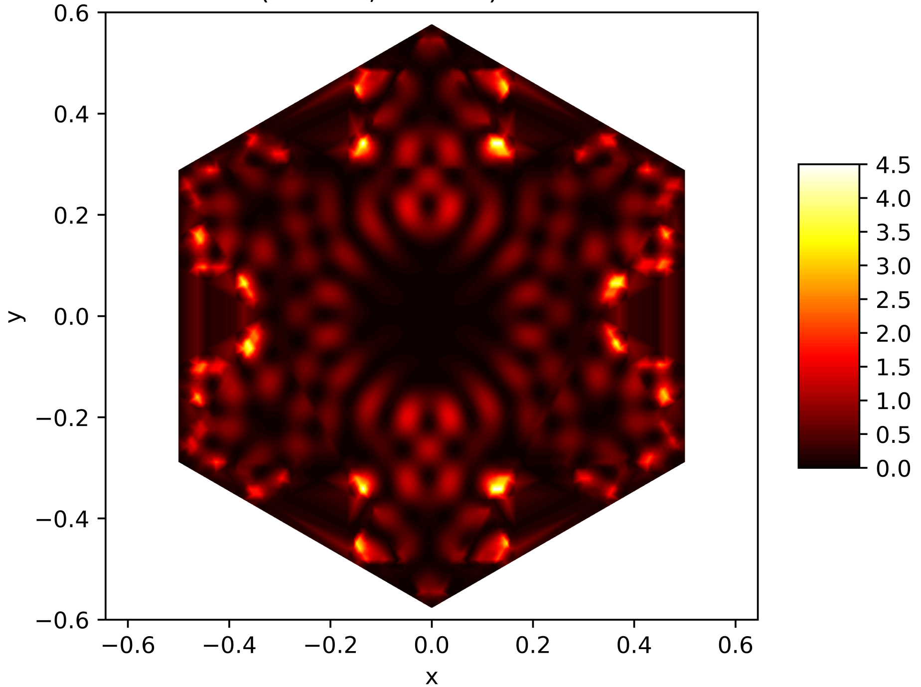
Energy Function of the 142. Eigenfunction on the Snowflake (Level 5, Res. 81) with Neumann BC
