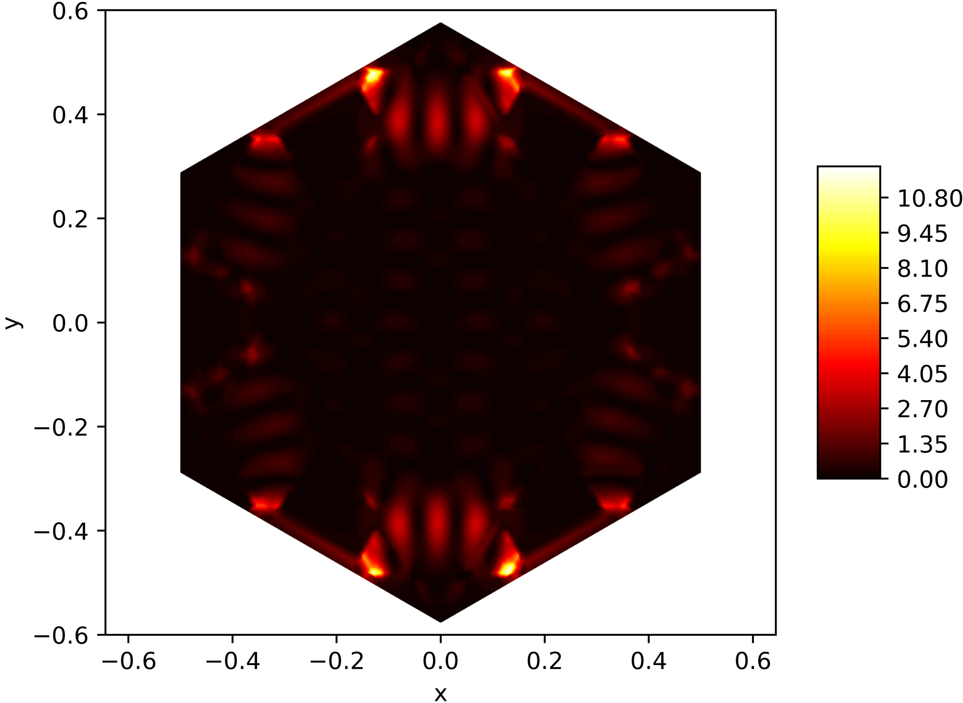
Energy Function of the 148. Eigenfunction on the Snowflake (Level 5, Res. 81) with Neumann BC
