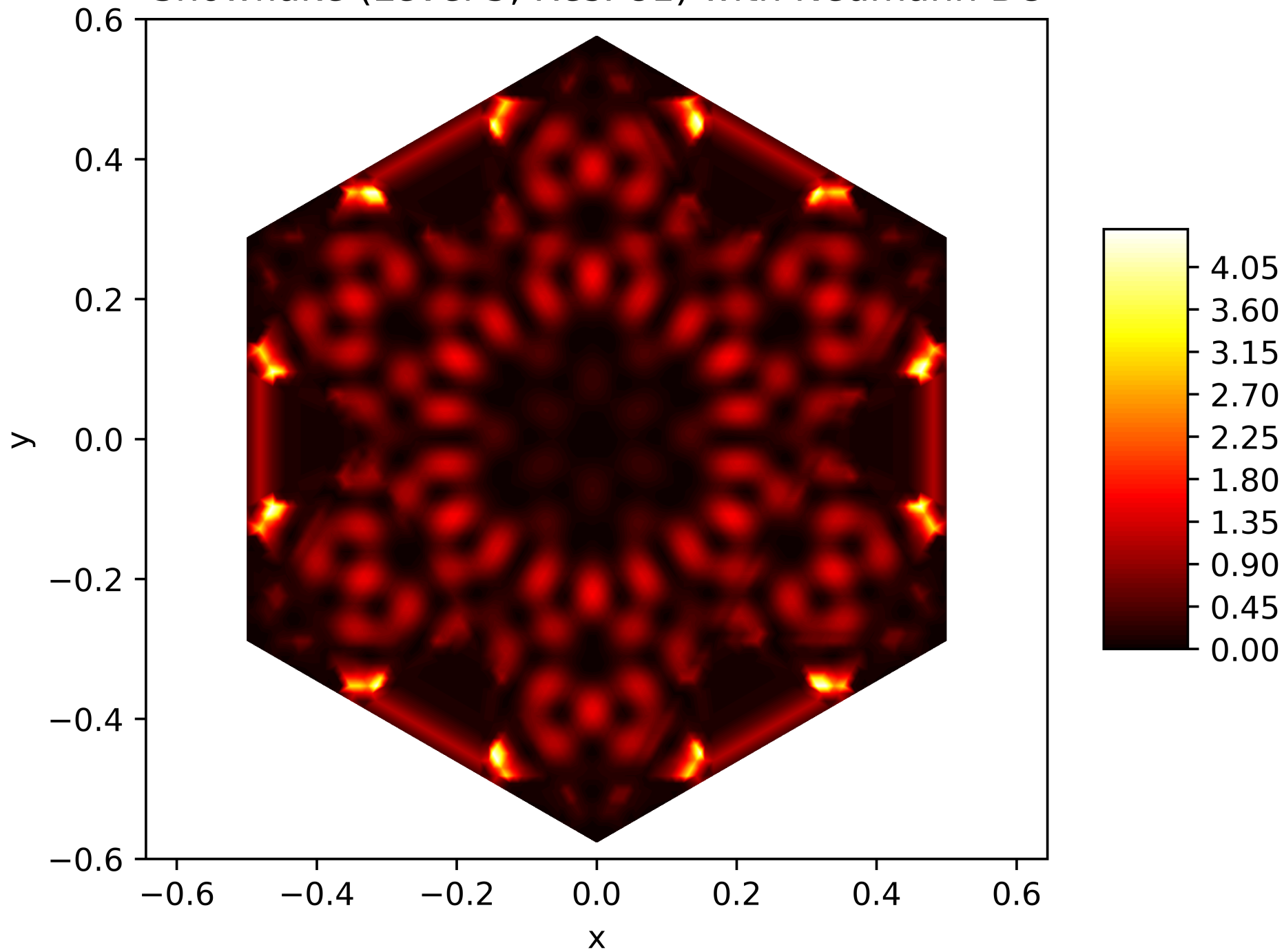
Energy Function of the 155. Eigenfunction on the Snowflake (Level 5, Res. 81) with Neumann BC
