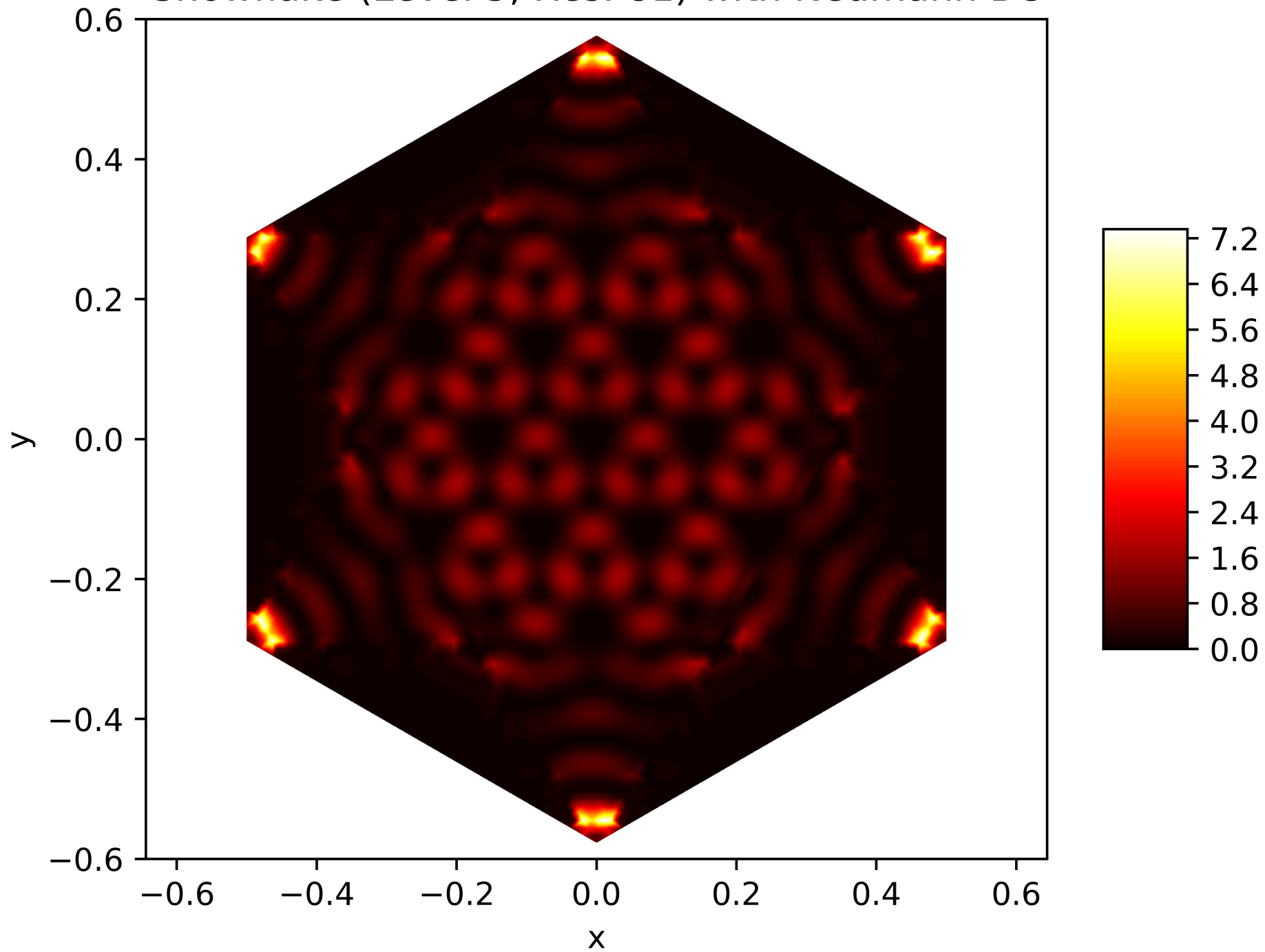
Energy Function of the 156. Eigenfunction on the Snowflake (Level 5, Res. 81) with Neumann BC
