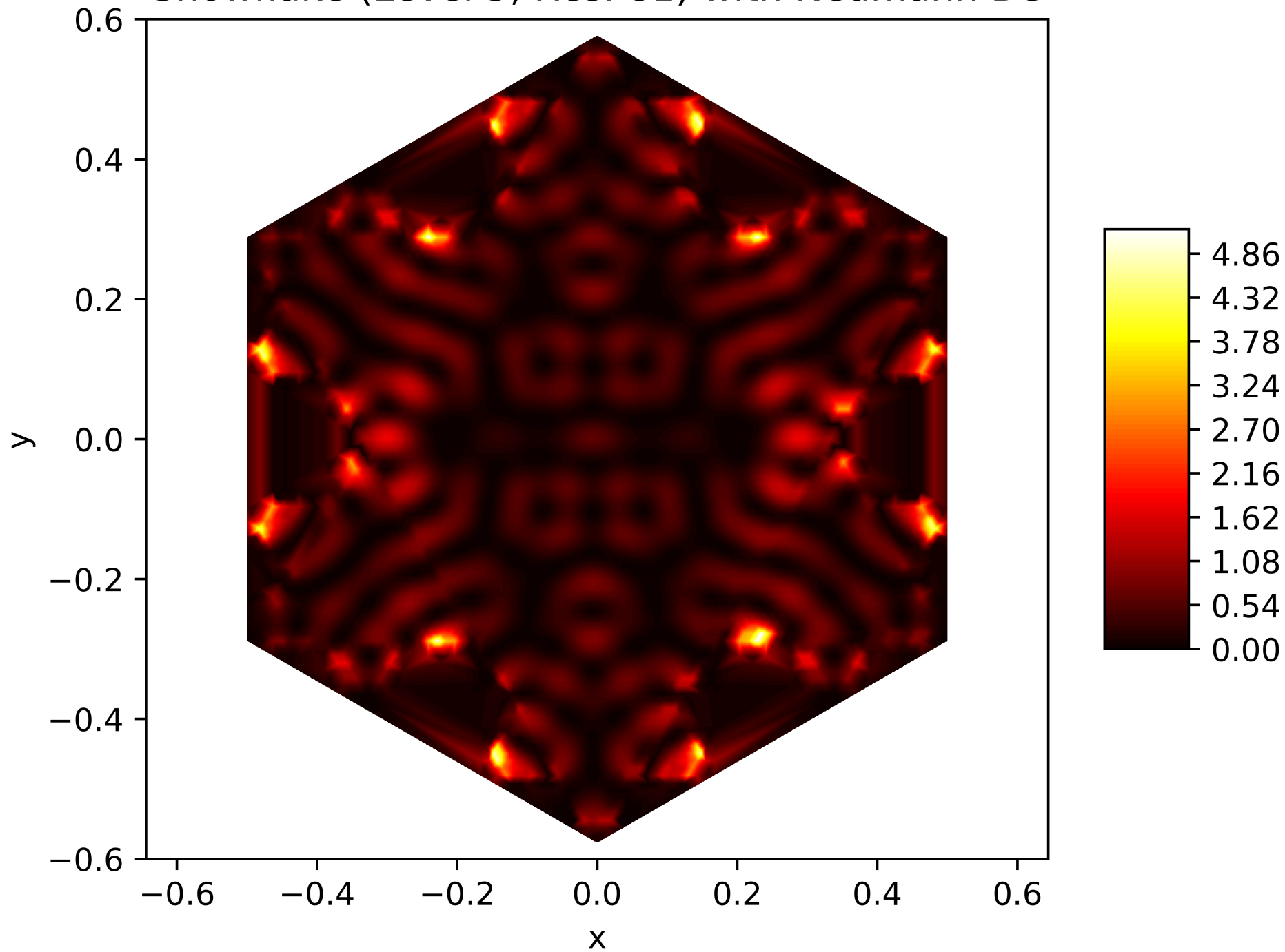
Energy Function of the 147. Eigenfunction on the Snowflake (Level 5, Res. 81) with Neumann BC
