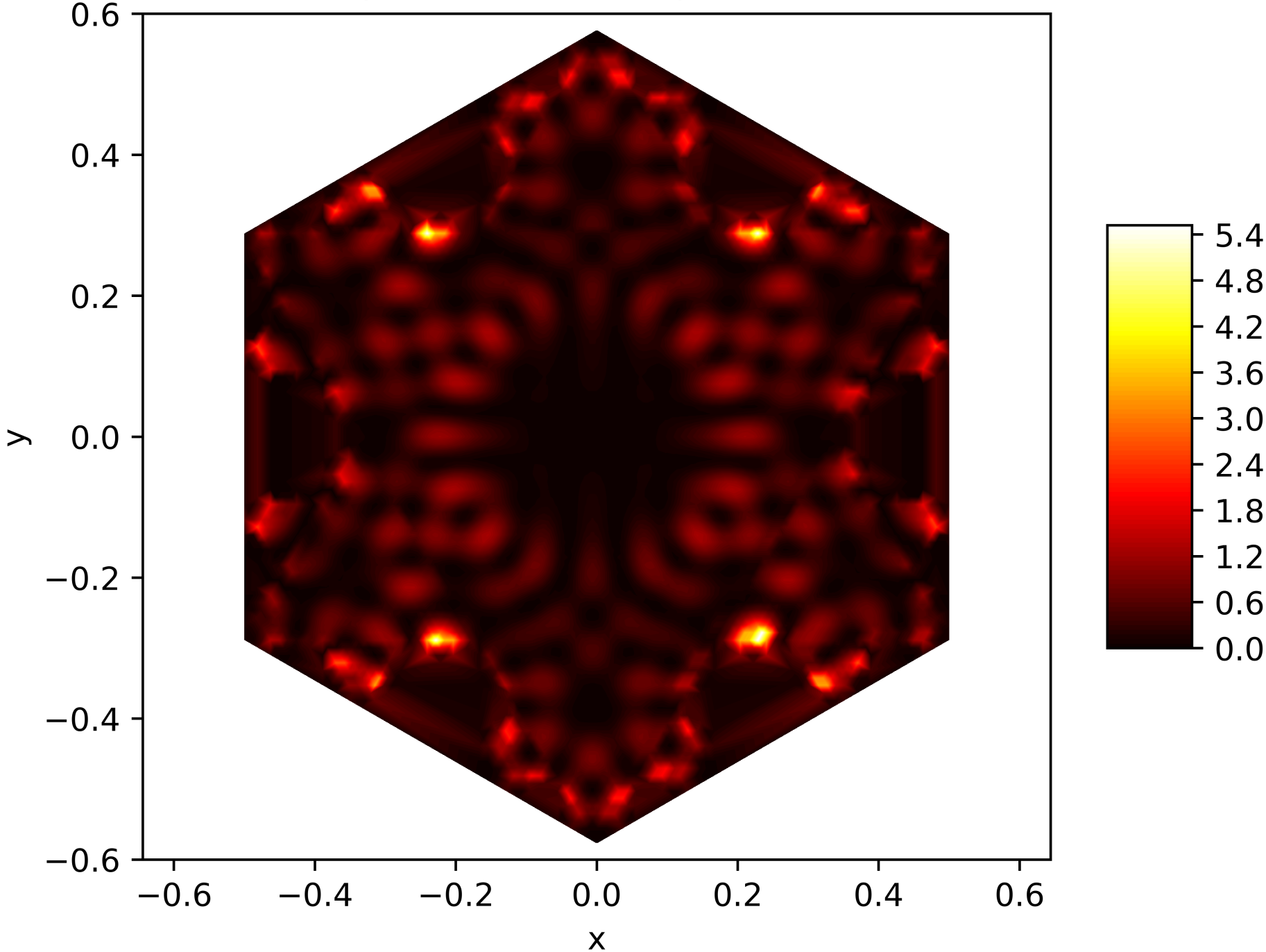
Energy Function of the 141. Eigenfunction on the Snowflake (Level 5, Res. 81) with Neumann BC
