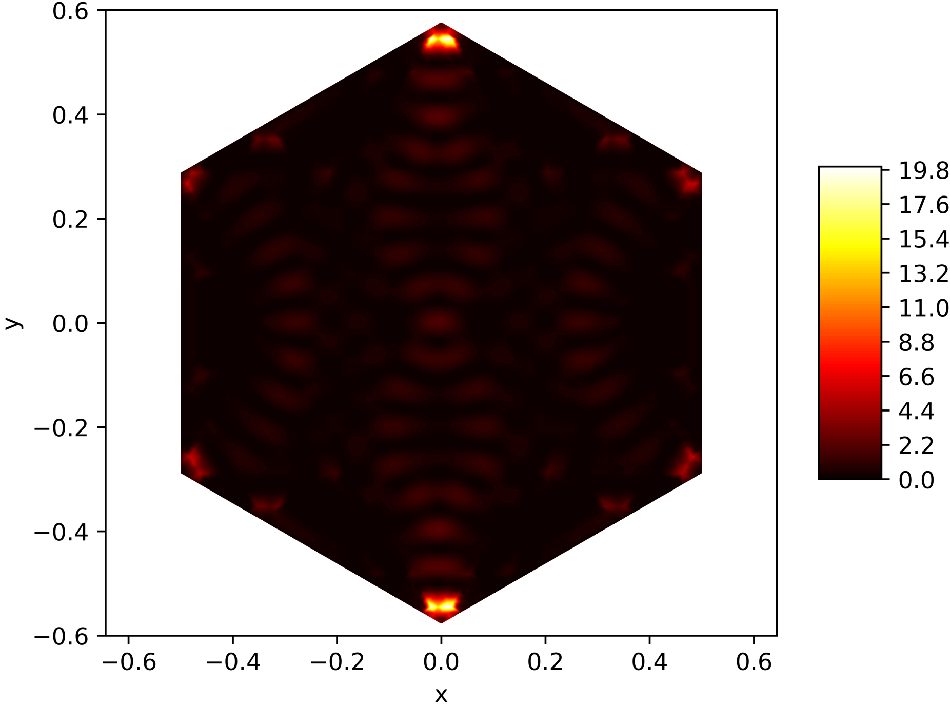
Energy Function of the 160. Eigenfunction on the Snowflake (Level 5, Res. 81) with Neumann BC
