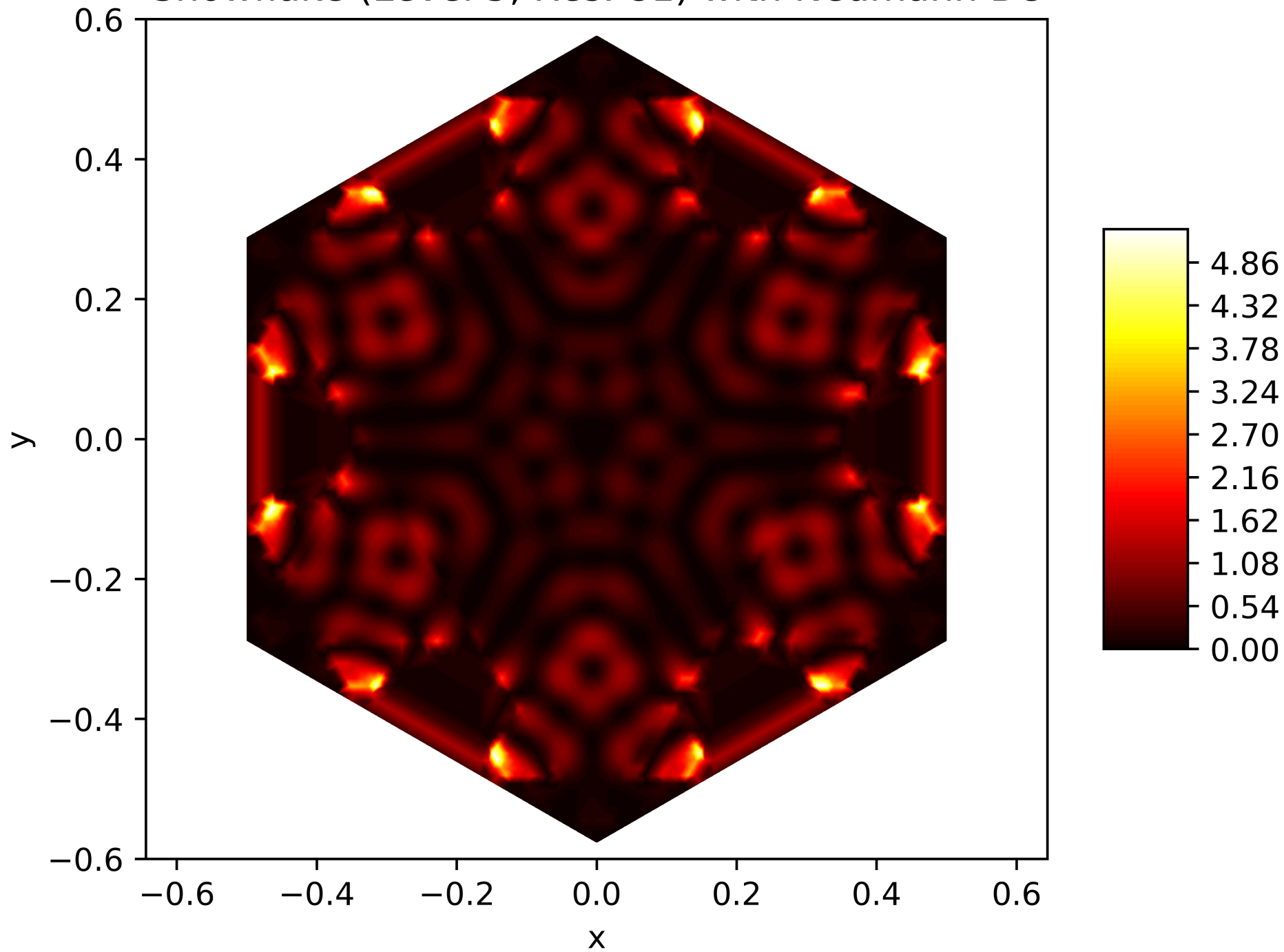
Energy Function of the 144. Eigenfunction on the Snowflake (Level 5, Res. 81) with Neumann BC
