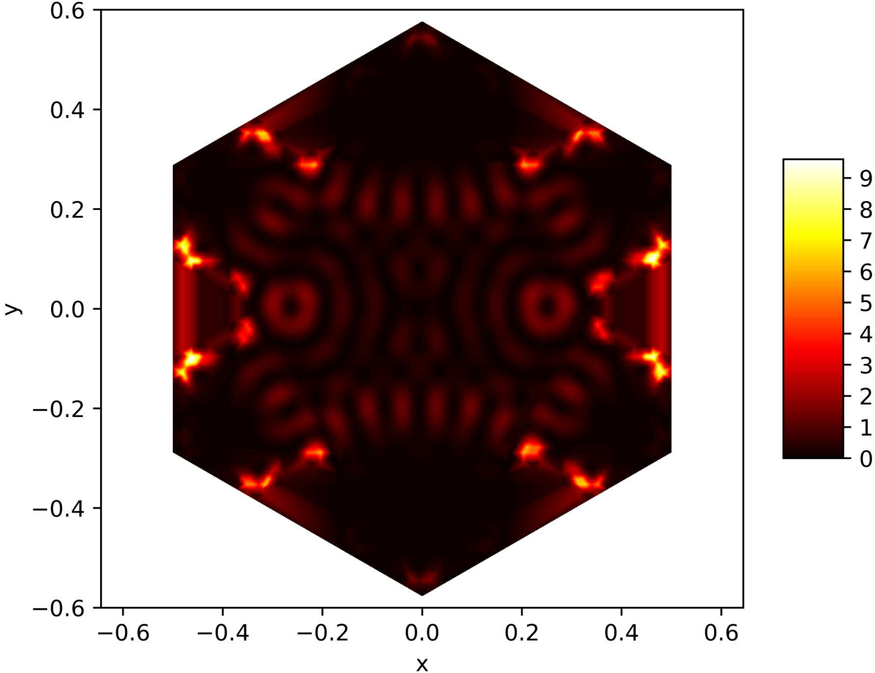
Energy Function of the 177. Eigenfunction on the Snowflake (Level 5, Res. 81) with Neumann BC
