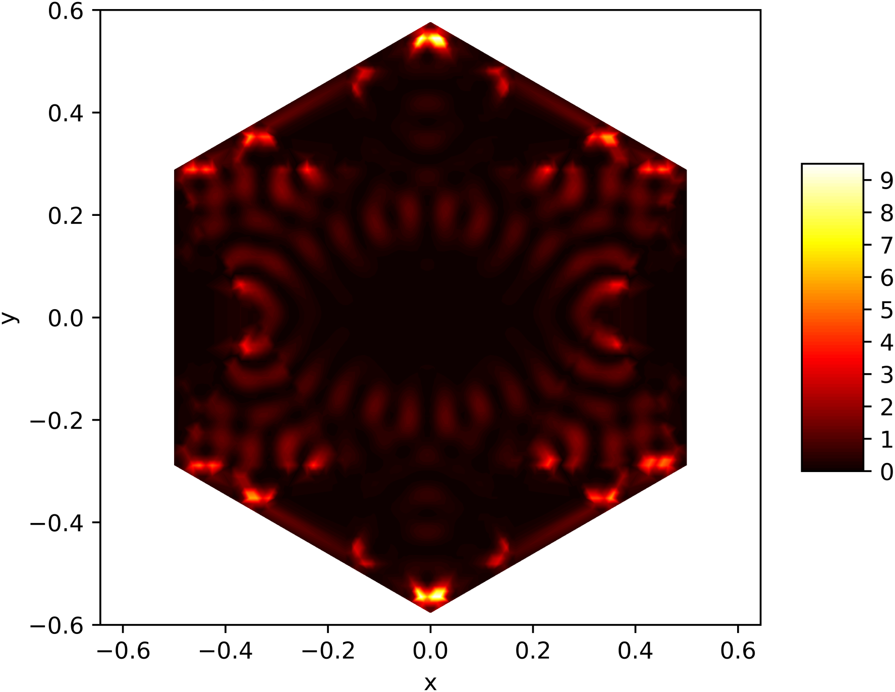
Energy Function of the 174. Eigenfunction on the Snowflake (Level 5, Res. 81) with Neumann BC
