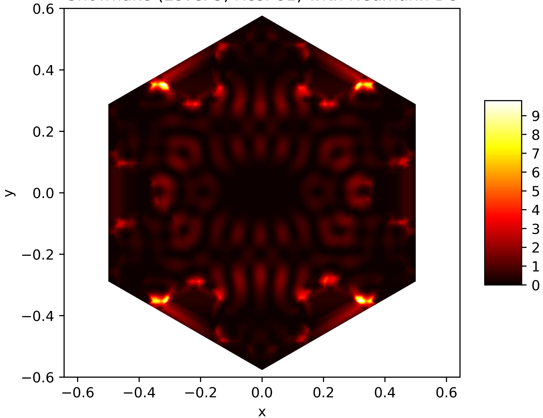
Energy Function of the 165. Eigenfunction on the Snowflake (Level 5, Res. 81) with Neumann BC
