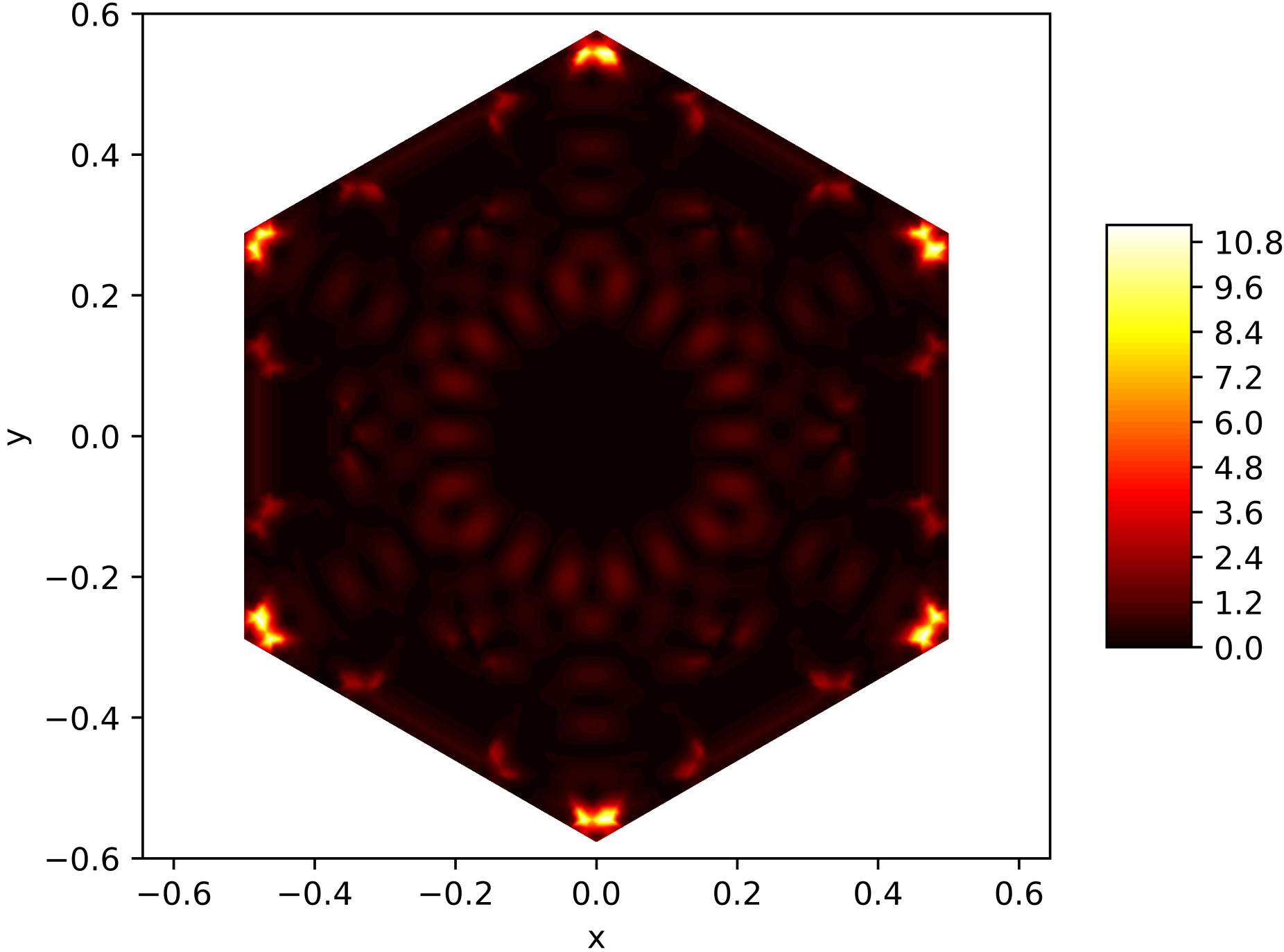
Energy Function of the 169. Eigenfunction on the Snowflake (Level 5, Res. 81) with Neumann BC
