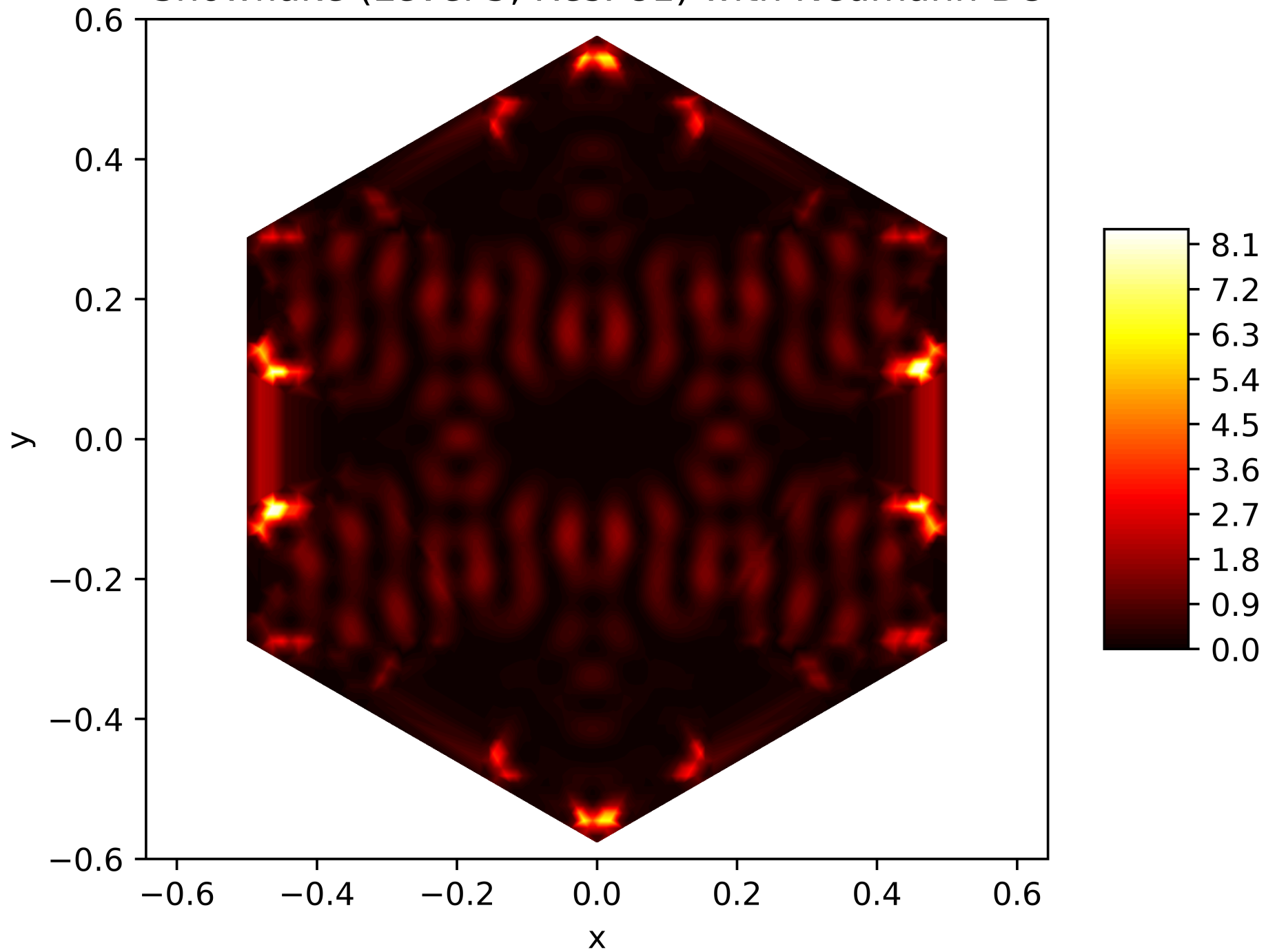
Energy Function of the 171. Eigenfunction on the Snowflake (Level 5, Res. 81) with Neumann BC
