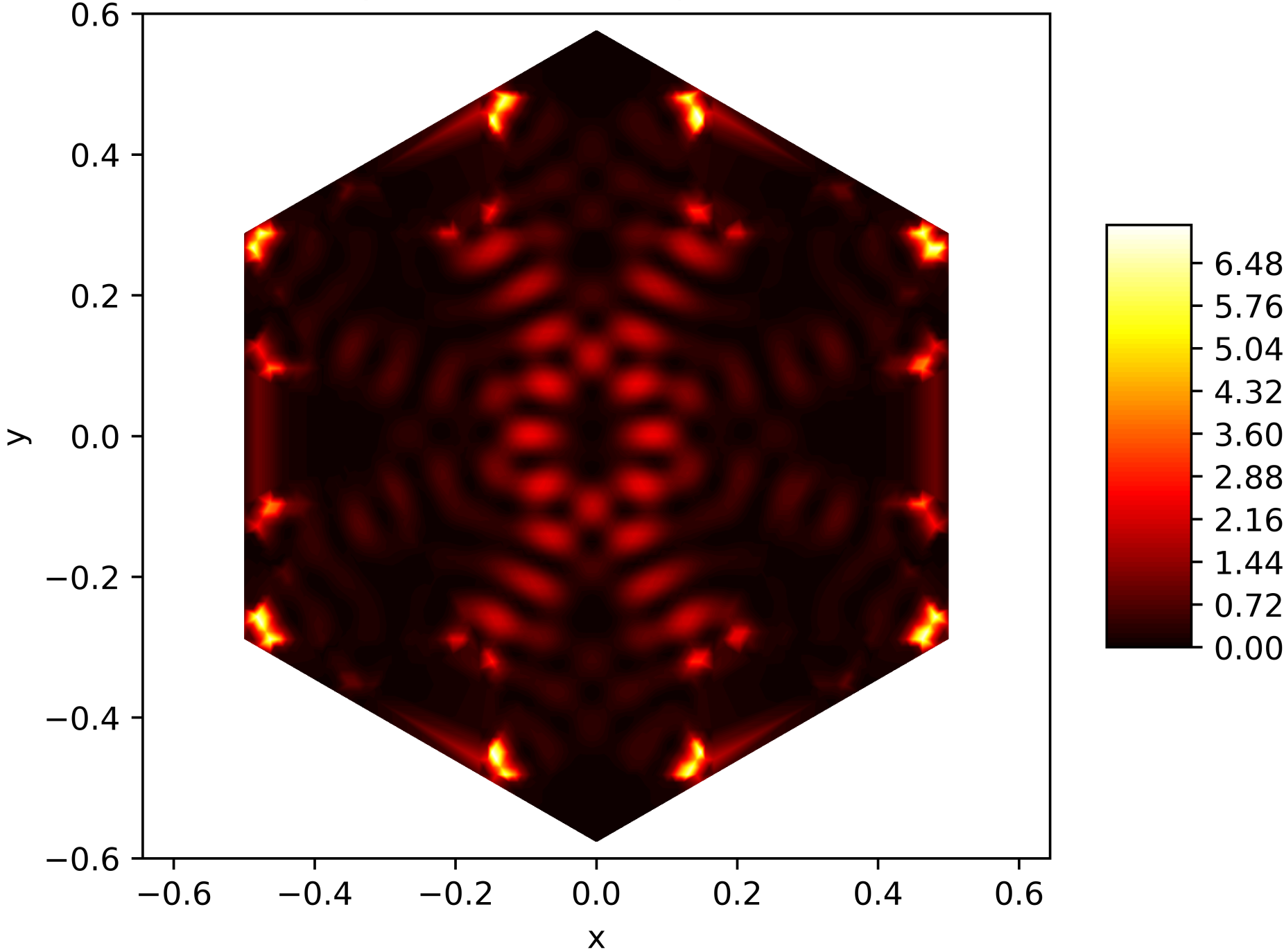
Energy Function of the 163. Eigenfunction on the Snowflake (Level 5, Res. 81) with Neumann BC
