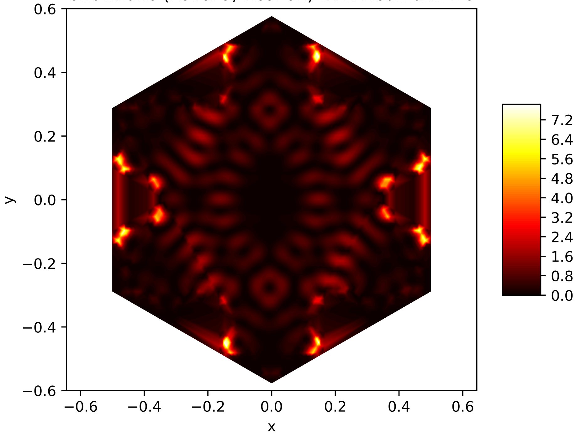
Energy Function of the 166. Eigenfunction on the Snowflake (Level 5, Res. 81) with Neumann BC
