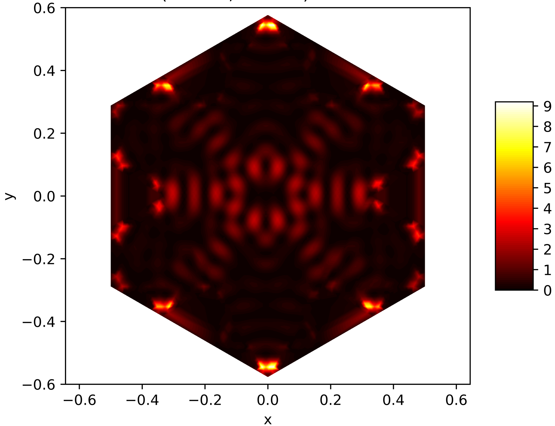
Energy Function of the 162. Eigenfunction on the Snowflake (Level 5, Res. 81) with Neumann BC
