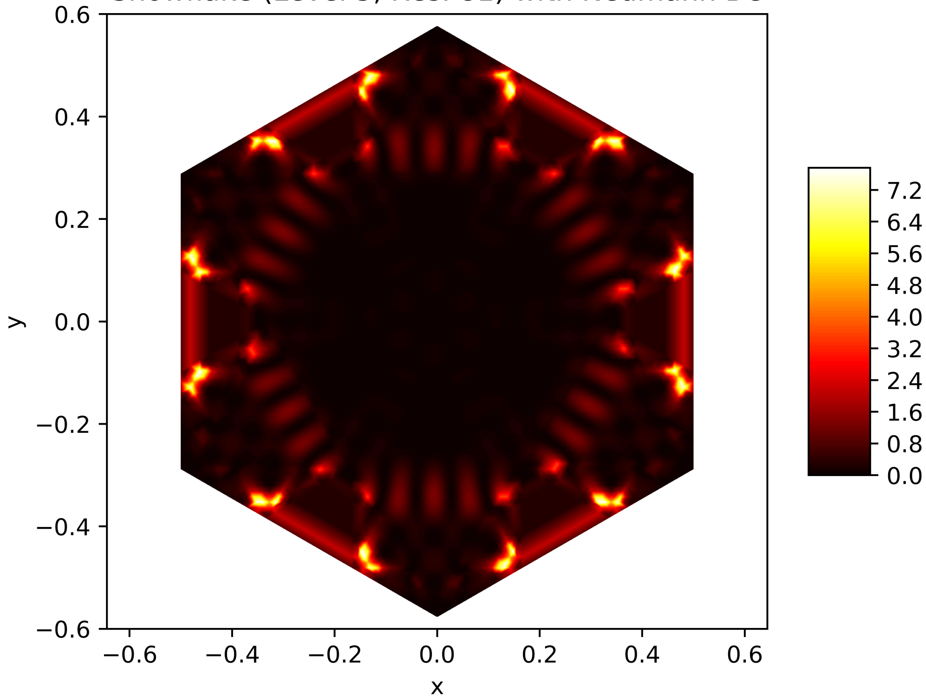
Energy Function of the 175. Eigenfunction on the Snowflake (Level 5, Res. 81) with Neumann BC
