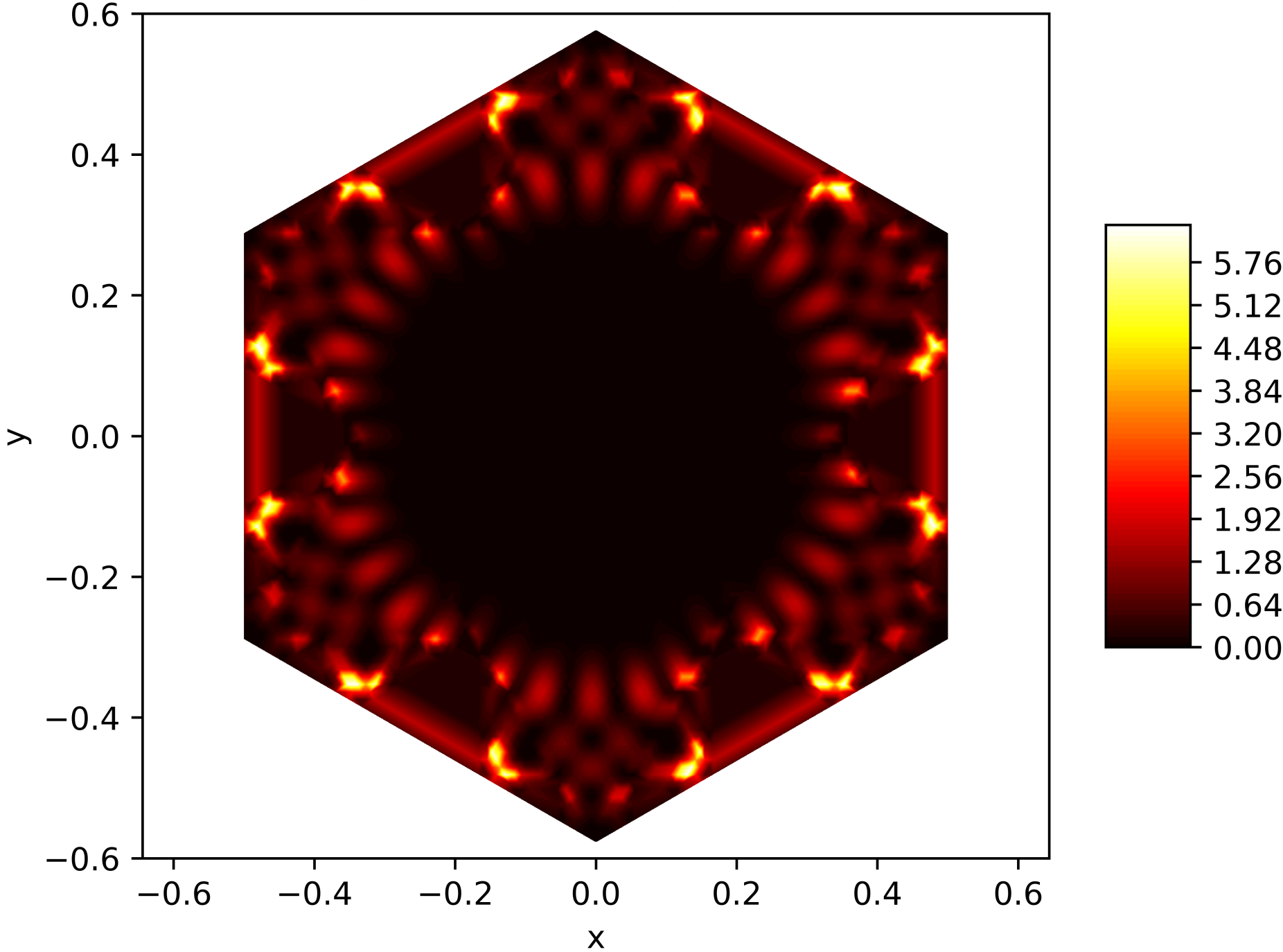
Energy Function of the 178. Eigenfunction on the Snowflake (Level 5, Res. 81) with Neumann BC
