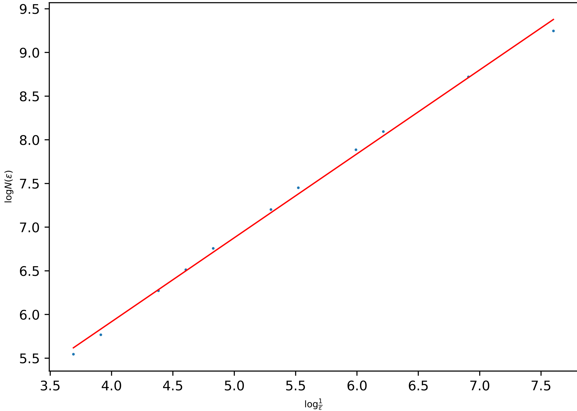
Power-Law of the BC-Dimension of the Snowflake (Level 4): 0.9611749645220451
