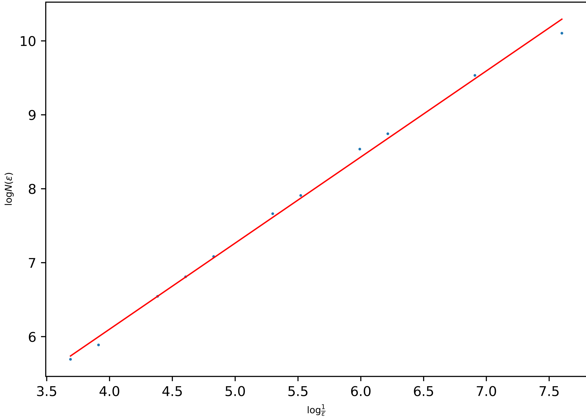
Power-Law of the BC-Dimension of the Snowflake (Level 7): 1.1642165940166977
