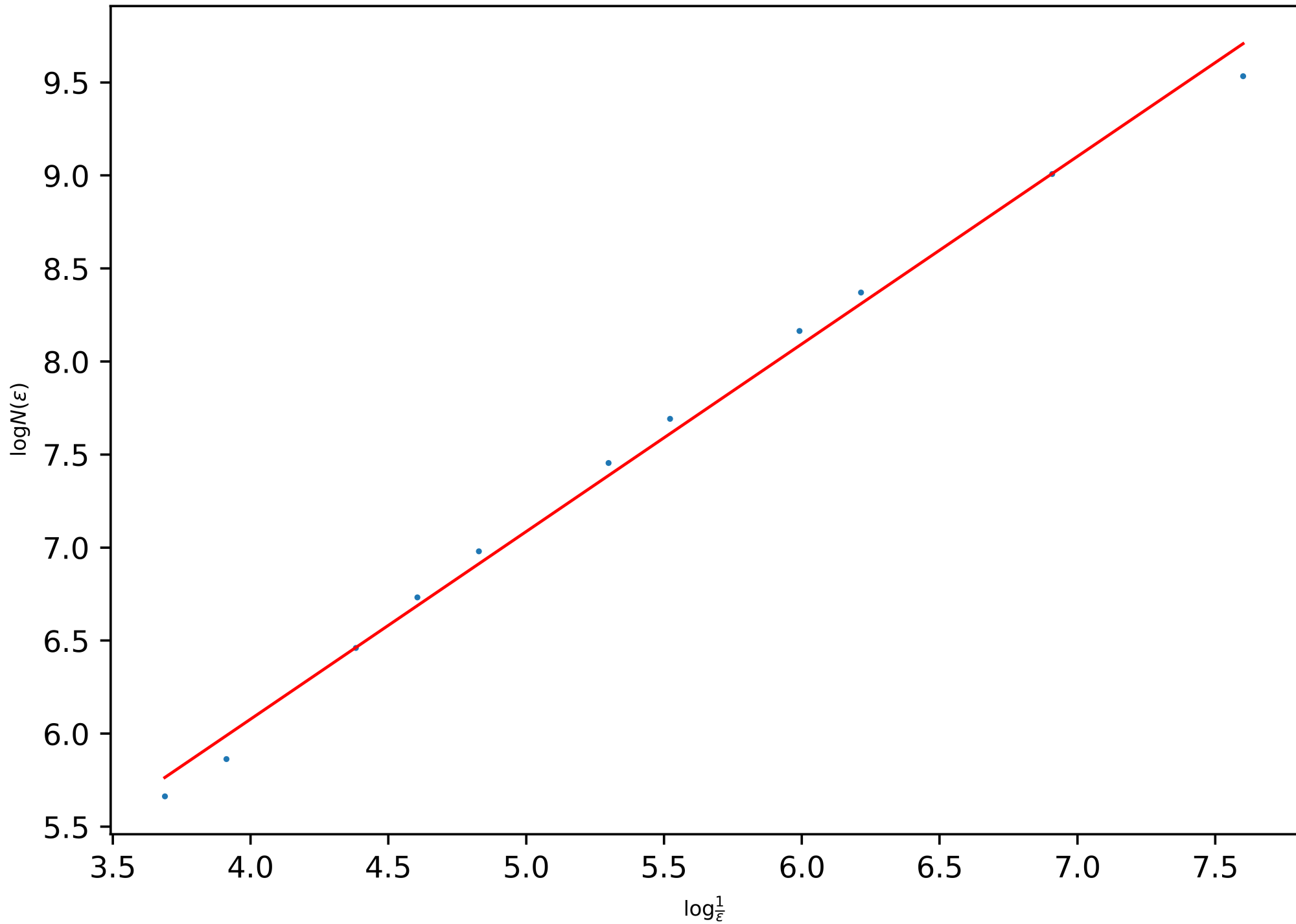
Power-Law of the BC-Dimension of the Snowflake (Level 5): 1.0082130670624296
