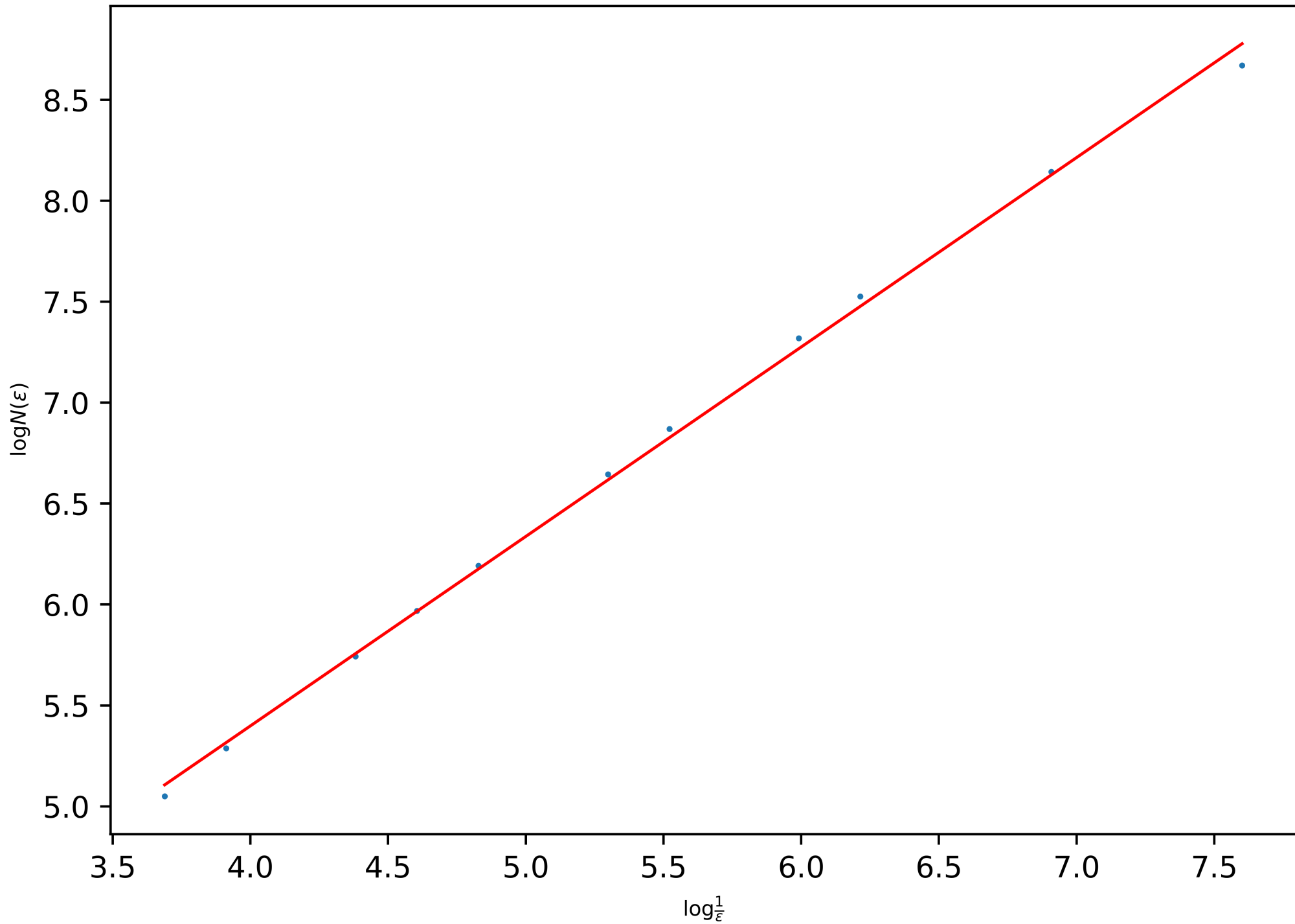
Power-Law of the BC-Dimension of the Snowflake (Level 2): 0.9385755538464642
