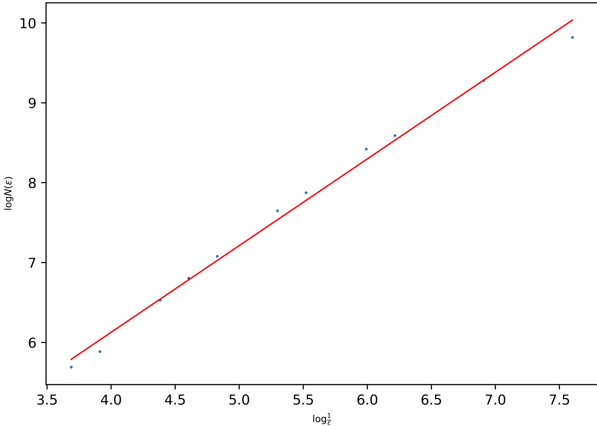
Power-Law of the BC-Dimension of the Snowflake (Level 6): 1.0854098816515818
