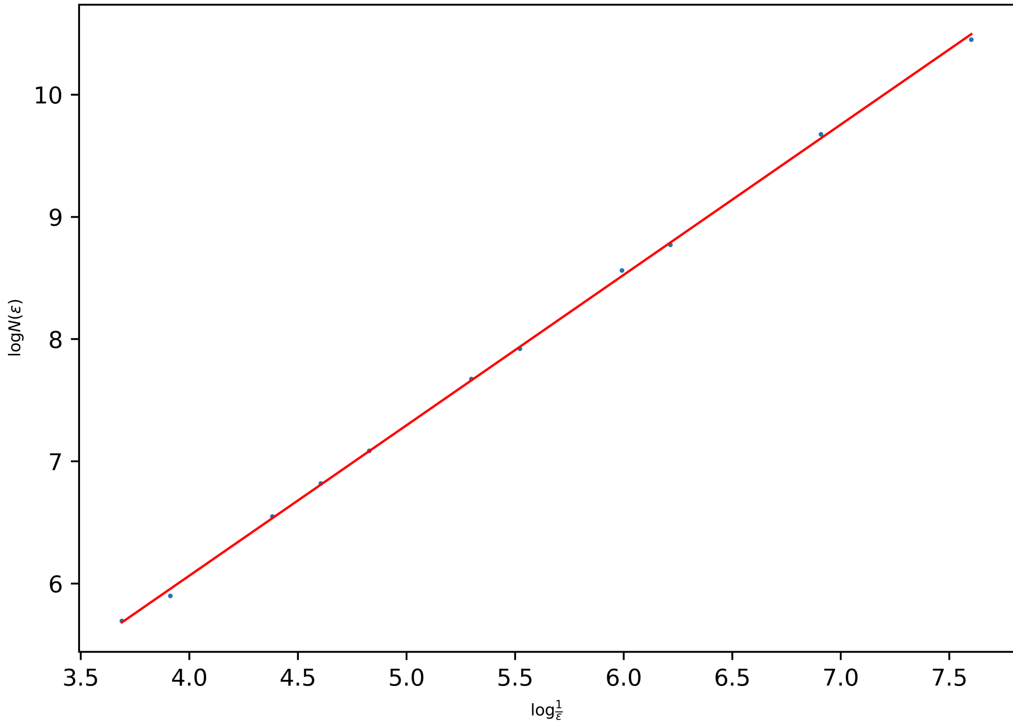
Power-Law of the BC-Dimension of the Snowflake (Level 8): 1.2305983742138389
