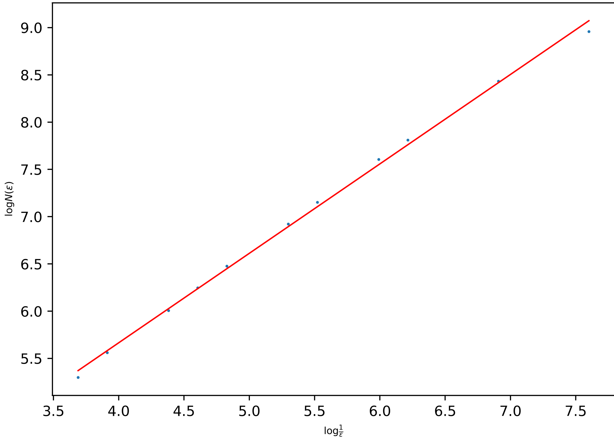
Power-Law of the BC-Dimension of the Snowflake (Level 3): 0.9463799089223158
