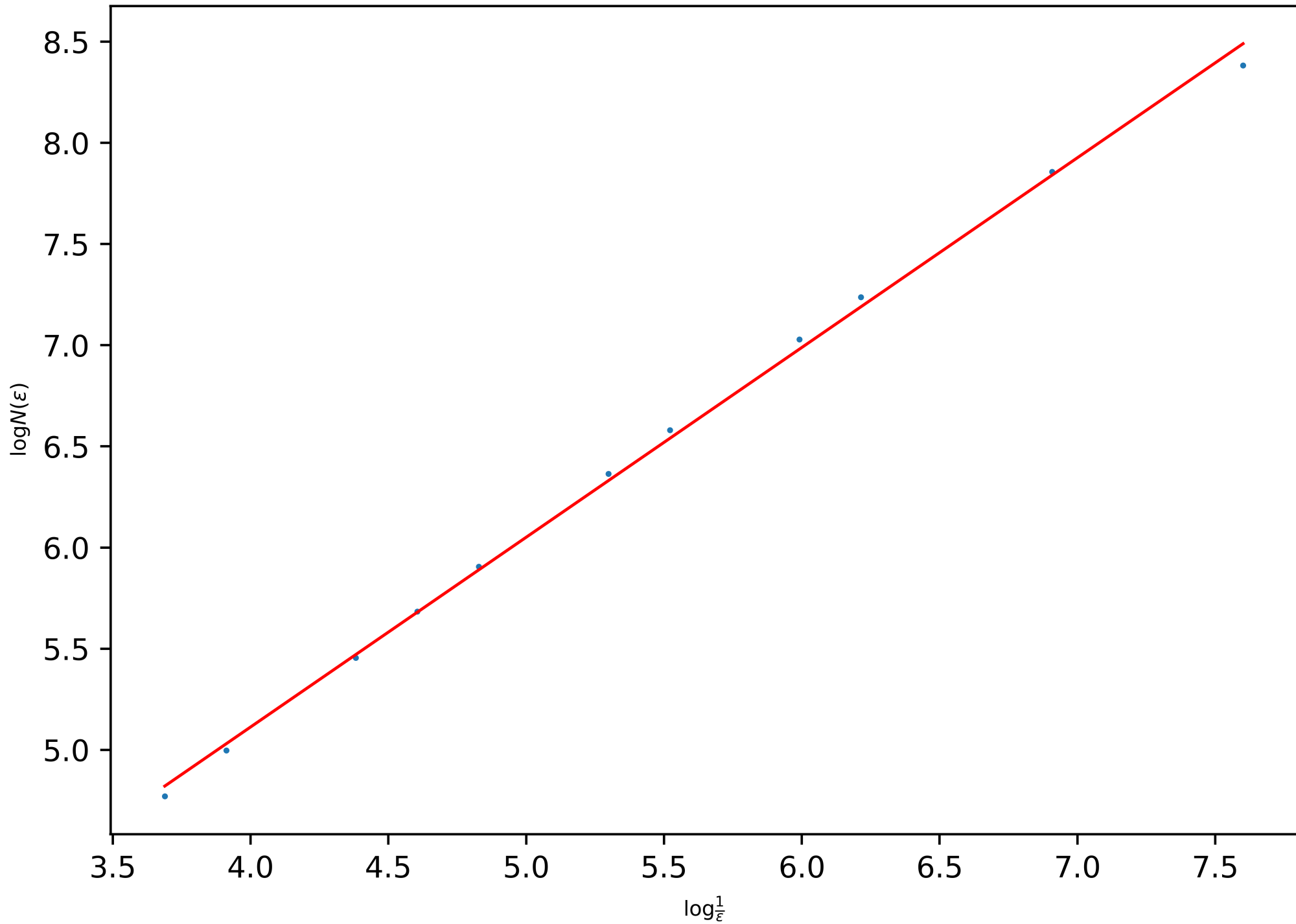
Power-Law of the BC-Dimension of the Snowflake (Level 1): 0.9378169076311864
