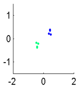
Eigval2871.4109
