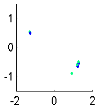
Eigval91515.464
