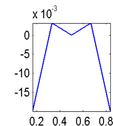
Eigval7316.4208
