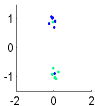
Eigval29512.7918
