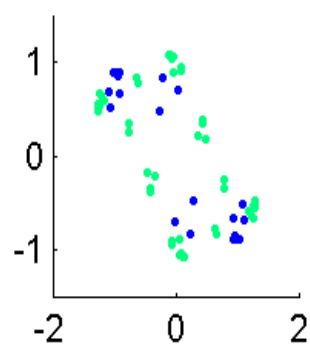
Eigval7316.4208
