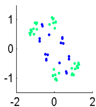
Eigval2102.1511
