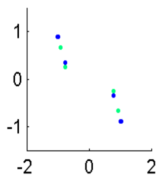
Eigval29512.7716
