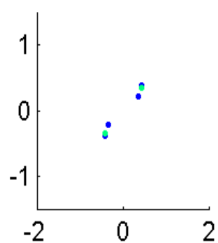
Eigval91515.464
