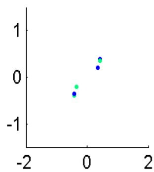
Eigval73353.1621
