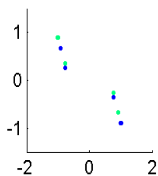
Eigval28525.495
