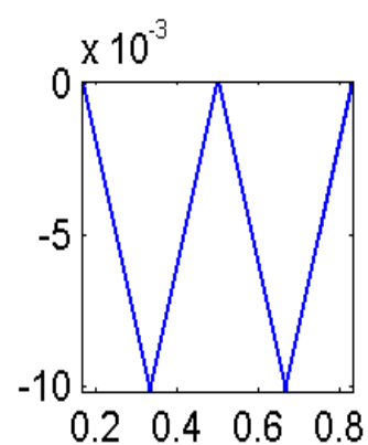
Eigval73353.1621
