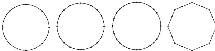
Figure 7: Interpolation using ENO. Interpolated circle, using 8, 16, and 24 points. Interpolated octagon using 16 points.
