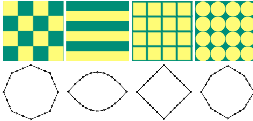
Figure 8: Period domains and computed vectograms: checkerboard, stripes, squares, and circles.
