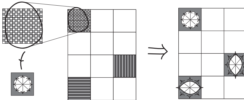
Figure 5: The three scale problem (left), result of homogenization in each medium scale cell (right) fig:3scaleSol
