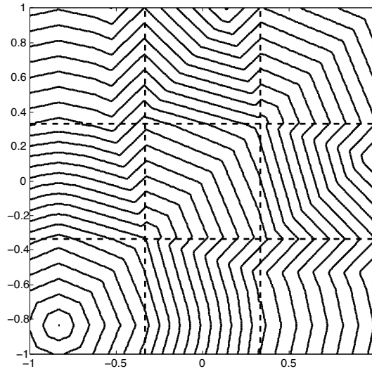
Figure 11: Level sets of the homogenized solution T(x) . The dotted lines are the interfaces where the periodic pattern changes.
