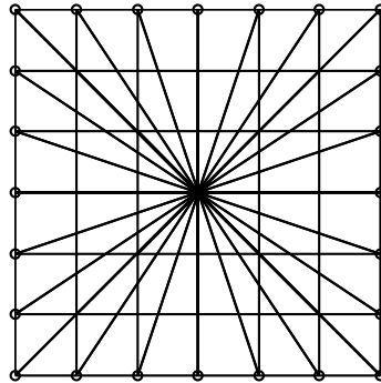
Figure 12: The grid directions \{q_i\} .
