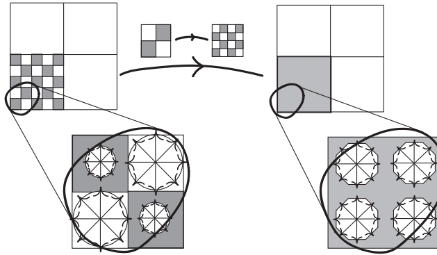
Figure 3: Homogenization of the checkerboard material, illustrated with vectograms.
