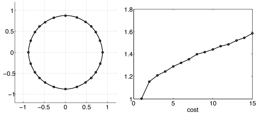
Figure 14: Illustration of the homogenized speed/cost in the random case. Left: computed vectogram, averaged over several trials, for c = 1, 1/2 with probability 1/2 . Right: computed homogenized cost \bar{b} as a function of the random cost b = 1 , or b = b_0 = 1/c_0 with probability 1/2 .
