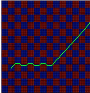
Figure 2: An optimal path in the (2, 1) direction for the checkerboard material.
