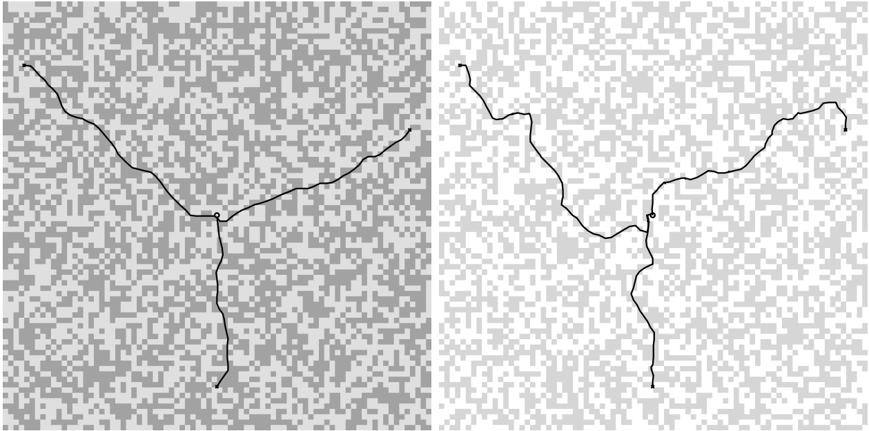
Figure 4: Optimal paths in a random media. The particle speed is c_0 > 1 in the dark and 1 in the light region. Left: c_0 = 2 . Right: c_0 = 10 . fig:randomPath
