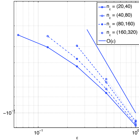
Figure 13: Convergence rate in \epsilon for various cell resolutions n_\epsilon .
