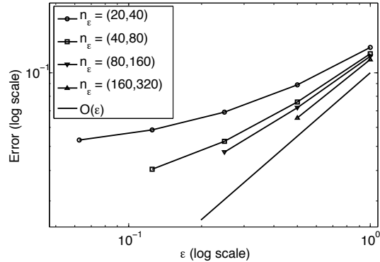
Figure 13: Convergence rate in \epsilon for various cell resolutions n_\epsilon .
